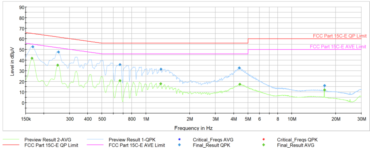
Plot 6-5. AC Line Conducted Plot (L1, Charging Rate 10C, with AC/DC Adapter)
