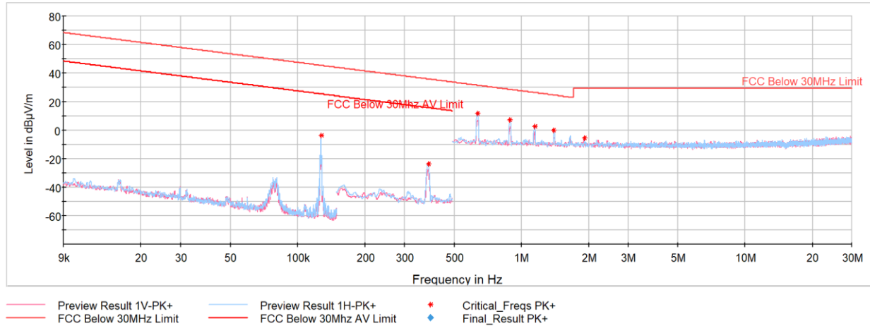
Plot 6-3. Radiated Spurious Emissions 9kHz-30MHz (Charging Rate 10C, with AC/DC Adapter)
