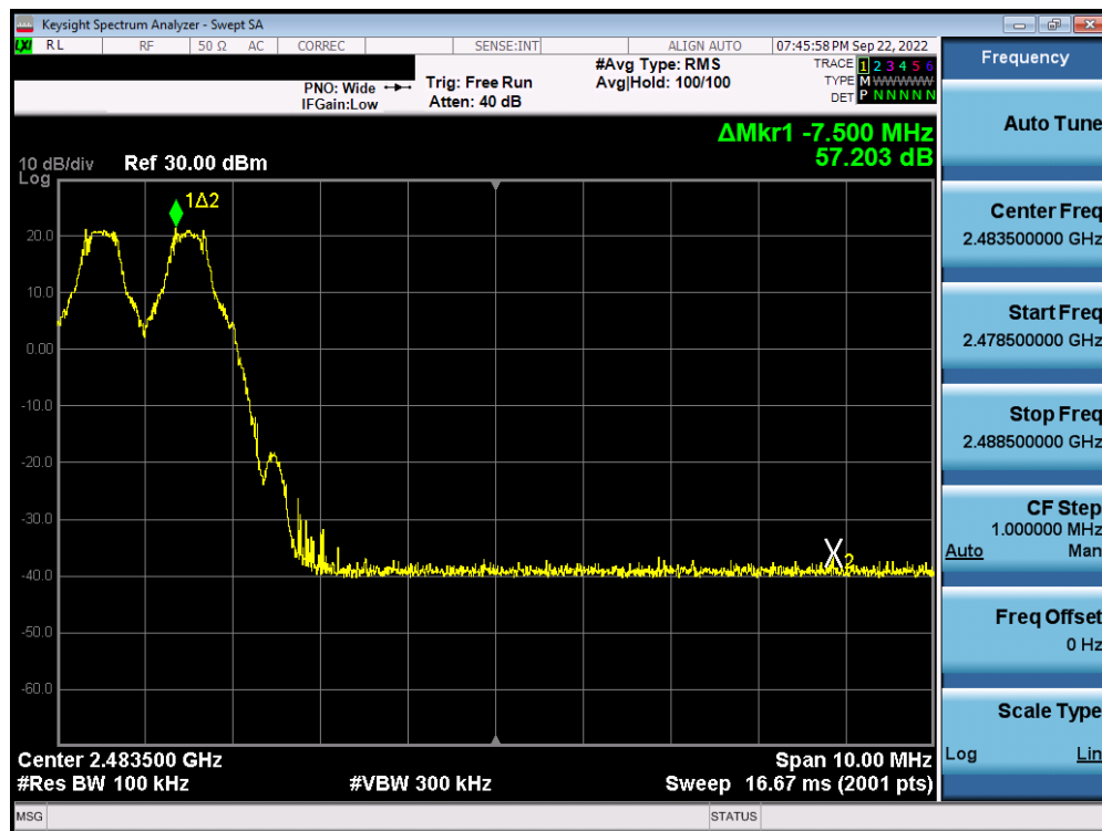
Plot 7-16. Band Edge Plot Antenna 4a (Bluetooth with Hopping Enabled, GFSK, ePA, 2.4GHz)
