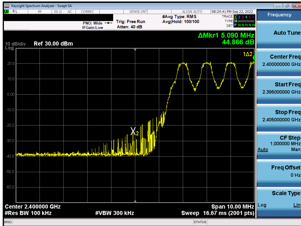
Plot 7-23. Band Edge Plot Antenna 2a (Bluetooth with Hopping Enabled, GFSK, ePA, 2.4GHz)
