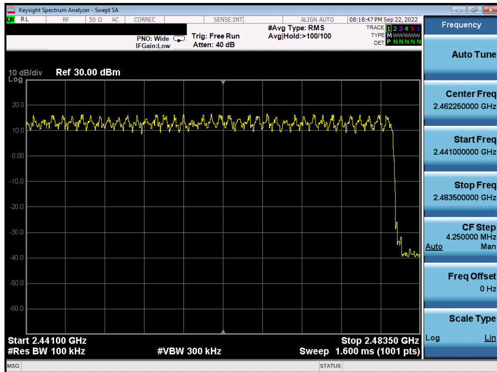
Plot 7-44. High End Spectrum Channel Hopping Plot Antenna 2a (Bluetooth, 8DPSK, ePA, 2.4GHz)
