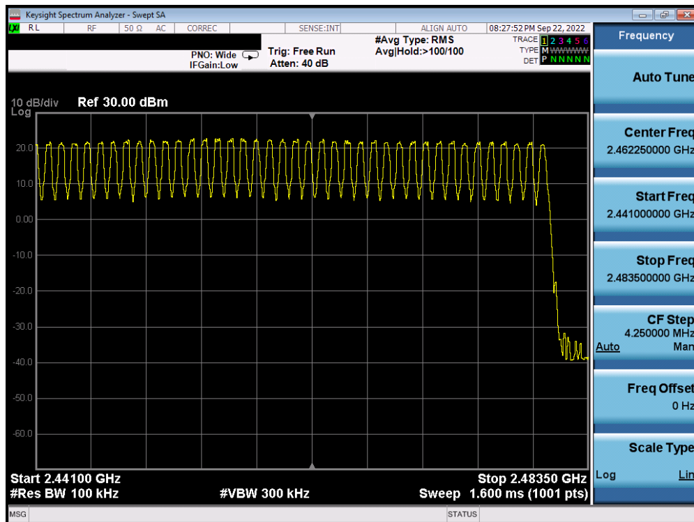
Plot 7-42. High End Spectrum Channel Hopping Plot Antenna 2a (Bluetooth, GFSK, ePA, 2.4GHz)
