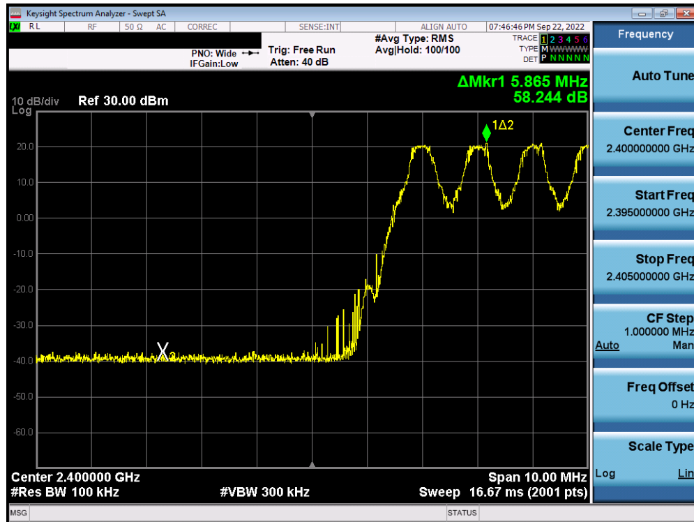
Plot 7-15. Band Edge Plot Antenna 4a (Bluetooth with Hopping Enabled, GFSK, ePA, 2.4GHz)
