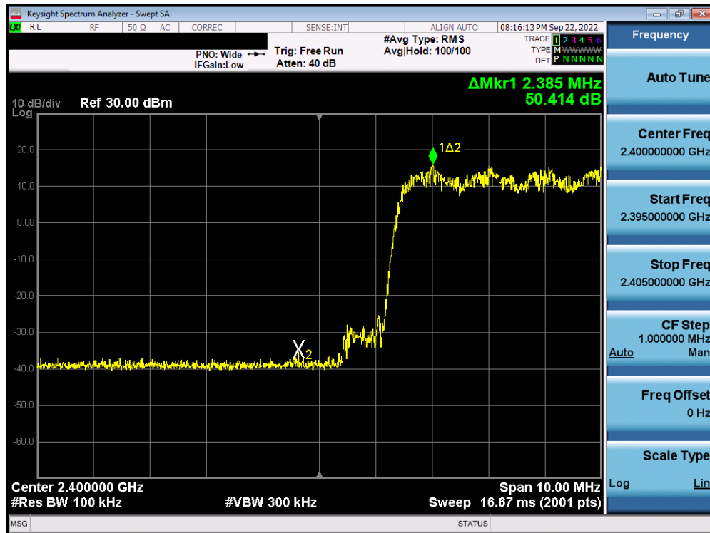
Plot 7-27. Band Edge Plot Antenna 2a (Bluetooth with Hopping Enabled, 8DPSK, ePA, 2.4GHz)
