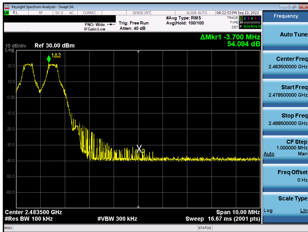
Plot 7-24. Band Edge Plot Antenna 2a (Bluetooth with Hopping Enabled, GFSK, ePA, 2.4GHz)
