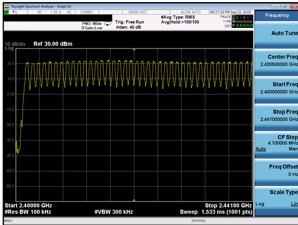
Plot 7-41. Low End Spectrum Channel Hopping Plot Antenna 2a (Bluetooth, GFSK, ePA, 2.4GHz)
