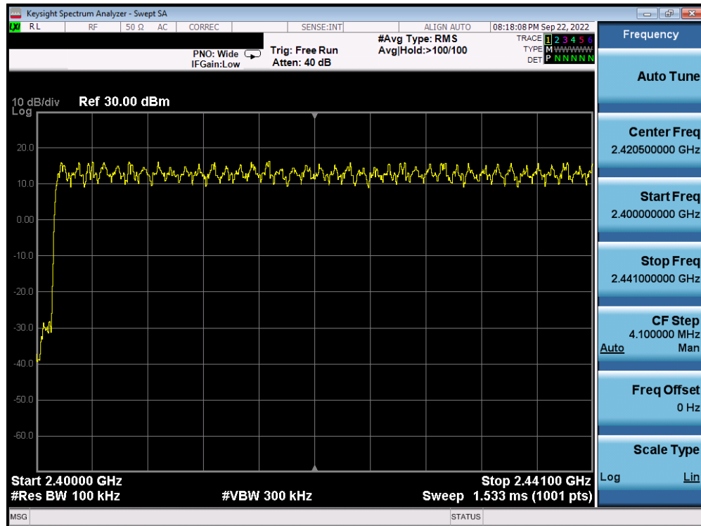
Plot 7-43. Low End Spectrum Channel Hopping Plot Antenna 2a (Bluetooth, 8DPSK, ePA, 2.4GHz)
