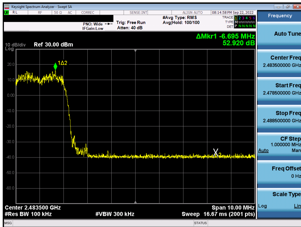
Plot 7-28. Band Edge Plot Antenna 2a (Bluetooth with Hopping Enabled, 8DPSK, ePA, 2.4GHz)
