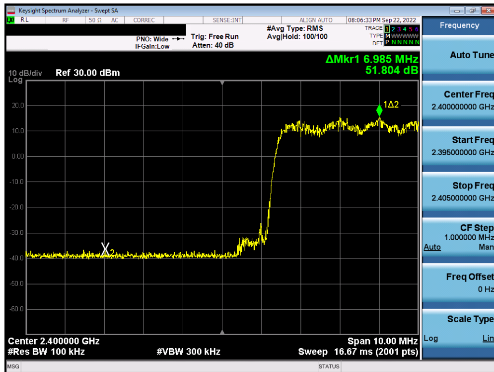
Plot 7-19. Band Edge Plot Antenna 4a (Bluetooth with Hopping Enabled, 8DPSK, ePA, 2.4GHz)
