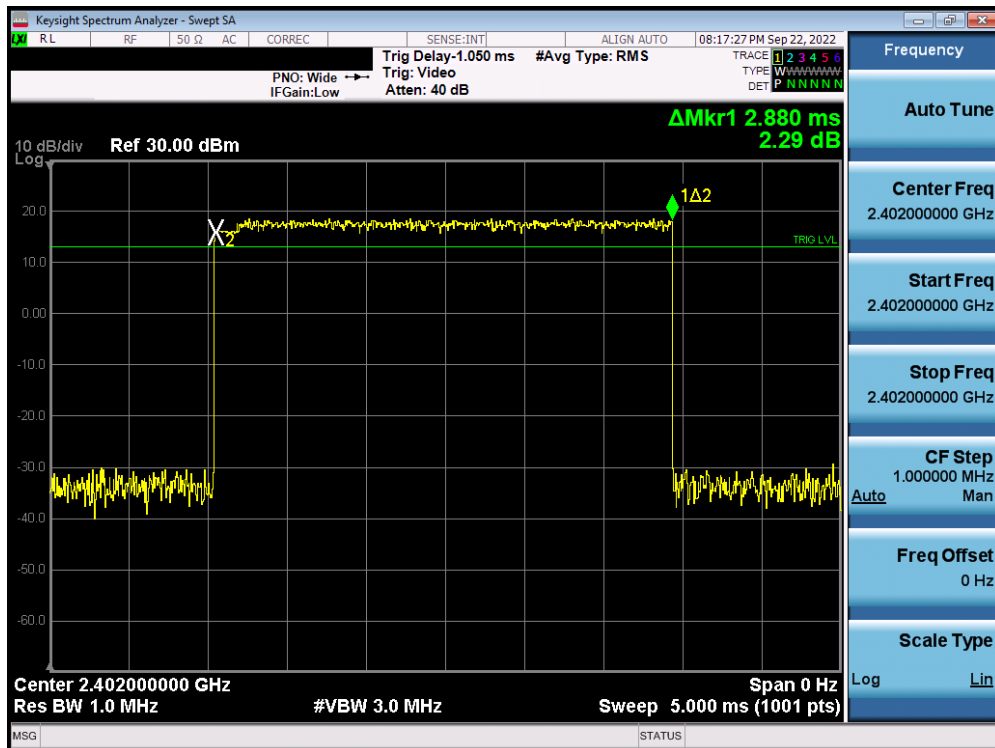
Plot 7-36. Time of Occupancy Plot Antenna 2a (Bluetooth, 8DPSK, ePA, 2.4GHz)
