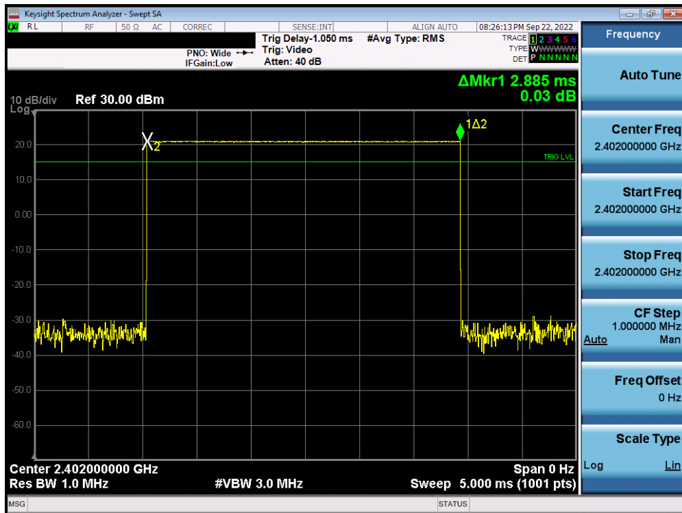
Plot 7-35. Time of Occupancy Plot Antenna 2a (Bluetooth, GFSK, ePA, 2.4GHz)
