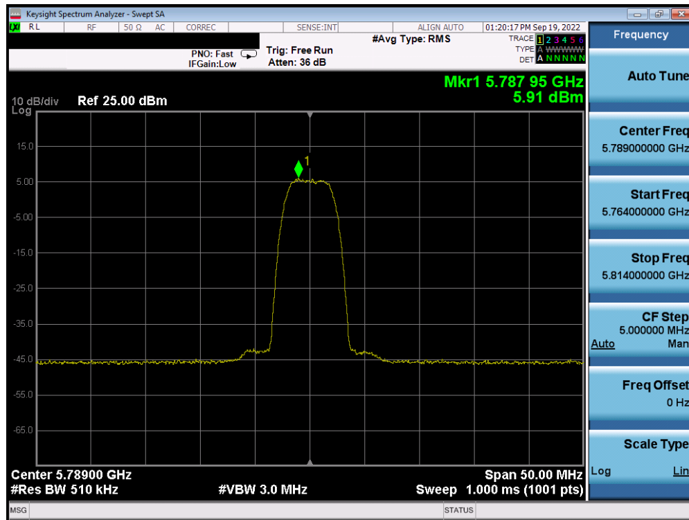
Plot 7-41. PSD Antenna 5b (HDR8, ePA, 5789MHz)
