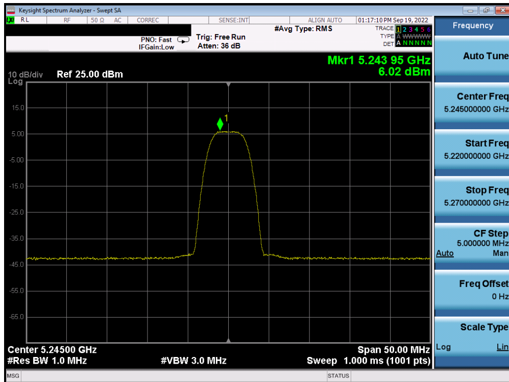
Plot 7-30. PSD Antenna 5b (HDR8, ePA, 5245MHz)
