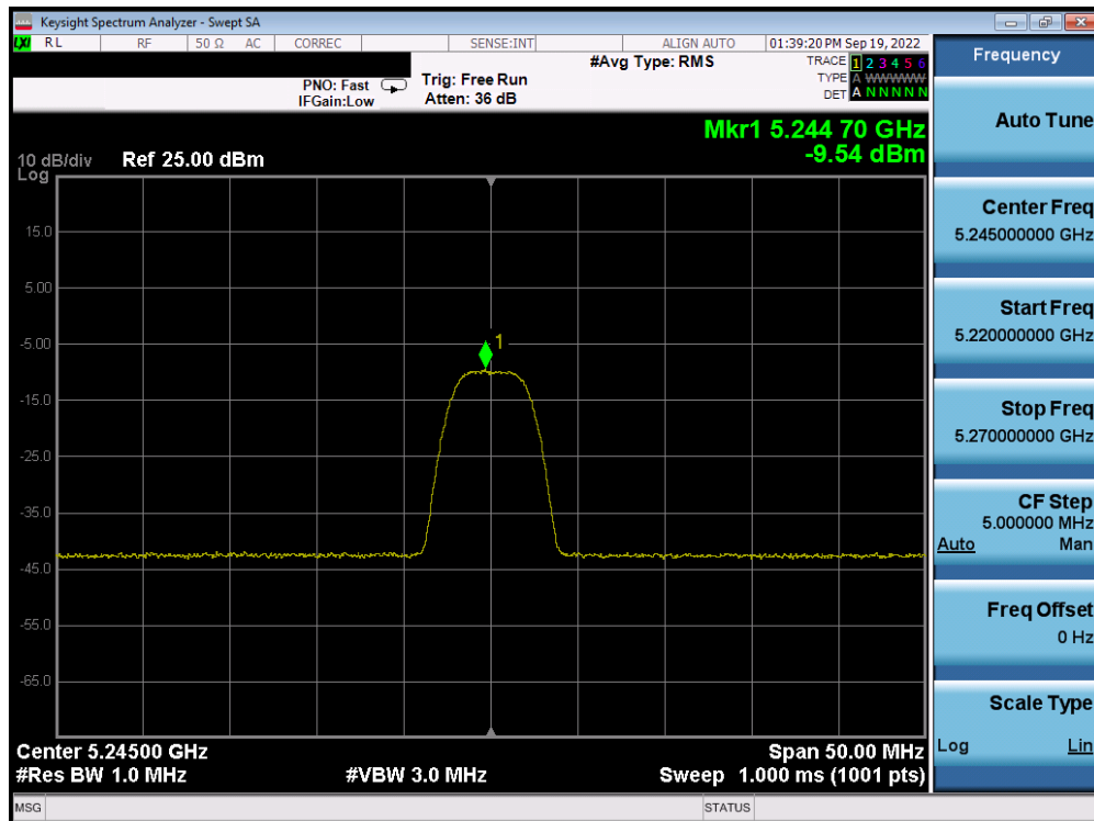
Plot 7-36. PSD Antenna 5b (HDR8, iPA, 5245MHz)
