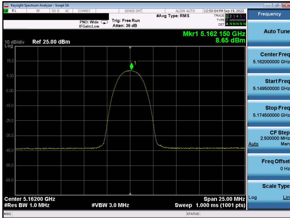
Plot 7-25. PSD Antenna 5b (HDR4, ePA, 5162MHz)
