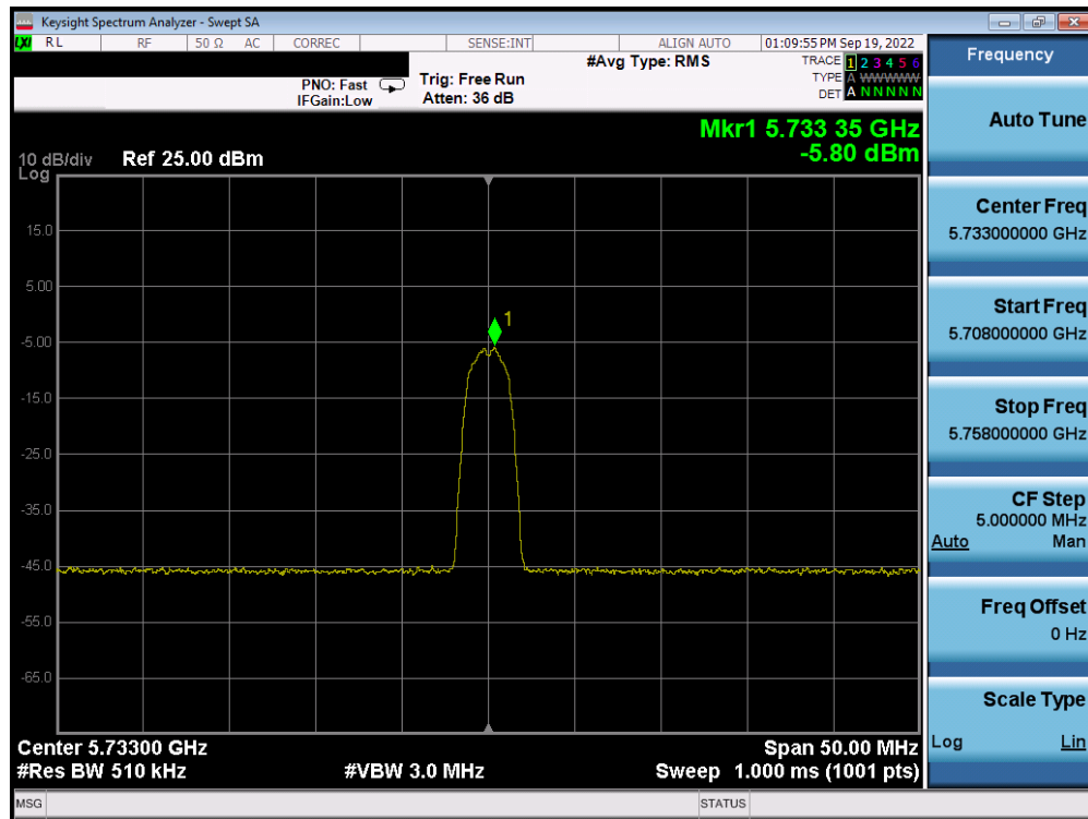
Plot 7-43. PSD Antenna 5b (HDR4, iPA, 5733MHz)
