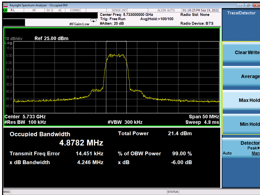
Plot 7-16. 6dB BW & 99% OBW Antenna 5b (HDR8, ePA, 5733MHz)
