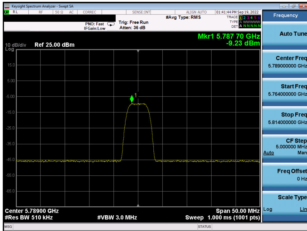
Plot 7-47. PSD Antenna 5b (HDR8, iPA, 5789MHz)
