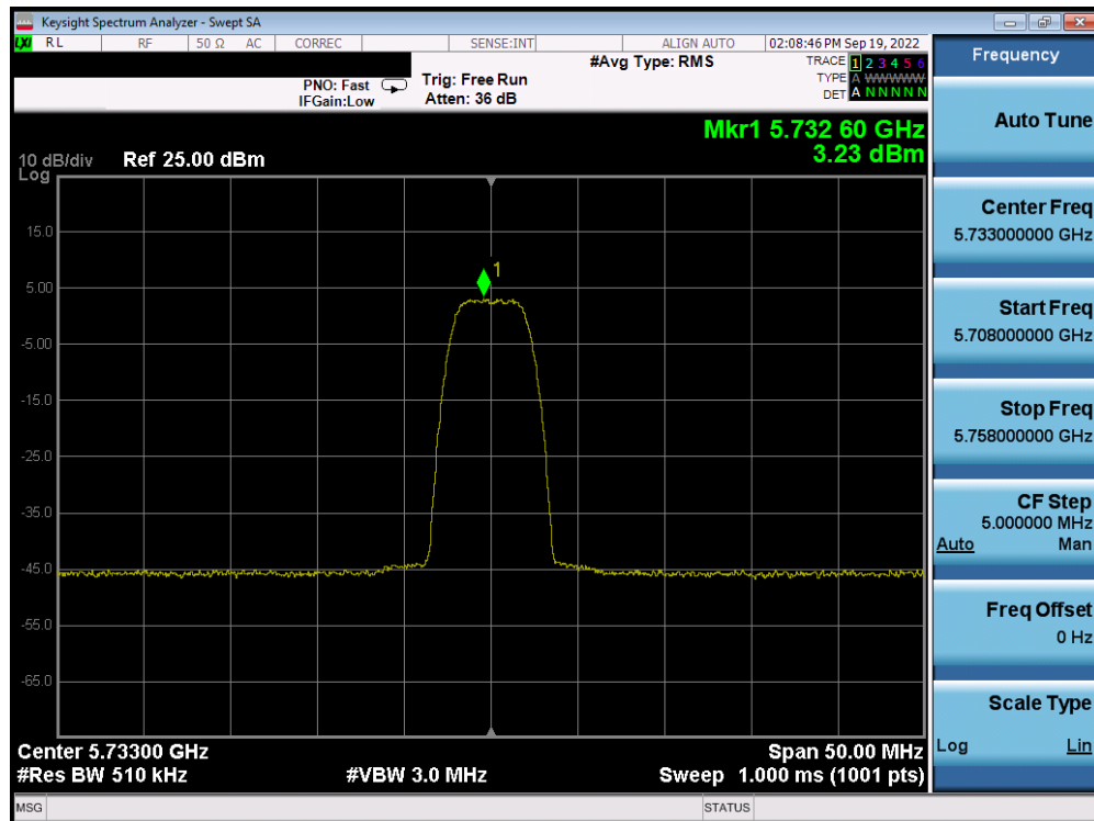
Plot 7-64. PSD Antenna 4a (HDR8, ePA, 5733MHz)
