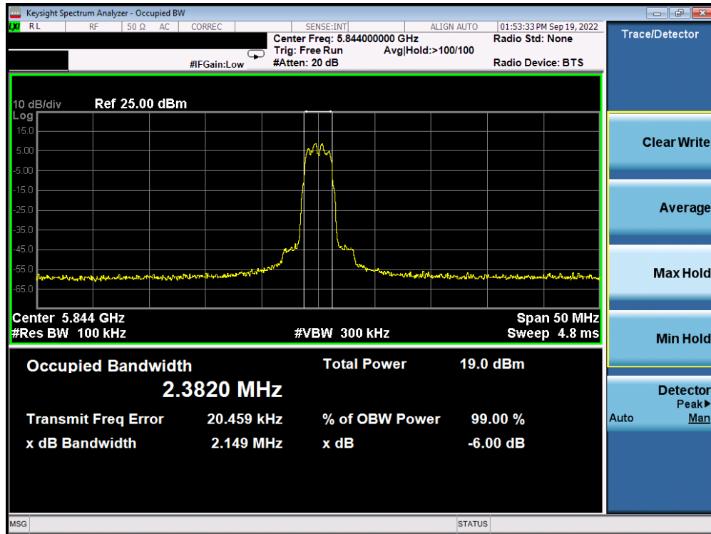
Plot 7-21. 6dB BW & 99% OBW Antenna 4a (HDR4, ePA, 5844MHz)
