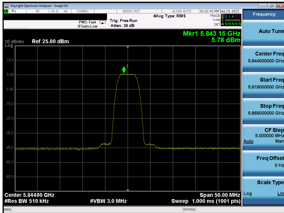
Plot 7-42. PSD Antenna 5b (HDR8, ePA, 5844MHz)
