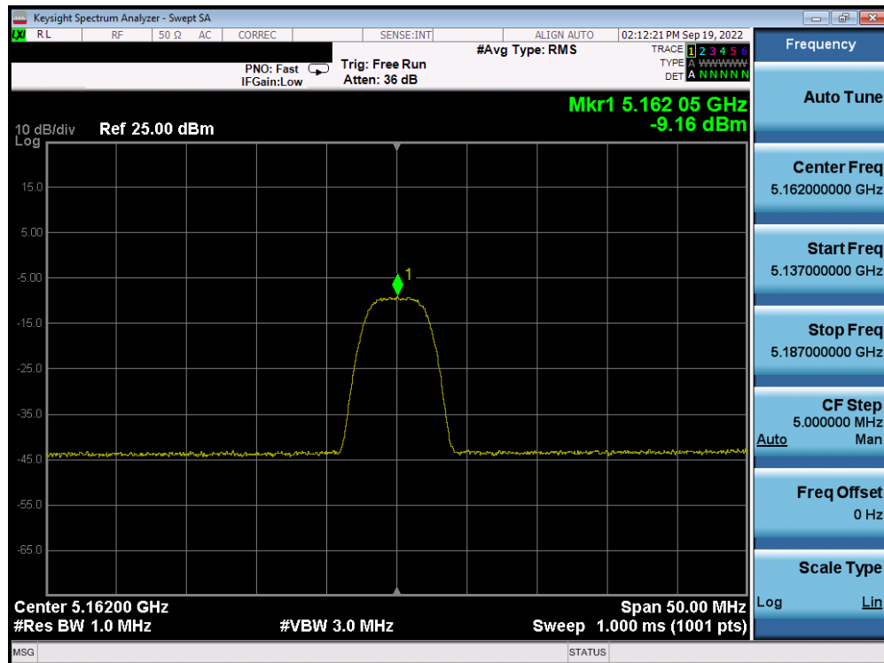
Plot 7-58. PSD Antenna 4a (HDR8, iPA, 5162MHz)
