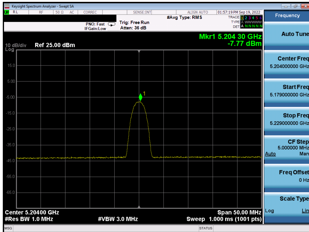
Plot 7-56. PSD Antenna 4a (HDR4, iPA, 5204MHz)
