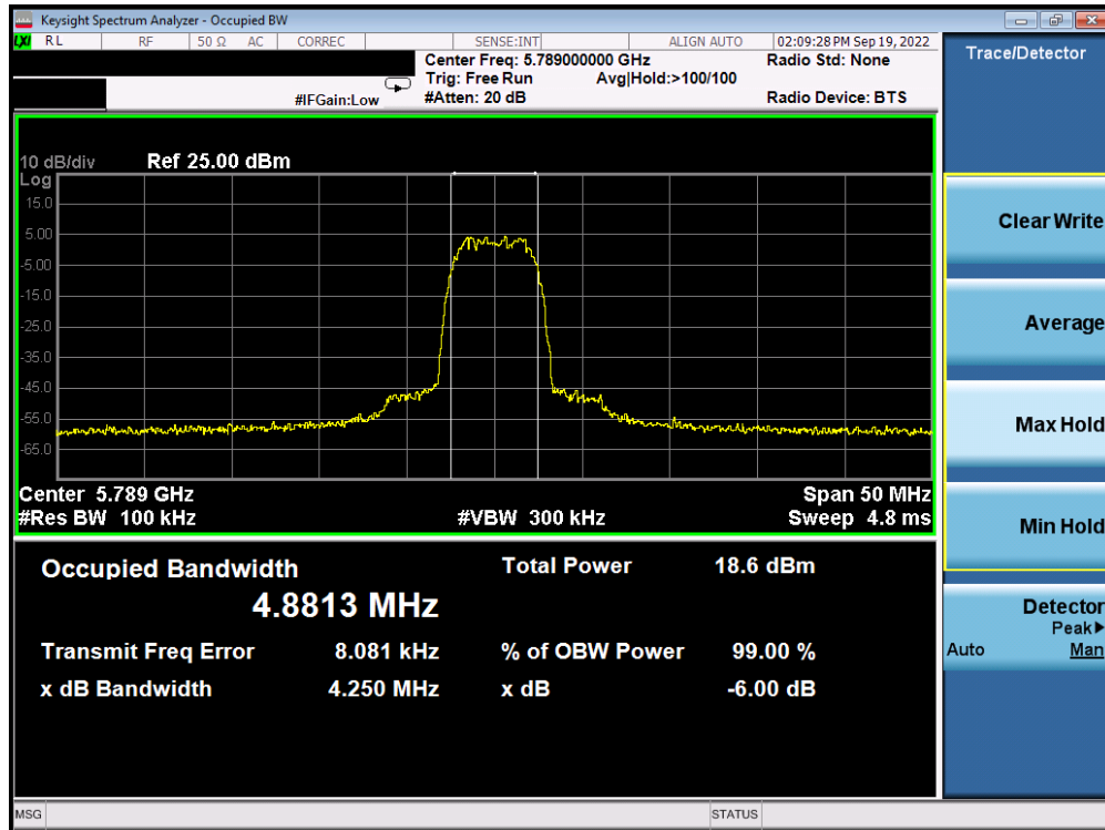
Plot 7-23. 6dB BW & 99% OBW Antenna 4a (HDR8, ePA, 5789MHz)
