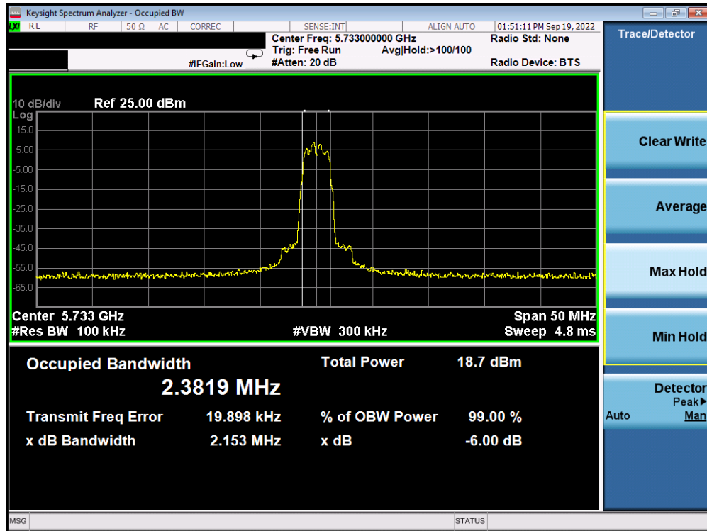
Plot 7-19. 6dB BW & 99% OBW Antenna 4a (HDR4, ePA, 5733MHz)
