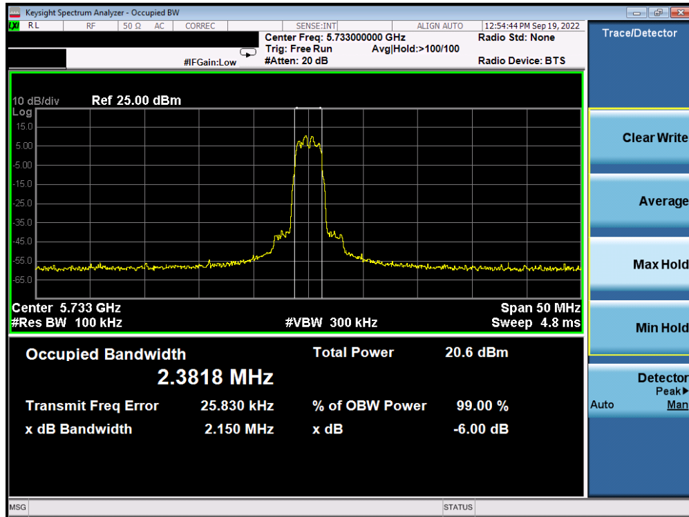
Plot 7-13. 6dB BW & 99% OBW Antenna 5b (HDR4, ePA, 5733MHz)
