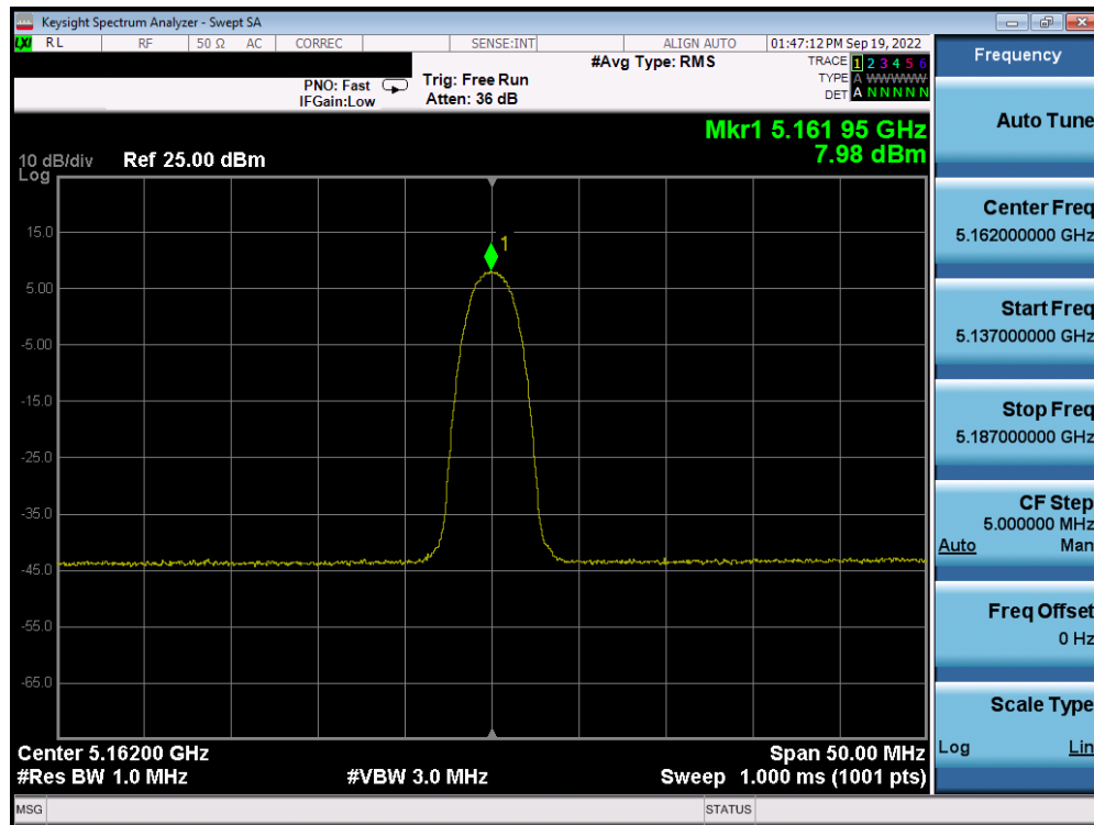
Plot 7-49. PSD Antenna 4a (HDR4, ePA, 5162MHz)
