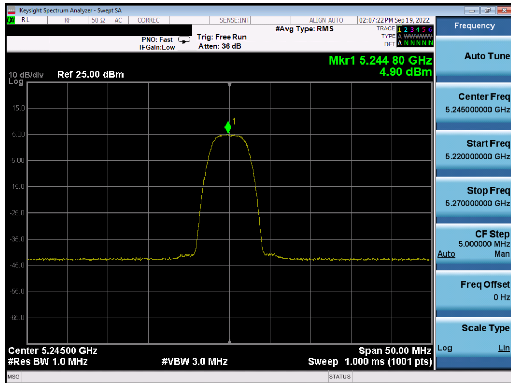
Plot 7-54. PSD Antenna 4a (HDR8, ePA, 5245MHz)
