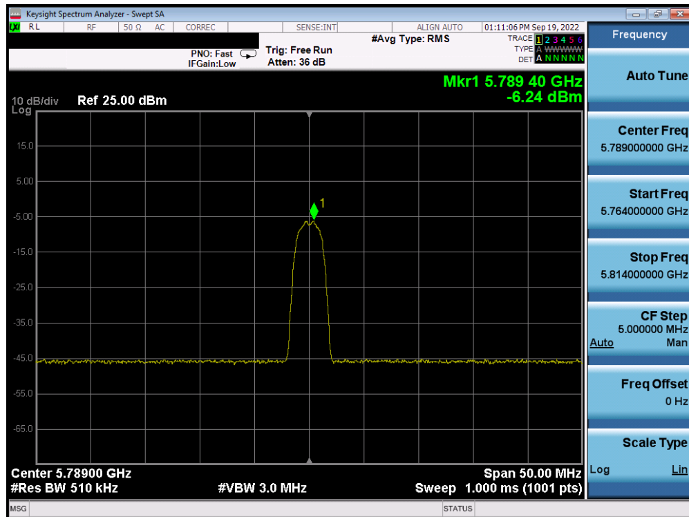
Plot 7-44. PSD Antenna 5b (HDR4, iPA, 5789MHz)
