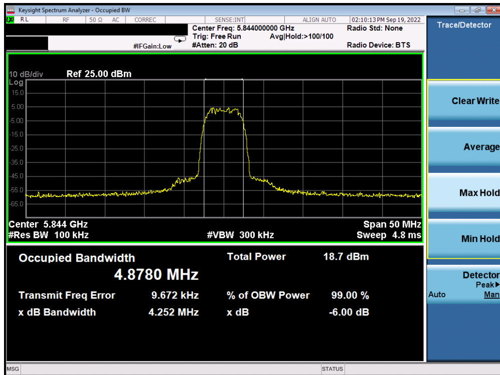
Plot 7-24. 6dB BW & 99% OBW Antenna 4a (HDR8, ePA, 5844MHz)
