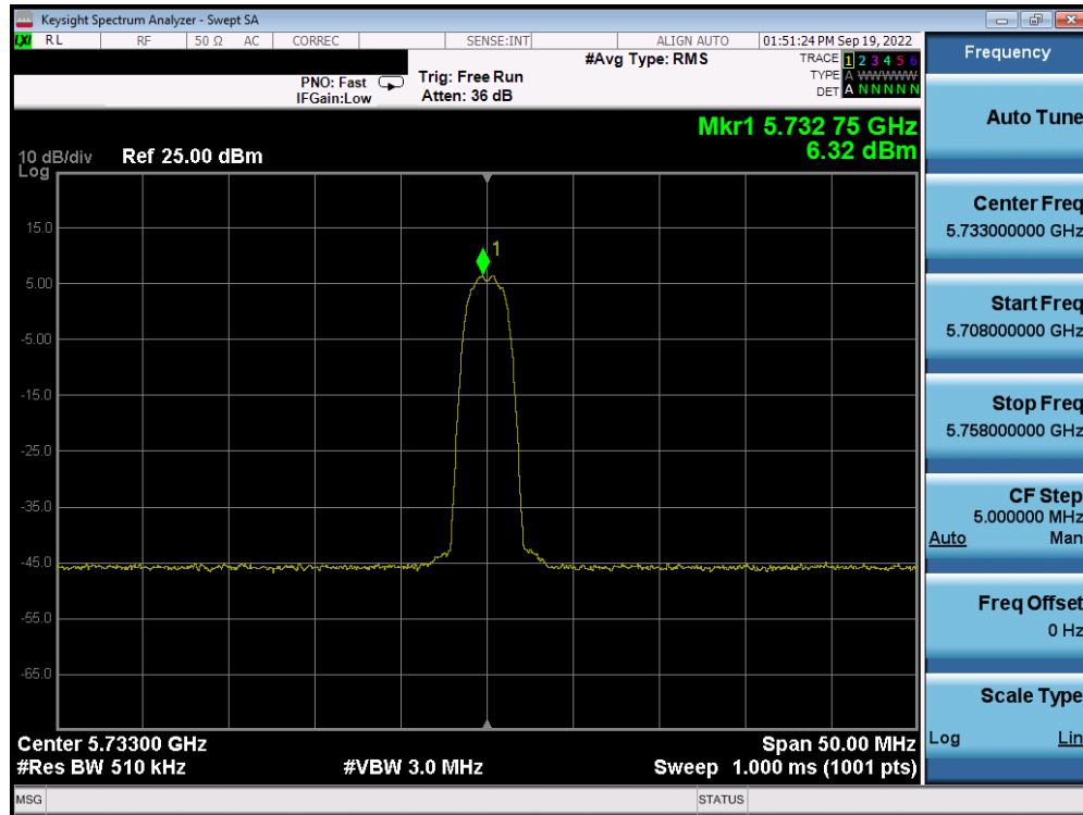
Plot 7-61. PSD Antenna 4a (HDR4, ePA, 5733MHz)
