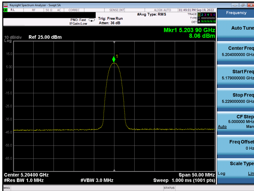
Plot 7-50. PSD Antenna 4a (HDR4, ePA, 5204MHz)
