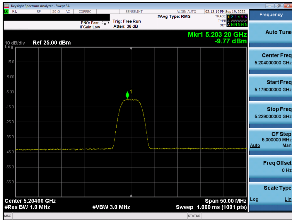
Plot 7-59. PSD Antenna 4a (HDR8, iPA, 5204MHz)
