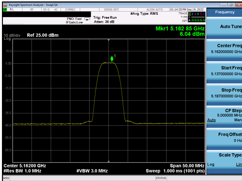
Plot 7-28. PSD Antenna 5b (HDR8, ePA, 5162MHz)
