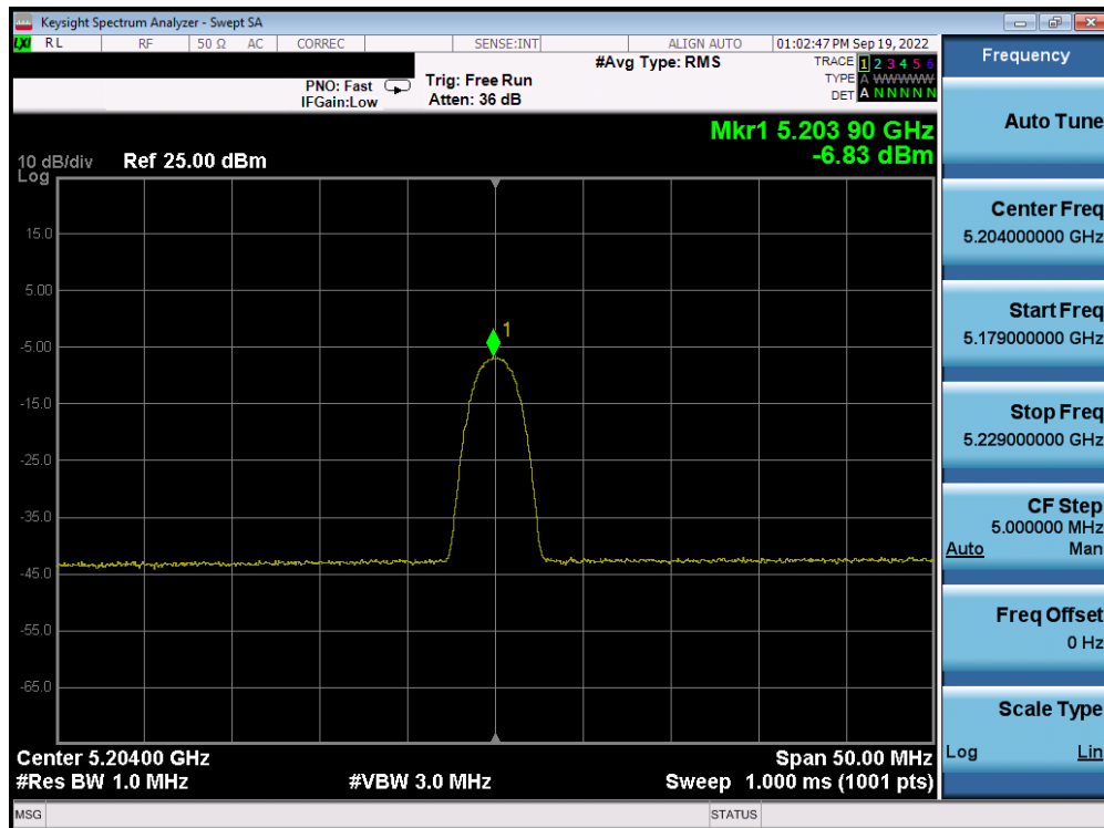
Plot 7-32. PSD Antenna 5b (HDR4, iPA, 5204MHz)
