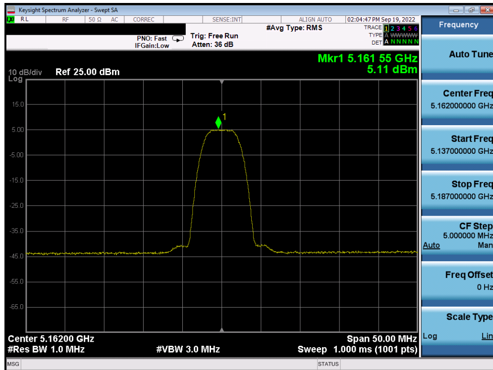
Plot 7-52. PSD Antenna 4a (HDR8, ePA, 5162MHz)
