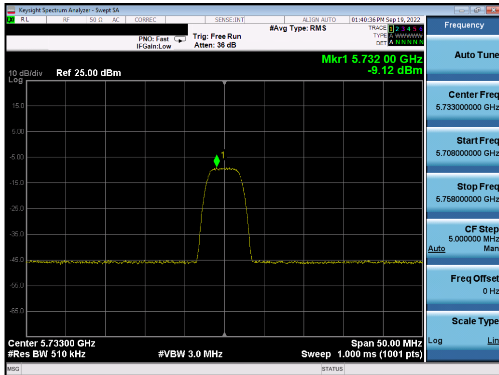
Plot 7-46. PSD Antenna 5b (HDR8, iPA, 5733MHz)
