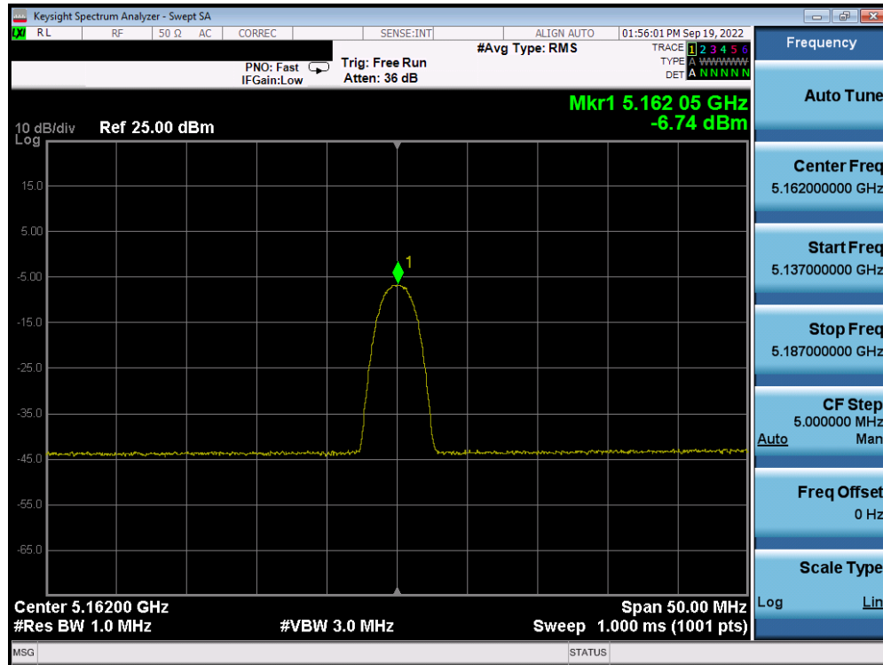
Plot 7-55. PSD Antenna 4a (HDR4, iPA, 5162MHz)
