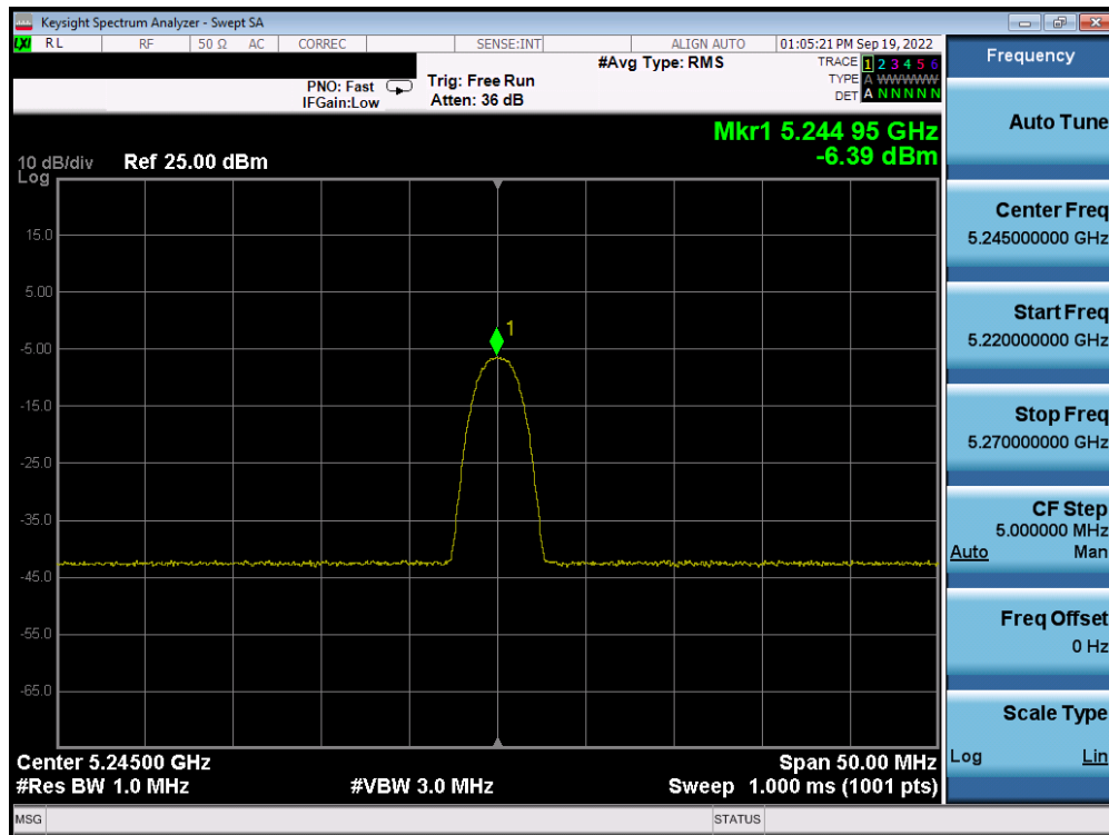
Plot 7-33. PSD Antenna 5b (HDR4, iPA, 5245MHz)
