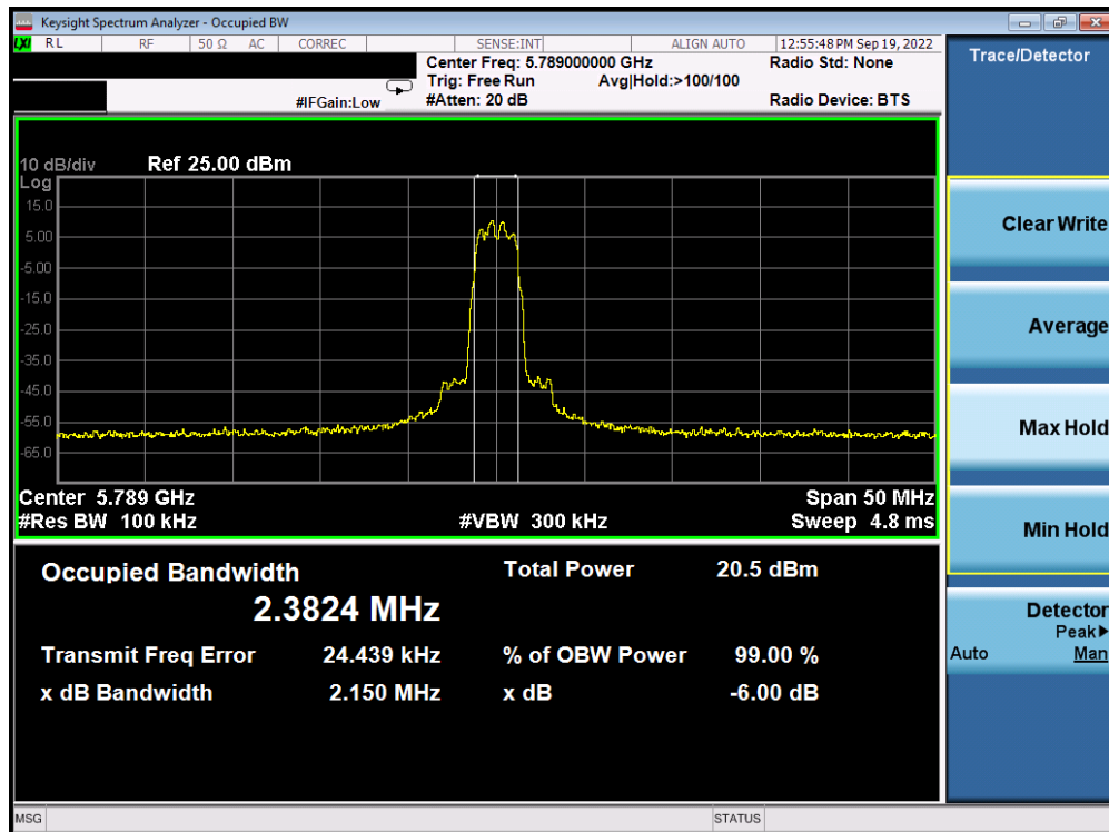
Plot 7-14. 6dB BW & 99% OBW Antenna 5b (HDR4, ePA, 5789MHz)
