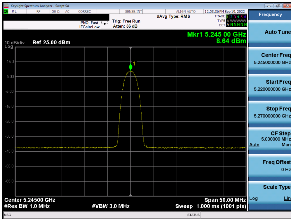
Plot 7-27. PSD Antenna 5b (HDR4, ePA, 5245MHz)
