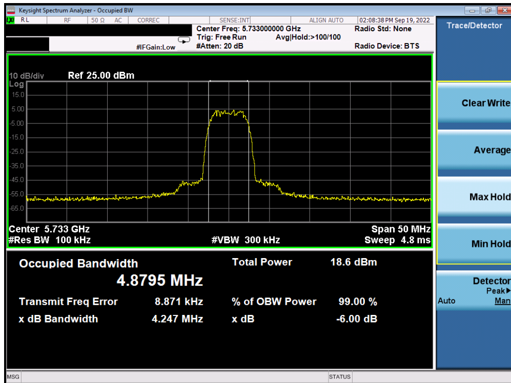
Plot 7-22. 6dB BW & 99% OBW Antenna 4a (HDR8, ePA, 5733MHz)
