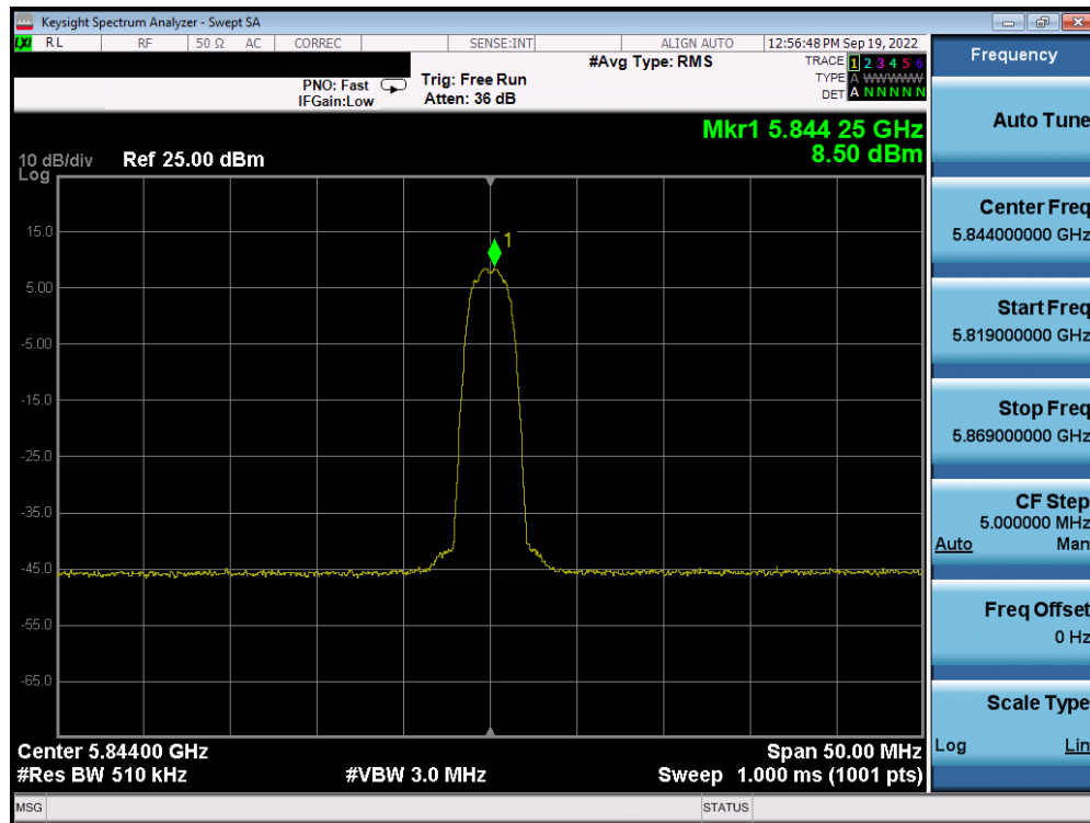
Plot 7-39. PSD Antenna 5b (HDR4, ePA, 5844MHz)
