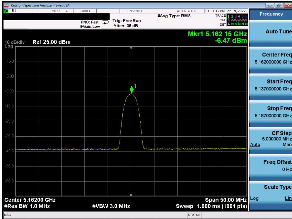
Plot 7-31. PSD Antenna 5b (HDR4, iPA, 5162MHz)
