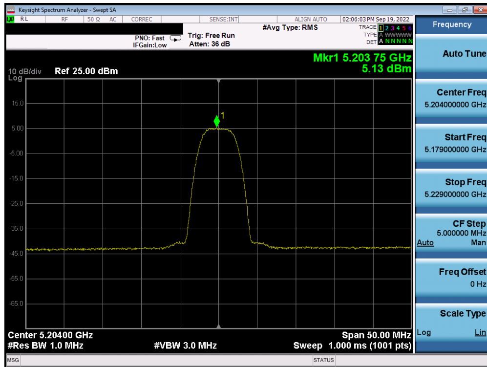
Plot 7-53. PSD Antenna 4a (HDR8, ePA, 5204MHz)
