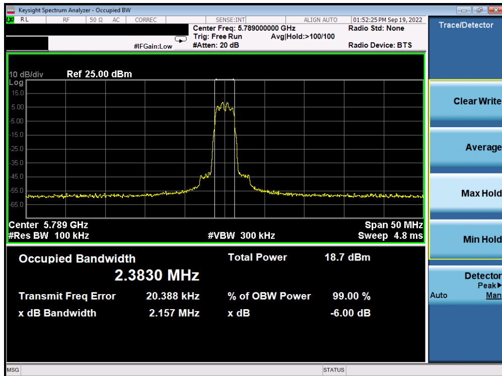
Plot 7-20. 6dB BW & 99% OBW Antenna 4a (HDR4, ePA, 5789MHz)
