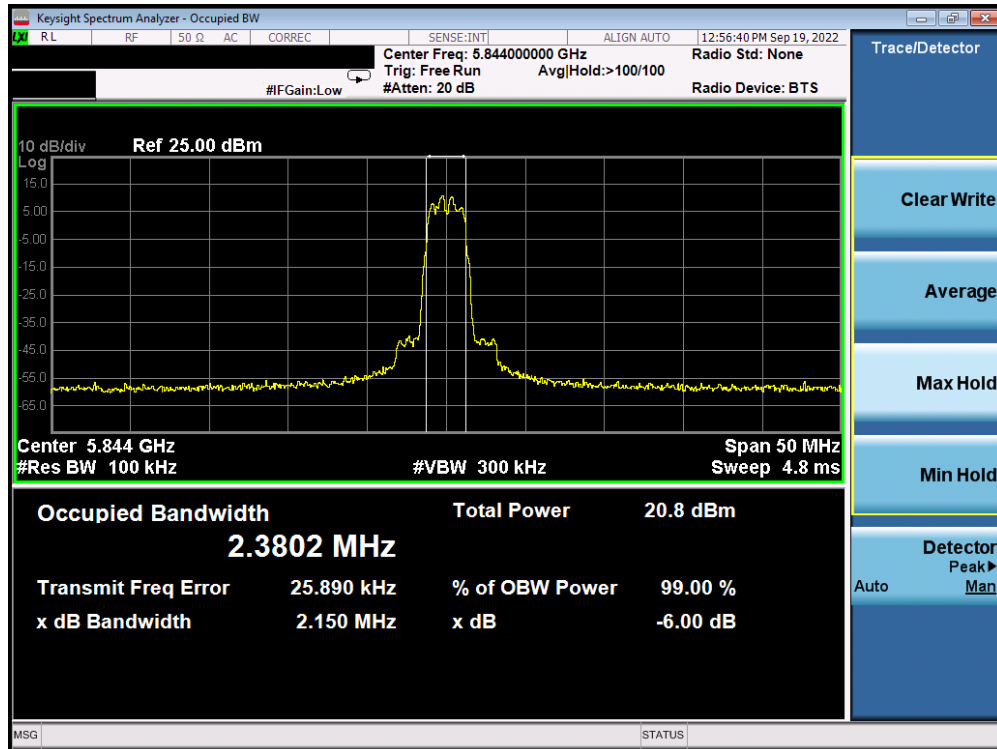
Plot 7-15. 6dB BW & 99% OBW Antenna 5b (HDR4, ePA, 5844MHz)
