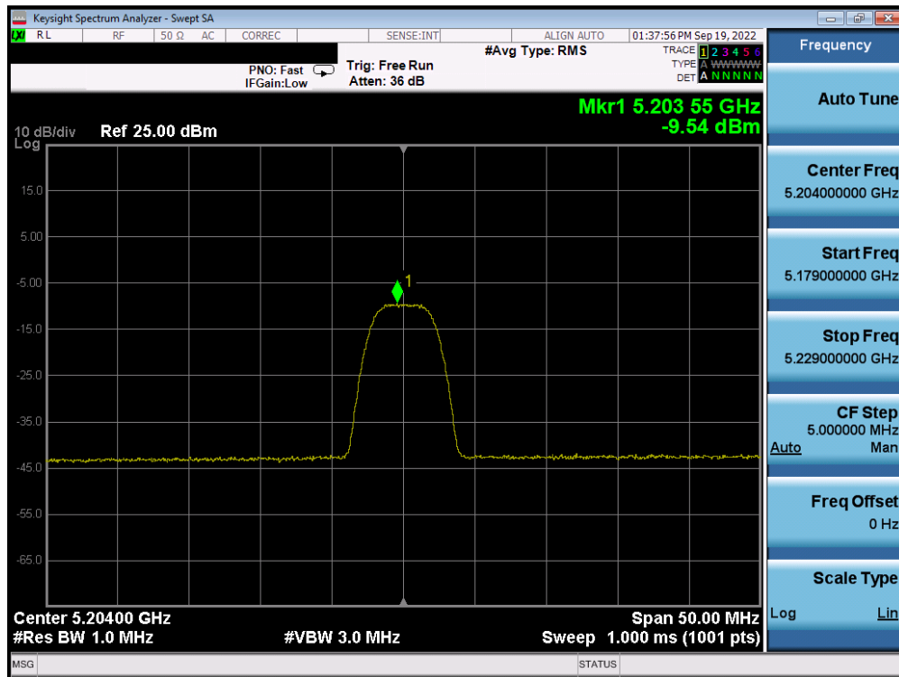
Plot 7-35. PSD Antenna 5b (HDR8, iPA, 5204MHz)
