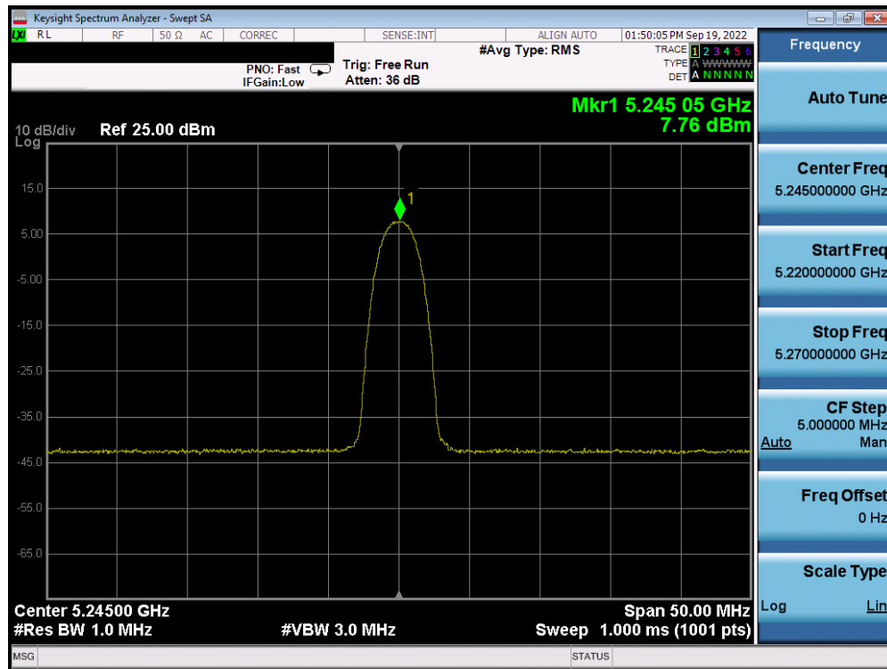
Plot 7-51. PSD Antenna 4a (HDR4, ePA, 5245MHz)
