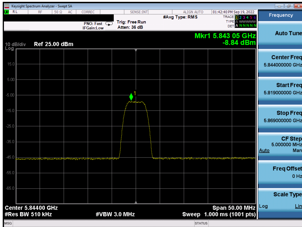
Plot 7-48. PSD Antenna 5b (HDR8, iPA, 5844MHz)
