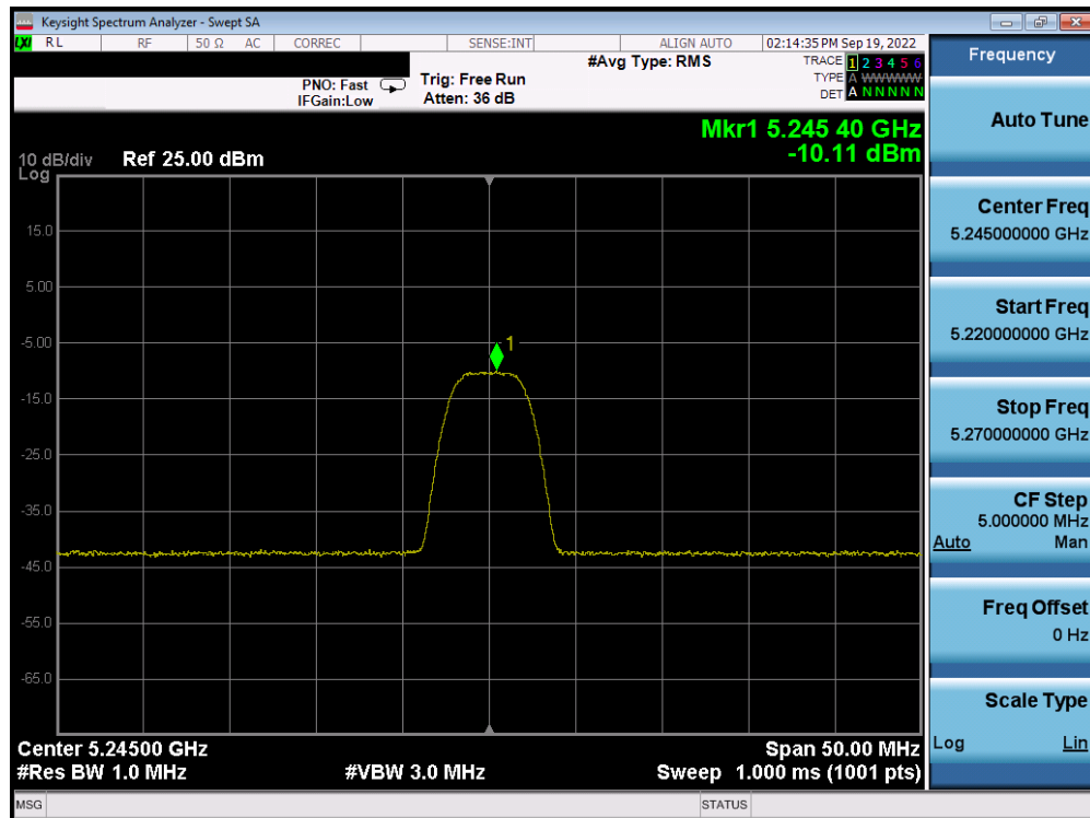
Plot 7-60. PSD Antenna 4a (HDR8, iPA, 5245MHz)
