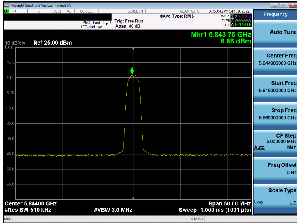
Plot 7-63. PSD Antenna 4a (HDR4, ePA, 5844MHz)
