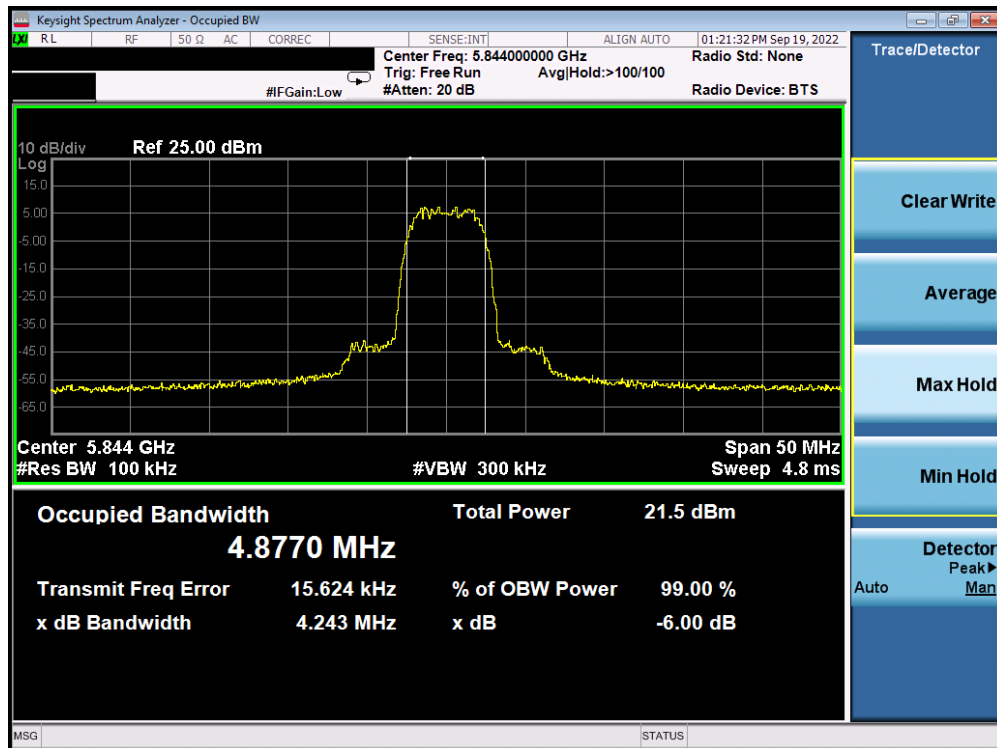
Plot 7-18. 6dB BW & 99% OBW Antenna 5b (HDR8, ePA, 5844MHz)
