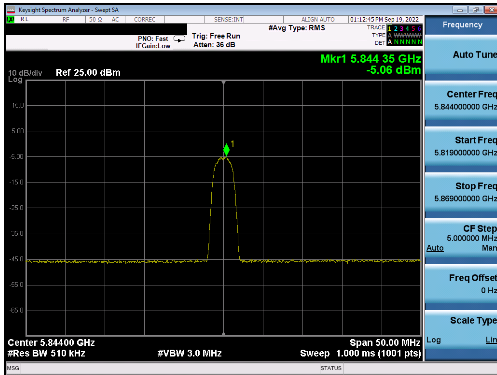
Plot 7-45. PSD Antenna 5b (HDR4, iPA, 5844MHz)
