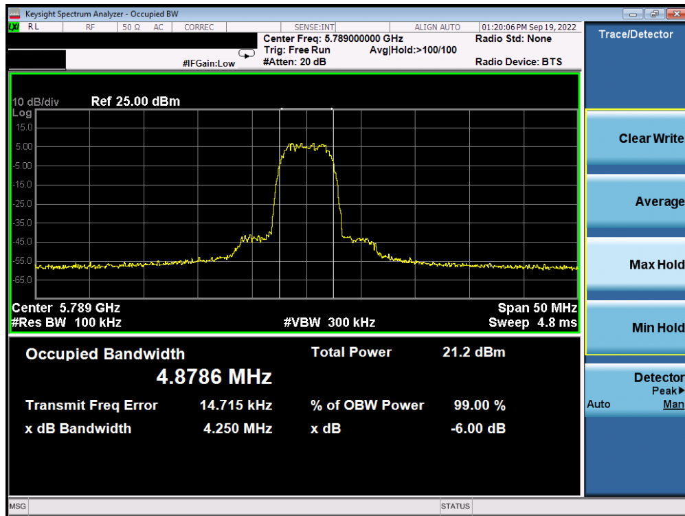
Plot 7-17. 6dB BW & 99% OBW Antenna 5b (HDR8, ePA, 5789MHz)
