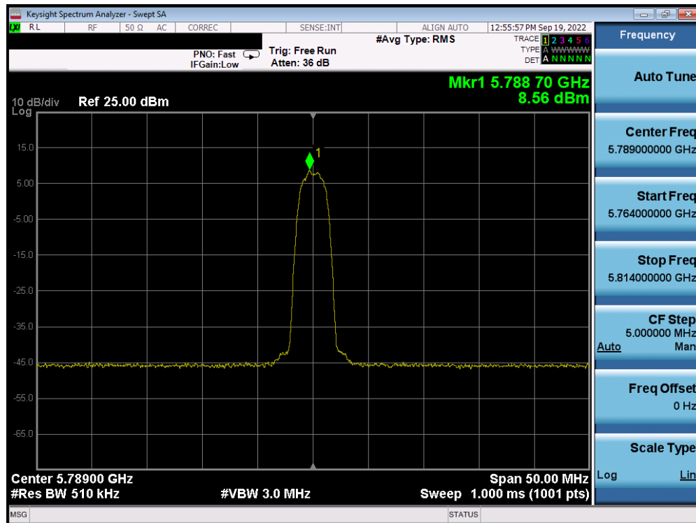
Plot 7-38. PSD Antenna 5b (HDR4, ePA, 5789MHz)
