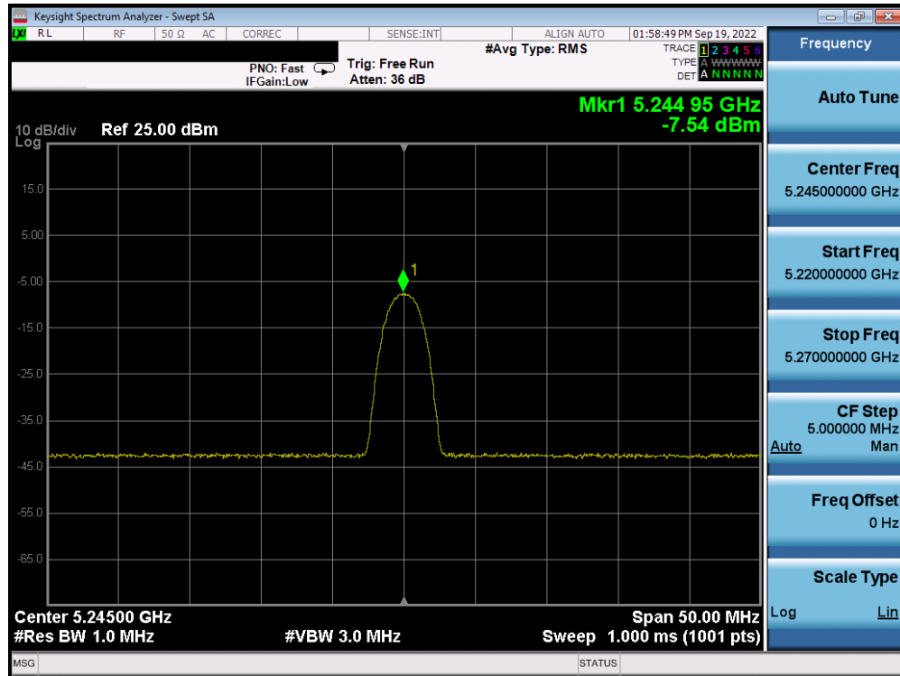
Plot 7-57. PSD Antenna 4a (HDR4, iPA, 5245MHz)
