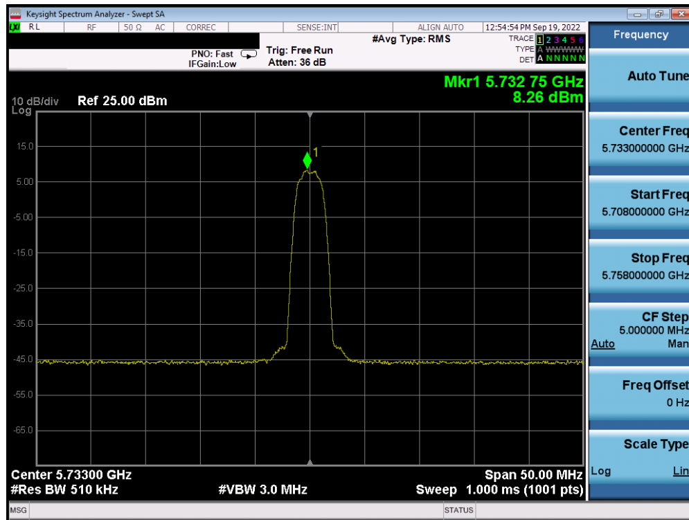
Plot 7-37. PSD Antenna 5b (HDR4, ePA, 5733MHz)
