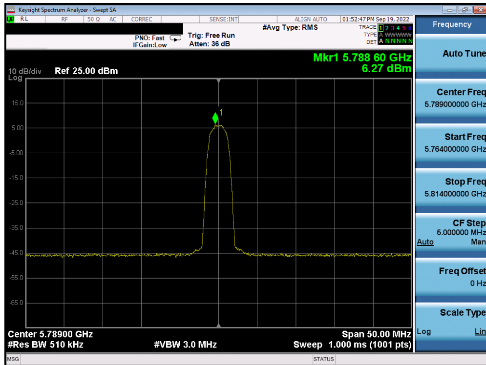
Plot 7-62. PSD Antenna 4a (HDR4, ePA, 5789MHz)
