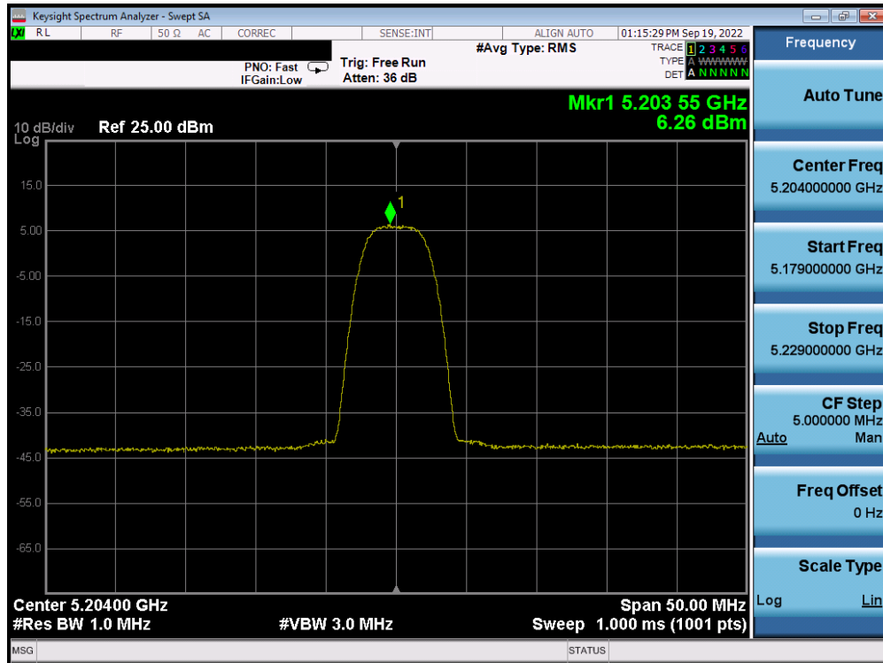
Plot 7-29. PSD Antenna 5b (HDR8, ePA, 5204MHz)
