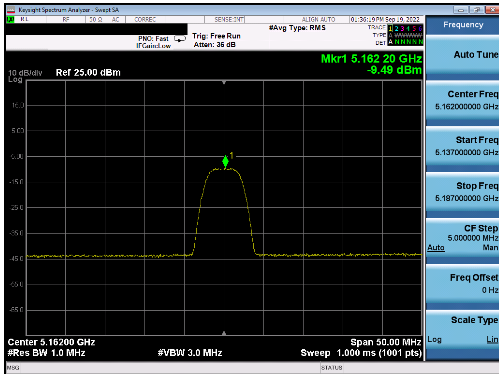
Plot 7-34. PSD Antenna 5b (HDR8, iPA, 5162MHz)
