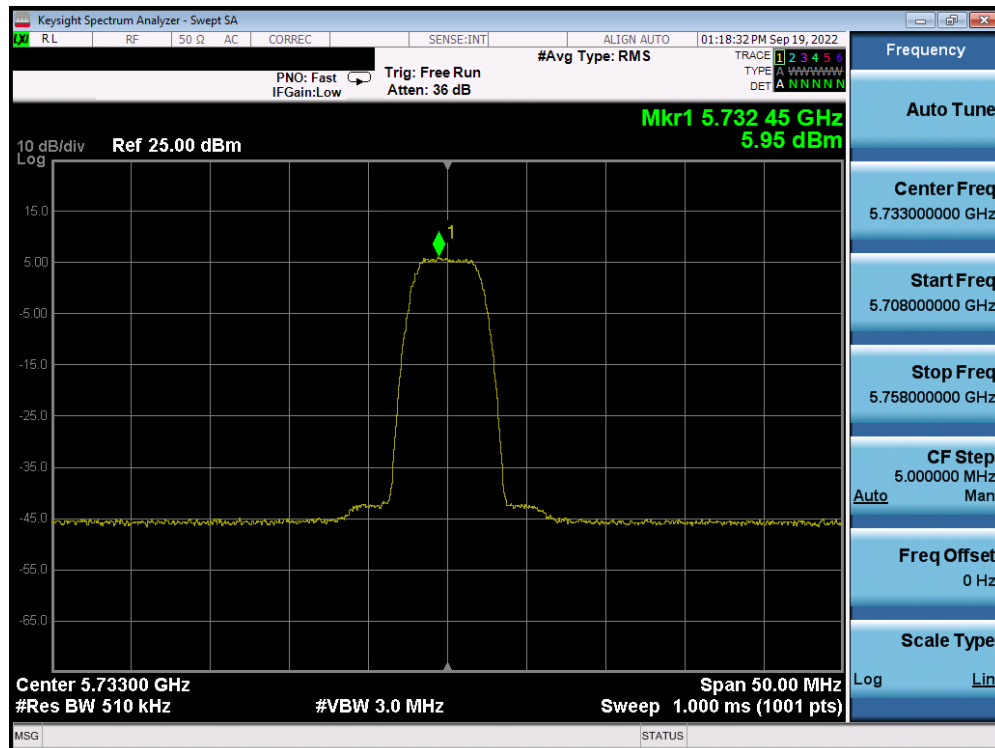
Plot 7-40. PSD Antenna 5b (HDR8, ePA, 5733MHz)
