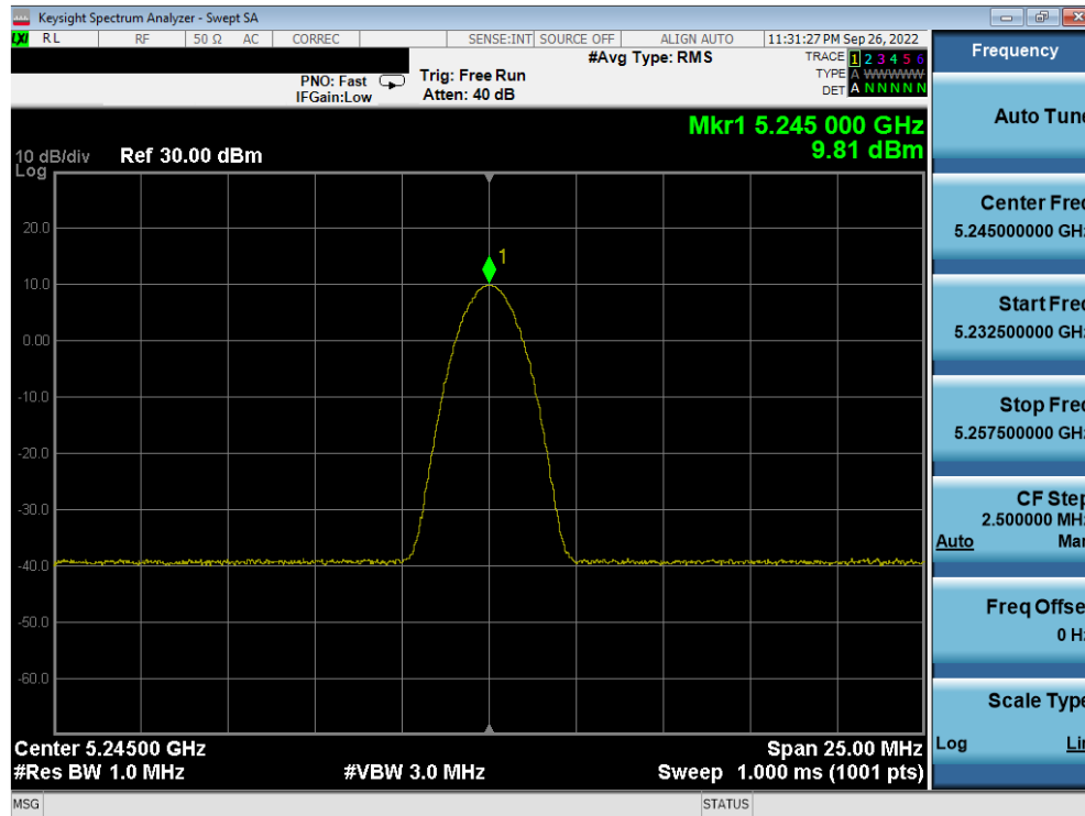
Plot 7-15. PSD Antenna 5b (BDR GFSK, ePA – 5245MHz)
