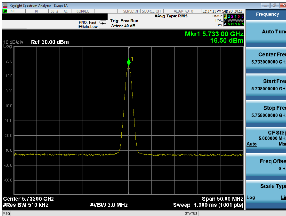
Plot 7-49. PSD TxBF Antenna 5b (BDR GFSK, ePA – 5733MHz)
