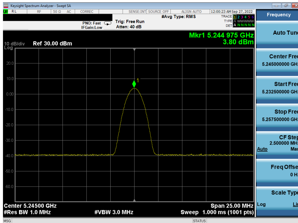
Plot 7-30. PSD Antenna 4a (BDR GFSK, iPA – 5245MHz)
