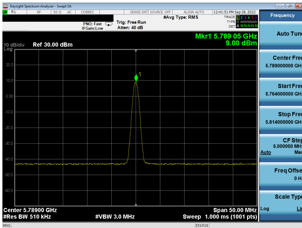
Plot 7-52. PSD TxBF Antenna 4a (BDR GFSK, ePA – 5789MHz)
