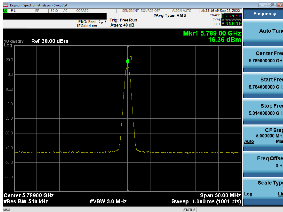
Plot 7-20. PSD Antenna 5b (BDR GFSK, ePA – 5789MHz)
