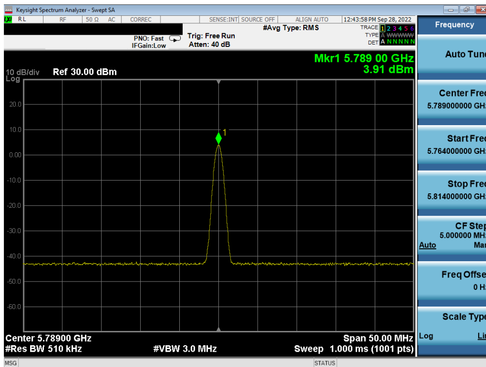
Plot 7-58. PSD TxBF Antenna 4a (BDR GFSK, iPA – 5789MHz)
