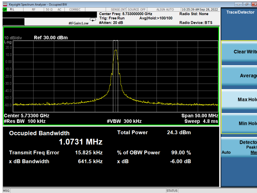
Plot 7-7. 6dB BW & 99% OBW Antenna 5b (BDR GFSK, ePA – 5733MHz)
