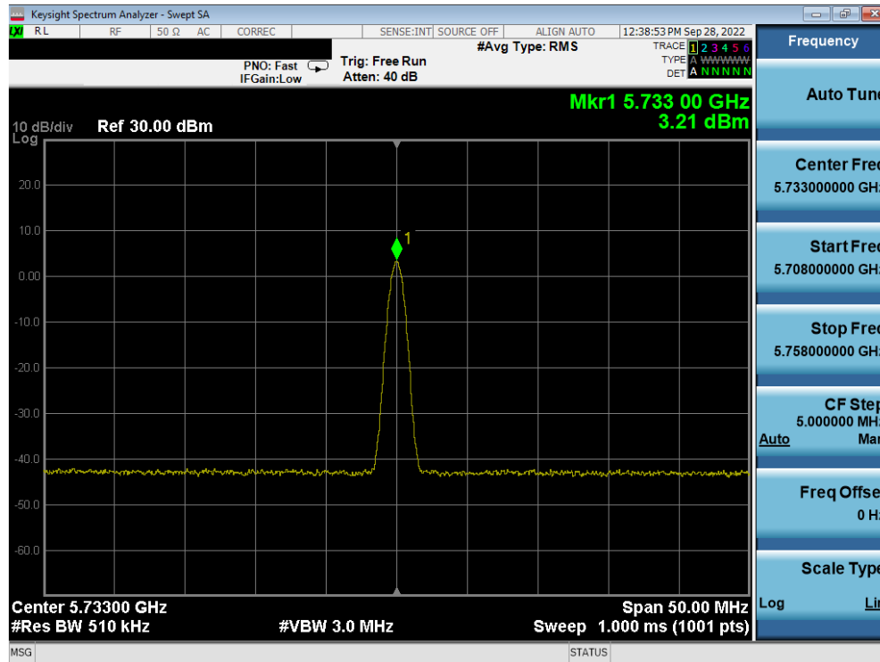
Plot 7-55. PSD TxBF Antenna 5b (BDR GFSK, iPA - 5733MHz)
