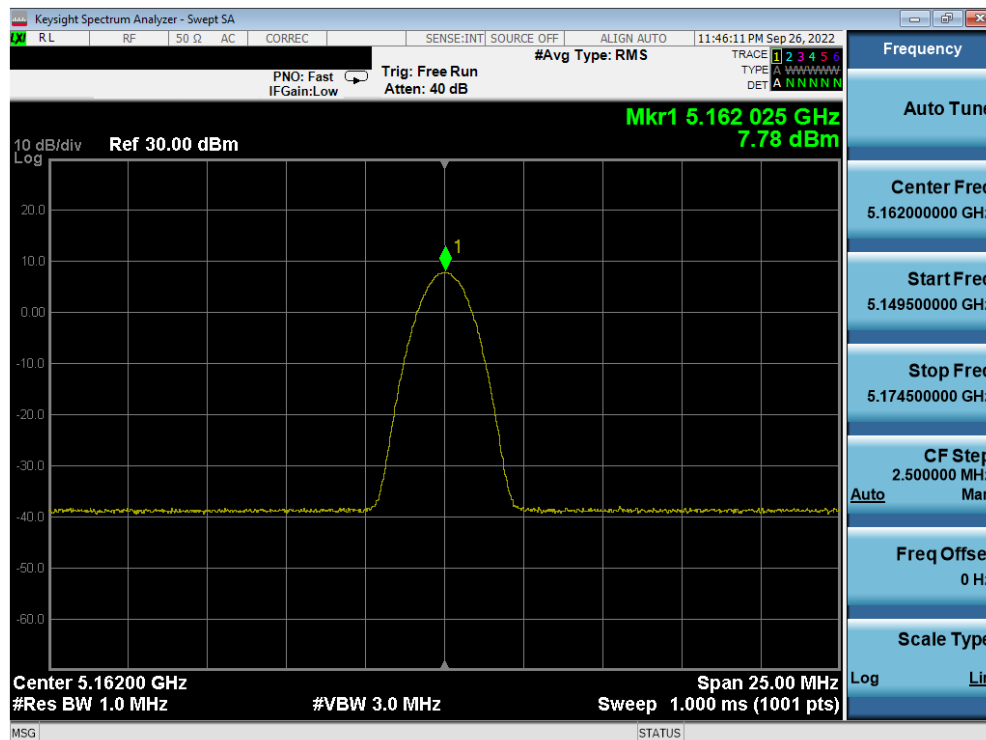
Plot 7-38. PSD TxBF Antenna 4a (BDR GFSK, ePA - 5162MHz)
