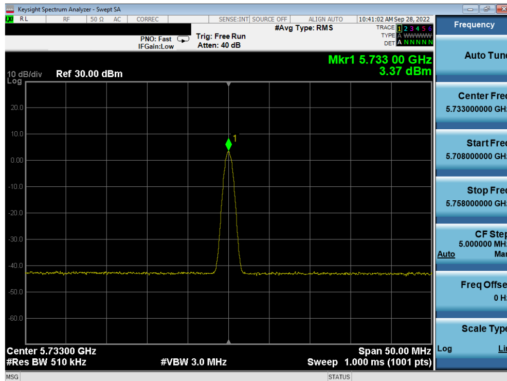
Plot 7-22. PSD Antenna 5b (BDR GFSK, iPA – 5733MHz)
