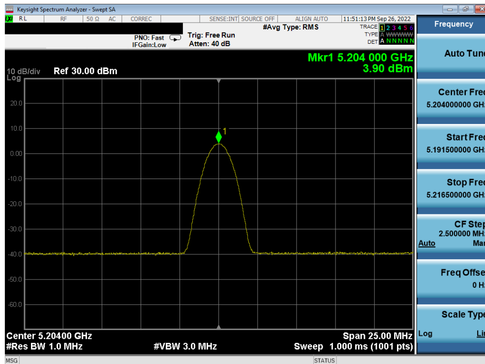
Plot 7-46. PSD TxBF Antenna 4a (BDR GFSK, iPA - 5204MHz)
