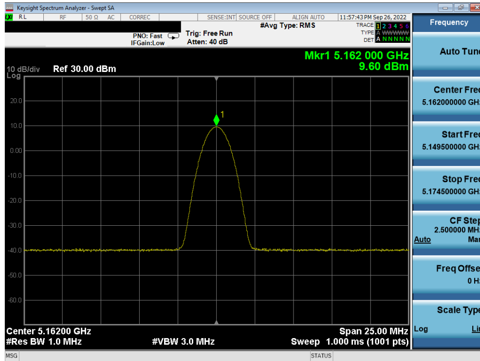
Plot 7-25. PSD Antenna 4a (BDR GFSK, ePA – 5162MHz)
