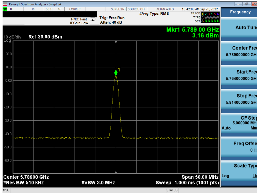
Plot 7-23. PSD Antenna 5b (BDR GFSK, iPA – 5789MHz)
