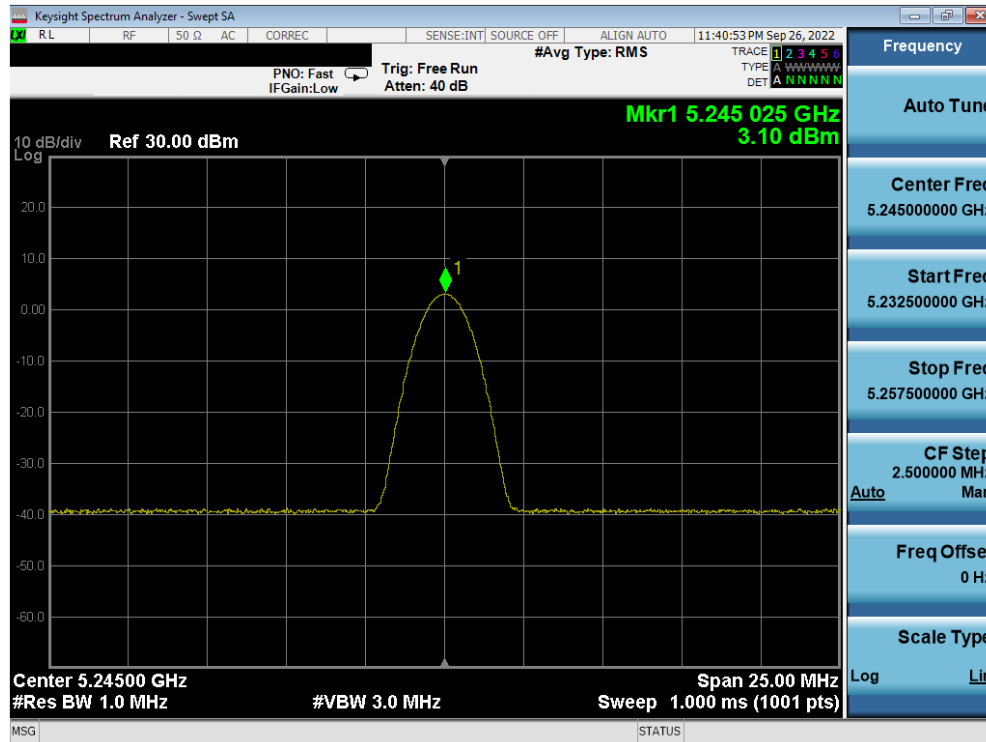
Plot 7-47. PSD TxBF Antenna 5b (BDR GFSK, iPA – 5245MHz)
