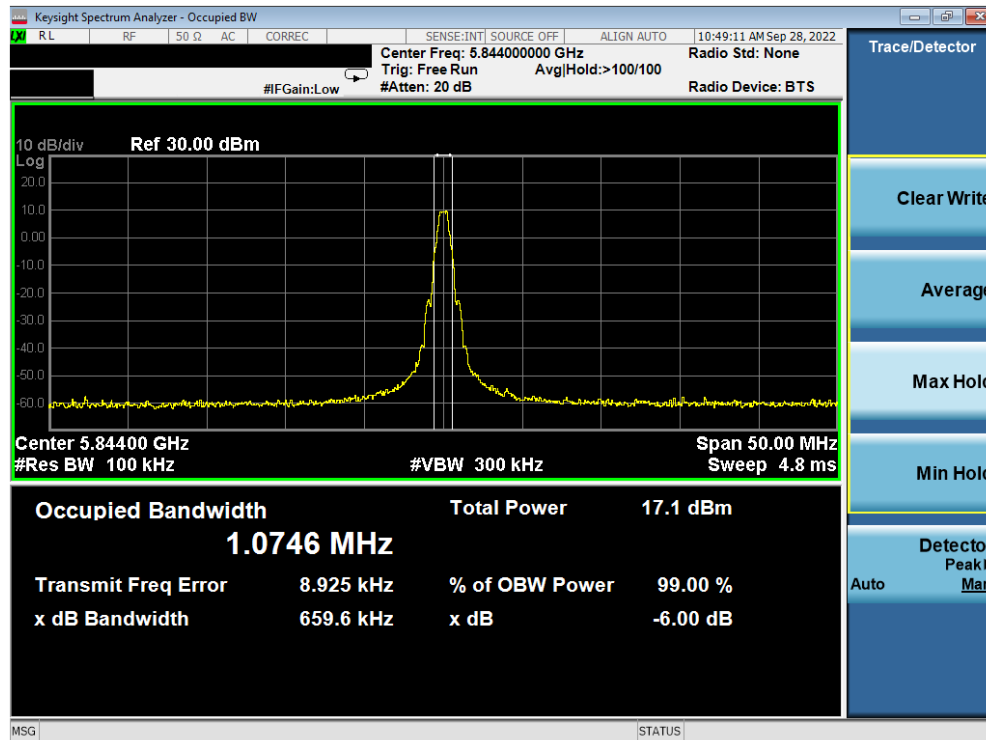
Plot 7-12. 6dB BW & 99% OBW Antenna 4a (BDR GFSK, ePA – 5844MHz)
