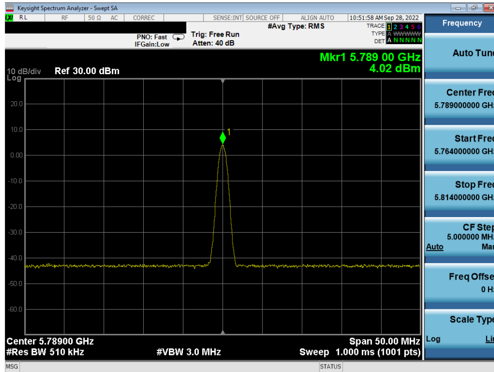
Plot 7-35. PSD Antenna 4a (BDR GFSK, iPA – 5789MHz)
