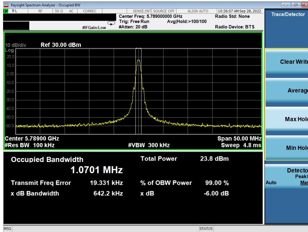
Plot 7-8. 6dB BW & 99% OBW Antenna 5b (BDR GFSK, ePA – 5789MHz)
