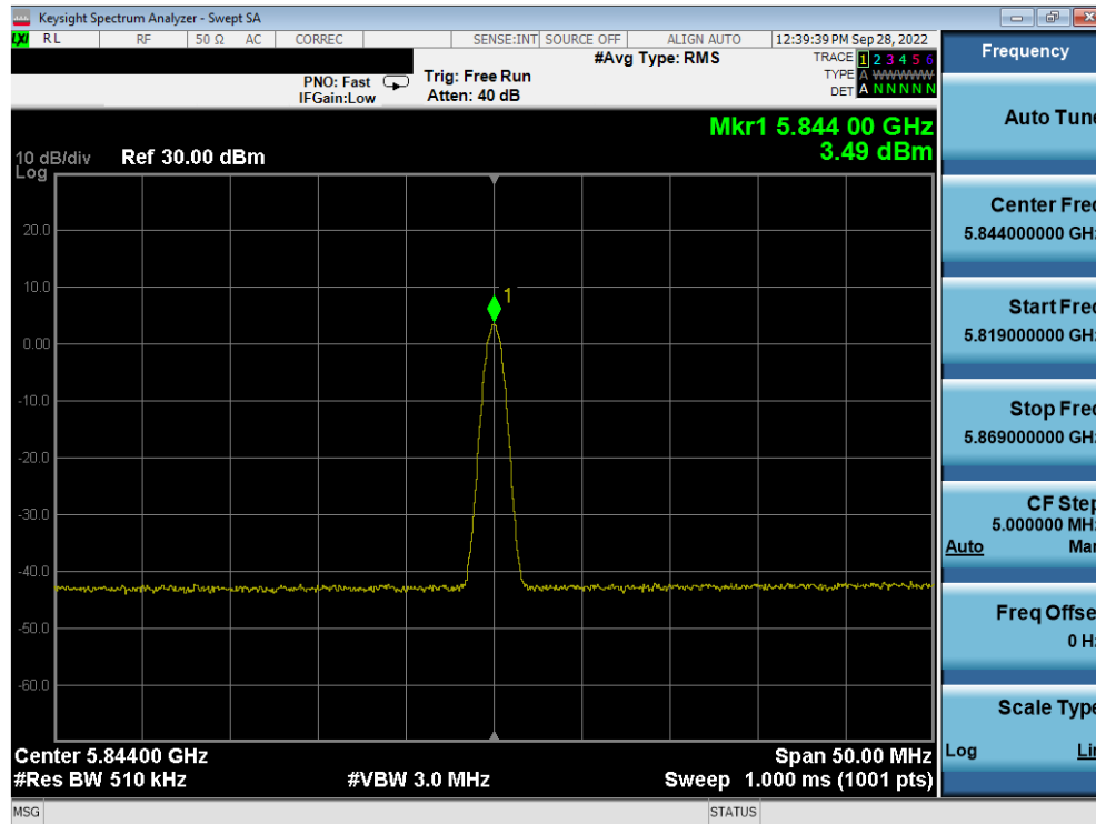
Plot 7-59. PSD TxBF Antenna 5b (BDR GFSK, iPA – 5844MHz)
