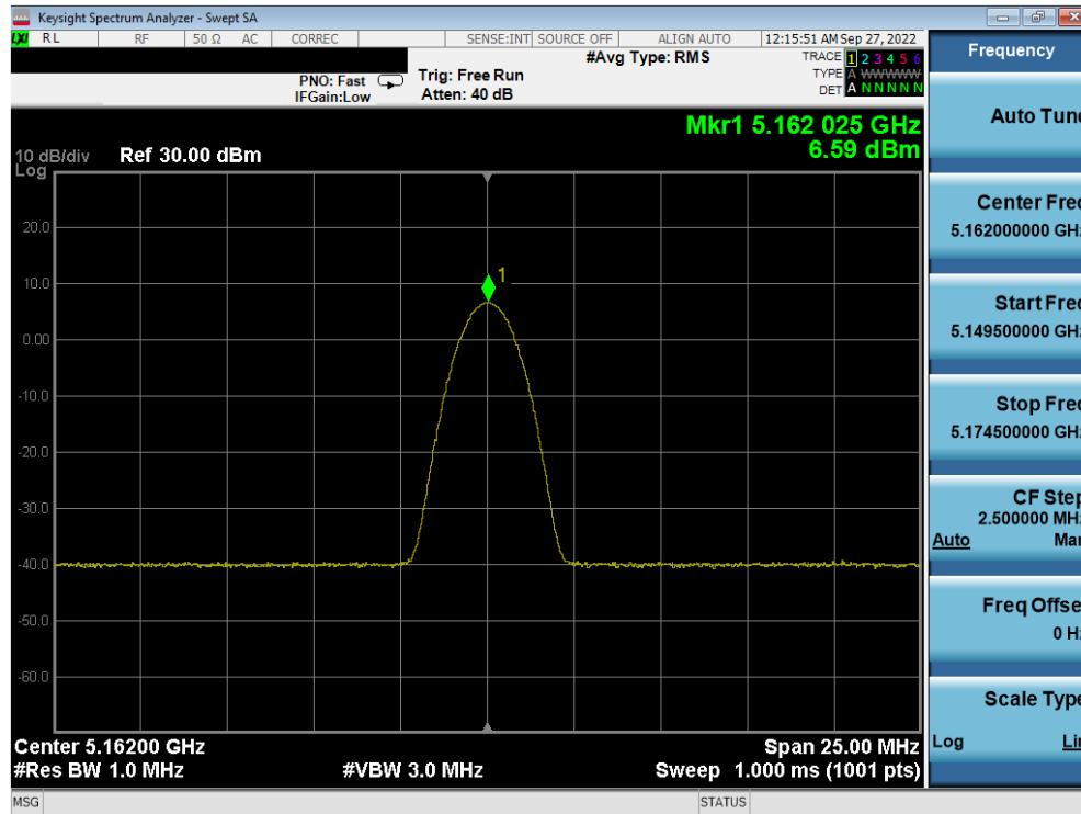
Plot 7-37. PSD TxBF Antenna 5b (BDR GFSK, ePA - 5162MHz)
