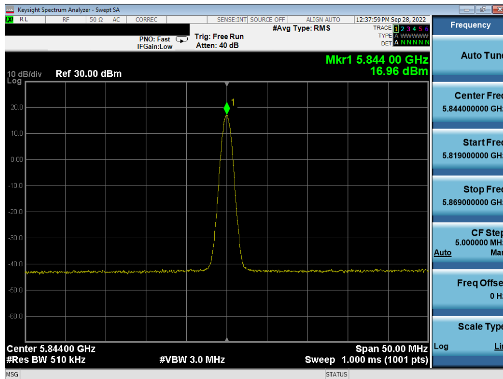
Plot 7-53. PSD TxBF Antenna 5b (BDR GFSK, ePA – 5844MHz)
