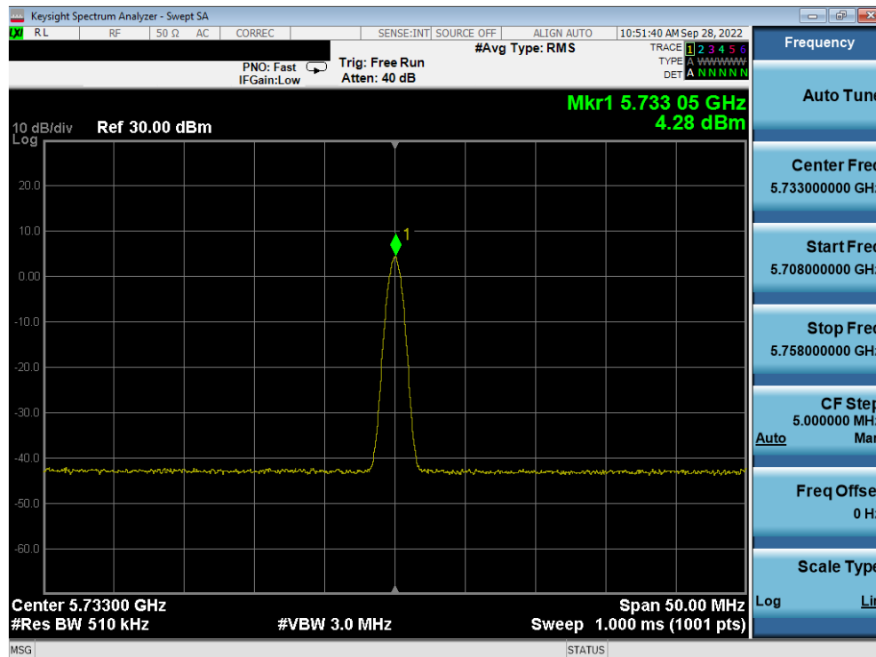
Plot 7-34. PSD Antenna 4a (BDR GFSK, iPA – 5733MHz)
