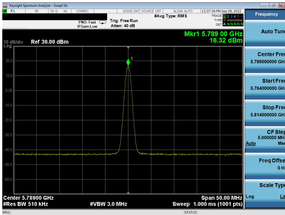
Plot 7-51. PSD TxBF Antenna 5b (BDR GFSK, ePA – 5789MHz)
