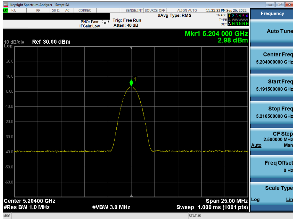
Plot 7-17. PSD Antenna 5b (BDR GFSK, iPA, – 5204MHz)
