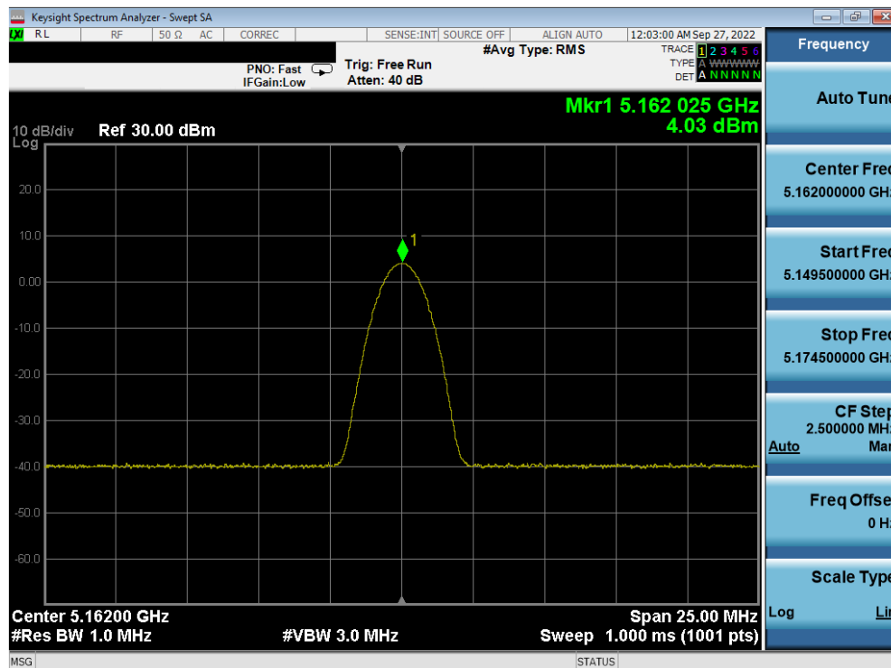
Plot 7-28. PSD Antenna 4a (BDR GFSK, iPA – 5162MHz)
