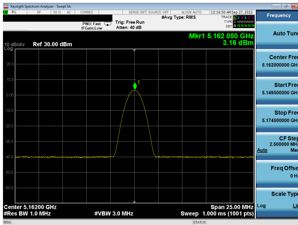
Plot 7-43. PSD TxBF Antenna 5b (BDR GFSK, iPA – 5162MHz)
