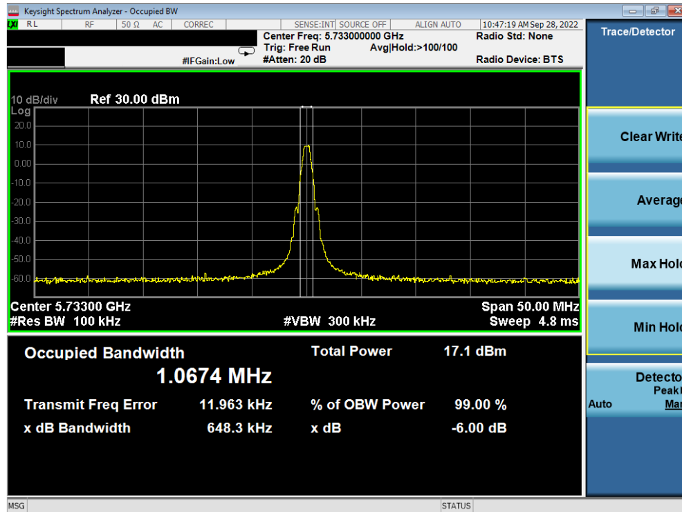
Plot 7-10. 6dB BW & 99% OBW Antenna 4a (BDR GFSK, ePA – 5733MHz)
