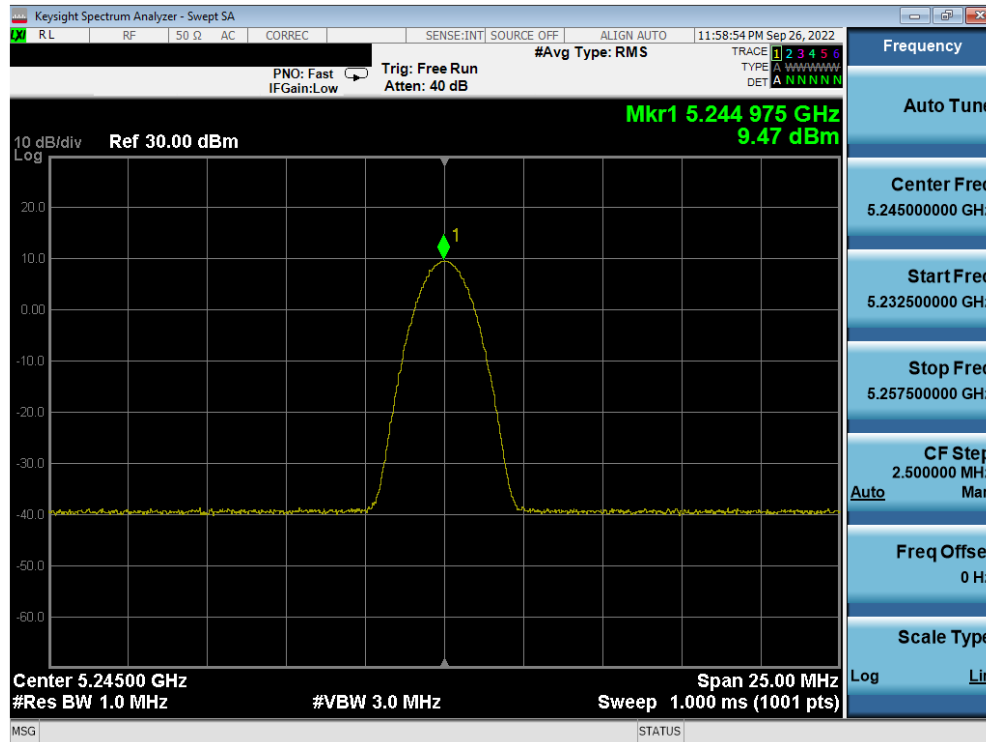
Plot 7-27. PSD Antenna 4a (BDR GFSK, ePA – 5245MHz)
