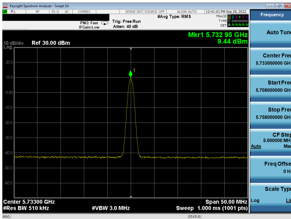
Plot 7-50. PSD TxBF Antenna 4a (BDR GFSK, ePA – 5733MHz)
