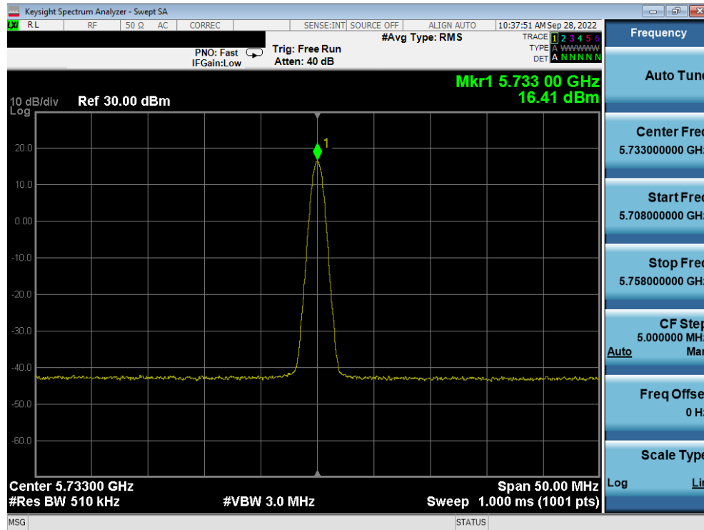
Plot 7-19. PSD Antenna 5b (BDR GFSK, ePA – 5733MHz)
