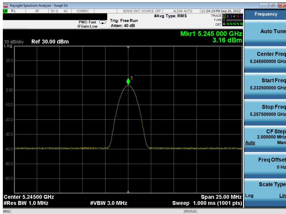
Plot 7-18. PSD Antenna 5b (BDR GFSK, iPA – 5245MHz)
