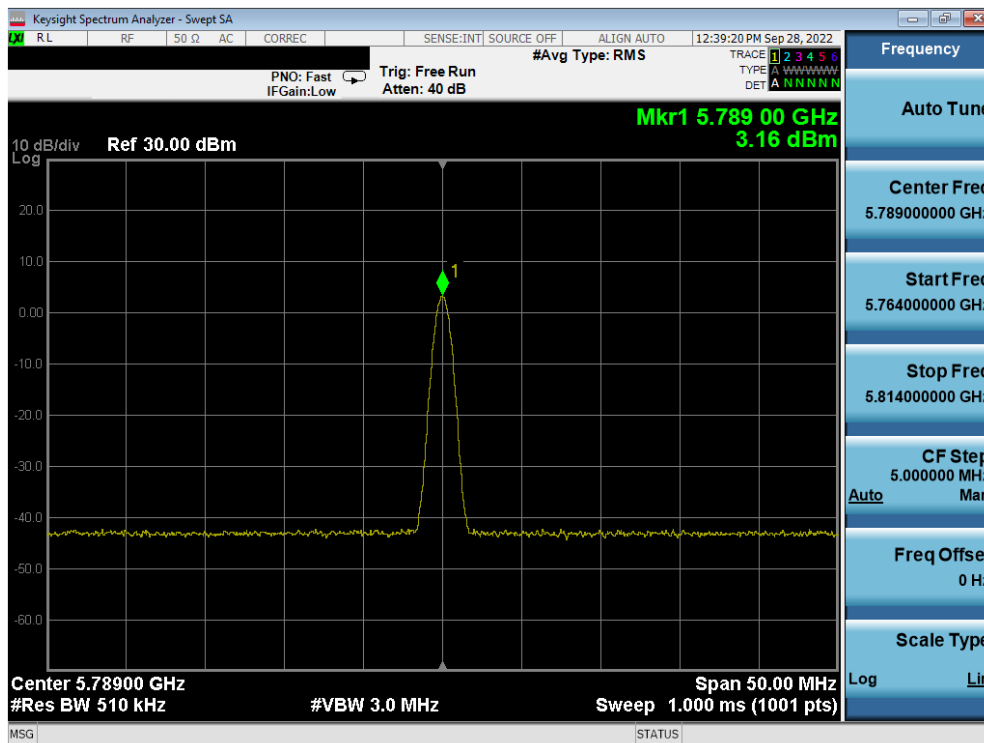
Plot 7-57. PSD TxBF Antenna 5b (BDR GFSK, iPA – 5789MHz)
