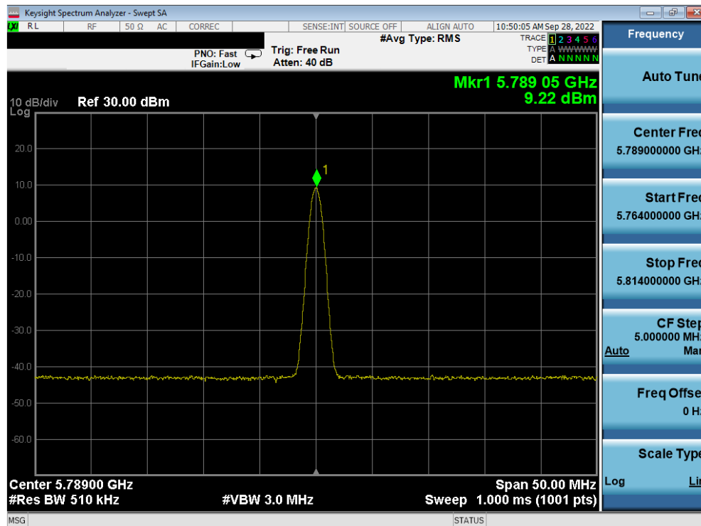
Plot 7-32. PSD Antenna 4a (BDR GFSK, ePA – 5789MHz)
