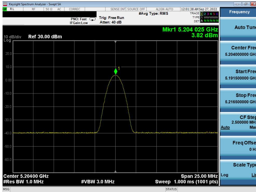
Plot 7-29. PSD Antenna 4a (BDR GFSK, iPA – 5204MHz)
