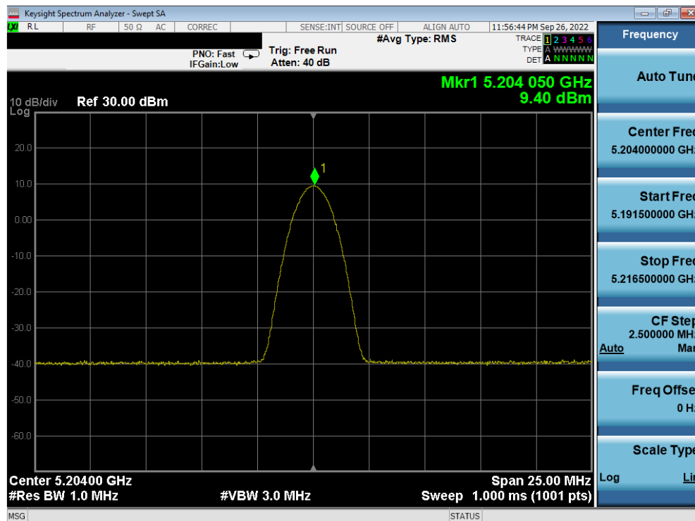
Plot 7-26. PSD Antenna 4a (BDR GFSK, ePA – 5204MHz)
