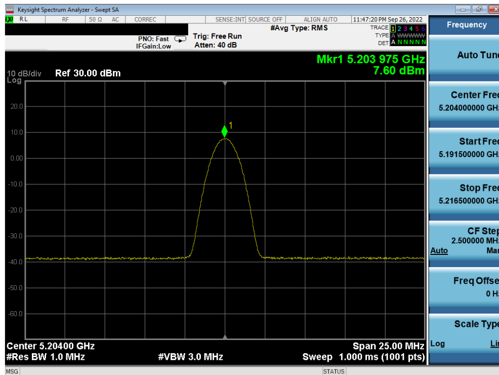
Plot 7-40. PSD TxBF Antenna 4a (BDR GFSK, ePA – 5204MHz)
