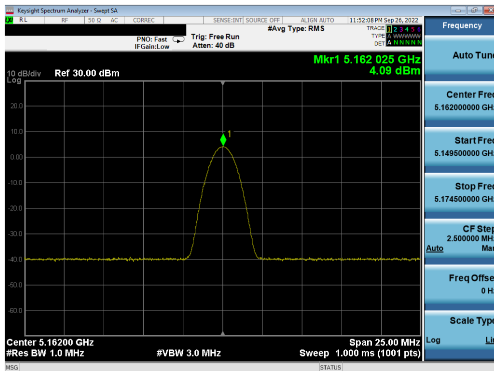
Plot 7-44. PSD TxBF Antenna 4a (BDR GFSK, iPA – 5162MHz)
