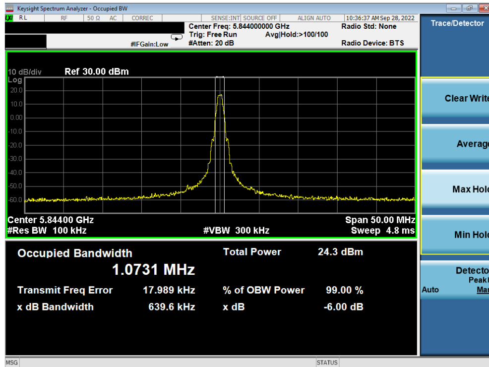
Plot 7-9. 6dB BW & 99% OBW Antenna 5b (BDR GFSK, ePA – 5844MHz)
