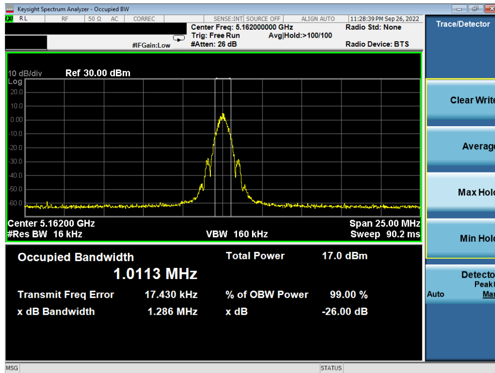
Plot 7-1. 26dB BW & 99% OBW Antenna 5b (BDR GFSK, ePA – 5162MHz)
