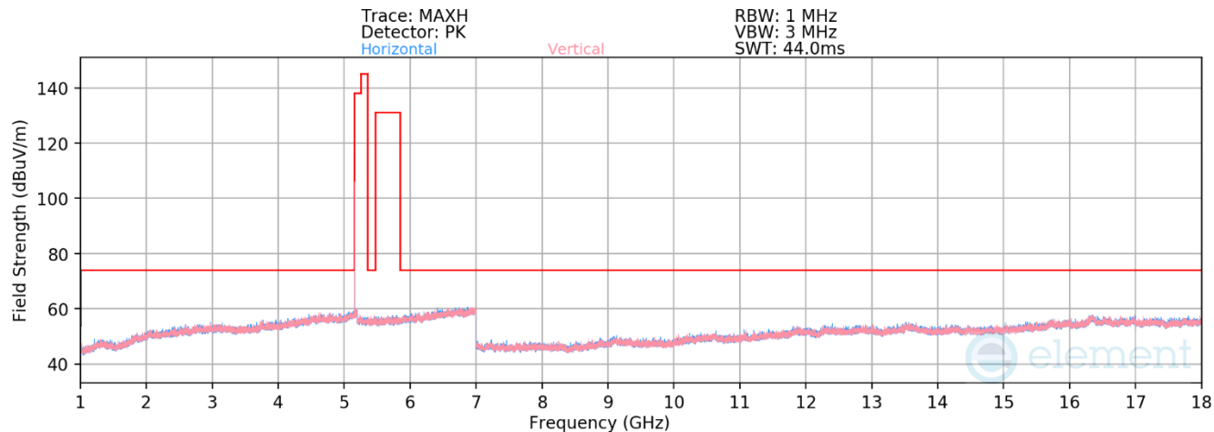
Plot 7-61. RSE 1-18GHz Antenna 5b (BDR GFSK ePA - 5162MHz)
