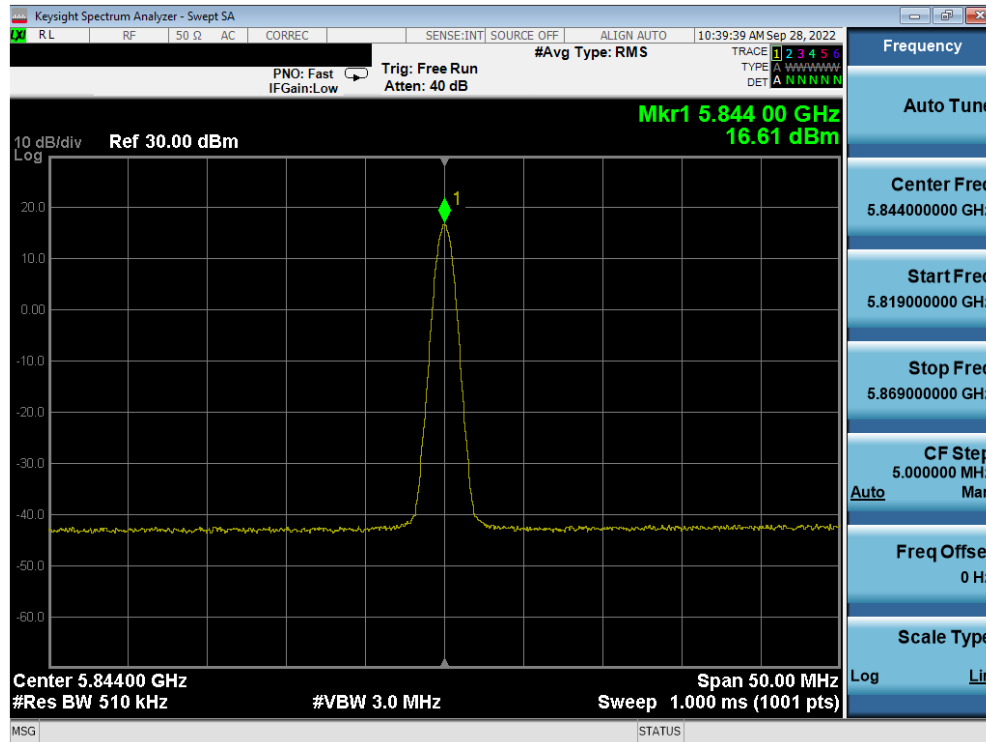
Plot 7-21. PSD Antenna 5b (BDR GFSK, ePA – 5844MHz)
