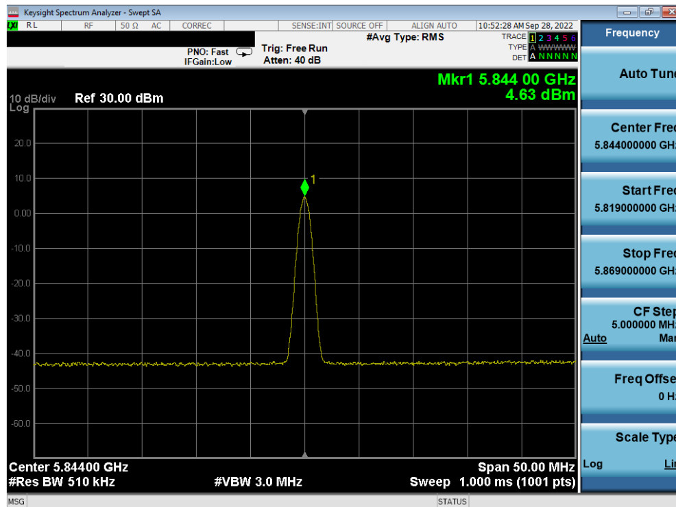
Plot 7-36. PSD Antenna 4a (BDR GFSK, iPA – 5844MHz)
