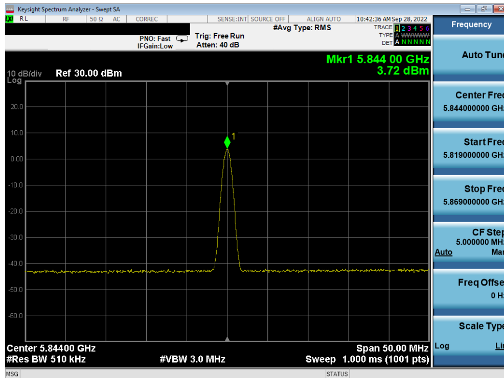
Plot 7-24. PSD Antenna 5b (BDR GFSK, iPA – 5844MHz)
