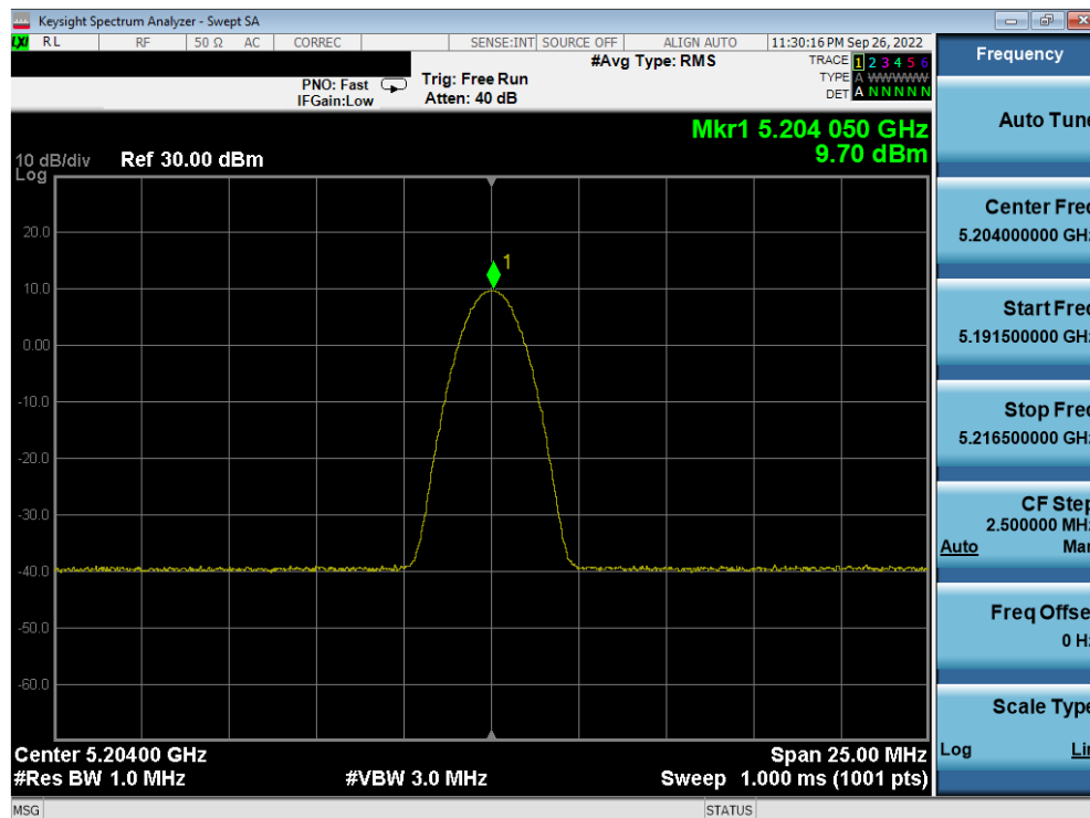
Plot 7-14. PSD Antenna 5b (BDR GFSK, ePA - 5204MHz)
