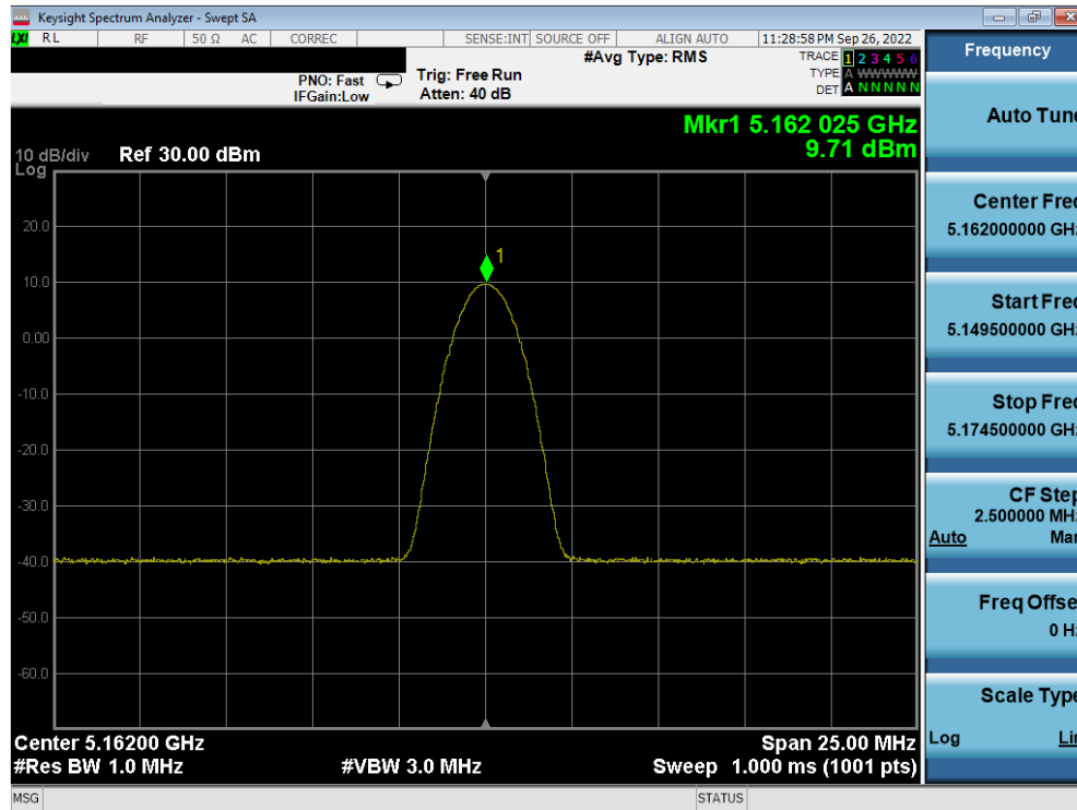
Plot 7-13. PSD Antenna 5b (BDR GFSK, ePA, - 5162MHz)
