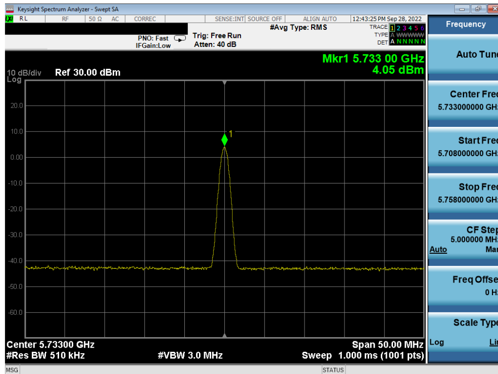
Plot 7-56. PSD TxBF Antenna 4a (BDR GFSK, iPA - 5733MHz)
