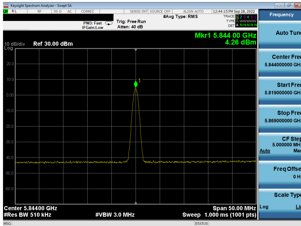
Plot 7-60. PSD TxBF Antenna 4a (BDR GFSK, iPA – 5844MHz)
