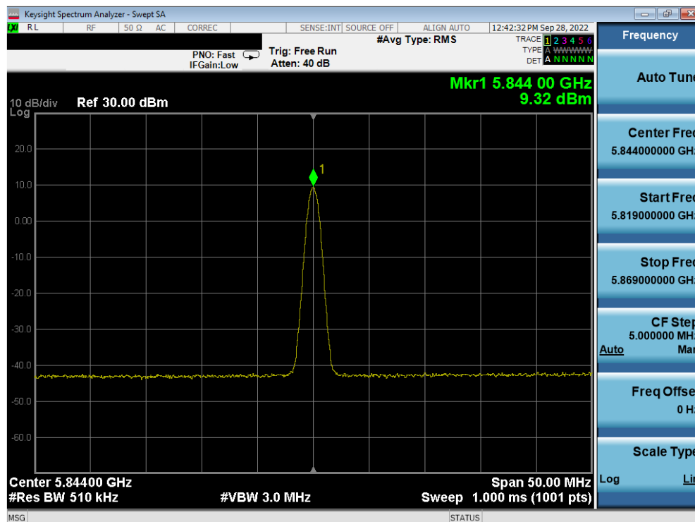
Plot 7-54. PSD TxBF Antenna 4a (BDR GFSK, ePA – 5844MHz)
