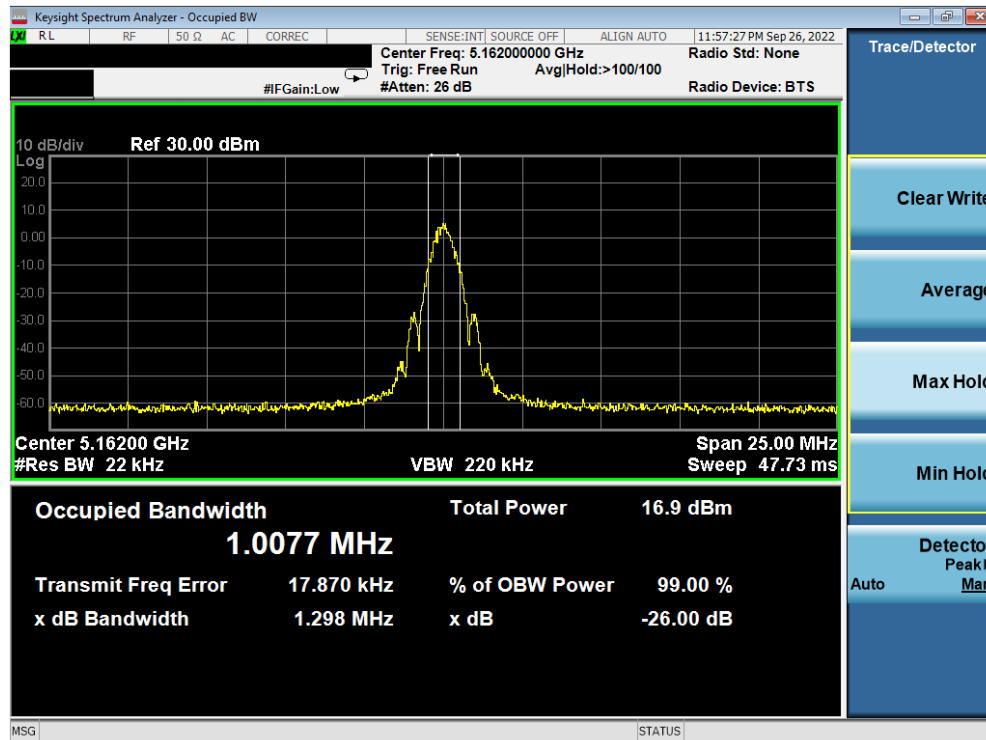
Plot 7-4. 26dB BW & 99% OBW Antenna 4a (BDR GFSK – 5162MHz)
