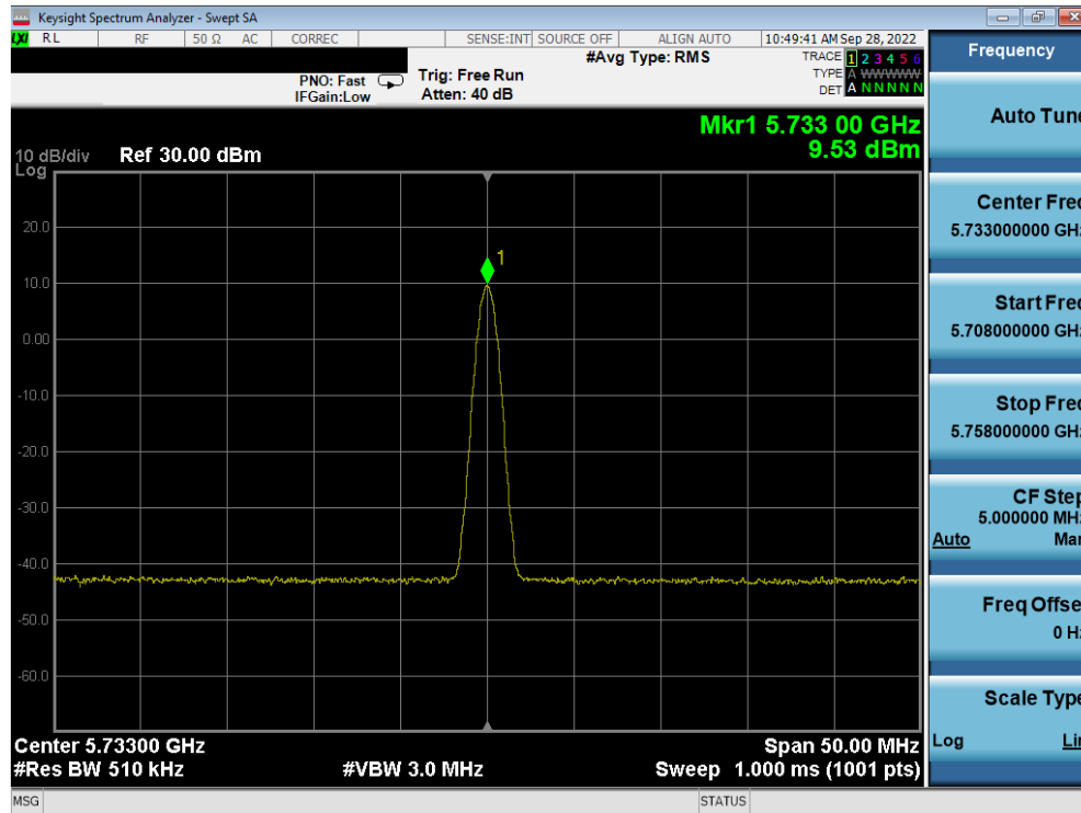
Plot 7-31. PSD Antenna 4a (BDR GFSK, ePA – 5733MHz)
