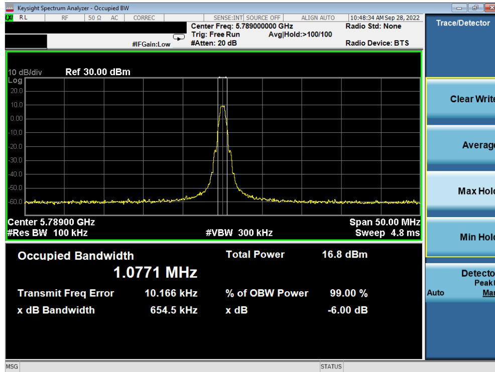
Plot 7-11. 6dB BW & 99% OBW Antenna 4a (BDR GFSK, ePA – 5789MHz)
