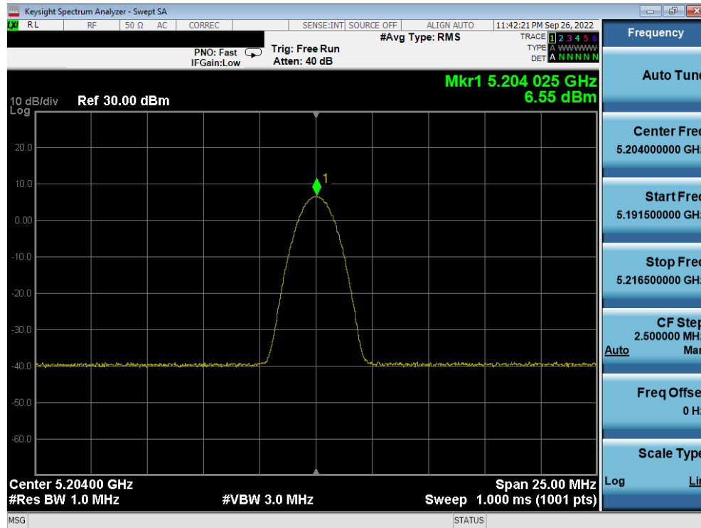
Plot 7-39. PSD TxBF Antenna 5b (BDR GFSK, ePA – 5204MHz)
