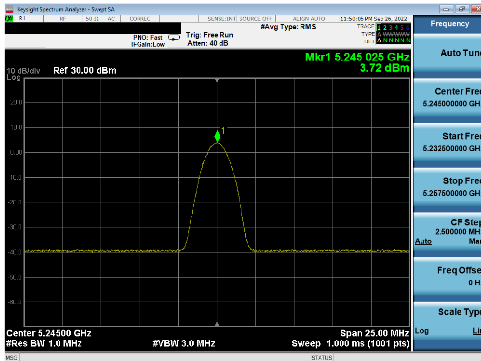
Plot 7-48. PSD TxBF Antenna 4a (BDR GFSK, iPA – 5245MHz)
