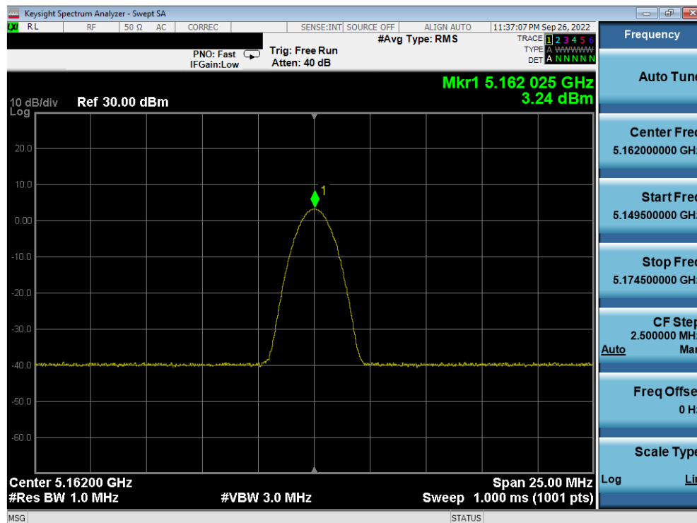
Plot 7-16. PSD Antenna 5b (BDR GFSK, iPA – 5162MHz)
