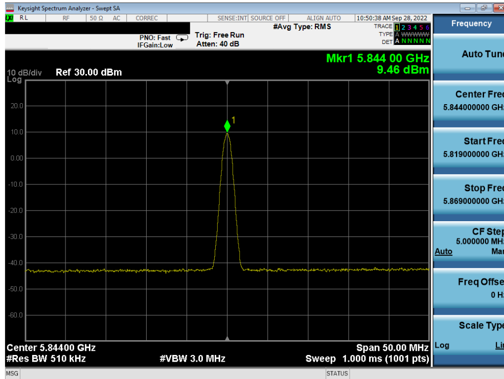
Plot 7-33. PSD Antenna 4a (BDR GFSK, ePA – 5844MHz)
