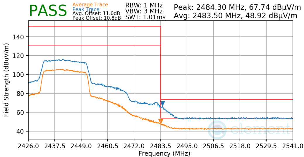
Plot 7-612. Radiated Restricted Upper Band Edge Measurement Antenna 2a
