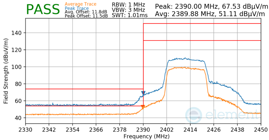
Plot 7-591. Radiated Restricted Lower Band Edge Measurement Antenna 2a
