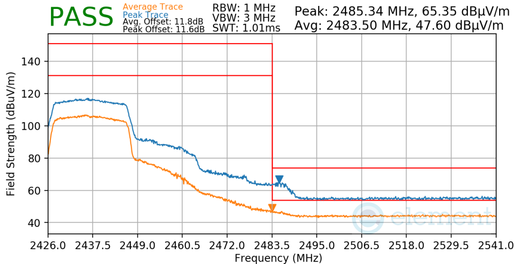
Plot 7-609. Radiated Restricted Upper Band Edge Measurement Antenna 2a
