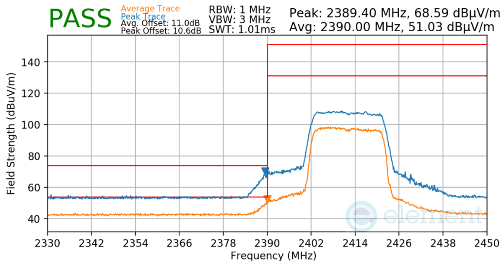
Plot 7-592. Radiated Restricted Lower Band Edge Measurement Antenna 2a
