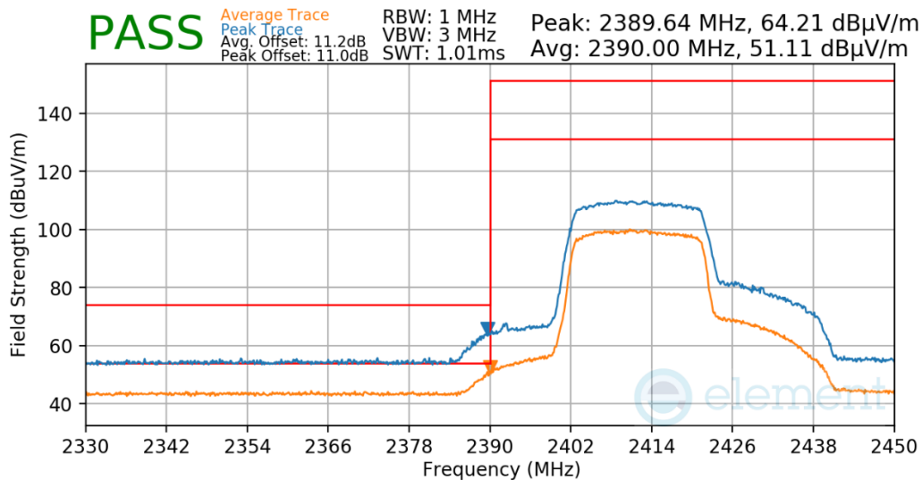
Plot 7-590. Radiated Restricted Lower Band Edge Measurement Antenna 2a
