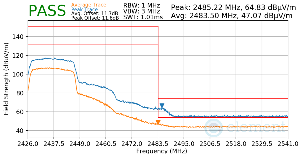
Plot 7-608. Radiated Restricted Upper Band Edge Measurement Antenna 2a
