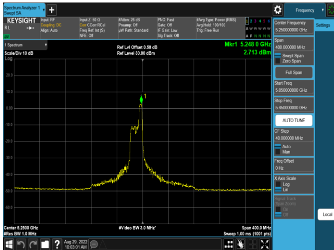
Plot 7-393. ISED PSD Antenna WF5b (20MHz BW 11ax Index 52 – RU52 – Ch.50(L))
