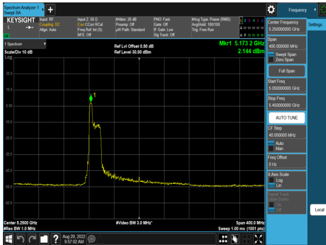
Plot 7-392. ISED PSD Antenna WF4a (20MHz BW 11ax Index 37 – RU52 – Ch.50(L))
