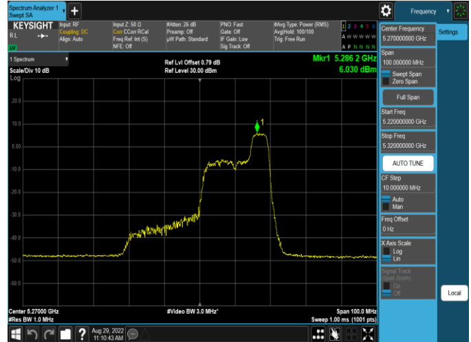
Plot 7-300. PSD CDD Antenna WF4a (40MHz BW 11ax Index 44 – RU52 – Ch.54)
