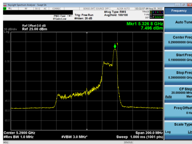
Plot 7-139. PSD Antenna WF5b (80MHz BW 11ax Index 52 - RU52 - Ch.58)
