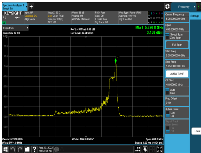
Plot 7-127. PSD Antenna WF5b (20MHz BW 11ax Index 52– RU52 – Ch.50(U))
