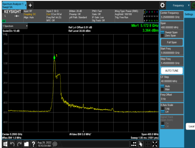
Plot 7-125. PSD Antenna WF5b (20MHz BW 11ax Index 37 – RU52 – Ch.50(L))
