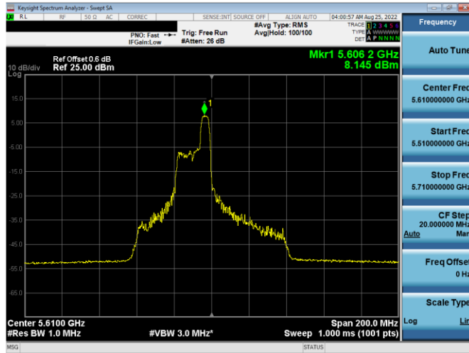
Plot 7-150. PSD Antenna WF5b (80MHz BW 11ax Index 44 - RU52 - Ch.122)
