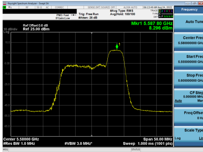
Plot 7-143. PSD Antenna WF5b (20MHz BW 11ax Index 40 – RU52 – Ch.116)
