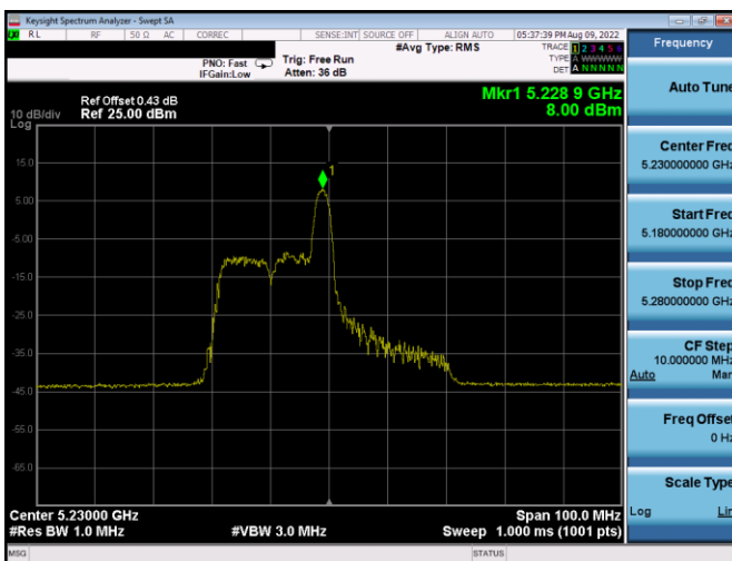
Plot 7-118. PSD Antenna WF5b (40MHz BW 11ax Index 8 - RU26 - Ch.46)
