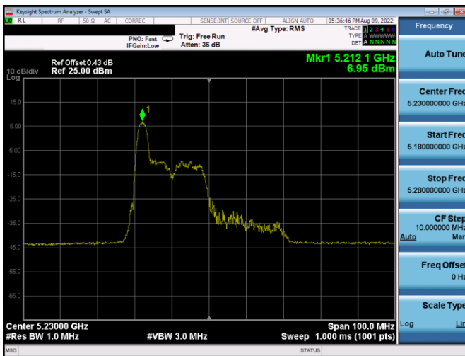
Plot 7-117. PSD Antenna WF5b (40MHz BW 11ax Index 0 - RU26 - Ch.46)
