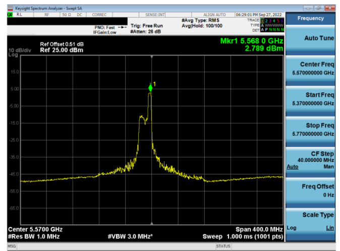
Plot 7-154. PSD Antenna WF5b (80MHz BW 11ax Index 52 - RU52 - Ch.114(L))
