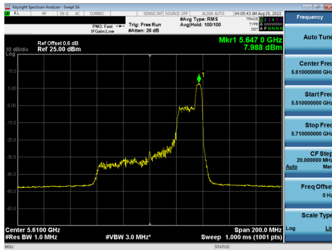
Plot 7-151. PSD Antenna WF5b (80MHz BW 11ax Index 52 - RU52 - Ch.122)
