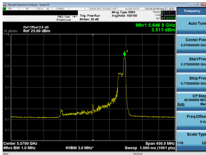
Plot 7-155. PSD Antenna WF5b (80MHz BW 11ax Index 52 – RU52 – Ch.114(U))
