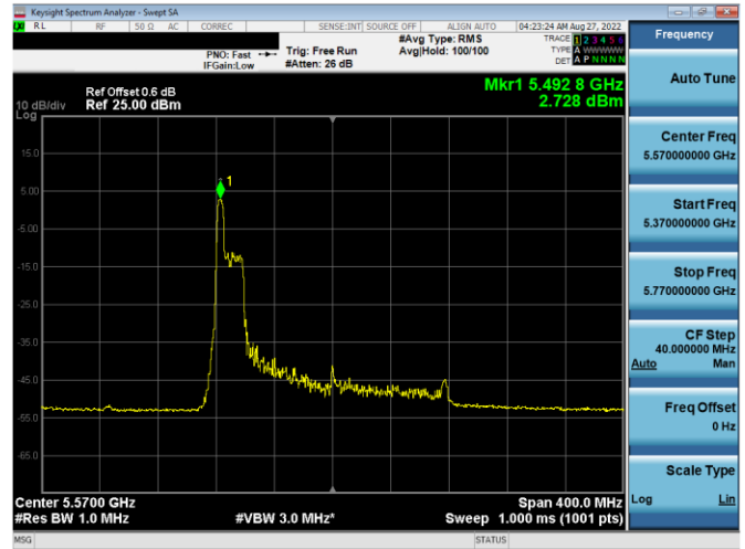
Plot 7-153. PSD Antenna WF5b (80MHz BW 11ax Index 37 - RU52 - Ch.114(L))
