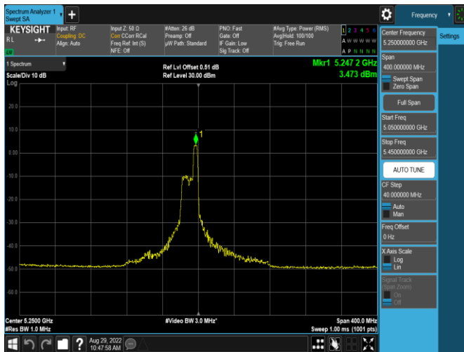
Plot 7-126. PSD Antenna WF5b (20MHz BW 11ax Index 52 – RU52 – Ch.50(L))
