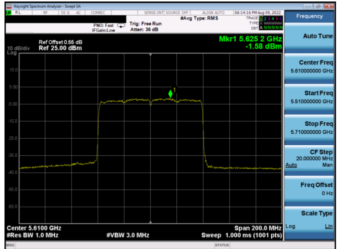
Plot 7-152. PSD Antenna WF5b (80MHz BW 11ax - RU996 - Ch.122)
