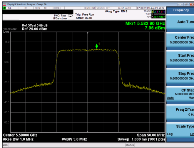
Plot 7-144. PSD Antenna WF5b (20MHz BW 11ax – RU242 – Ch.116)
