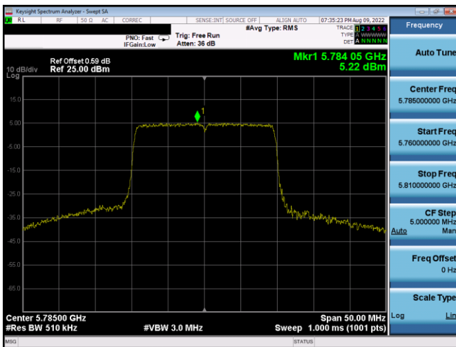
Plot 7-160. PSD Antenna WF5b (20MHz BW 11ax– RU242 – Ch.157)
