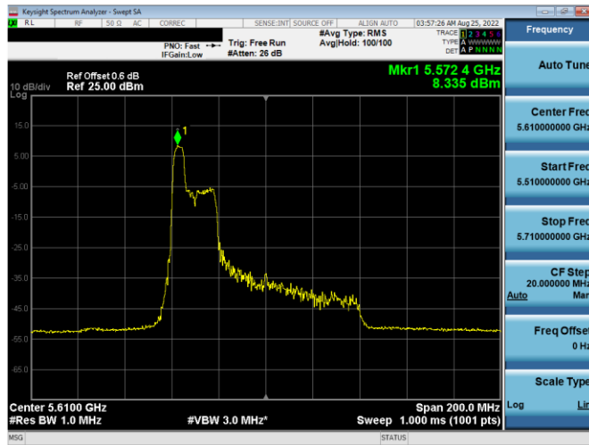
Plot 7-149. PSD Antenna WF5b (80MHz BW 11ax Index 37 - RU52 - Ch.122)
