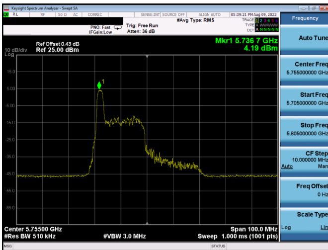
Plot 7-161. PSD Antenna WF5b (40MHz BW 11ax Index 0 – RU26 – Ch.151)
