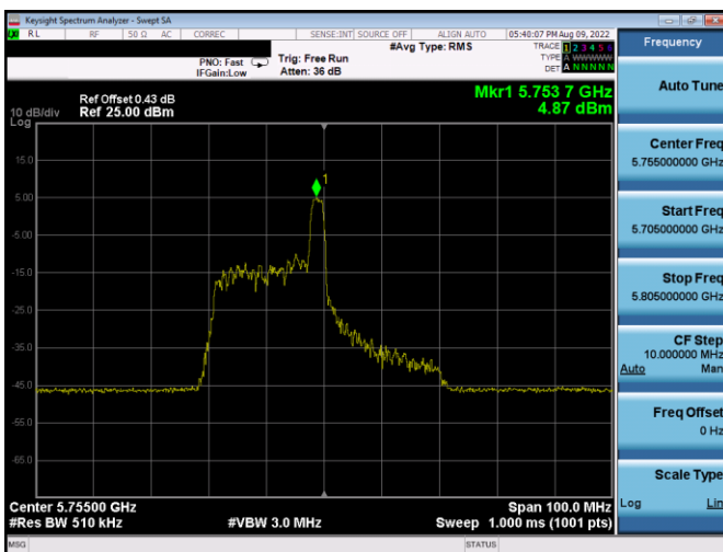
Plot 7-162. PSD Antenna WF5b (40MHz BW 11ax Index 8 – RU26 – Ch.151)
