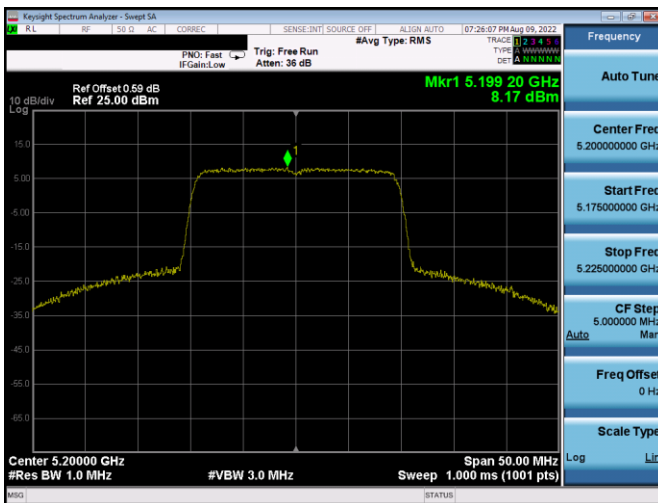
Plot 7-116. PSD Antenna WF5b (20MHz BW 11ax- RU242 - Ch.40)
