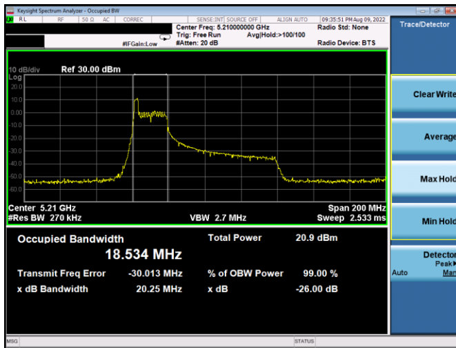
Plot 7-53. 26dB BW & 99% OBW Antenna WF4a (80MHz BW 11ax Index 0 - RU26 - Ch.42)
