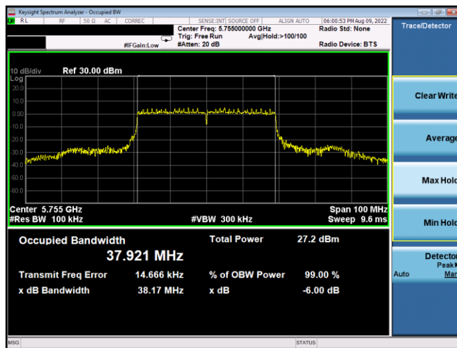
Plot 7-96. 6dB BW & 99% OBW Antenna WF5b (40MHz BW 11ax - RU484 - Ch.151)
