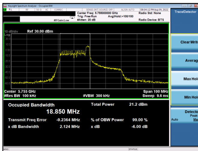
Plot 7-106. 6dB BW & 99% OBW Antenna WF4a (40MHz BW 11ax Index 8 – RU26 – Ch.151)
