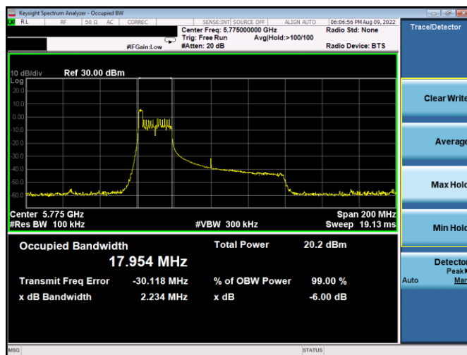
Plot 7-97. 6dB BW & 99% OBW Antenna WF5b (80MHz BW 11ax Index 0 - RU26 - Ch.155)
