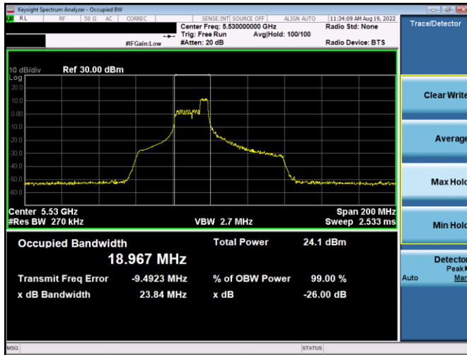
Plot 7-38. 26dB BW & 99% OBW Antenna WF5b (80MHz BW 11ax Index 44 – RU52 – Ch.106)
