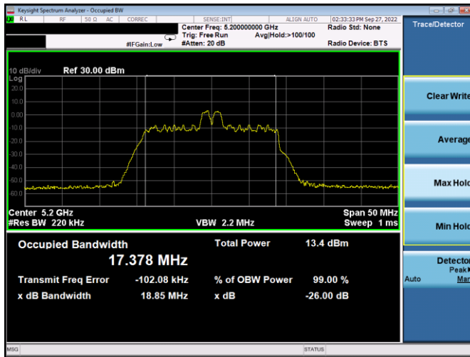
Plot 7-46. 26dB BW & 99% OBW Antenna WF4a (20MHz BW 11ax Index 4 – RU26 – Ch.40)
