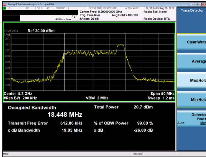
Plot 7-47. 26dB BW & 99% OBW Antenna WF4a (20MHz BW 11ax Index 8– RU26 – Ch.40)
