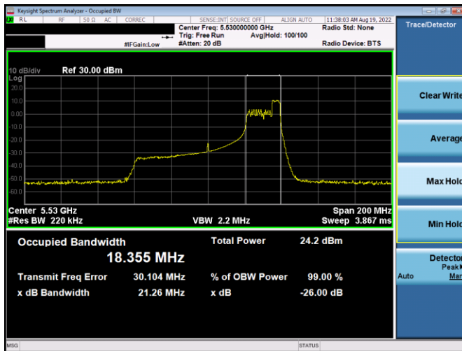
Plot 7-39. 26dB BW & 99% OBW Antenna WF5b (80MHz BW 11ax Index 52 – RU52 – Ch.106)
