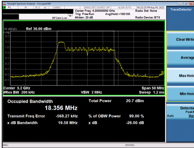
Plot 7-45. 26dB BW & 99% OBW Antenna WF4a (20MHz BW 11ax Index 0 – RU26 – Ch.40)
