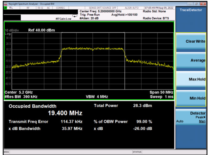
Plot 7-48. 26dB BW & 99% OBW Antenna WF4a (20MHz BW 11ax– RU242 – Ch.40)
