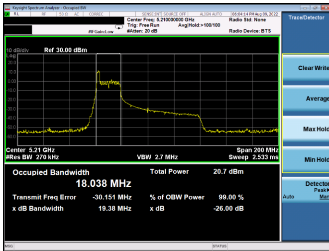
Plot 7-9. 26dB BW & 99% OBW Antenna WF5b (80MHz BW 11ax Index 0 – RU26 – Ch.42)
