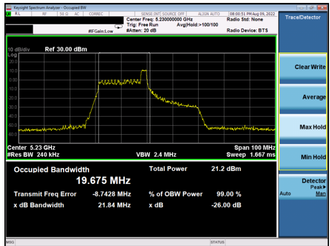
Plot 7-50. 26dB BW & 99% OBW Antenna WF4a (40MHz BW 11ax Index 8 – RU26 – Ch.46)
