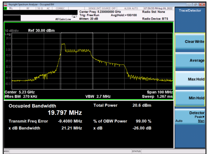
Plot 7-49. 26dB BW & 99% OBW Antenna WF4a (40MHz BW 11ax Index 0 – RU26 – Ch.46)
