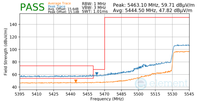
Plot 7-987. Antenna 4a (Pk & Avg, Ch.110, 80.11ax(SU), MCS4)
