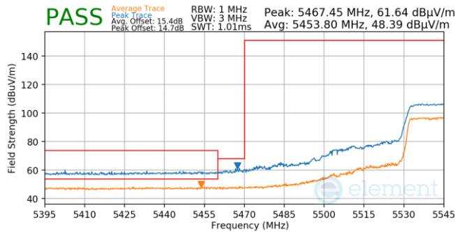
Plot 7-957. Antenna 4a (Pk & Avg, Ch.110, 802.11n, MCS7)
