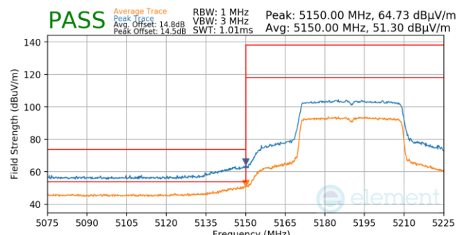
Plot 7-971. Antenna 4a (Pk & Avg, Ch.38, 80.11ax(SU), MCS2)
