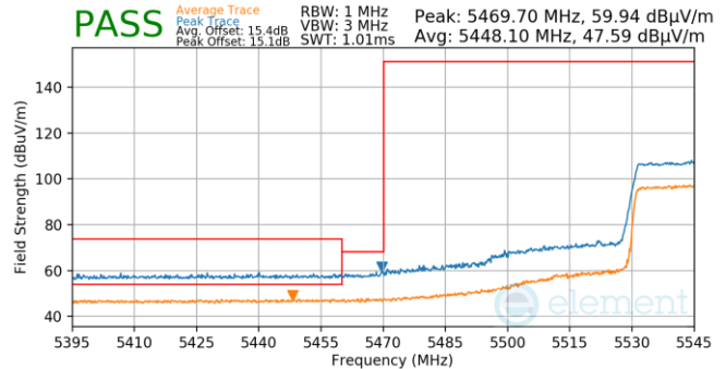
Plot 7-986. Antenna 4a (Pk & Avg, Ch.110, 80.11ax(SU), MCS2)
