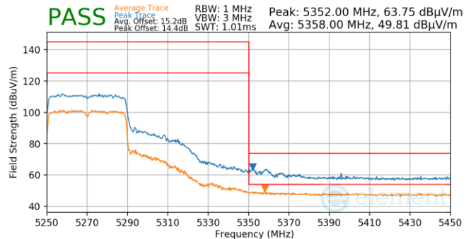
Plot 7-979. Antenna 4a (Pk & Avg, Ch.54, 80.11ax(SU), MCS11)
