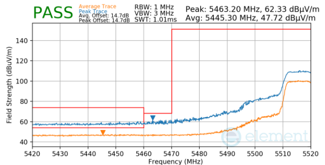
Plot 7-891. Antenna 4a (Pk & Avg, Ch.104, 802.11n, MCS7)
