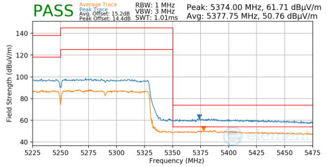
Plot 7-870. Antenna 5b (Pk & Avg, Ch.50, 802.11ax(SU), MCS2)
