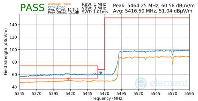
Plot 7-873. (FCC Only) Antenna 5b (Pk & Avg, Ch.114, 802.11ax(SU), MCS2)
