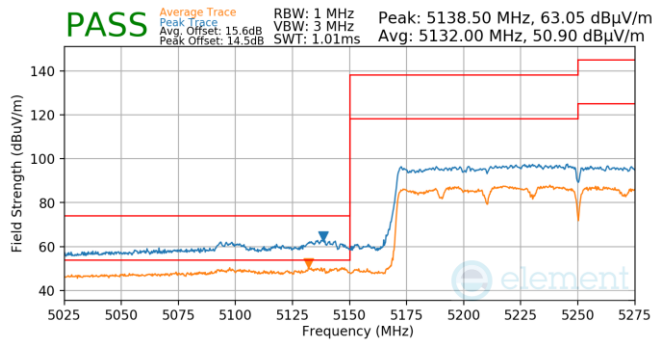
Plot 7-869. Antenna 5b (Pk & Avg, Ch.50, 802.11ax(SU), MCS11)
