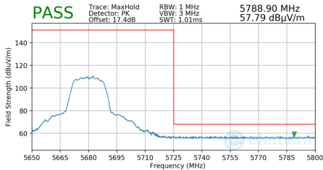
Plot 7-893. Antenna 4a (Pk, Ch.136, 802.11n, MCS2)
