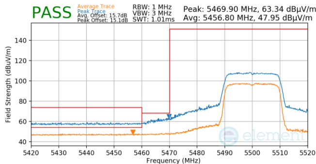
Plot 7-919. Antenna 4a (Pk & Avg, Ch.100, 802.11ax(SU), MCS11)
