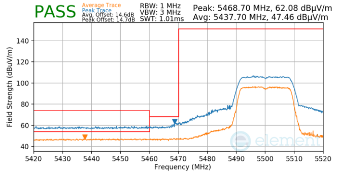
Plot 7-889. Antenna 4a (Pk & Avg, Ch.100, 802.11n, MCS7)
