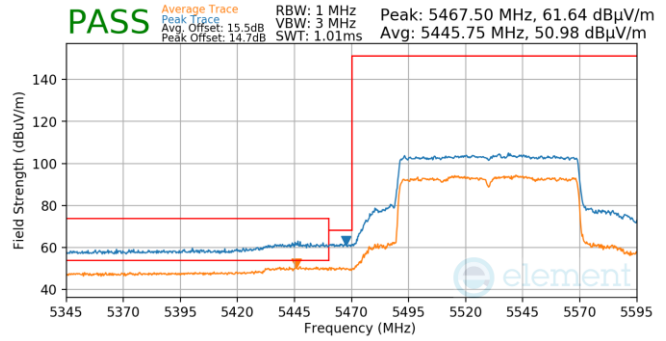
Plot 7-844. Antenna 5b (Pk & Avg, Ch.106, 802.11ax(SU), MCS4)
