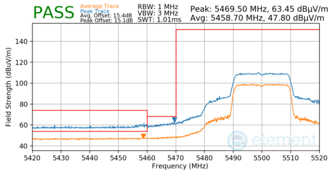
Plot 7-918. Antenna 4a (Pk & Avg, Ch.100, 802.11ax(SU), MCS4)
