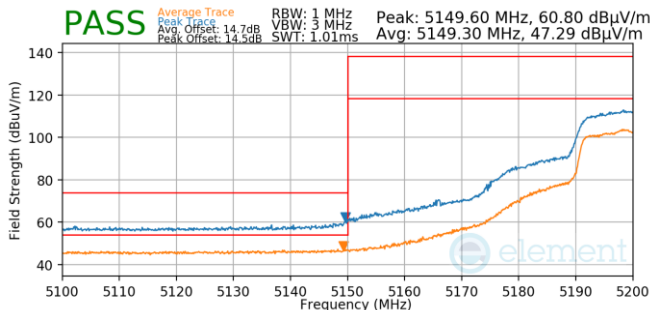
Plot 7-879. Antenna 4a (Pk & Avg, Ch.40, 802.11n, MCS2)
