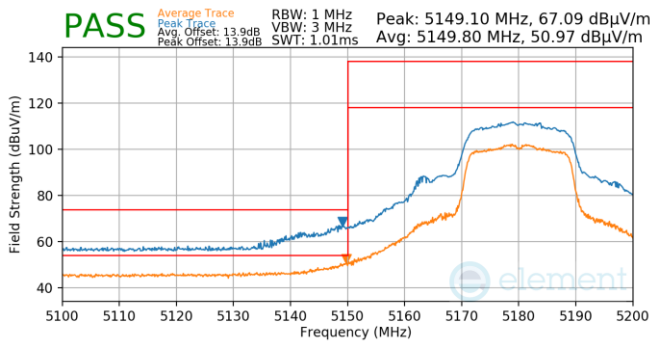
Plot 7-877. Antenna 4a (Pk & Avg, Ch.36, 802.11n, MCS4)
