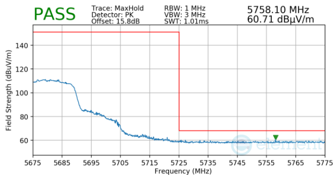
Plot 7-894. Antenna 4a (Pk, Ch.136, 802.11n, MCS4)
