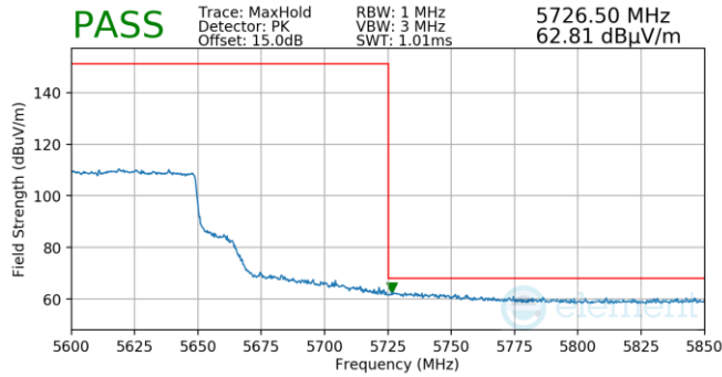
Plot 7-849. (FCC Only) Antenna 5b (Pk, Ch.122, 802.11ax(SU), MCS2)
