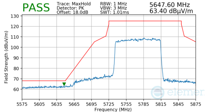
Plot 7-854. Antenna 5b (Pk, Ch.155, 802.11ax(SU), MCS11)
