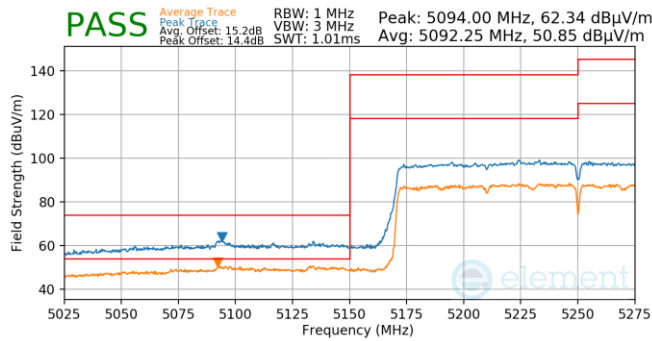
Plot 7-867. Antenna 5b (Pk & Avg, Ch.50, 802.11ax(SU), MCS2)
