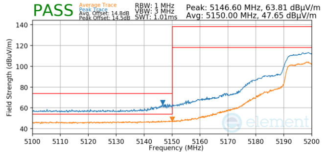
Plot 7-880. Antenna 4a (Pk & Avg, Ch.40, 802.11n, MCS4)
