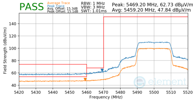
Plot 7-917. Antenna 4a (Pk & Avg, Ch.100, 802.11ax(SU), MCS2)
