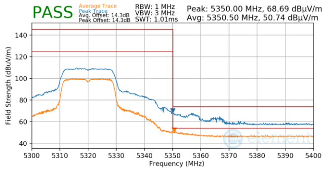
Plot 7-886. Antenna 4a (Pk & Avg, Ch.64, 802.11n, MCS7)
