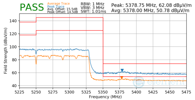
Plot 7-872. Antenna 5b (Pk & Avg, Ch.50, 802.11ax(SU), MCS11)
