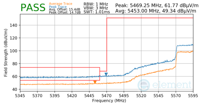
Plot 7-846. (FCC Only) Antenna 5b (Pk & Avg, Ch.122, 802.11ax(SU), MCS2)
