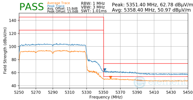
Plot 7-841. Antenna 5b (Pk & Avg, Ch.58, 802.11ax(SU), MCS4)
