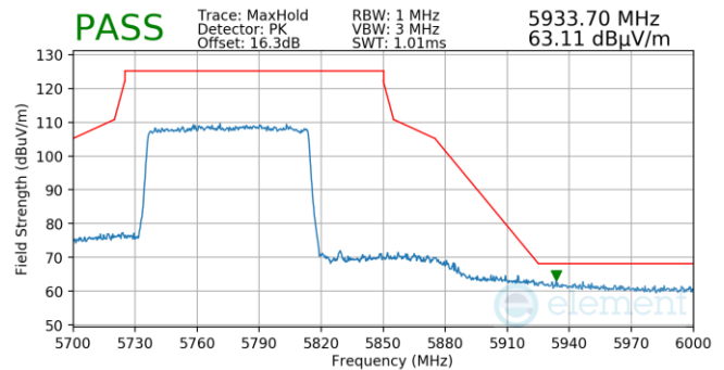
Plot 7-855. Antenna 5b (Pk, Ch.155, 802.11ax(SU), MCS2)
