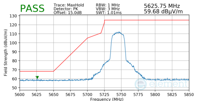
Plot 7-899. Antenna 4a (Pk, Ch.149, 802.11n, MCS2)
