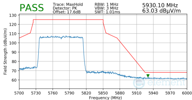
Plot 7-856. Antenna 5b (Pk, Ch.155, 802.11ax(SU), MCS4)
