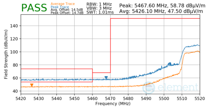
Plot 7-890. Antenna 4a (Pk & Avg, Ch.104, 802.11n, MCS4)
