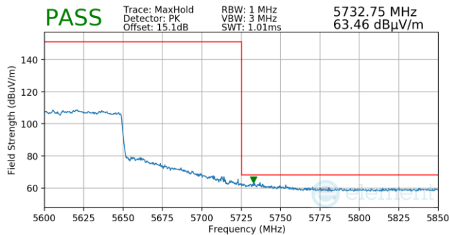
Plot 7-851. (FCC Only) Antenna 5b (Pk, Ch.122, 802.11ax(SU), MCS11)
