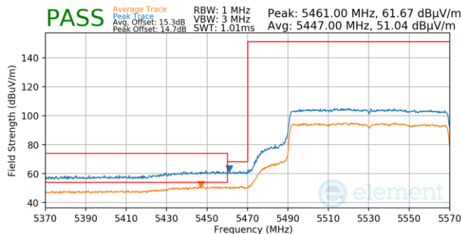
Plot 7-843. Antenna 5b (Pk & Avg, Ch.106, 802.11ax(SU), MCS2)
