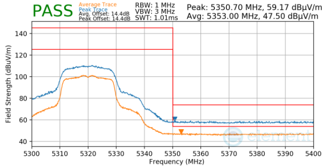
Plot 7-884. Antenna 4a (Pk & Avg, Ch.64, 802.11n, MCS2)
