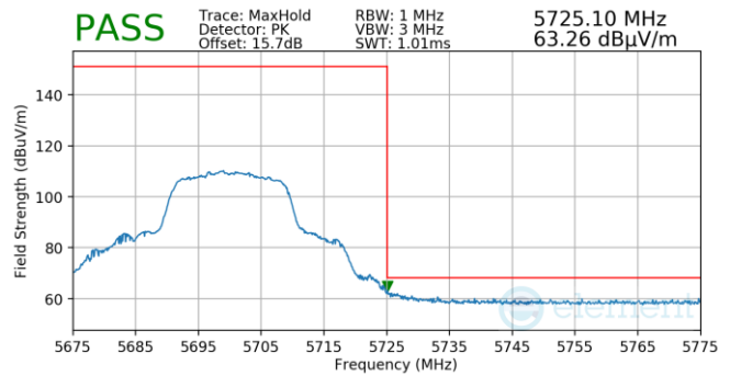
Plot 7-897. Antenna 4a (Pk, Ch.140, 802.11n, MCS4)
