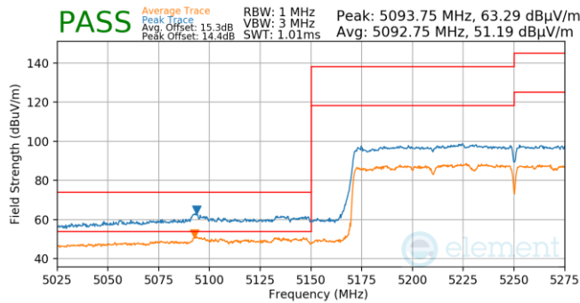
Plot 7-868. Antenna 5b (Pk & Avg, Ch.50, 802.11ax(SU), MCS4)
