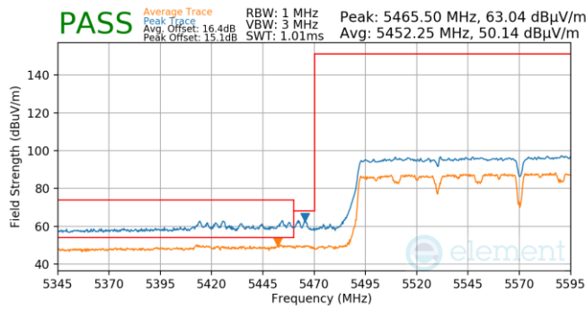
Plot 7-866. (FCC Only) Antenna 5b (Pk & Avg, Ch.114, 802.11n, MCS11)
