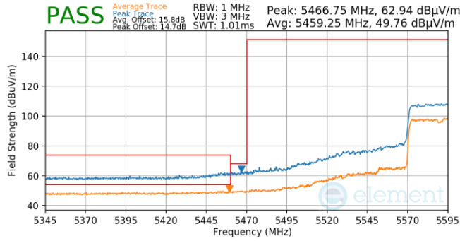
Plot 7-848. (FCC Only) Antenna 5b (Pk & Avg, Ch.122, 802.11ax(SU), MCS11)
