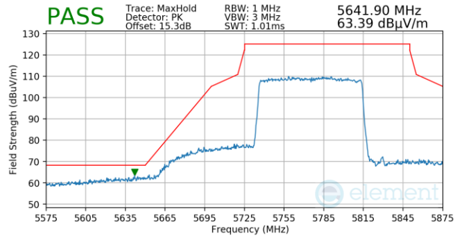
Plot 7-852. Antenna 5b (Pk, Ch.155, 802.11ax(SU), MCS2)
