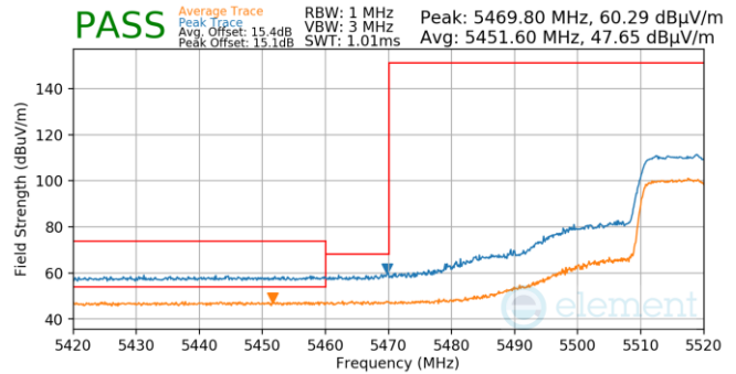
Plot 7-921. Antenna 4a (Pk & Avg, Ch.104, 802.11ax(SU), MCS4)
