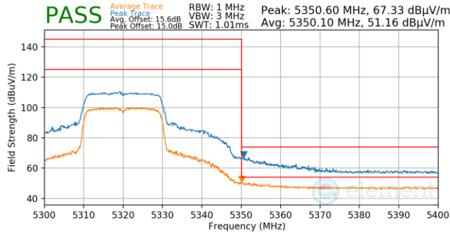
Plot 7-916. Antenna 4a (Pk & Avg, Ch.64, 802.11ax(SU), MCS11)
