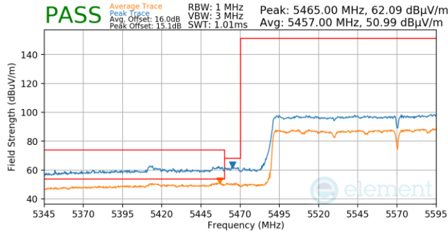
Plot 7-874. Antenna 5b (FCC Only) (Pk & Avg. CH. 114, 802.11ax(SU), MCS4)
