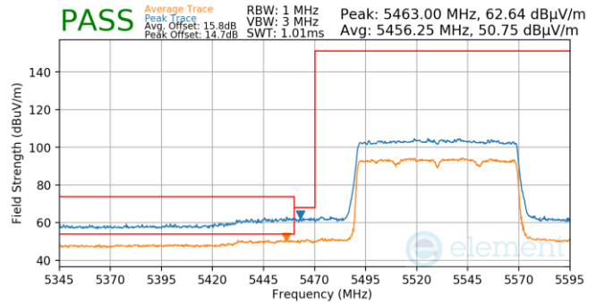
Plot 7-845. Antenna 5b (Pk & Avg, Ch.106, 802.11ax(SU), MCS11)
