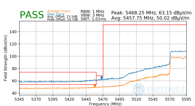
Plot 7-847. (FCC Only) Antenna 5b (Pk & Avg, Ch.122, 802.11ax(SU), MCS4)
