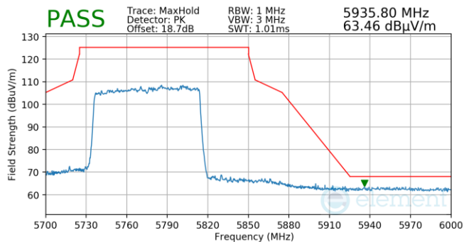
Plot 7-857. Antenna 5b (Pk, Ch.155, 802.11ax(SU), MCS11)
