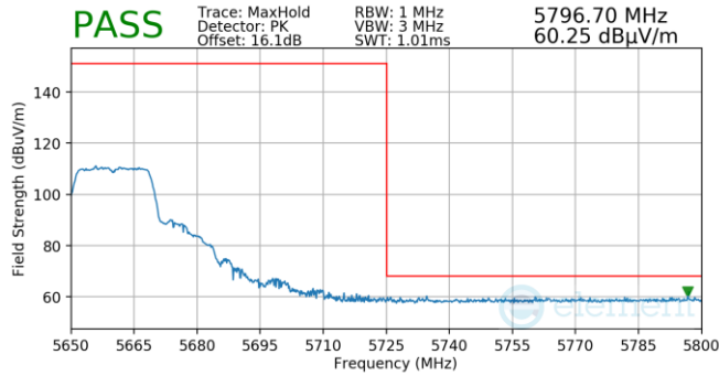
Plot 7-892. Antenna 4a (Pk, Ch.132, 802.11n, MCS7)
