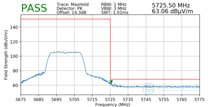
Plot 7-898. Antenna 4a (Pk, Ch.140, 802.11n, MCS7)
