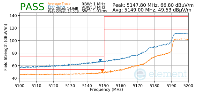
Plot 7-881. Antenna 4a (Pk & Avg, Ch.40, 802.11n, MCS7)
