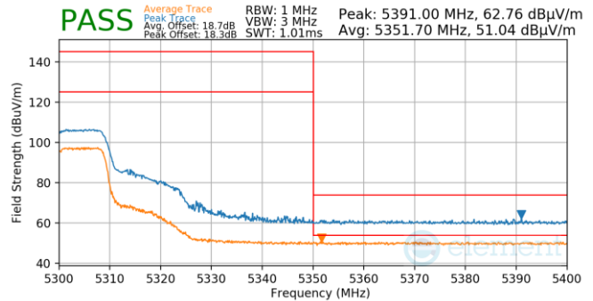
Plot 7-883. Antenna 4a (Pk & Avg, Ch.60, 802.11n, MCS7)
