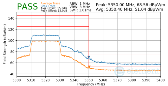
Plot 7-915. Antenna 4a (Pk & Avg, Ch.64, 802.11ax(SU), MCS4)
