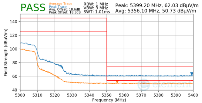
Plot 7-882. Antenna 4a (Pk & Avg, Ch.60, 802.11n, MCS4)
