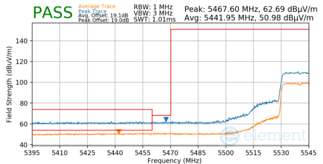
Plot 7-923. Antenna 4a (Pk & Avg, Ch.108, 802.11ax(SU), MCS4)
