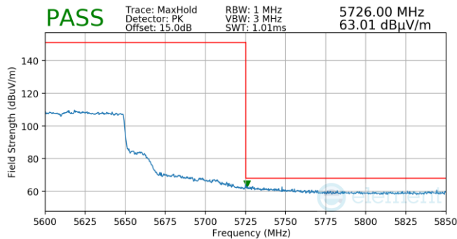
Plot 7-850. (FCC Only) Antenna 5b (Pk, Ch.122, 802.11ax(SU), MCS4)
