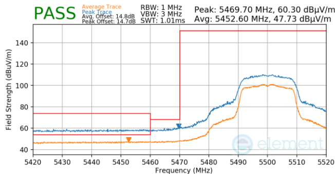
Plot 7-887. Antenna 4a (Pk & Avg, Ch.100, 802.11n, MCS2)
