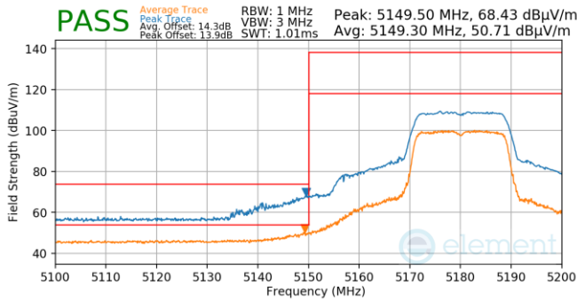
Plot 7-878. Antenna 4a (Pk & Avg, Ch.36, 802.11n, MCS7)
