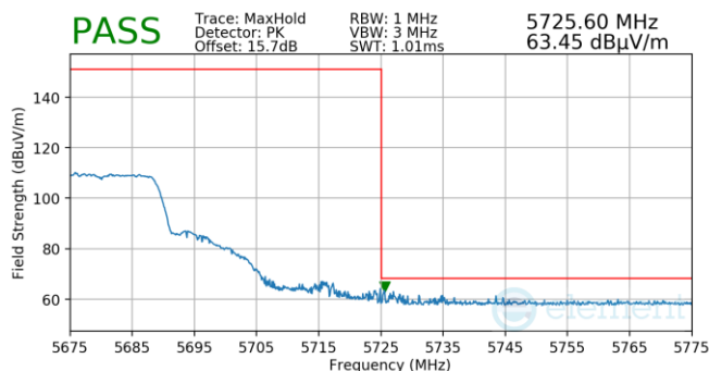
Plot 7-895. Antenna 4a (Pk, Ch.136, 802.11n, MCS7)
