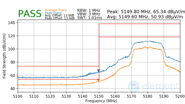
Plot 7-876. Antenna 4a (Pk & Avg, Ch.36, 802.11n, MCS2)
