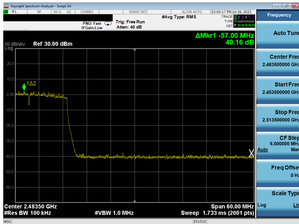
Plot 7-296. Band Edge Plot Antenna 4a (802.11ax (SU - 2.4GHz) - Ch. 10) - MCS5
