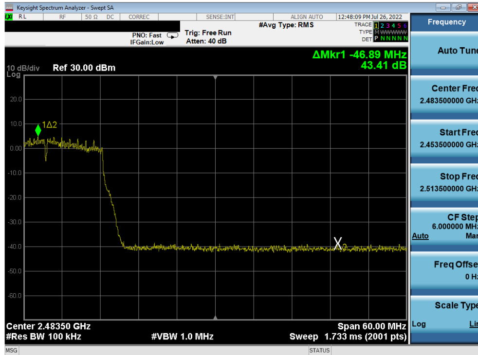
Plot 7-232. Band Edge Plot Antenna 4a (802.11n (2.4GHz) - Ch. 10) - MCS3
