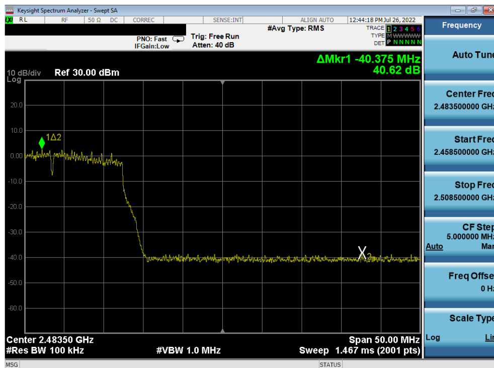
Plot 7-233. Band Edge Plot Antenna 4a (802.11n (2.4GHz) - Ch. 11) - MCS3
