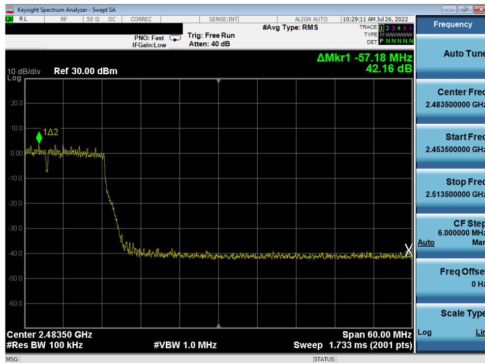
Plot 7-282. Band Edge Plot Antenna 4a (802.11n (2.4GHz) – Ch. 10) – MCS5
