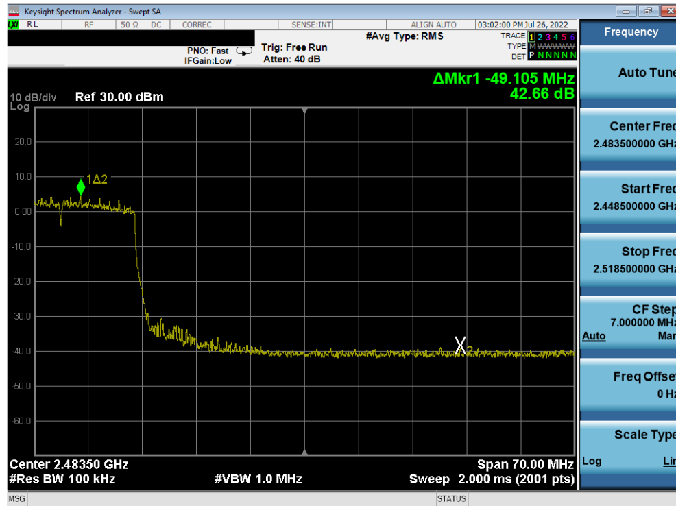
Plot 7-295. Band Edge Plot Antenna 4a (802.11ax (SU - 2.4GHz) - Ch. 9) - MCS5
