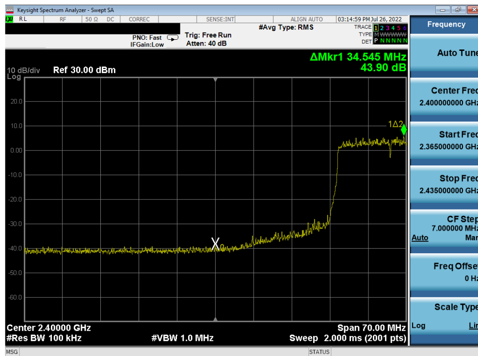
Plot 7-290. Band Edge Plot Antenna 4a (802.11ax (SU - 2.4GHz) – Ch. 5) – MCS5
