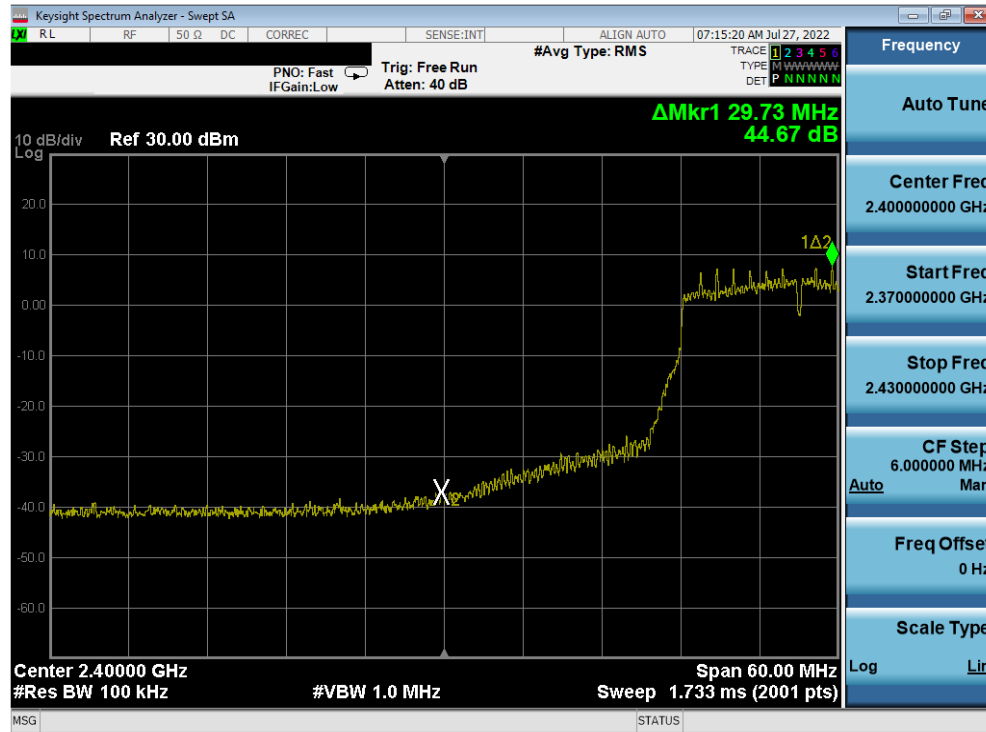
Plot 7-313. Band Edge Plot Antenna 2a (802.11n (2.4GHz) - Ch. 4) - MCS2
