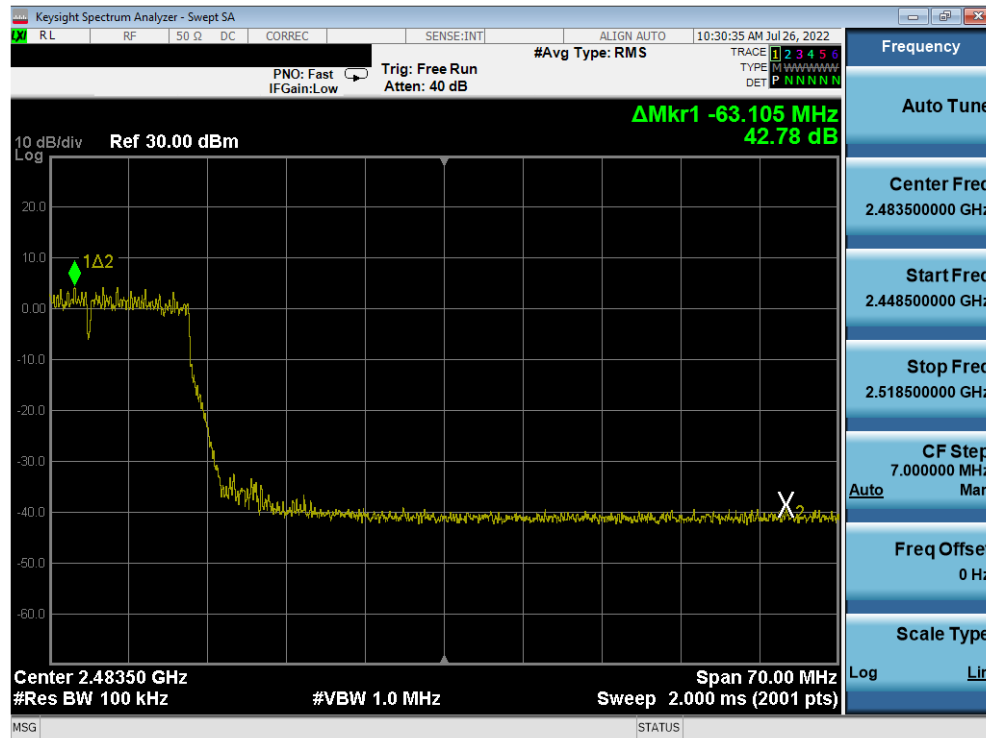
Plot 7-281. Band Edge Plot Antenna 4a (802.11n (2.4GHz) – Ch. 9) – MCS5
