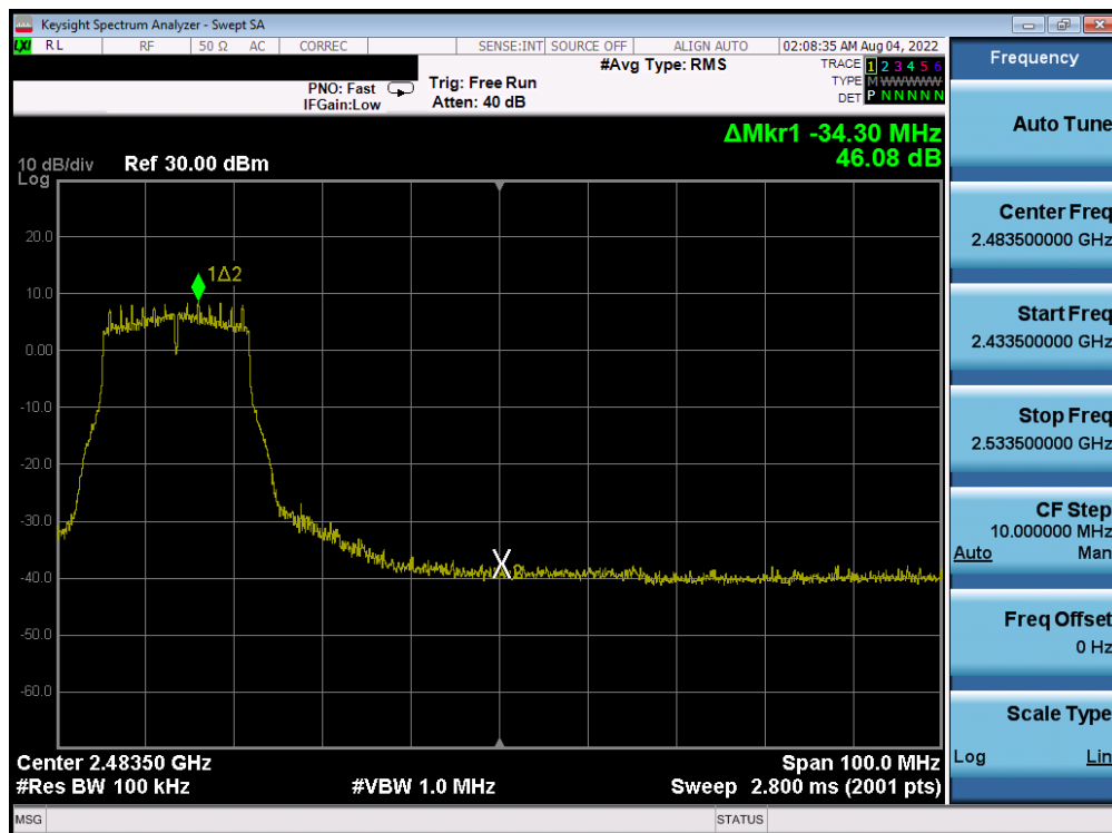
Plot 7-217. Band Edge Plot Antenna 4a (802.11g- Ch. 8) – 18Mbps
