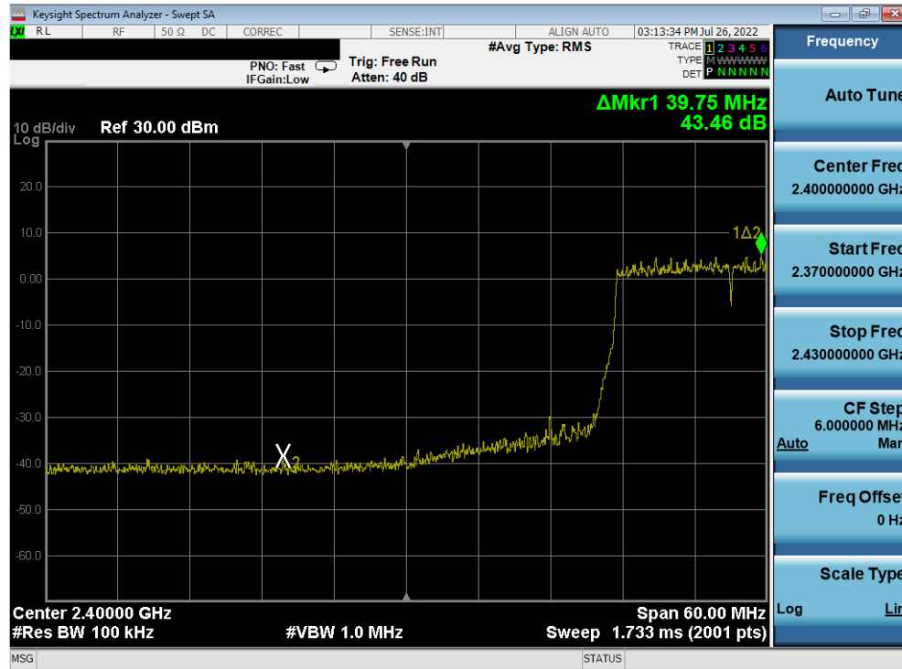
Plot 7-289. Band Edge Plot Antenna 4a (802.11ax (SU - 2.4GHz) – Ch. 4) – MCS5
