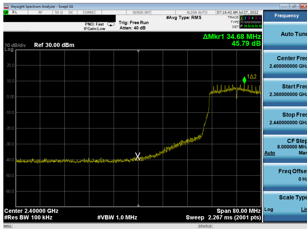
Plot 7-314. Band Edge Plot Antenna 2a (802.11n (2.4GHz) - Ch. 5) - MCS2
