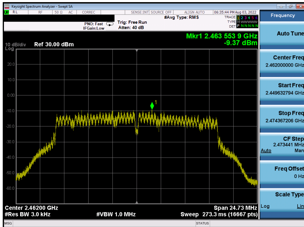
Plot 7-84. Power Spectral Density Plot Antenna 4a (802.11g – Ch. 11) – 36Mbps
