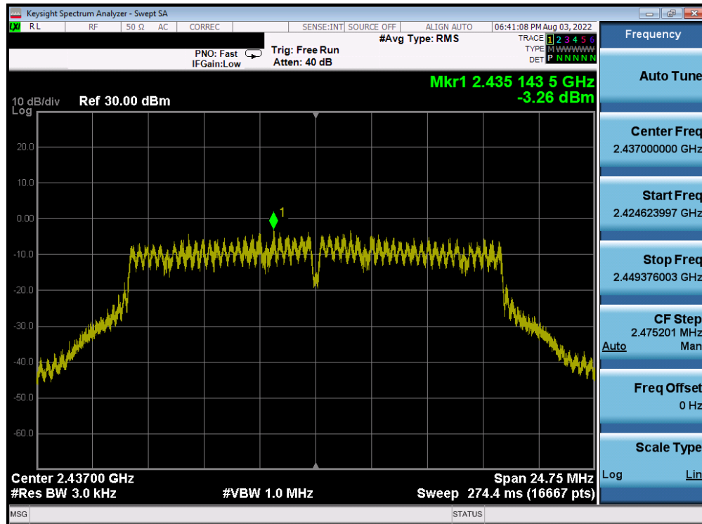
Plot 7-83. Power Spectral Density Plot Antenna 4a (802.11g – Ch. 6) – 36Mbps
