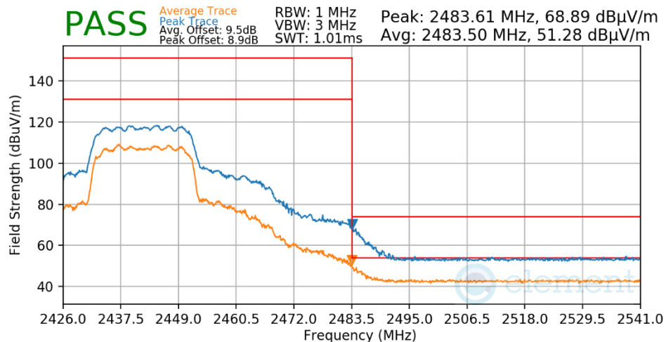
Plot 7-188. Radiated Restricted Upper Band Edge Measurement CDD (Peak & Average – RU242)
