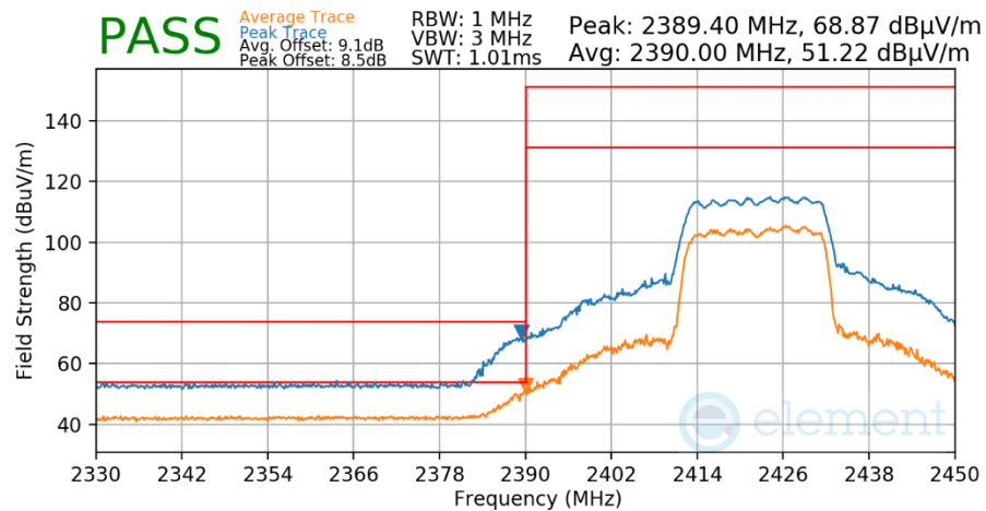
Plot 7-183. Radiated Restricted Lower Band Edge Measurement CDD (Peak & Average – RU242)
