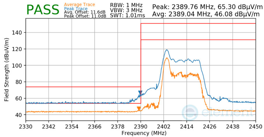
Plot 7-179. Radiated Restricted Lower Band Edge Measurement CDD (Peak & Average – RU26)
