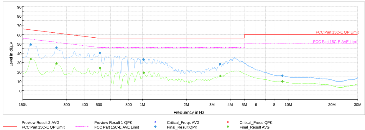
Plot 7-199. AC Line Conducted Emissions with 802.11ax (RU242) Ch.11 (N, with AC/DC Adapter)
