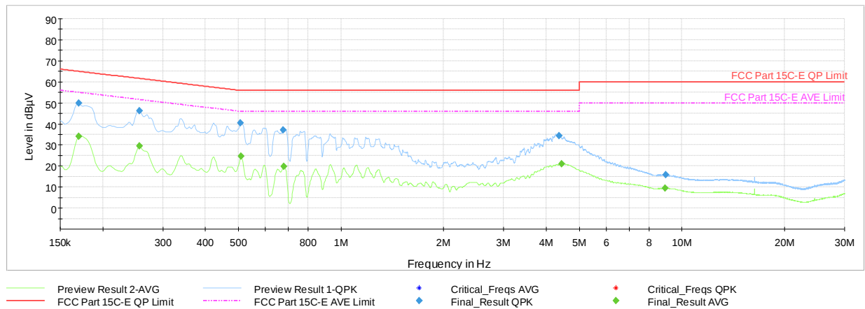
Plot 7-197. AC Line Conducted Emissions with 802.11ax (RU26) Ch.6 (N, with AC/DC Adapter)
