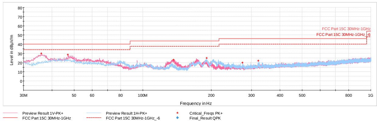
Plot 7-194. Radiated Spurious Emissions below 1GHz CDD Ch.6 (RU26), with AC/DC Adapter
