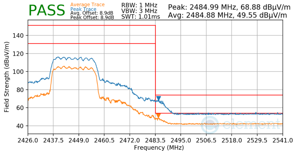
Plot 7-189. Radiated Restricted Upper Band Edge Measurement CDD (Peak & Average – RU242)
