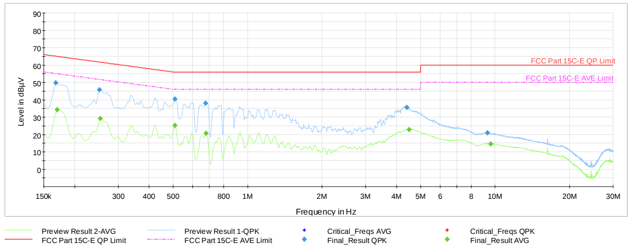
Plot 7-198. AC Line Conducted Emissions with 802.11ax (RU242) Ch.6 (L1, with AC/DC Adapter)
