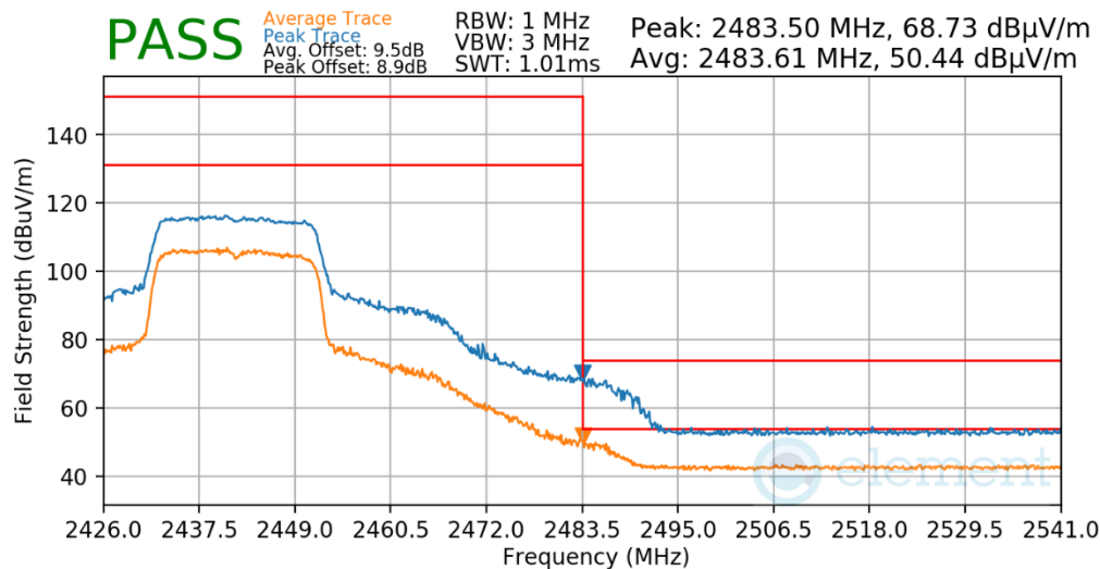
Plot 7-173. Radiated Restricted Upper Band Edge Measurement Antenna 2a (Peak & Average – RU242)
