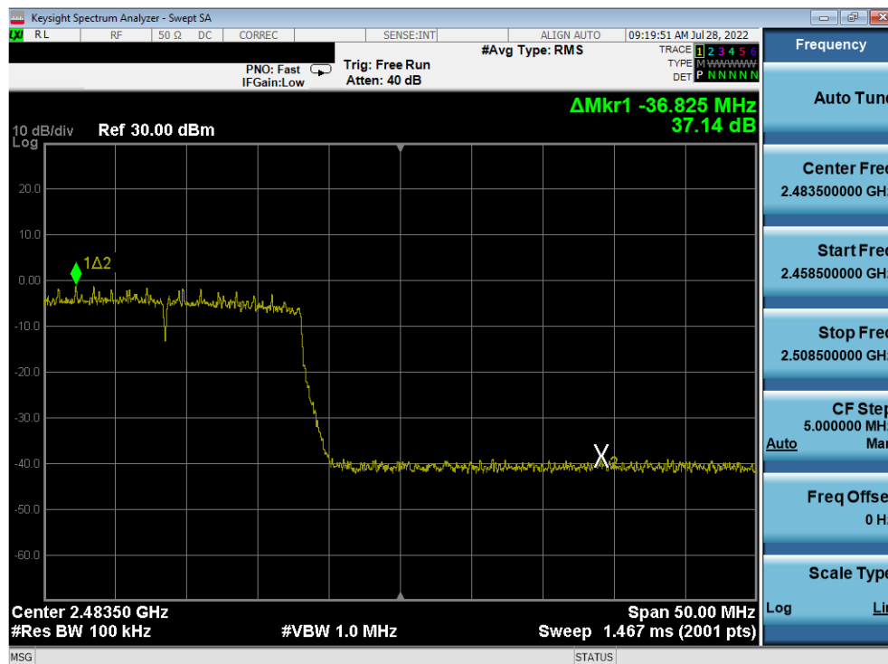
Plot 7-87. Band Edge Antenna 4a (802.11ax OFDMA – RU242 – Ch. 12)
