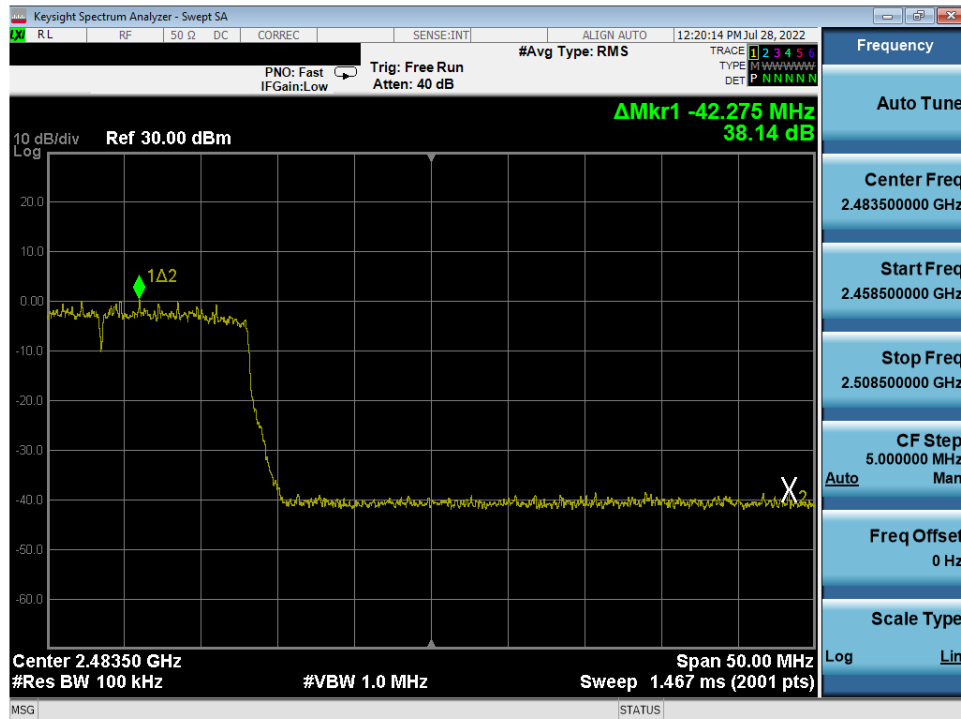
Plot 7-101. Band Edge Antenna 2a (802.11ax OFDMA – RU242 – Ch. 11)
