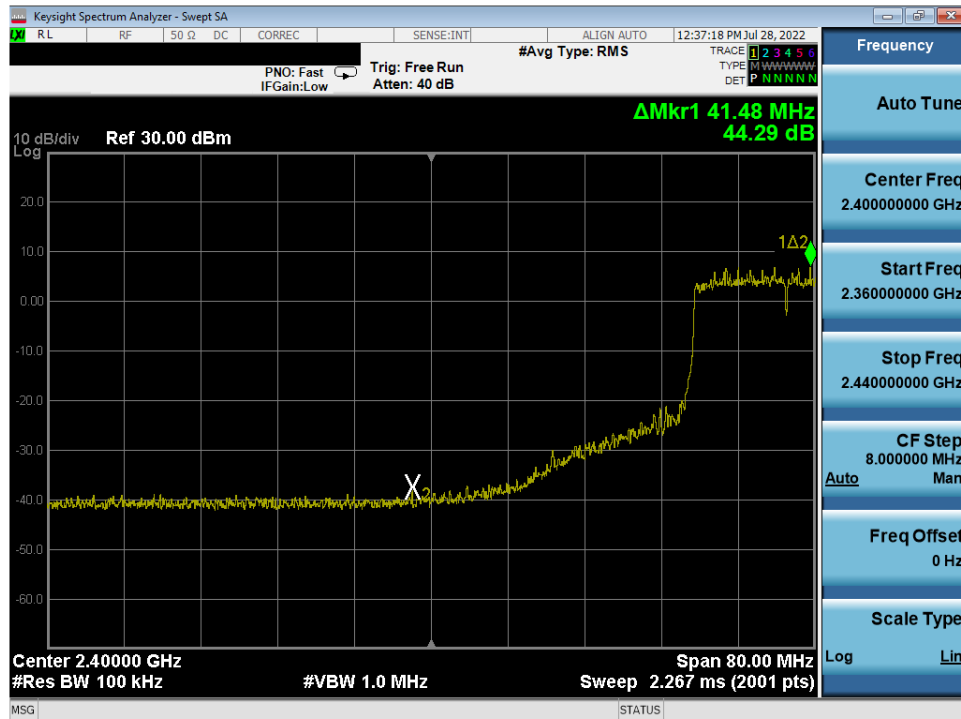
Plot 7-95. Band Edge Antenna 2a (802.11ax OFDMA – RU242 – Ch. 6)
