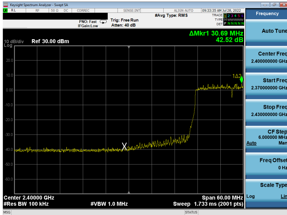
Plot 7-78. Band Edge Antenna 4a (802.11ax OFDMA – RU242 – Ch. 4)
