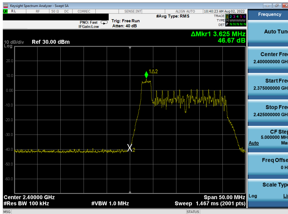
Plot 7-88. Band Edge Antenna 2a (802.11ax OFDMA – RU26 Index 0 – Ch. 1)
