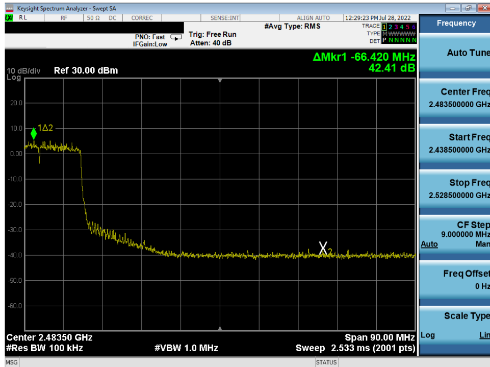
Plot 7-97. Band Edge Antenna 2a (802.11ax OFDMA – RU242 – Ch. 7)
