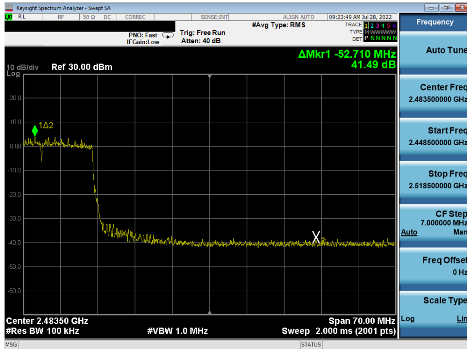
Plot 7-84. Band Edge Antenna 4a (802.11ax OFDMA – RU242 – Ch. 9)
