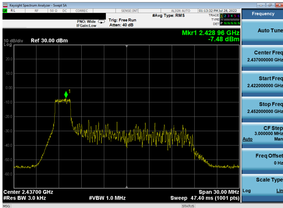
Plot 7-56. Power Spectral Density Plot CDD Antenna 2a (802.11ax OFDMA – RU26 Index 0 – Ch. 6)
