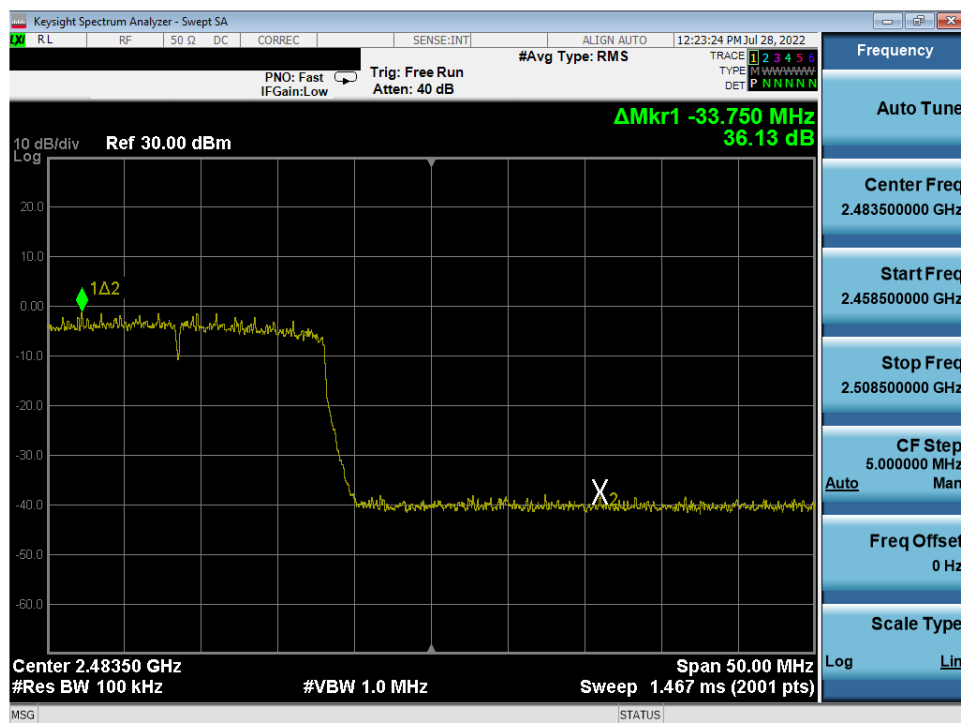
Plot 7-102. Band Edge Antenna 2a (802.11ax OFDMA – RU242 – Ch. 12)
