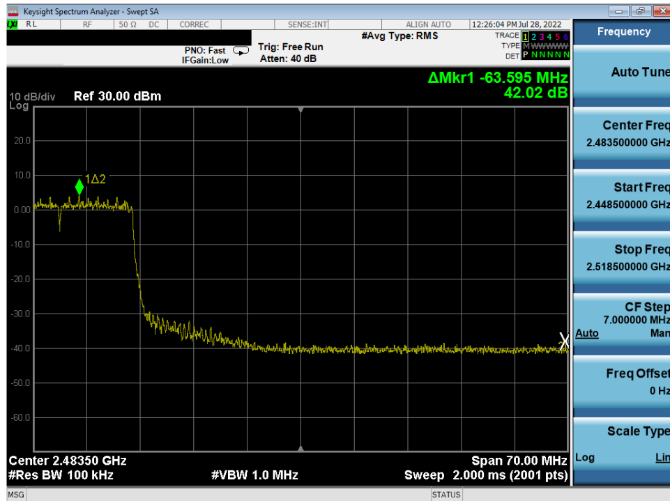
Plot 7-99. Band Edge Antenna 2a (802.11ax OFDMA – RU242 – Ch. 9)
