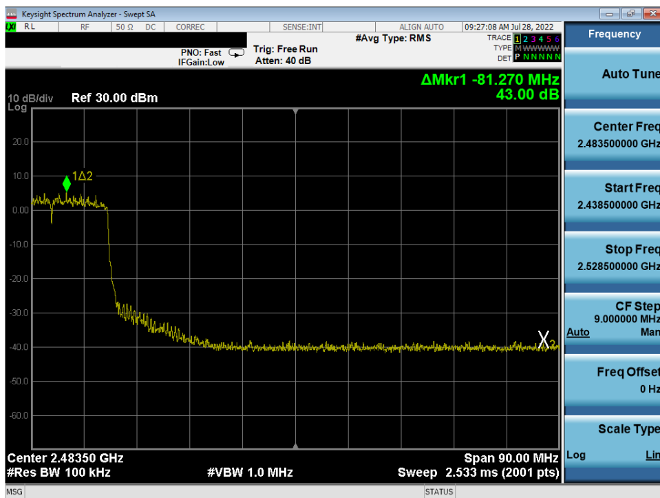
Plot 7-82. Band Edge Antenna 4a (802.11ax OFDMA – RU242 – Ch. 7)
