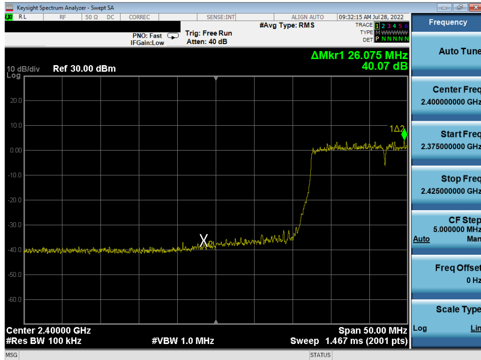
Plot 7-77. Band Edge Antenna 4a (802.11ax OFDMA – RU242 – Ch. 3)
