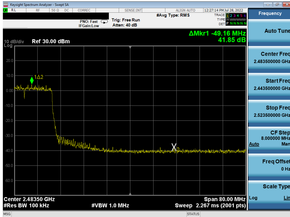
Plot 7-98. Band Edge Antenna 2a (802.11ax OFDMA – RU242 – Ch. 8)
