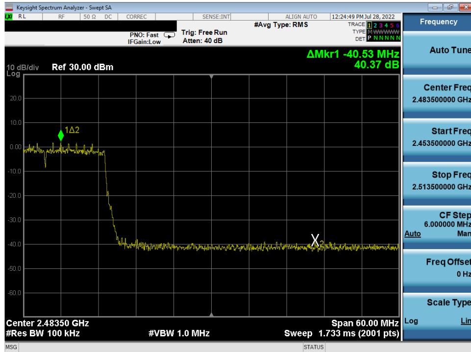
Plot 7-100. Band Edge Antenna 2a (802.11ax OFDMA – RU242 – Ch. 10)
