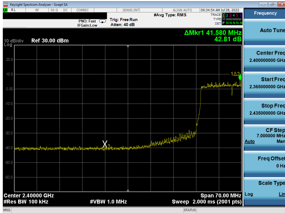
Plot 7-79. Band Edge Antenna 4a (802.11ax OFDMA – RU242 – Ch. 5)
