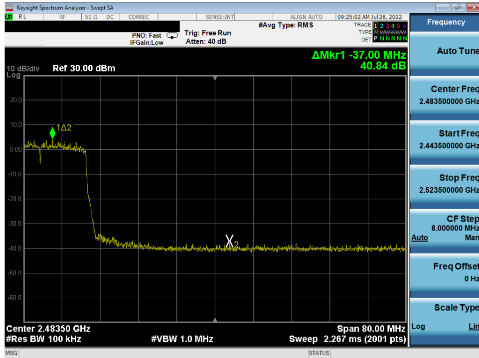
Plot 7-83. Band Edge Antenna 4a (802.11ax OFDMA – RU242 – Ch. 8)
