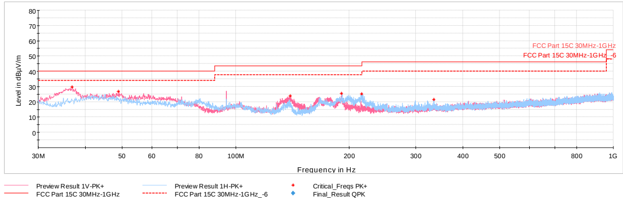
Plot 7-104. Radiated Spurious Emissions Below 1GHz TxBF (4Mbps, ePA – Ch.38 with AC/DC Adapter)
