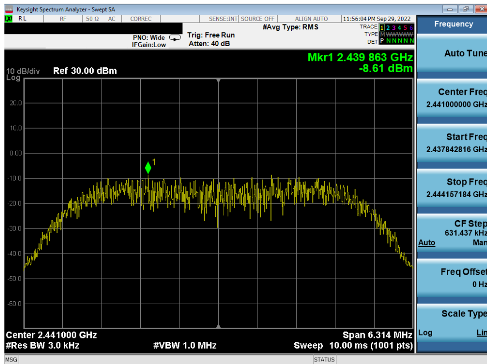
Plot 7-20. Power Spectral Density Plot Antenna 4a (Bluetooth (HDR8), 8Mbps, ePA – Ch. 38)
