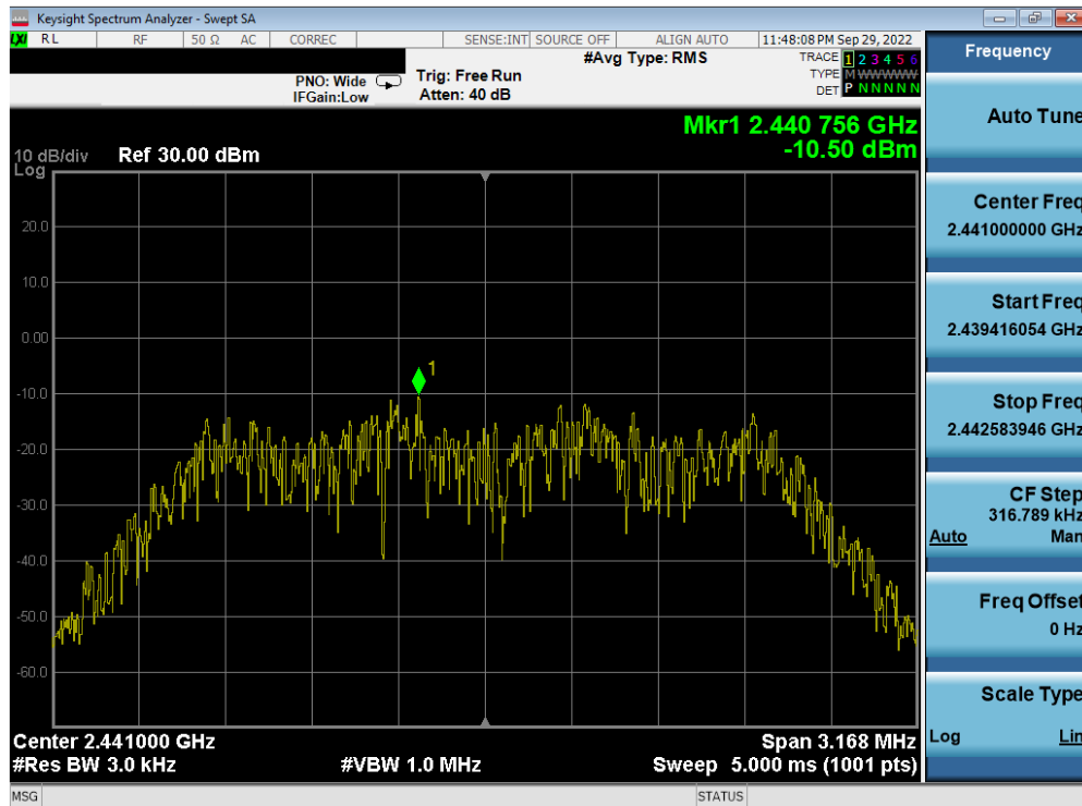
Plot 7-17. Power Spectral Density Plot Antenna 4a (Bluetooth (HDR4), 4Mbps, iPA – Ch. 38)
