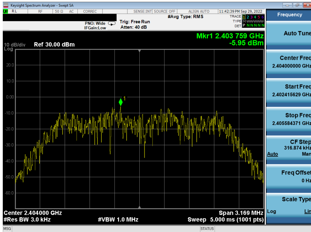
Plot 7-13. Power Spectral Density Plot Antenna 4a (Bluetooth (HDR4), 4Mbps, ePA – Ch. 1)
