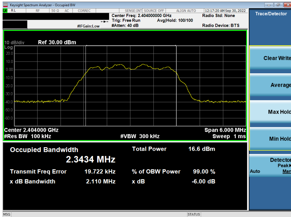
Plot 7-7. 6dB BW & 99% OBW Plot Antenna 2a (Bluetooth (HDR4), 4Mbps, ePA – Ch. 1)
