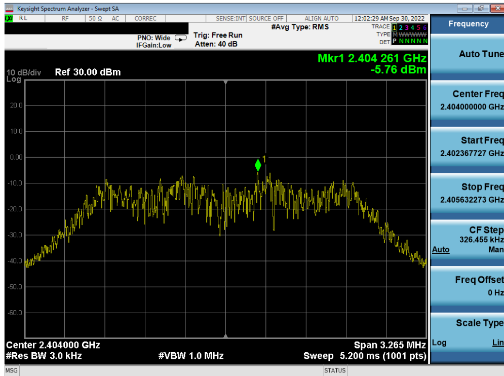
Plot 7-37. Power Spectral Density Plot TxBF Antenna 4a (Bluetooth (HDR4), 4Mbps, ePA – Ch. 1)
