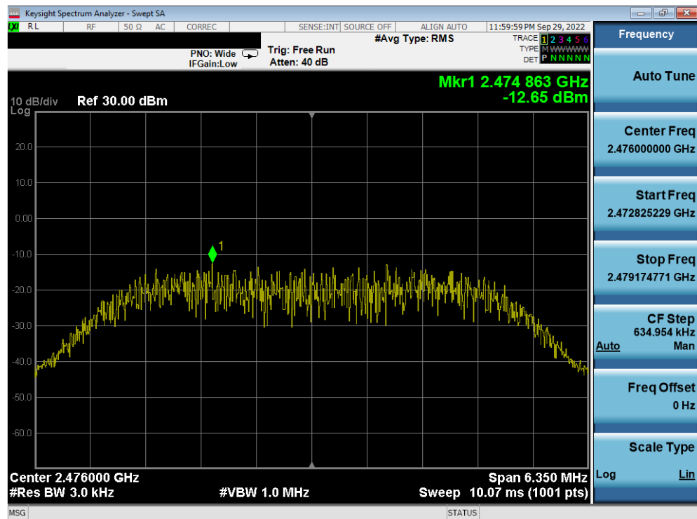
Plot 7-24. Power Spectral Density Plot Antenna 4a (Bluetooth (HDR8), 8Mbps, iPA – Ch. 73)
