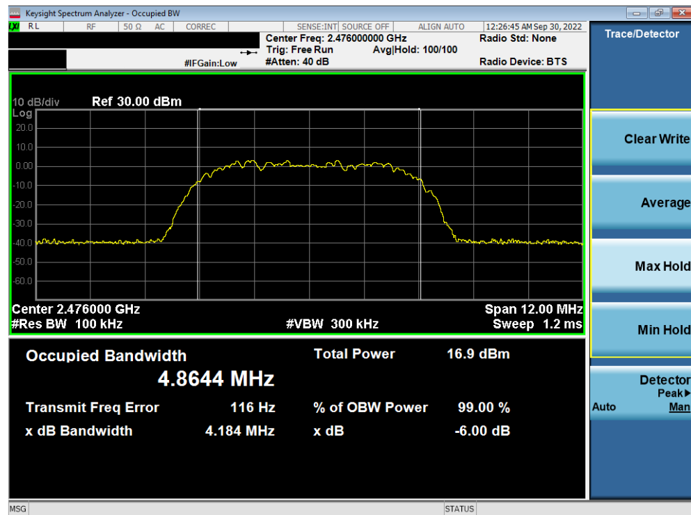
Plot 7-12. 6dB BW & 99% OBW Plot Antenna 2a (Bluetooth (HDR8), 8Mbps, ePA – Ch. 73)
