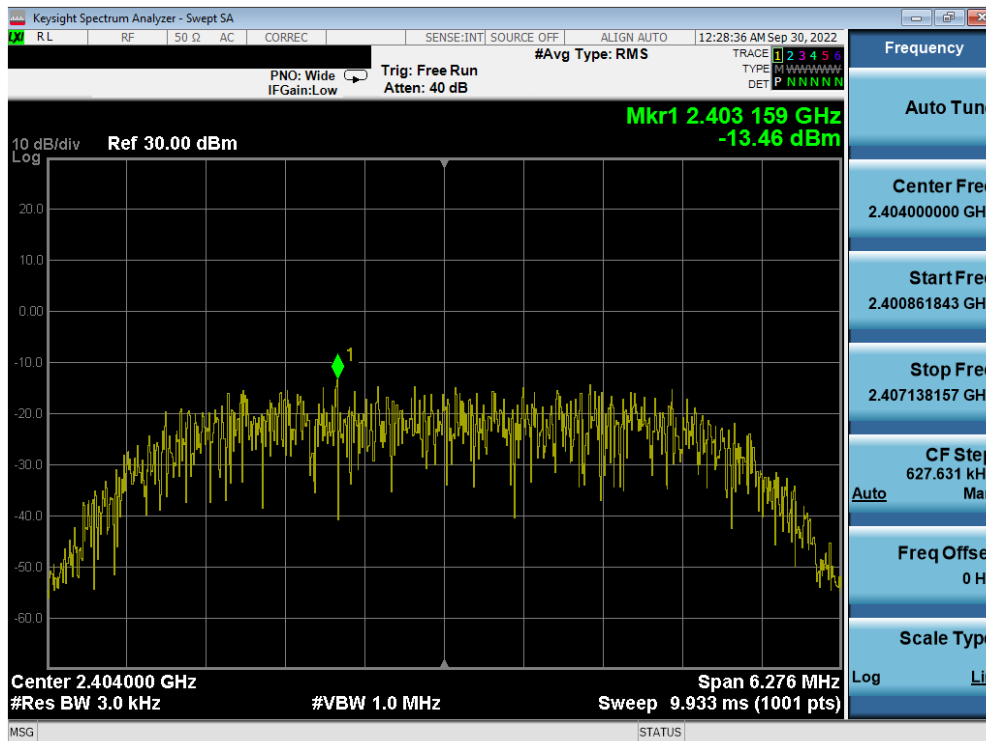
Plot 7-34. Power Spectral Density Plot Antenna 2a (Bluetooth (HDR8), 8Mbps, iPA – Ch. 1)
