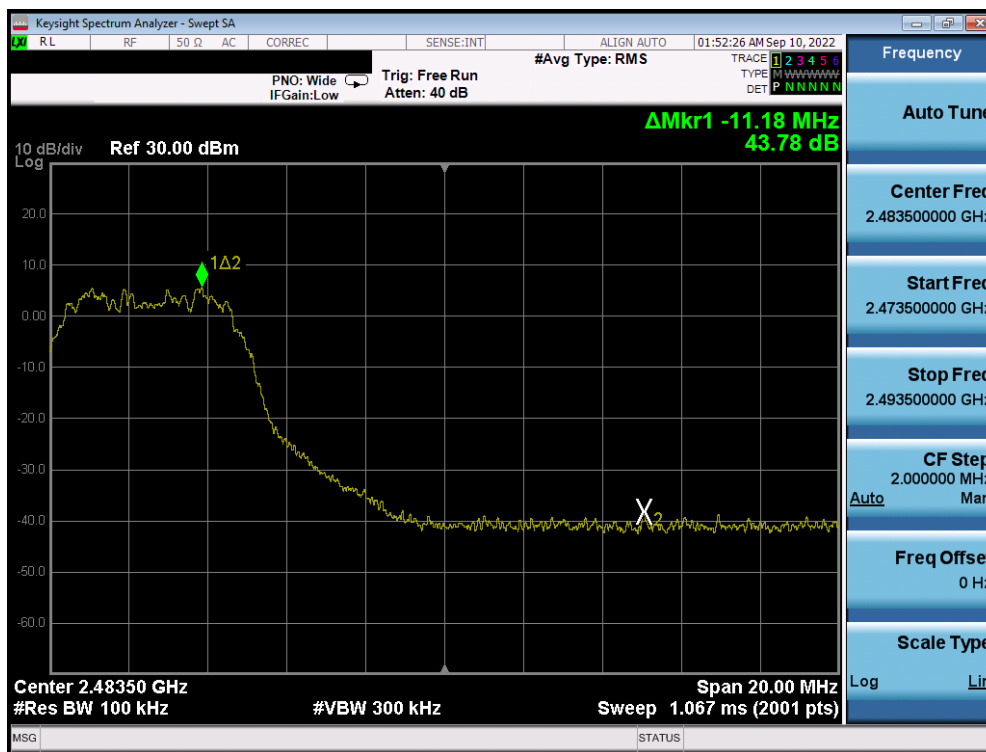
Plot 7-64. Band Edge Plot Antenna 4a (Bluetooth (HDR8), ePA – Ch. 73)
