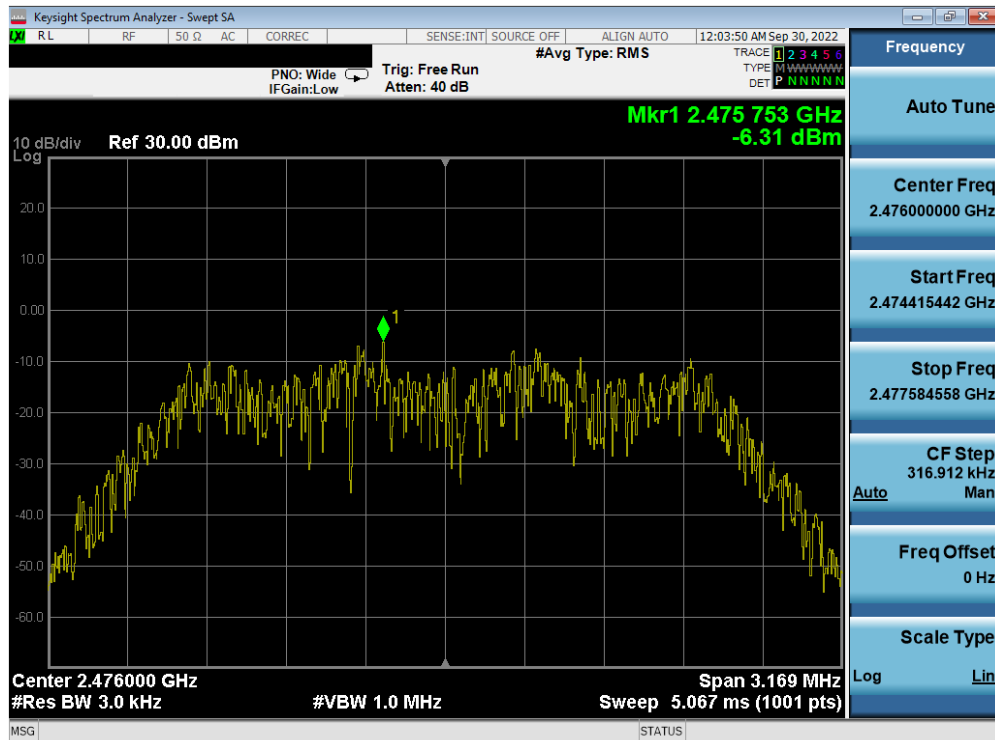
Plot 7-41. Power Spectral Density Plot TxBF Antenna 4a (Bluetooth (HDR4), 4Mbps, ePA – Ch. 73)
