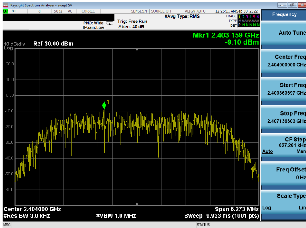
Plot 7-31. Power Spectral Density Plot Antenna 2a (Bluetooth (HDR8), 8Mbps, ePA – Ch. 1)
