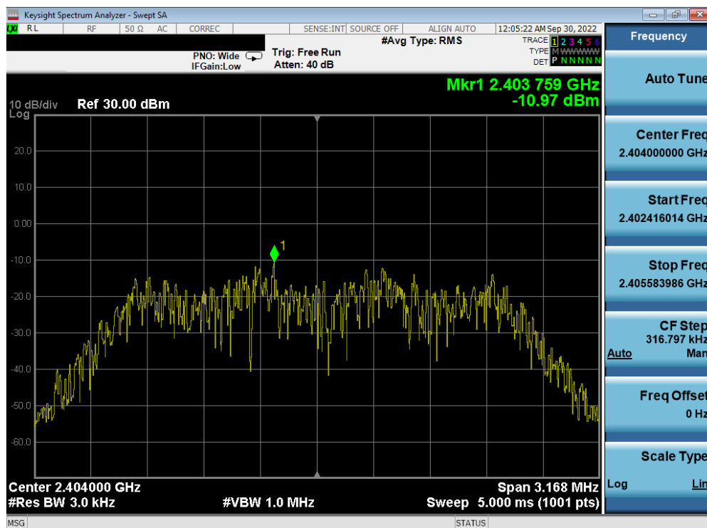
Plot 7-43. Power Spectral Density Plot TxBF Antenna 4a (Bluetooth (HDR4), 4Mbps, iPA – Ch. 1)
