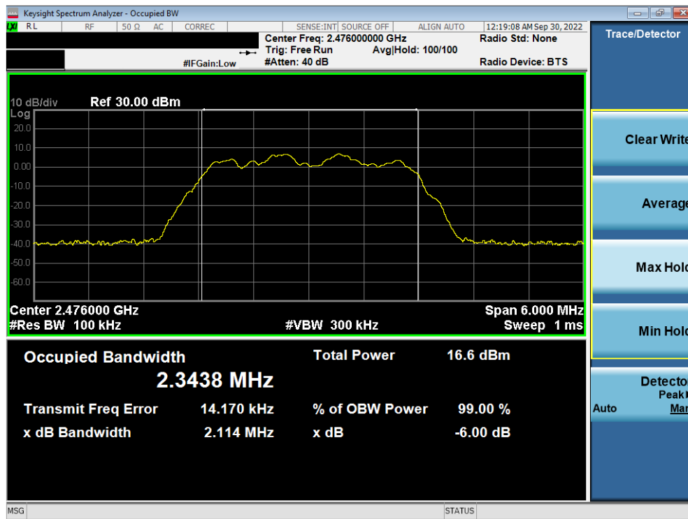
Plot 7-9. 6dB BW & 99% OBW Plot Antenna 2a (Bluetooth (HDR4), 4Mbps, ePA – Ch. 73)
