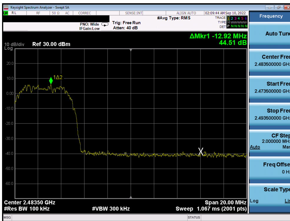
Plot 7-68. Band Edge Plot Antenna 2a (Bluetooth (HDR8), ePA – Ch. 73)
