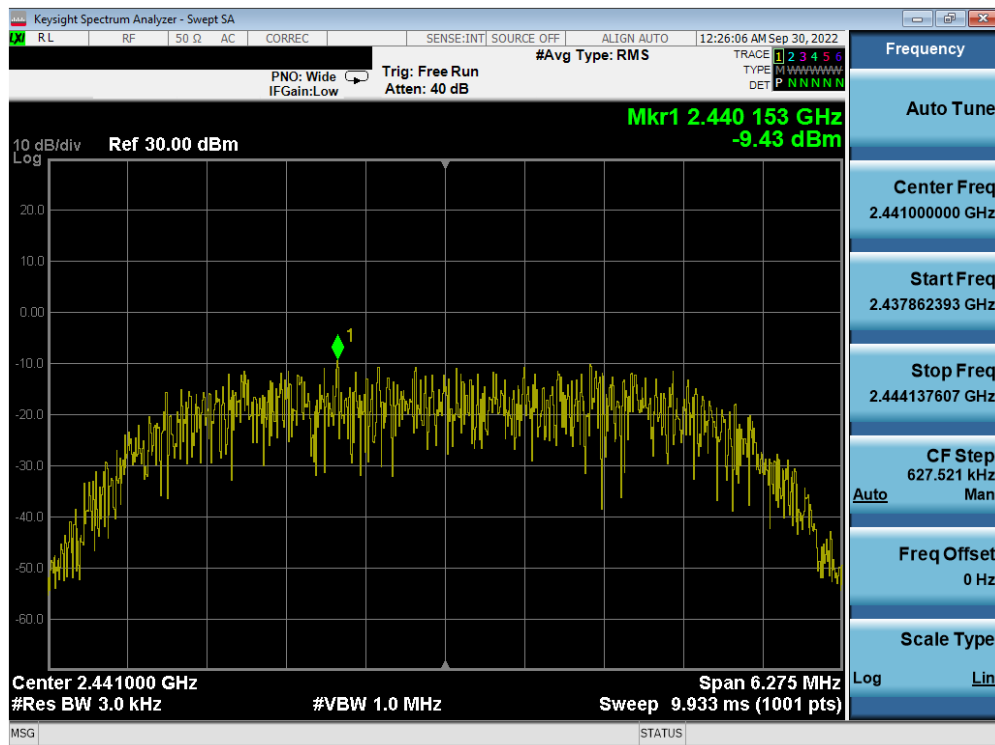
Plot 7-32. Power Spectral Density Plot Antenna 2a (Bluetooth (HDR8), 8Mbps, ePA – Ch. 38)
