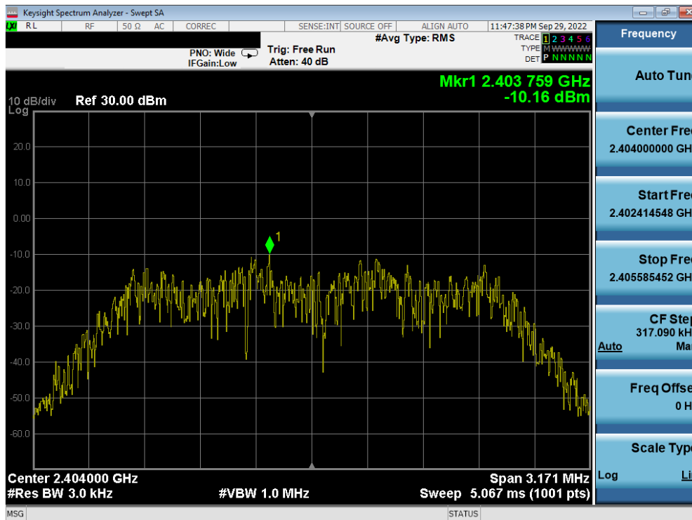
Plot 7-16. Power Spectral Density Plot Antenna 4a (Bluetooth (HDR4), 4Mbps, iPA – Ch. 1)
