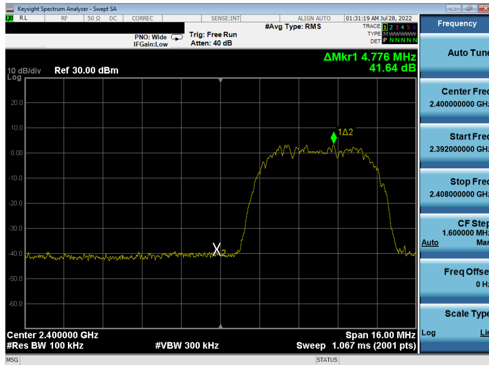
Plot 7-63. Band Edge Plot Antenna 4a (Bluetooth (HDR8), ePA – Ch. 1)
