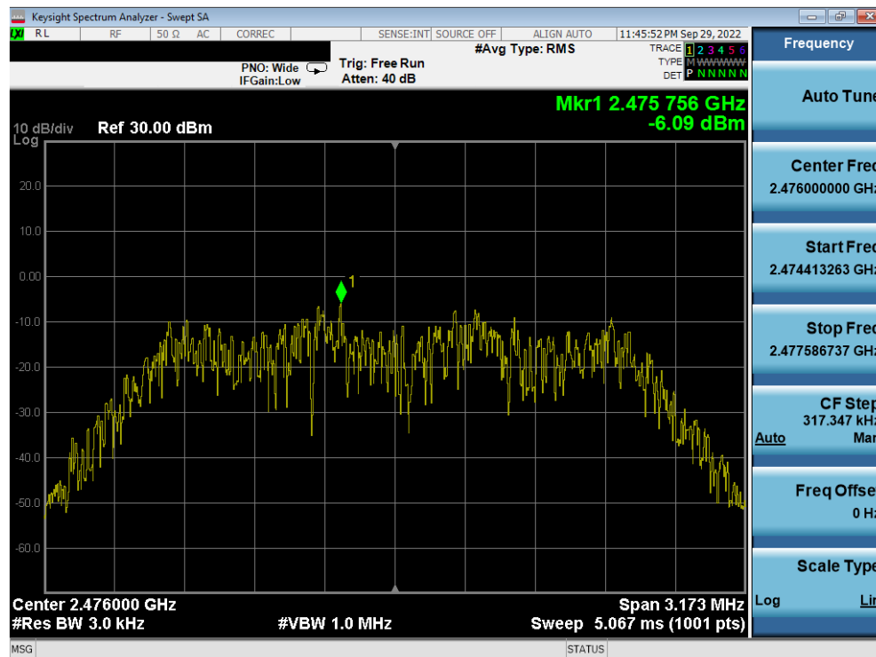
Plot 7-15. Power Spectral Density Plot Antenna 4a (Bluetooth (HDR4), 4Mbps, ePA – Ch. 73)
