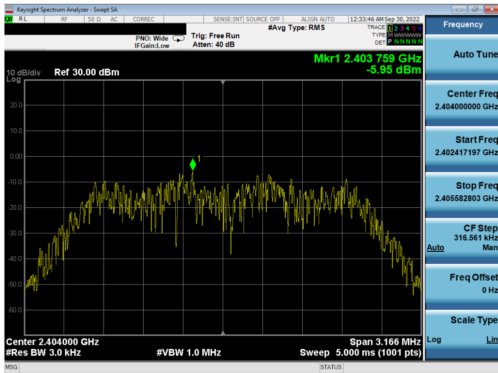
Plot 7-38. Power Spectral Density Plot TxBF Antenna 2a (Bluetooth (HDR4), 4Mbps, ePA – Ch. 1)
