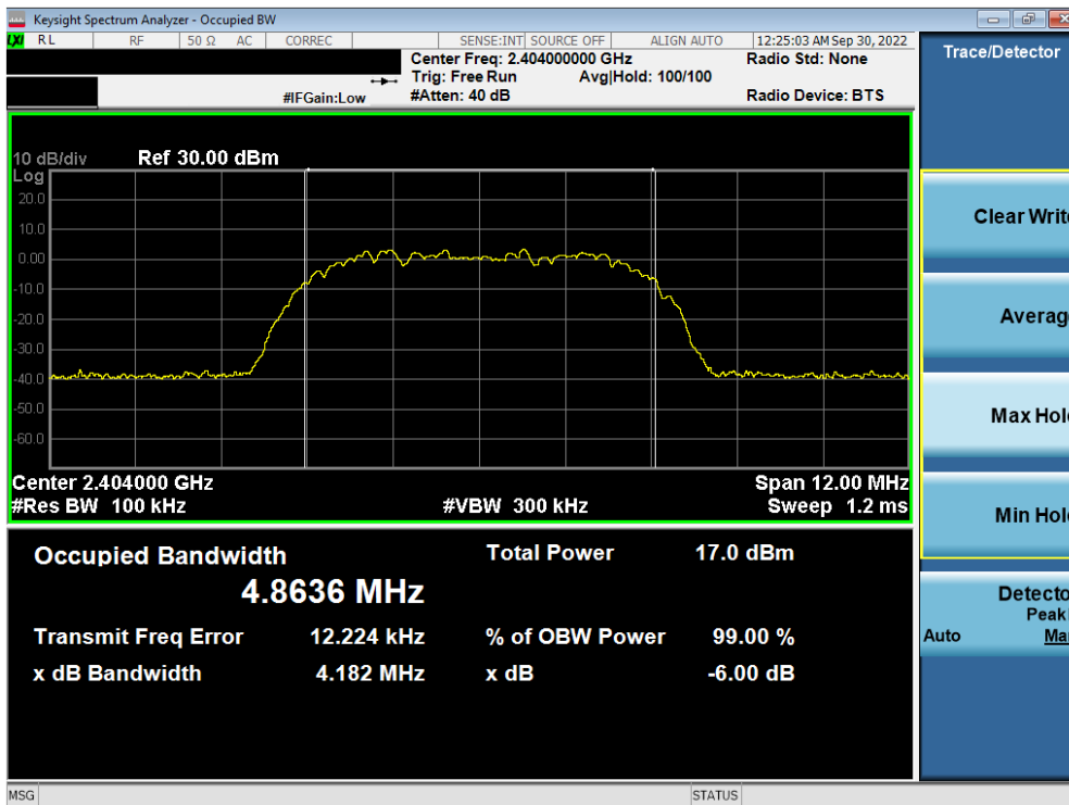
Plot 7-10. 6dB BW & 99% OBW Plot Antenna 2a (Bluetooth (HDR8), 8Mbps, ePA – Ch. 1)
