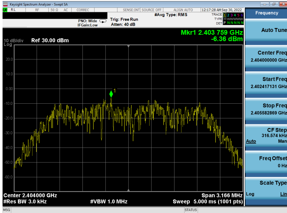
Plot 7-25. Power Spectral Density Plot Antenna 2a (Bluetooth (HDR4), 4Mbps, ePA – Ch. 1)
