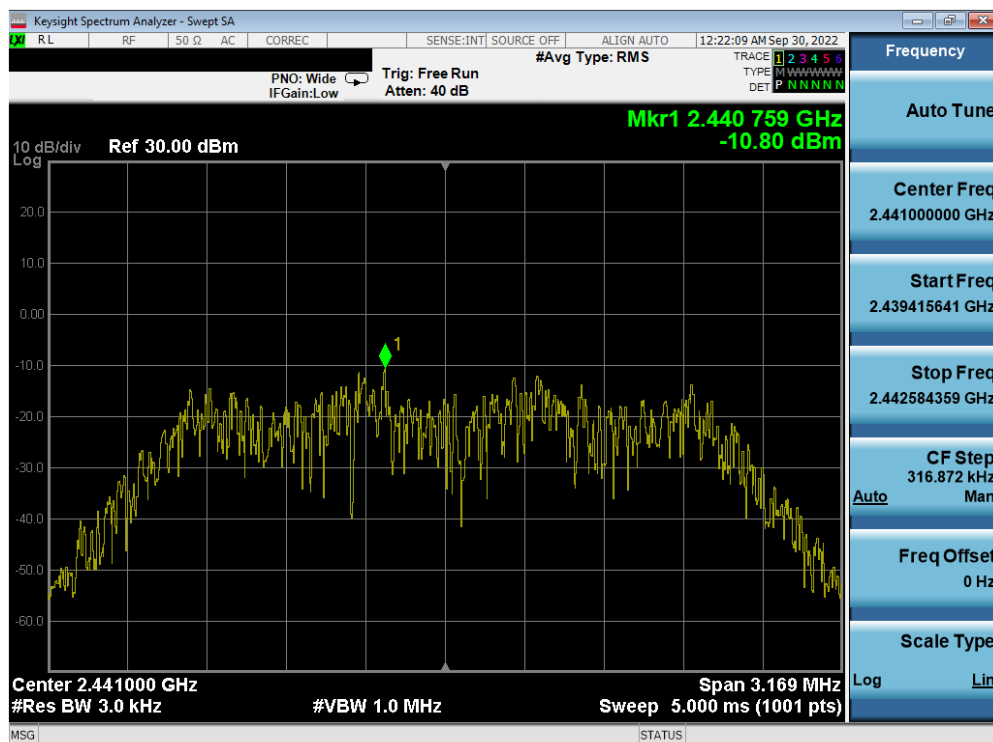
Plot 7-29. Power Spectral Density Plot Antenna 2a (Bluetooth (HDR4), 4Mbps, iPA – Ch. 38)
