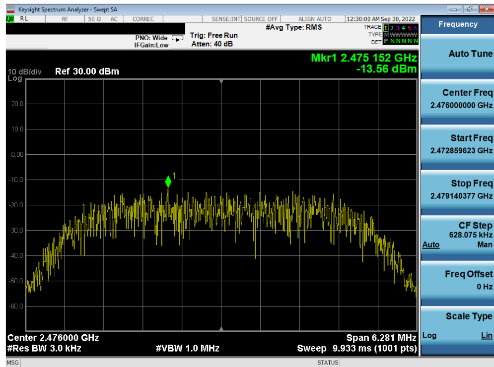
Plot 7-36. Power Spectral Density Plot Antenna 2a (Bluetooth (HDR8), 8Mbps, iPA – Ch. 73)
