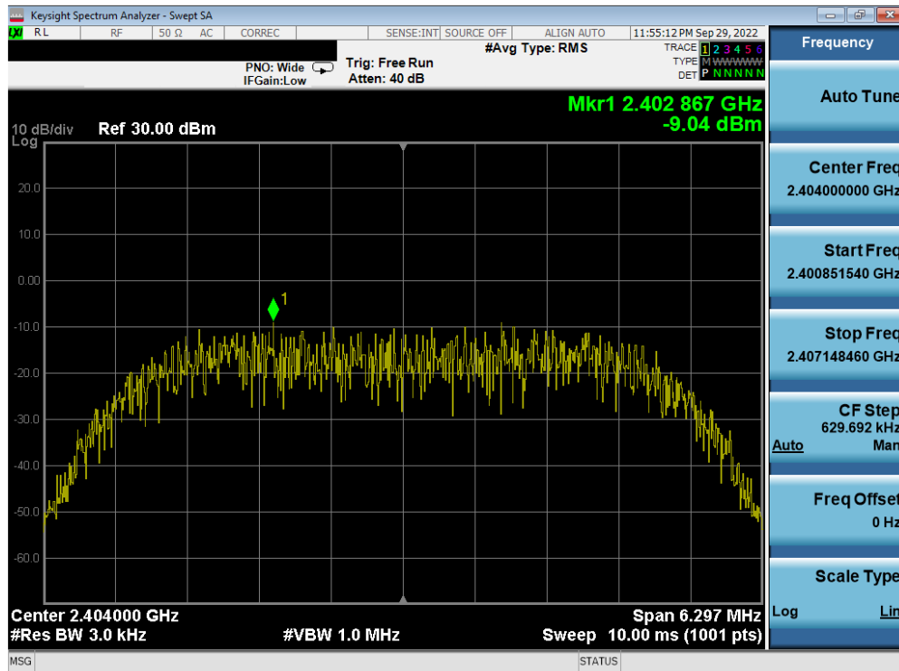
Plot 7-19. Power Spectral Density Plot Antenna 4a (Bluetooth (HDR8), 8Mbps, ePA – Ch. 1)
