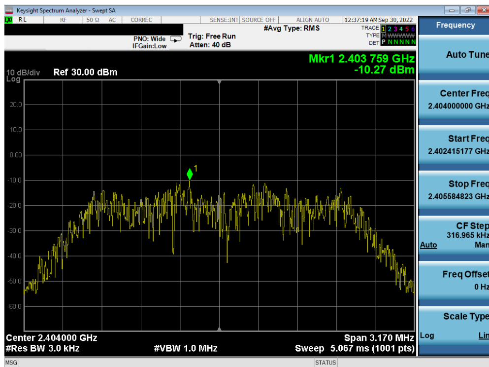
Plot 7-44. Power Spectral Density Plot TxBF Antenna 2a (Bluetooth (HDR4), 4Mbps, iPA – Ch. 1)
