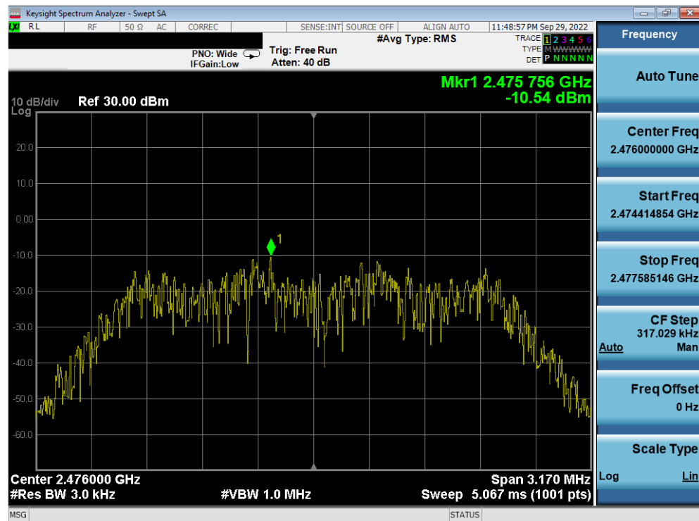
Plot 7-18. Power Spectral Density Plot Antenna 4a (Bluetooth (HDR4), 4Mbps, iPA – Ch. 73)
