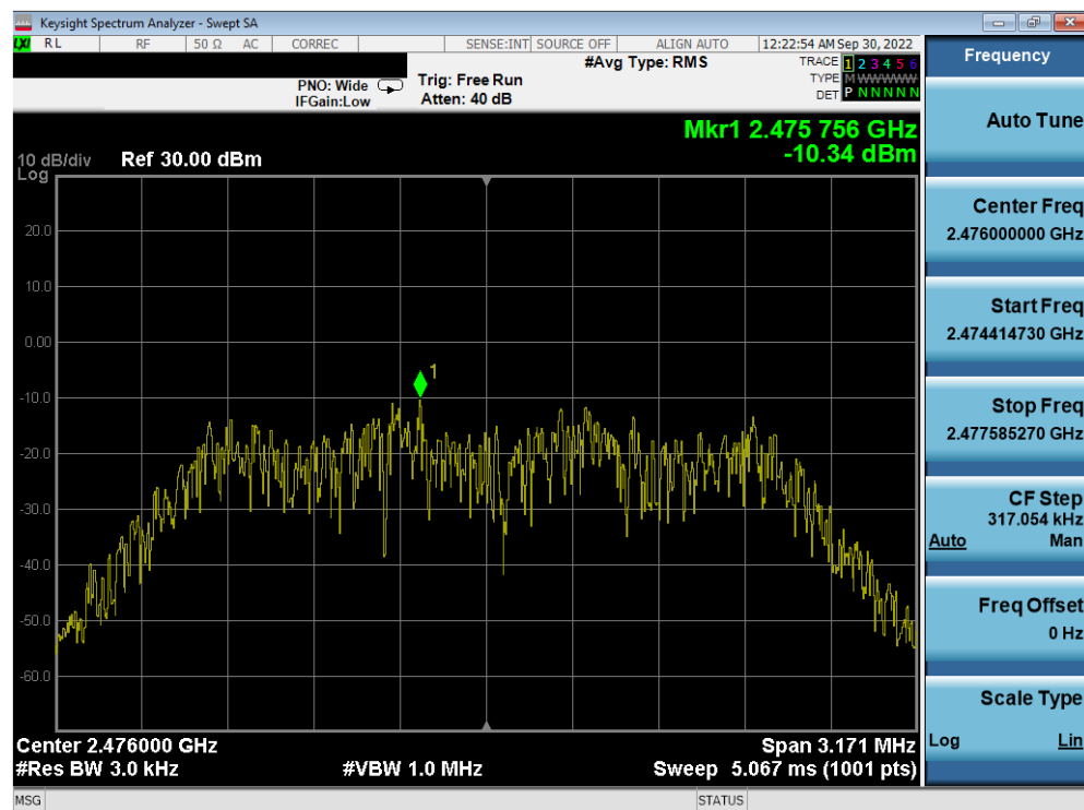
Plot 7-30. Power Spectral Density Plot Antenna 2a (Bluetooth (HDR4), 4Mbps, iPA – Ch. 73)
