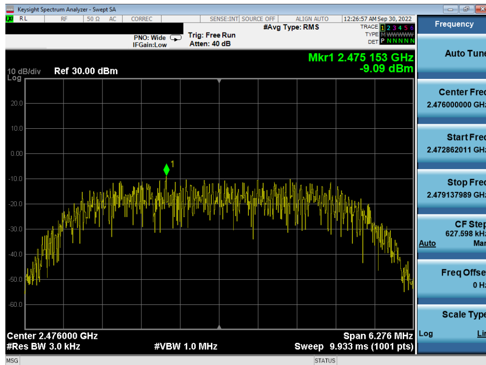
Plot 7-33. Power Spectral Density Plot Antenna 2a (Bluetooth (HDR8), 8Mbps, ePA – Ch. 73)
