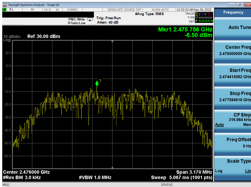
Plot 7-42. Power Spectral Density Plot TxBF Antenna 2a (Bluetooth (HDR4), 4Mbps, ePA – Ch. 73)
