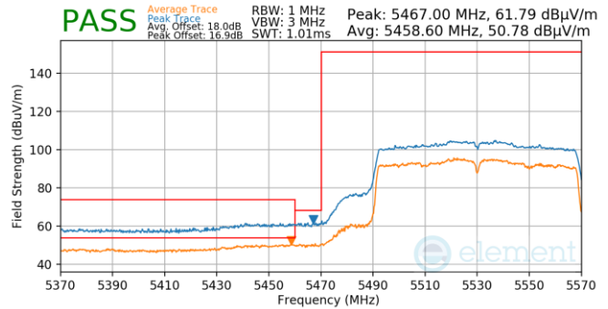
Plot 7-823. Antenna 5b (Pk & Avg, Ch.106, 802.11ac, MCS4)
