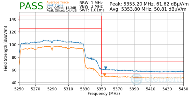
Plot 7-820. Antenna 5b (Pk & Avg, Ch.58, 802.11ac, MCS4)
