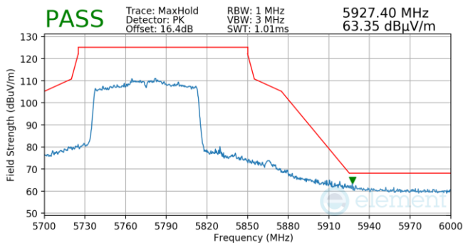
Plot 7-835. Antenna 5b (Pk, Ch.155, 802.11ac, MCS4)
