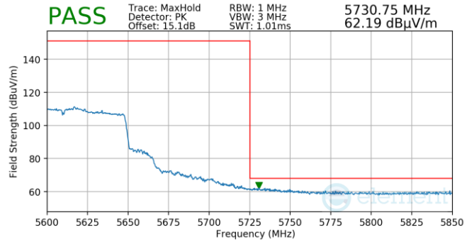
Plot 7-829. (FCC Only) Antenna 5b (Pk, Ch.122, 802.11ac, MCS4)
