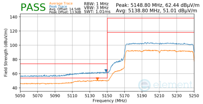
Plot 7-837. Antenna 5b (Pk & Avg, Ch.42, 802.11ax(SU), MCS2)
