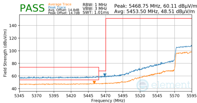
Plot 7-826. (FCC Only) Antenna 5b (Pk & Avg, Ch.122, 802.11ac, MCS4)
