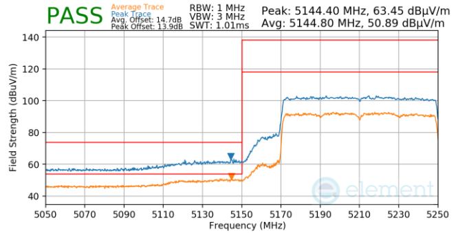
Plot 7-838. Antenna 5b (Pk & Avg, Ch.42, 802.11ax(SU), MCS4)
