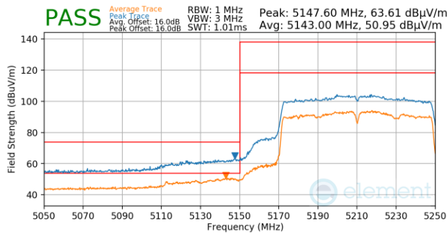
Plot 7-817. Antenna 5b (Pk & Avg, Ch.42, 802.11ac, MCS4)
