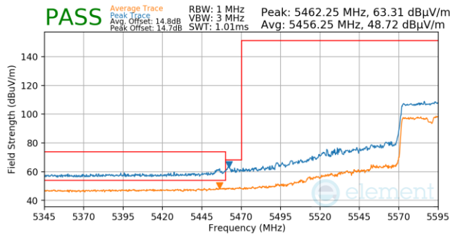
Plot 7-827. (FCC Only) Antenna 5b (Pk & Avg, Ch.122, 802.11ac, MCS9)
