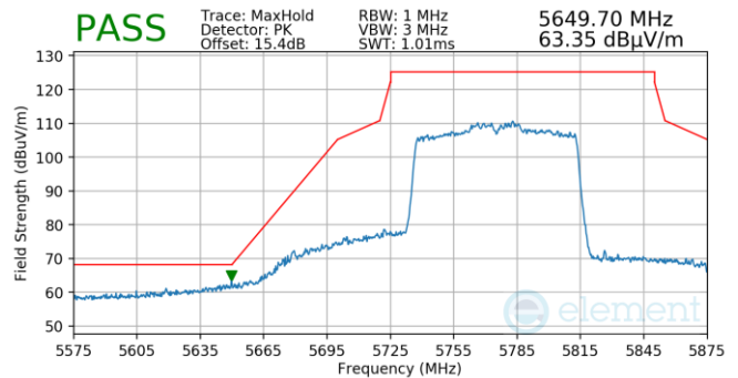
Plot 7-831. Antenna 5b (Pk, Ch.155, 802.11ac, MCS2)
