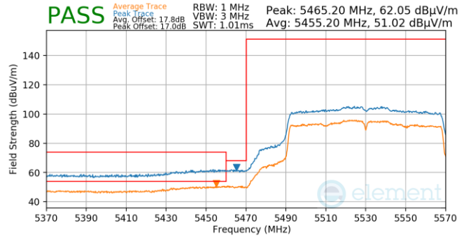
Plot 7-822. Antenna 5b (Pk & Avg, Ch.106, 802.11ac, MCS2)
