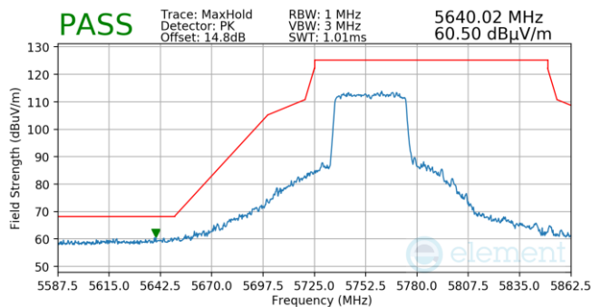
Plot 7-811. Antenna 5b (Pk, Ch.151, 802.11ax(SU), MCS4)
