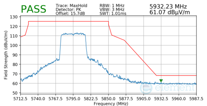
Plot 7-815. Antenna 5b (Pk, Ch.159, 802.11ax(SU), MCS11)
