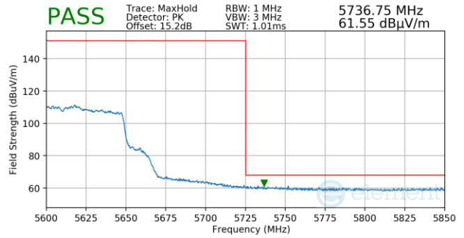
Plot 7-828. (FCC Only) Antenna 5b (Pk, Ch.122, 802.11ac, MCS2)
