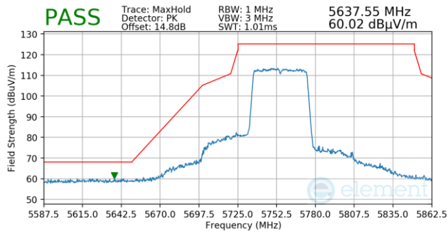
Plot 7-810. Antenna 5b (Pk, Ch.151, 802.11ax(SU), MCS2)
