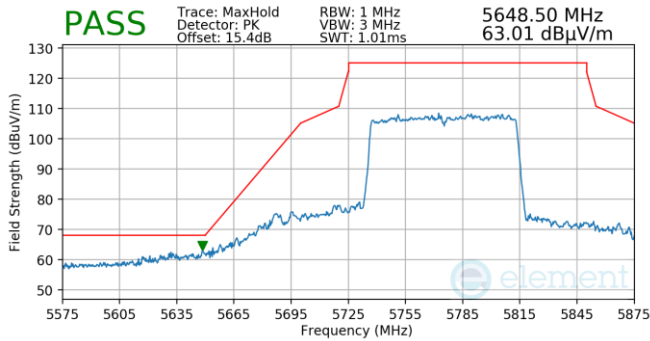
Plot 7-833. Antenna 5b (Pk, Ch.155, 802.11ac, MCS9)
