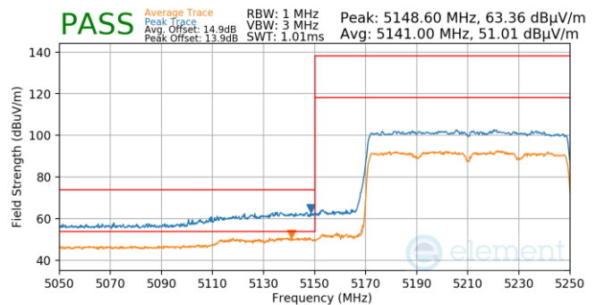
Plot 7-839. Antenna 5b (Pk & Avg, Ch.42, 802.11ax(SU), MCS11)
