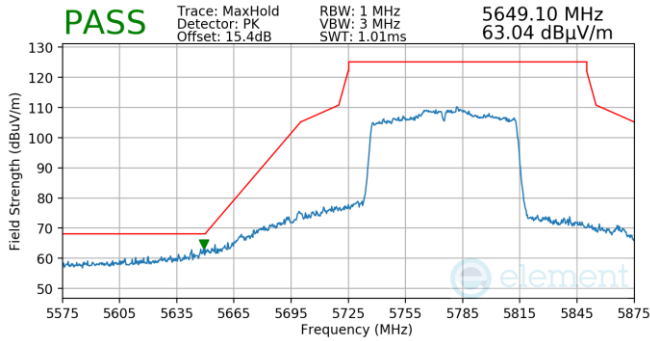
Plot 7-832. Antenna 5b (Pk, Ch.155, 802.11ac, MCS4)
