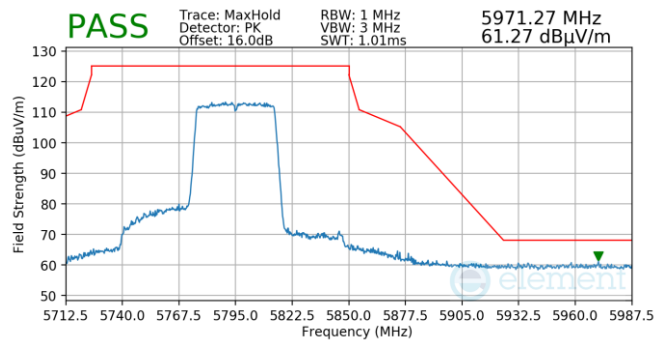
Plot 7-813. Antenna 5b (Pk, Ch.159, 802.11ax(SU), MCS2)
