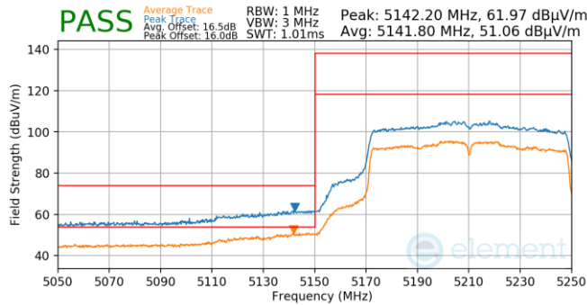
Plot 7-816. Antenna 5b (Pk & Avg, Ch.42, 802.11ac, MCS2)
