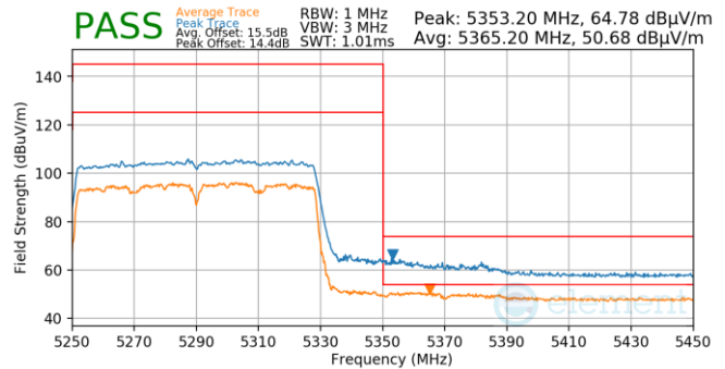
Plot 7-821. Antenna 5b (Pk & Avg, Ch.58, 802.11ac, MCS9)
