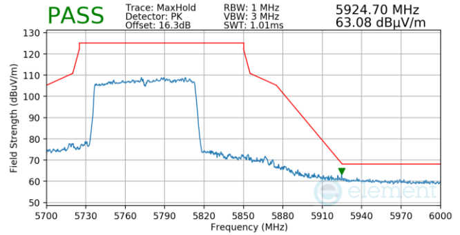
Plot 7-836. Antenna 5b (Pk, Ch.155, 802.11ac, MCS9)
