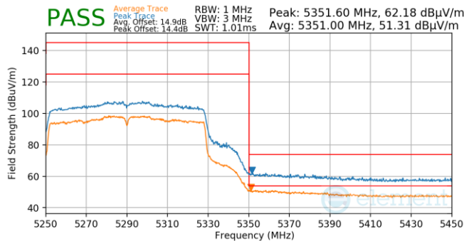
Plot 7-819. Antenna 5b (Pk & Avg, Ch.58, 802.11ac, MCS2)
