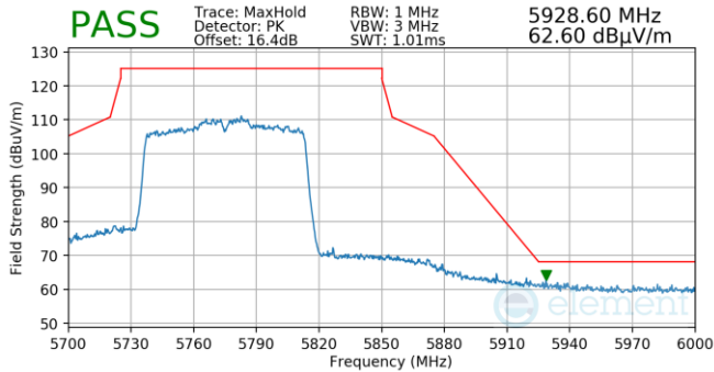
Plot 7-834. Antenna 5b (Pk, Ch.155, 802.11ac, MCS2)
