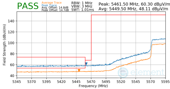
Plot 7-825. (FCC Only) Antenna 5b (Pk & Avg, Ch.122, 802.11ac, MCS2)
