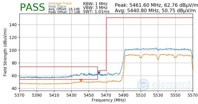
Plot 7-824. Antenna 5b (Pk & Avg, Ch.106, 802.11ac, MCS9)
