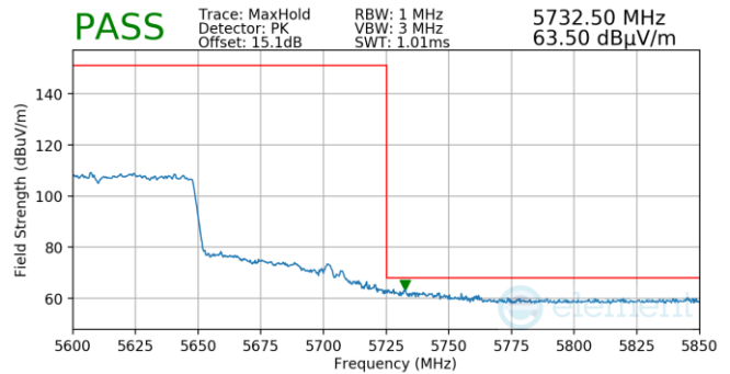
Plot 7-830. (FCC Only) Antenna 5b (Pk, Ch.122, 802.11ac, MCS9)
