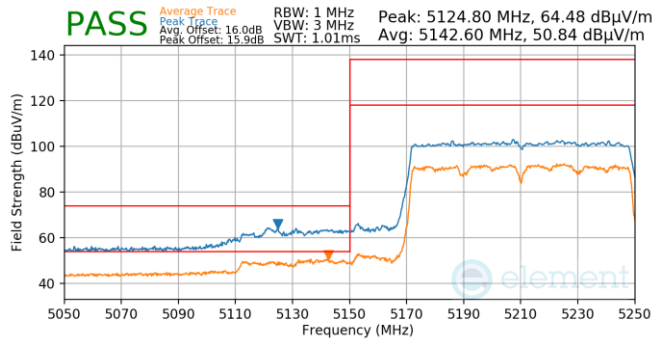
Plot 7-818. Antenna 5b (Pk & Avg, Ch.42, 802.11ac, MCS9)
