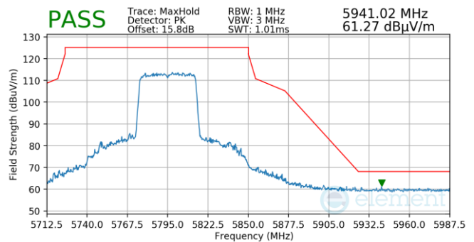
Plot 7-814. Antenna 5b (Pk, Ch.159, 802.11ax(SU), MCS4)
