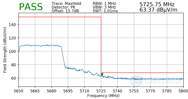
Plot 7-809. Antenna 5b (Pk, Ch.134, 802.11ax(SU), MCS11)
