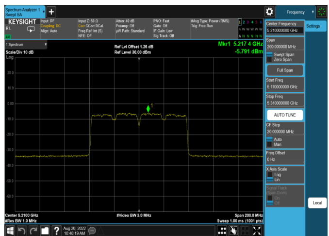
Plot 7-594. ISED PSD CDD Antenna 4a (80MHz BW 11ac - Ch.42, MCS9)
