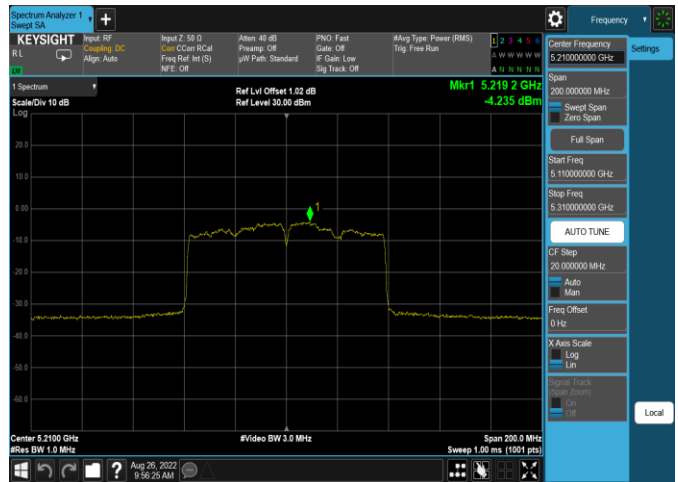
Plot 7-578. ISSED PSD Antenna 4a (80MHz BW 11ac – Ch.42, MCS4)
