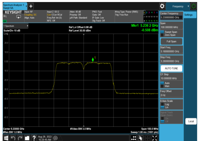
Plot 7-589. ISED PSD SDM Antenna 5b (40MHz BW 11n - Ch.46, MCS15)
