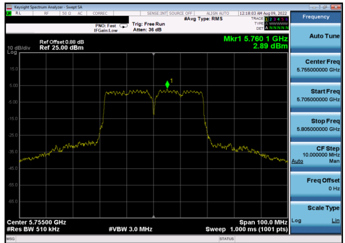
Plot 7-546. PSD CDD Antenna 4a (40MHz BW 802.11n - Ch. 151, MCS15)
