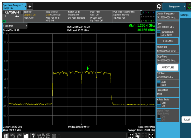
Plot 7-599. ISED PSD CDD Antenna 5b (160MHz BW 11ax (SU) – Ch.50, MCS11)
