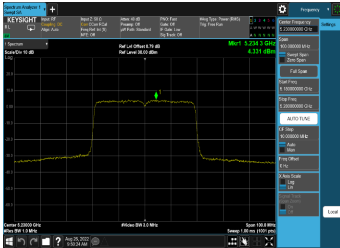
Plot 7-575. ISSED PSD SDM Antenna 5b (40MHz BW 11ax(SU) – Ch.46, MCS4)
