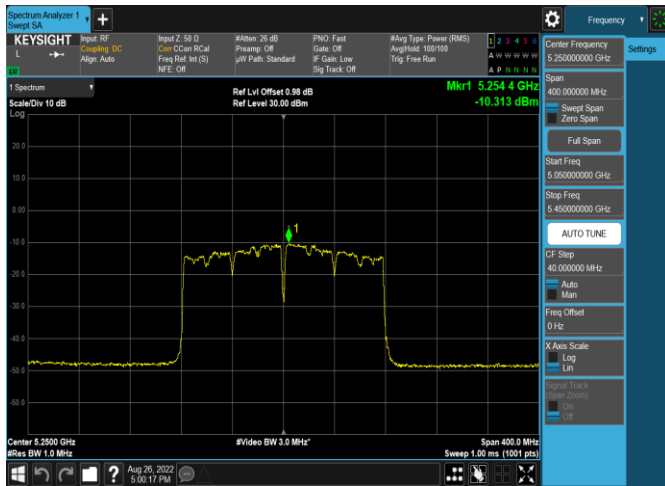
Plot 7-566. ISSED PSD CDD Antenna 4a (160MHz BW 11ac – Ch.50, MCS2)
