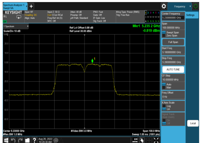
Plot 7-590. ISED PSD SDM Antenna 4a (40MHz BW 11n - Ch.46, MCS15)
