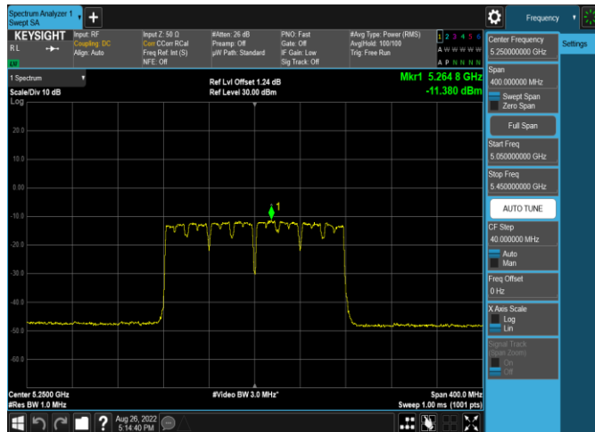
Plot 7-597. ISED PSD CDD Antenna 5b (160MHz BW 11ac – Ch.50, MCS9)
