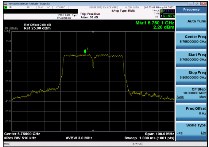
Plot 7-545. PSD CDD Antenna 5b (40MHz BW 802.11n - Ch. 151, MCS15)
