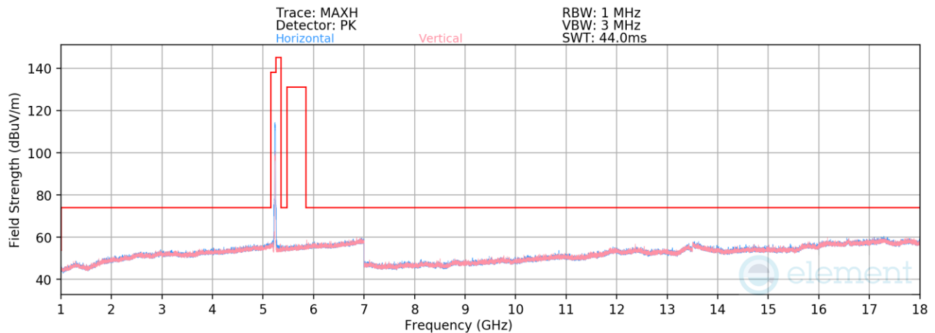
Plot 7-603. Radiated Spurious Emissions above 1GHz Antenna 5b (802.11n – Ch. 48)
