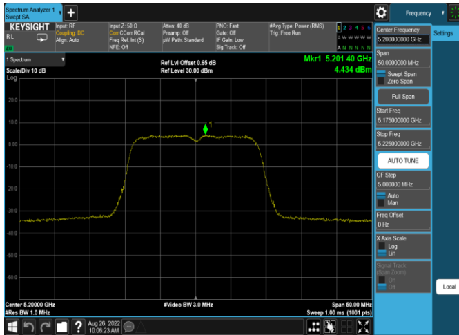
Plot 7-586. ISED PSD SDM Antenna 4a (20MHz BW 11n - Ch.40, MCS15)
