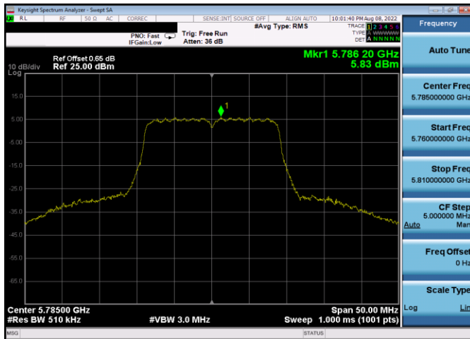
Plot 7-542. PSD CDD Antenna 4a (20MHz BW 802.11n - Ch. 157, MCS15)
