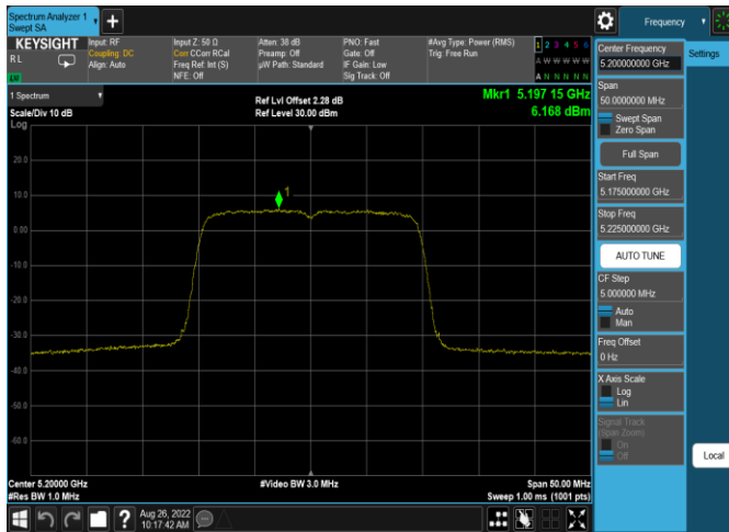
Plot 7-587. ISED PSD SDM Antenna 5b (20MHz BW 11ax(SU) - Ch.40, MCS11)
