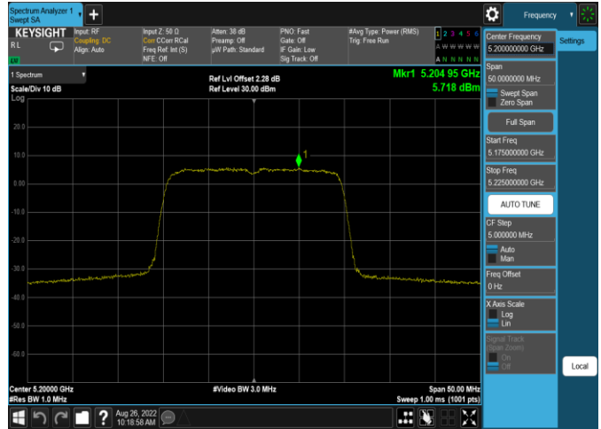
Plot 7-588. ISED PSD SDM Antenna 4a (20MHz BW 11ax(SU) - Ch.40, MCS11)
