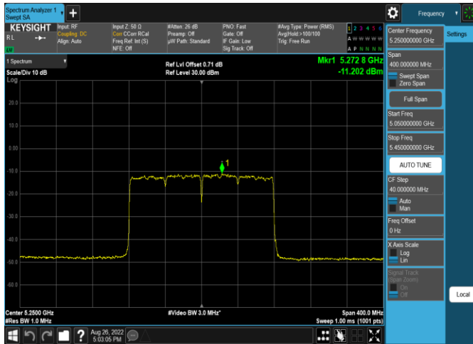
Plot 7-567. ISSED PSD CDD Antenna 5b (160MHz BW 11ax (SU) – Ch.50, MCS2)
