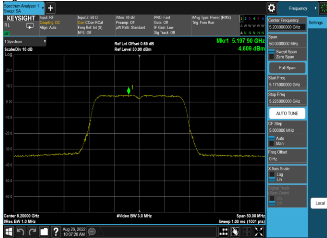
Plot 7-585. ISED PSD SDM Antenna 5b (20MHz BW 11n - Ch.40, MCS15)
