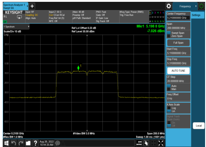
Plot 7-596. ISED PSD CDD Antenna 5b (80MHz BW 11ax(SU) - Ch.42, MCS11)
