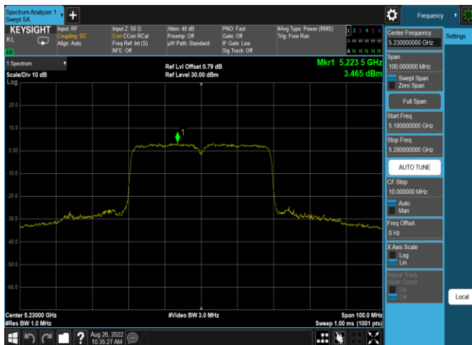
Plot 7-592. ISED PSD SDM Antenna 4a (40MHz BW 11ax(SU) - Ch.46, MCS11)
