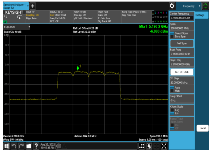
Plot 7-595. ISED PSD CDD Antenna 5b (80MHz BW 11ax(SU) - Ch.42, MCS11)
