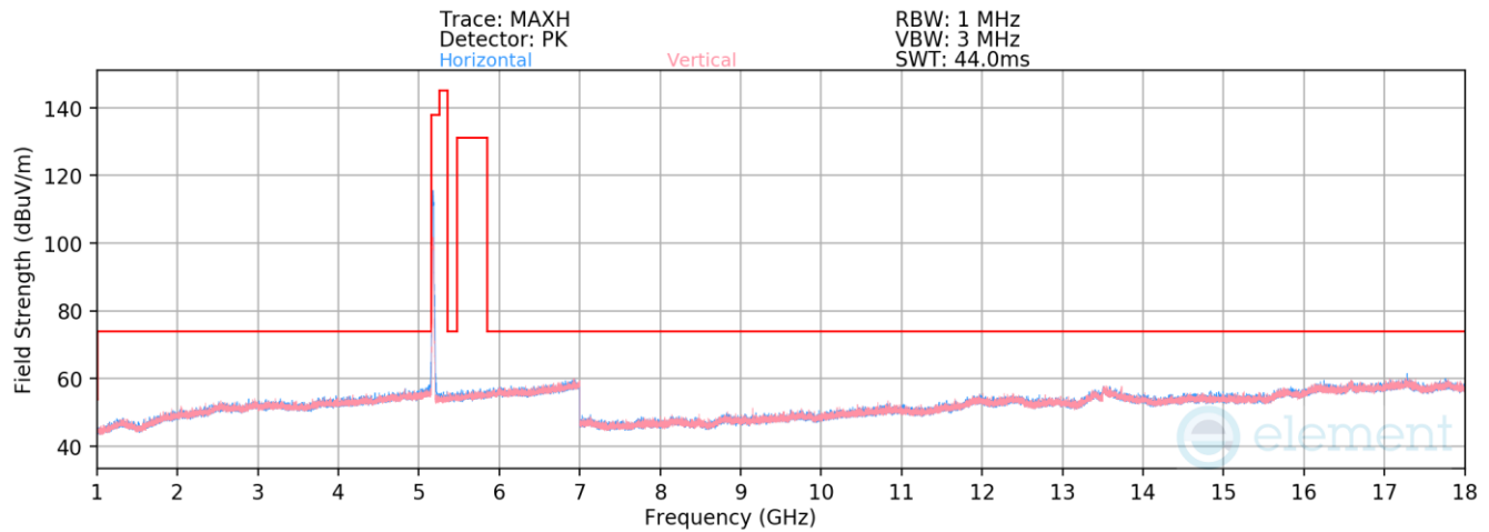
Plot 7-601. Radiated Spurious Emissions above 1GHz Antenna 5b (802.11n – Ch. 36)
