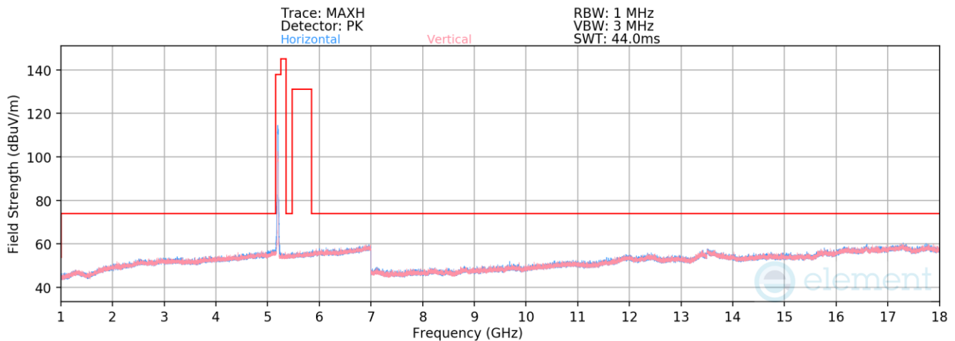
Plot 7-602. Radiated Spurious Emissions above 1GHz Antenna 5b (802.11n – Ch. 40)
