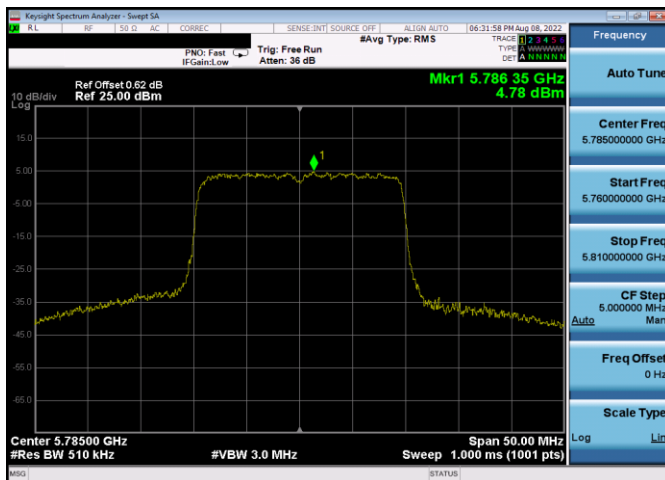
Plot 7-543. PSD CDD Antenna 5b (20MHz BW 802.11ax(SU) - Ch. 157, MCS11)
