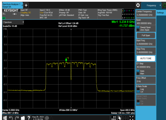
Plot 7-598. ISED PSD CDD Antenna 4a (160MHz BW 11ac – Ch.50, MCS9)
