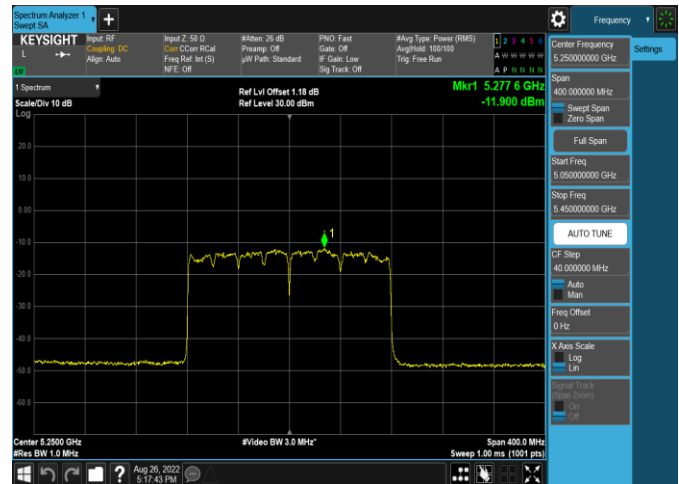
Plot 7-600. ISED PSD CDD Antenna 4a (160MHz BW 11ax (SU) – Ch.50, MCS11)
