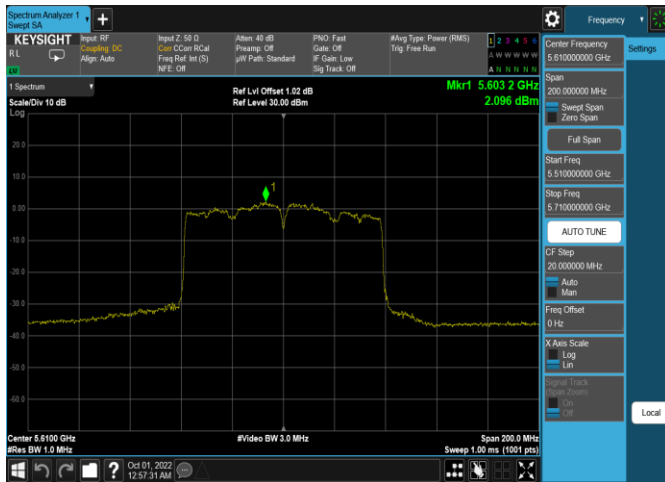
Plot 7-465. PSD CDD Antenna 5b (80MHz BW 802.11ac – Ch. 122, MCS4 (FCC))
