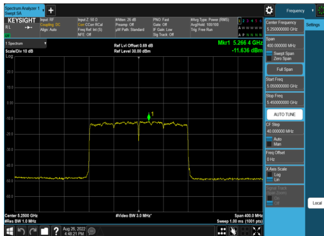
Plot 7-368. ISED PSD Antenna 4a (160MHz BW 11ax(SU) – Ch.50 MCS2)
