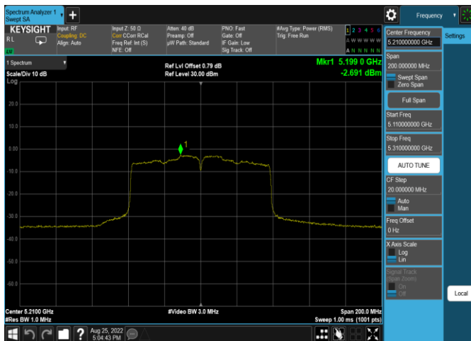
Plot 7-393. PSD CDD Antenna 5b (80MHz BW 802.11ac – Ch. 42, MCS2)
