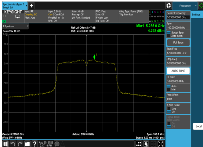
Plot 7-371. ISED PSD Antenna 4a (40MHz BW 11n – Ch.46, MCS4)
