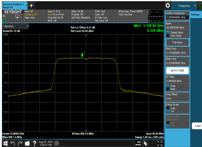
Plot 7-370. ISED PSD Antenna 4a (20MHz BW 11ax(SU) – Ch.40, MCS4)
