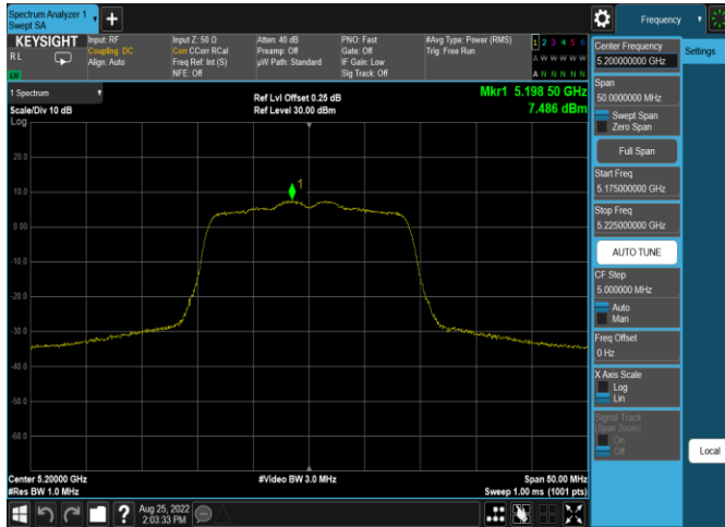
Plot 7-369. ISED PSD Antenna 4a (20MHz BW 11n – Ch.40, MCS4)
