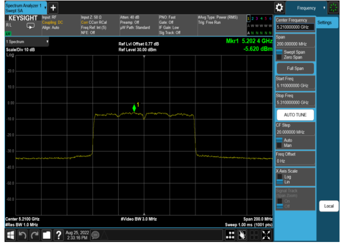
Plot 7-374. ISED PSD Antenna 4a (80MHz BW 11ax (SU) – Ch.42, MCS4)
