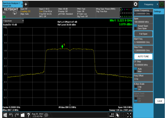
Plot 7-372. ISED PSD Antenna 4a (40MHz BW 11ax(SU) – Ch.46, MCS4)
