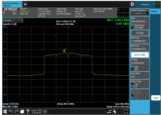
Plot 7-373. ISED PSD Antenna 4a (80MHz BW 11ac – Ch.42, MCS4)
