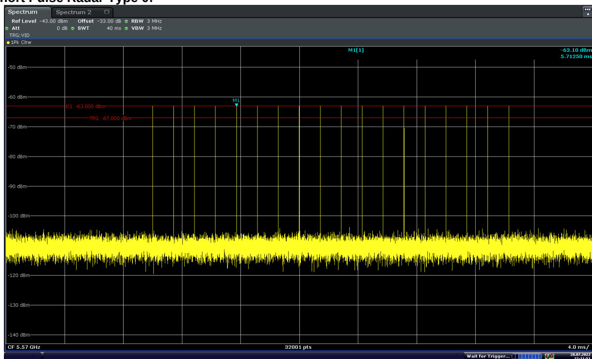
Figure 7-4. 5570MHz – Radar Pulse Type 0 (160MHz)
