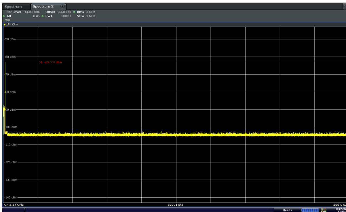
Figure 9-17. 5570MHz - Non-Occupancy Period (30 Minutes) - Mode 1 (160MHz)
