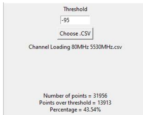
Figure 9-6. 5530MHz - Channel Loading Calculation - Mode 2 (80MHz)
