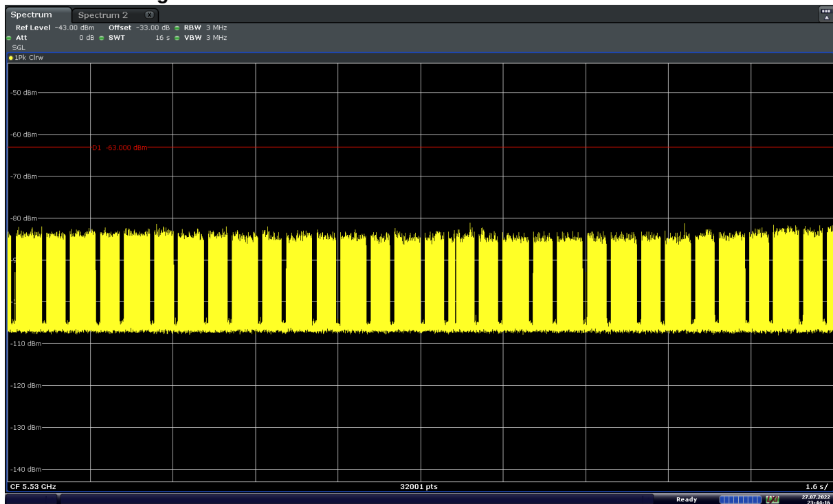
Figure 9-5. 5530MHz - Channel Loading - Mode 2 (80MHz)
