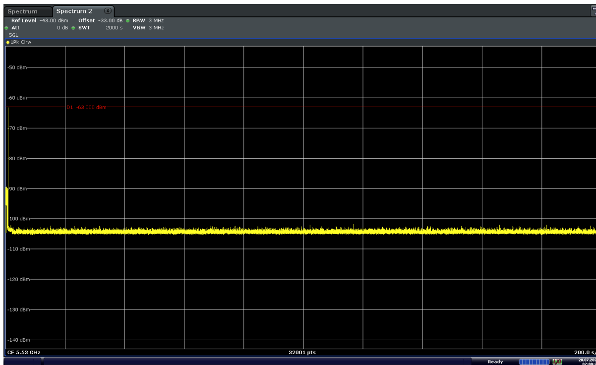
Figure 9-19. 5530MHz - Non-Occupancy Period (30 Minutes) - Mode 3 (80MHz)
