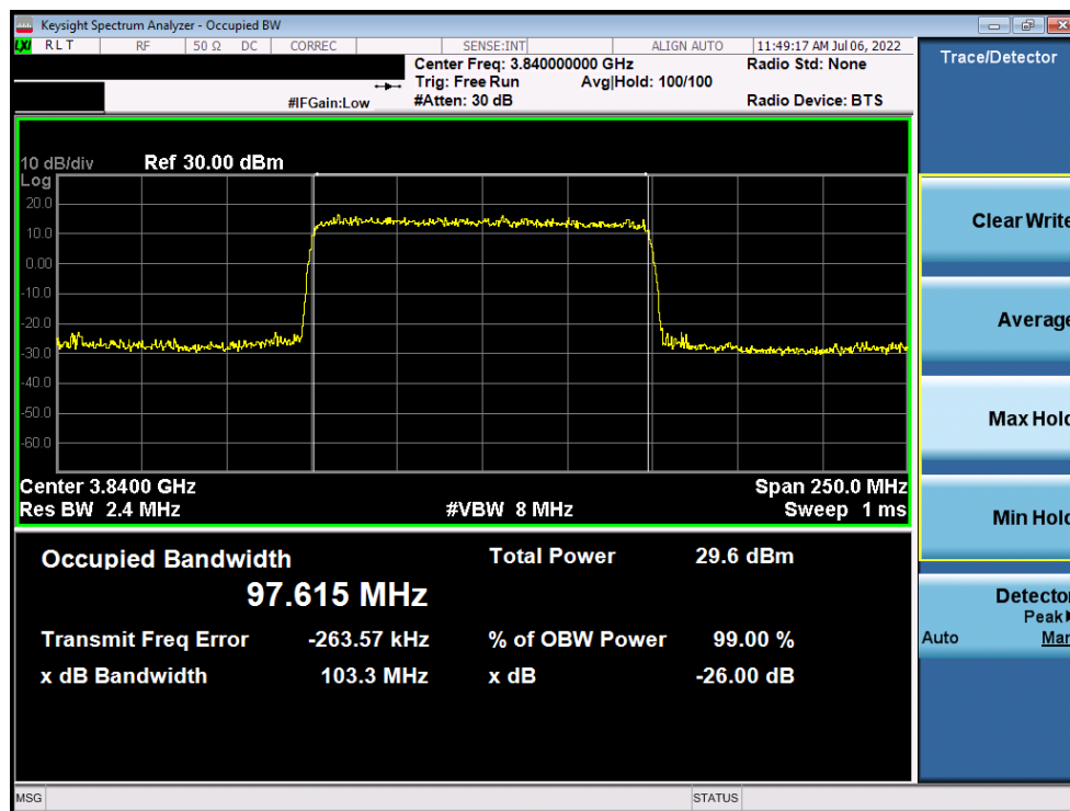
Plot 7-110. Occupied Bandwidth Plot (NR Band n77 C-Band - 100MHz CP-OFDM 256-QAM - Full RB)
