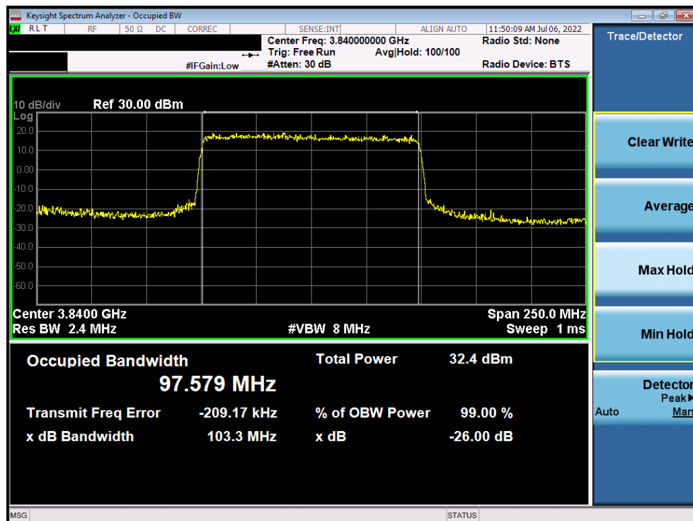
Plot 7-109. Occupied Bandwidth Plot (NR Band n77 C-Band - 100MHz CP-OFDM 64-QAM - Full RB)
