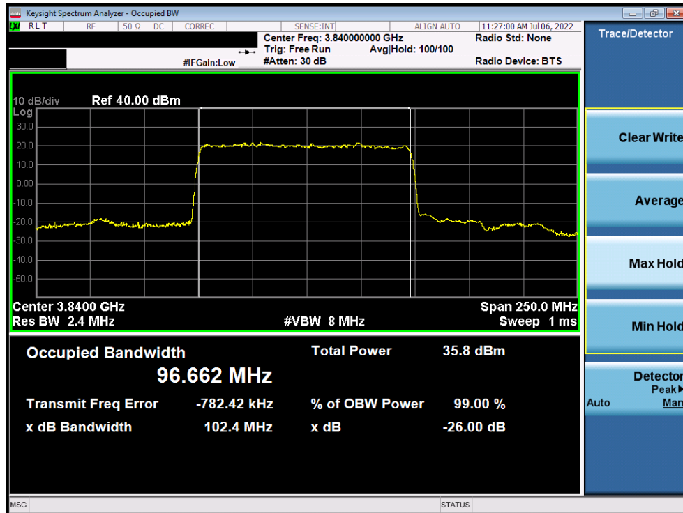
Plot 7-106. Occupied Bandwidth Plot (NR Band n77 C-Band - 100MHz DFT-s-OFDM \pi/2 BPSK - Full RB)
