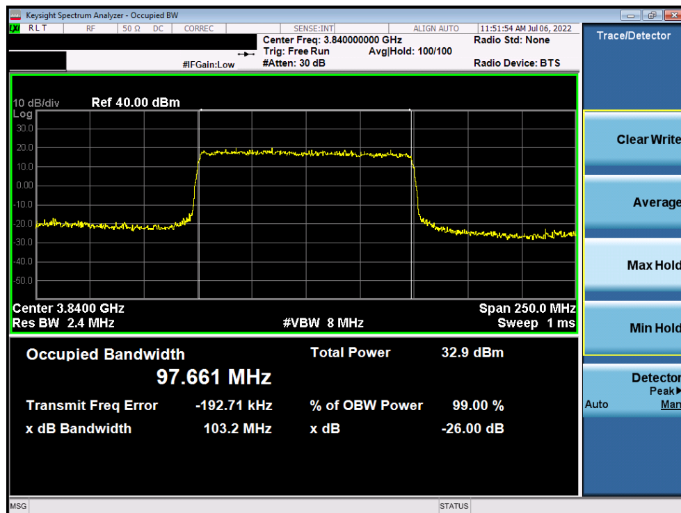
Plot 7-107. Occupied Bandwidth Plot (NR Band n77 C-Band - 100MHz CP-OFDM QPSK - Full RB)
