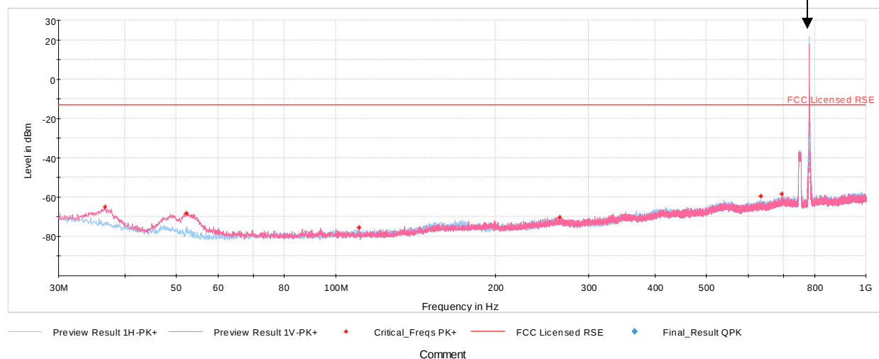
Plot 7-453. Antenna 3 Radiated Spurious Emission below 1GHz (LTE Band 13)
