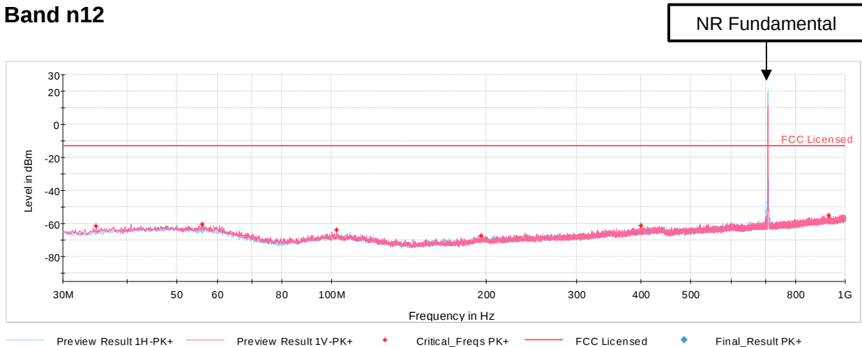
Plot 7-457. Antenna 4b Radiated Spurious Emission below 1GHz (NR Band n12)
