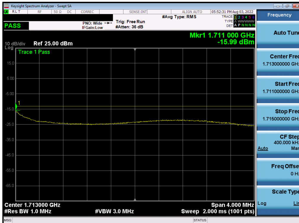
Plot 7-328. Upper Extended Band Edge Plot (NR Band n70 – 10.0MHz DFT-s-OFDM \pi/2 BPSK - Full RB)
