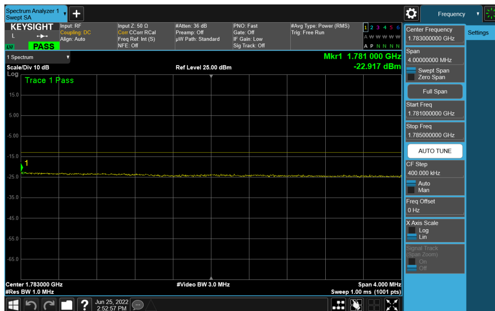
Plot 7-316. Upper Extended Band Edge Plot (NR Band n66 – 30.0MHz DFT-s-OFDM QPSK - Full RB)
