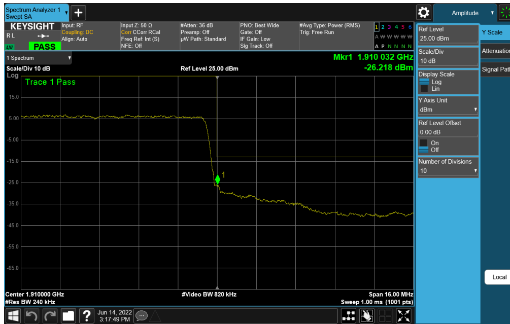
Plot 7-178. Upper Band Edge Plot (NR Band n2 – 20MHz DFT-s-OFDM \pi/2 BPSK – Full RB Configuration)
