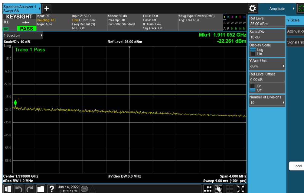
Plot 7-179. Extended Upper Band Edge Plot (NR Band n2 – 20MHz CP-OFDM \pi/2 QPSK – Full RB Configuration)
