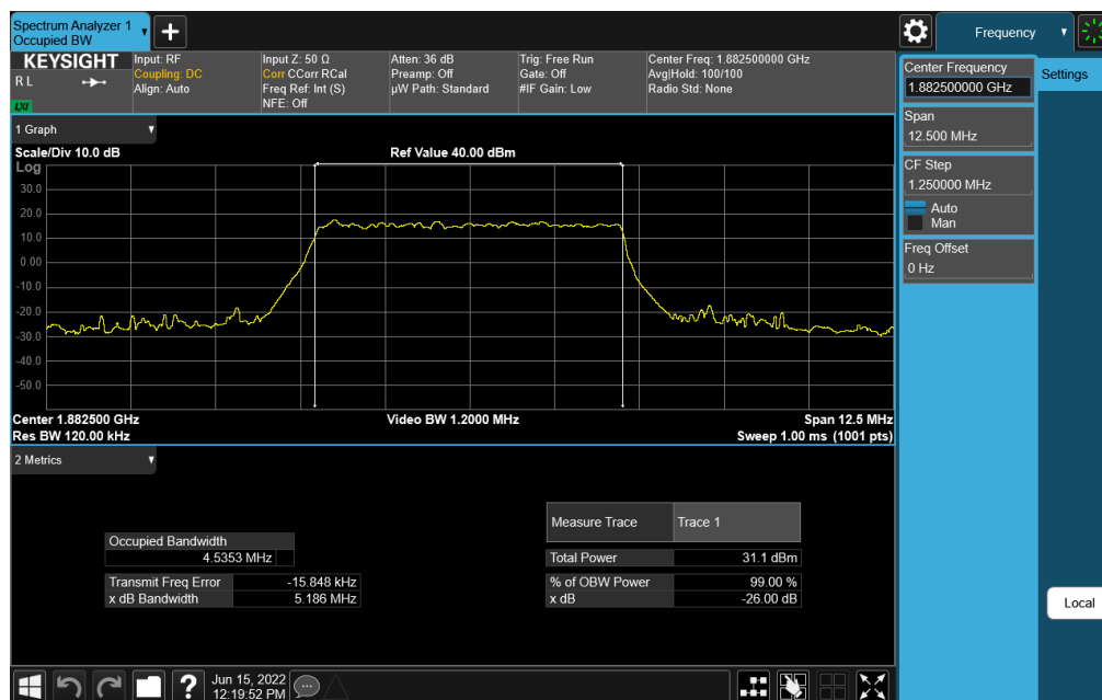
Plot 7-28. Occupied Bandwidth Plot (NR Band n25/n2 - 5.0MHz DFT-s-OFDM 64QAM - Full RB)
