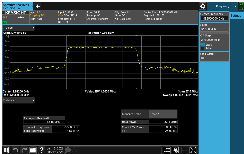
Plot 7-35. Occupied Bandwidth Plot (NR Band n25/n2 - 15.0MHz DFT-s-OFDM \pi/2 BPSK - Full RB)
