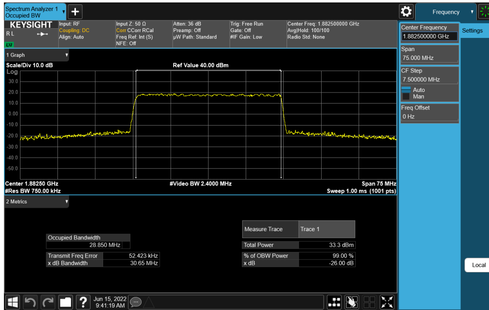
Plot 7-51. Occupied Bandwidth Plot (NR Band n25 - 30.0MHz DFT-s-OFDM QPSK - Full RB)
