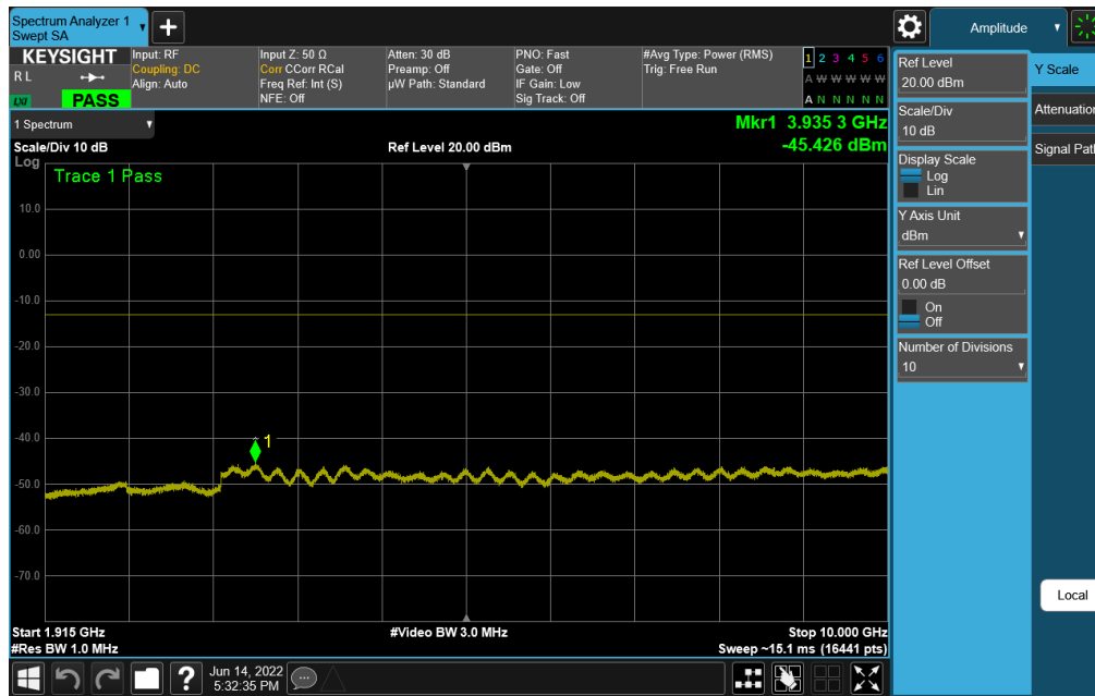
Plot 7-74. Conducted Spurious Plot (NR Band n25/n2 - 40.0MHz - RB Size 1, RB Offset 0 - Mid Channel)
