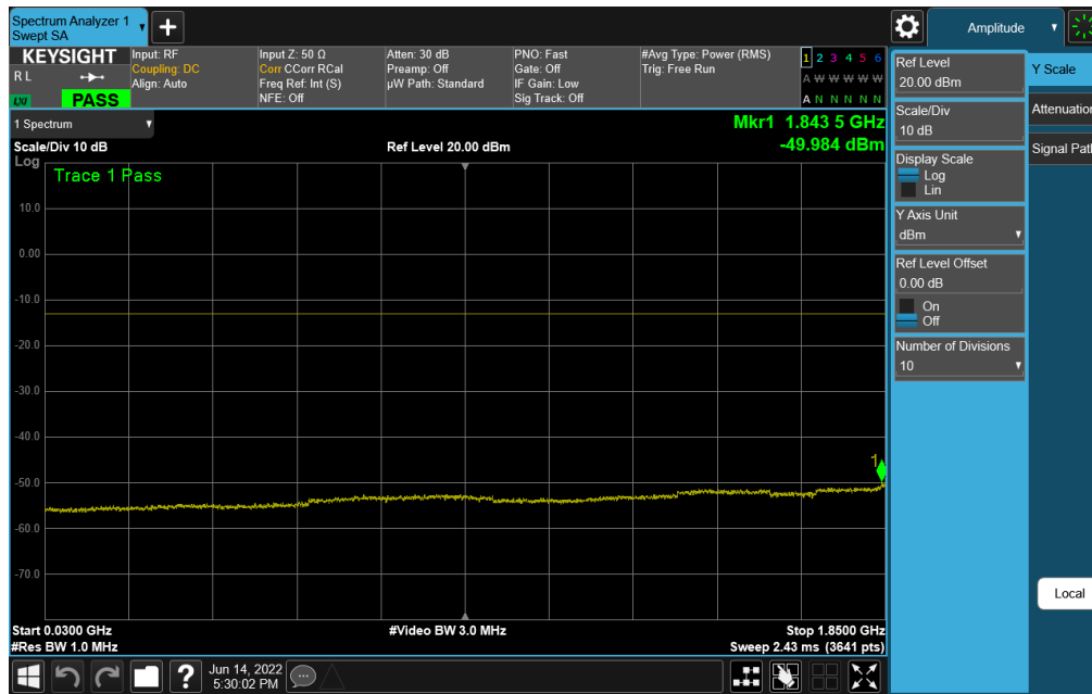
Plot 7-70. Conducted Spurious Plot (NR Band n25/n2 - 40.0MHz - RB Size 1, RB Offset 0 - Low Channel)
