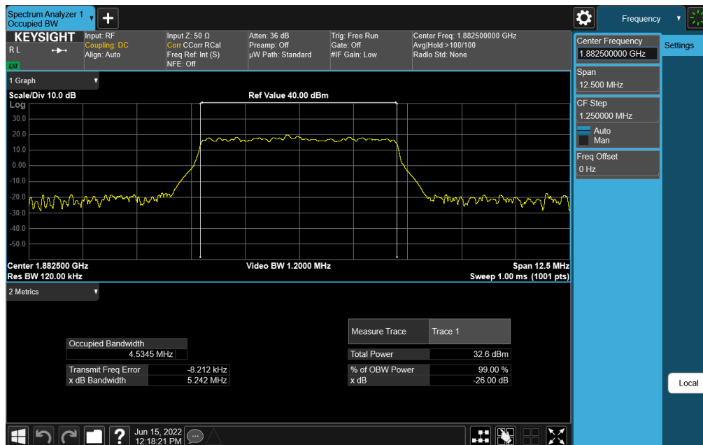
Plot 7-26. Occupied Bandwidth Plot (NR Band n25/n2 - 5.0MHz DFT-s-OFDM QPSK - Full RB)
