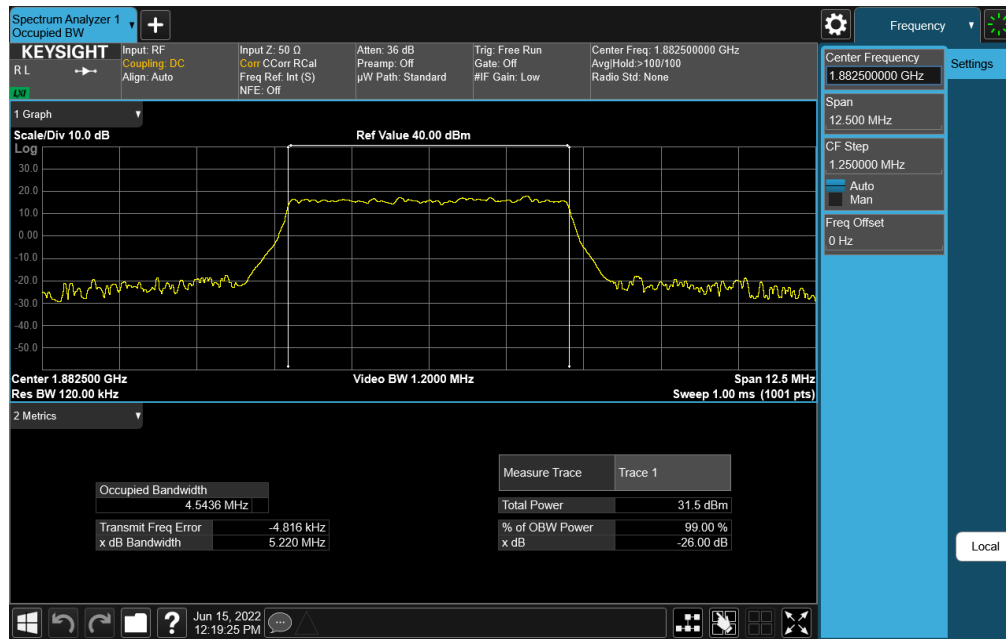
Plot 7-27. Occupied Bandwidth Plot (NR Band n25/n2 - 5.0MHz DFT-s-OFDM 16QAM - Full RB)
