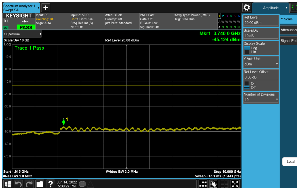
Plot 7-71. Conducted Spurious Plot (NR Band n25/n2 - 40.0MHz - RB Size 1, RB Offset 0 - Low Channel)
