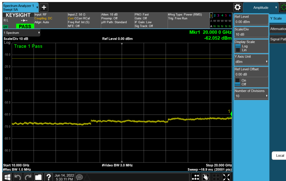
Plot 7-75. Conducted Spurious Plot (NR Band n25/n2 - 40.0MHz - RB Size 1, RB Offset 0 - Mid Channel)
