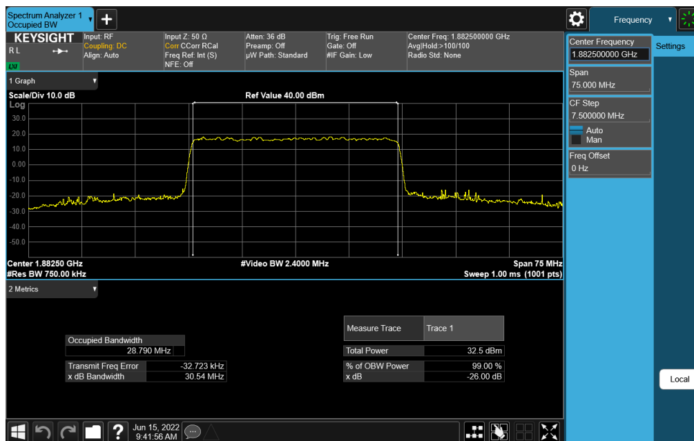
Plot 7-52. Occupied Bandwidth Plot (NR Band n25 - 30.0MHz DFT-s-OFDM 16QAM - Full RB)
