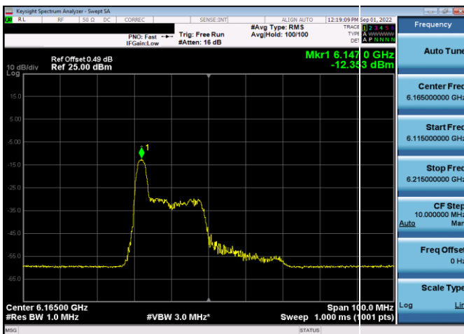
Plot 7-265. Power Spectral Density Plot SDM Antenna 5b (40MHz 802.11ax RU26 (UNII Band 5) – Ch. 43)
