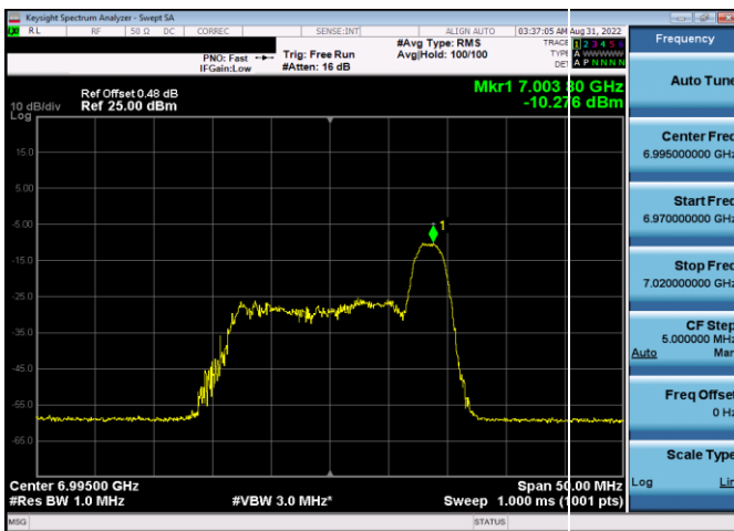
Plot 7-243. Power Spectral Density Plot Antenna 4a (20MHz 802.11ax RU26 (UNII Band 8) – Ch. 209)
