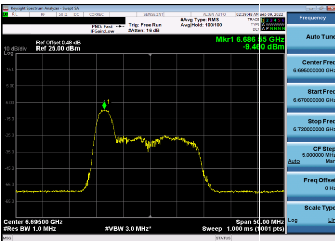
Plot 7-161. Power Spectral Density Plot Antenna 5b (20MHz 802.11ax RU26 (UNII Band 7) – Ch. 149)
