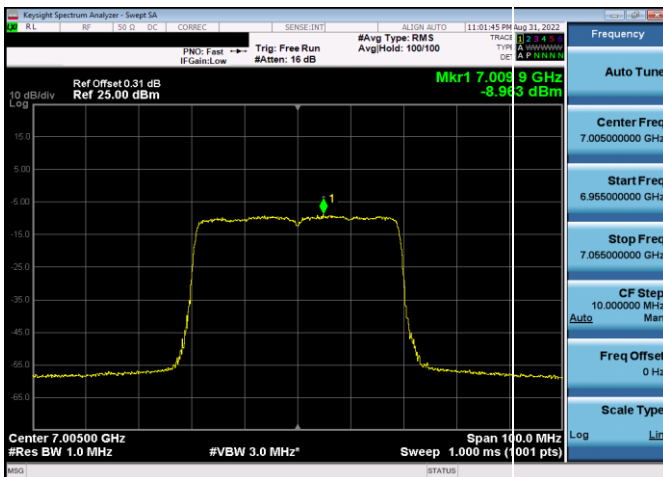
Plot 7-367. Power Spectral Density Plot SDM Antenna 5b (40MHz 802.11ax RU484 (UNII Band 8) – Ch. 211)
