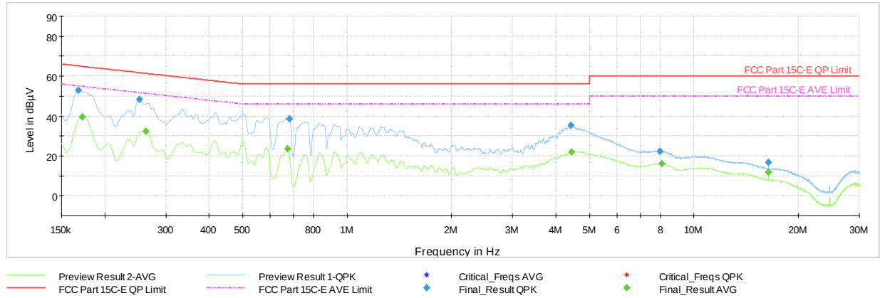
Plot 6-5. AC Line Conducted Plot (L1, Charging Rate 10C, with AC/DC Adapter)
