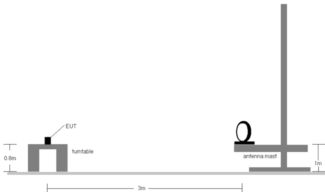
Figure 6-1. Test Setup
