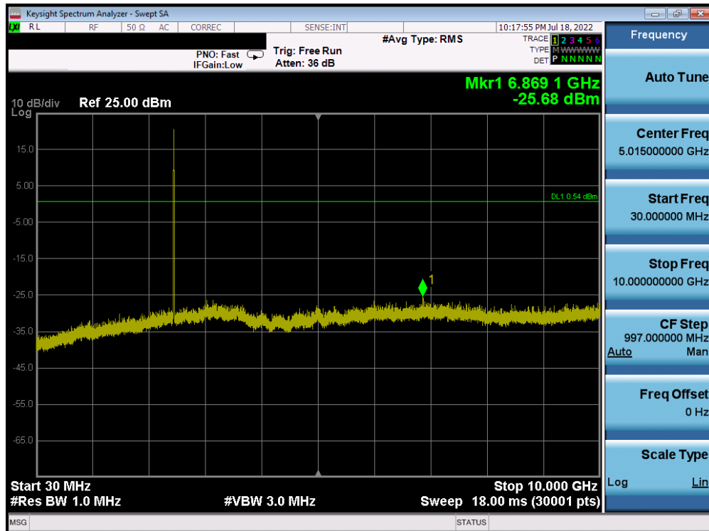
Plot 7-431. Conducted Spurious Plot Antenna 4a (802.11b – Ch. 11)
