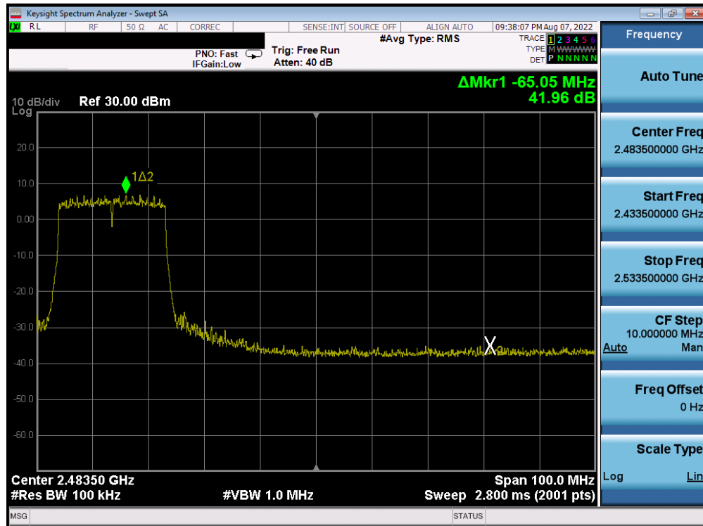
Plot 7-422. Band Edge Plot Antenna 2a (802.11ax (2.4GHz) - Ch. 8) - MCS5
