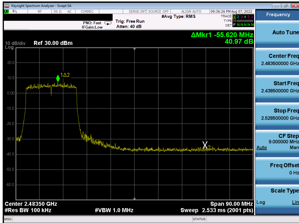
Plot 7-423. Band Edge Plot Antenna 2a (802.11ax (SU - 2.4GHz) - Ch. 9) - MCS5
