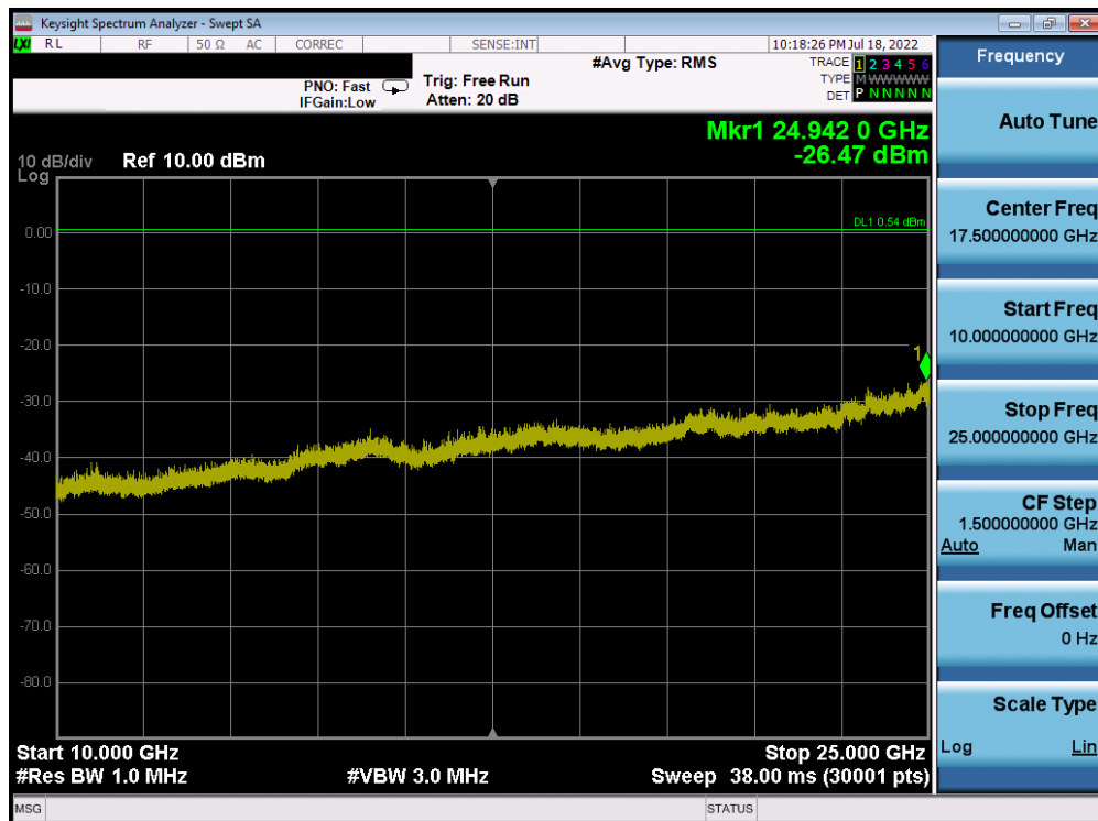
Plot 7-432. Conducted Spurious Plot Antenna 4a (802.11b – Ch. 11)
