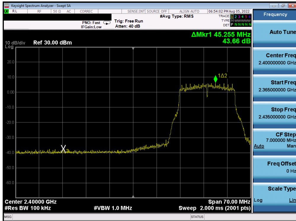
Plot 7-262. Band Edge Plot Antenna 4a (802.11g- Ch. 3) - 36Mbps
