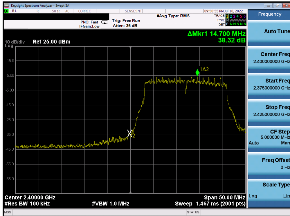
Plot 7-227. Band Edge Plot Antenna 4a (802.11n (2.4GHz) – Ch. 1) – MCS3
