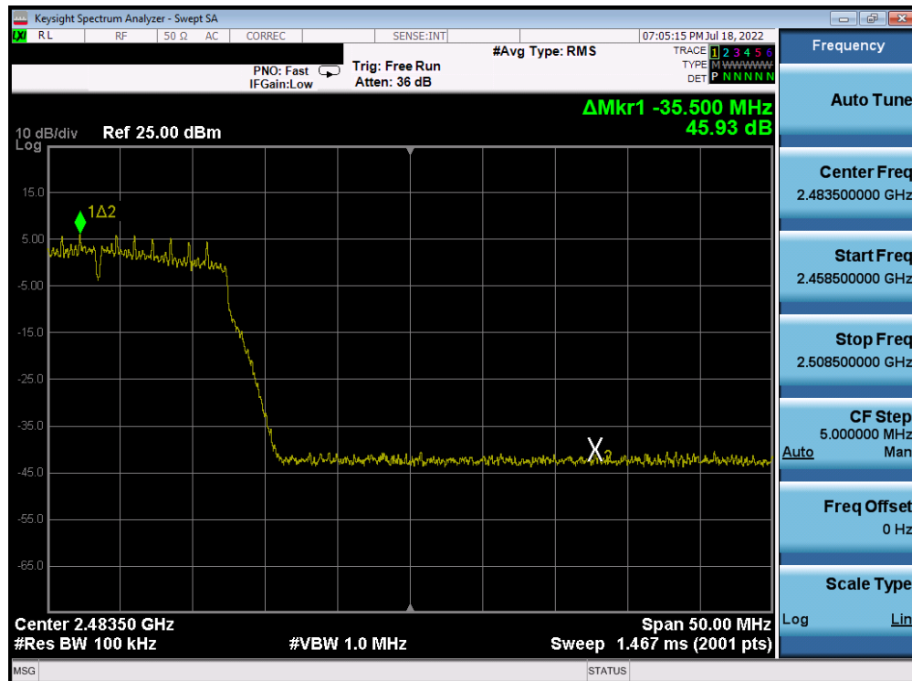
Plot 7-198. Band Edge Plot Antenna 4a (802.11n (2.4GHz) - Ch. 11) - MCS2
