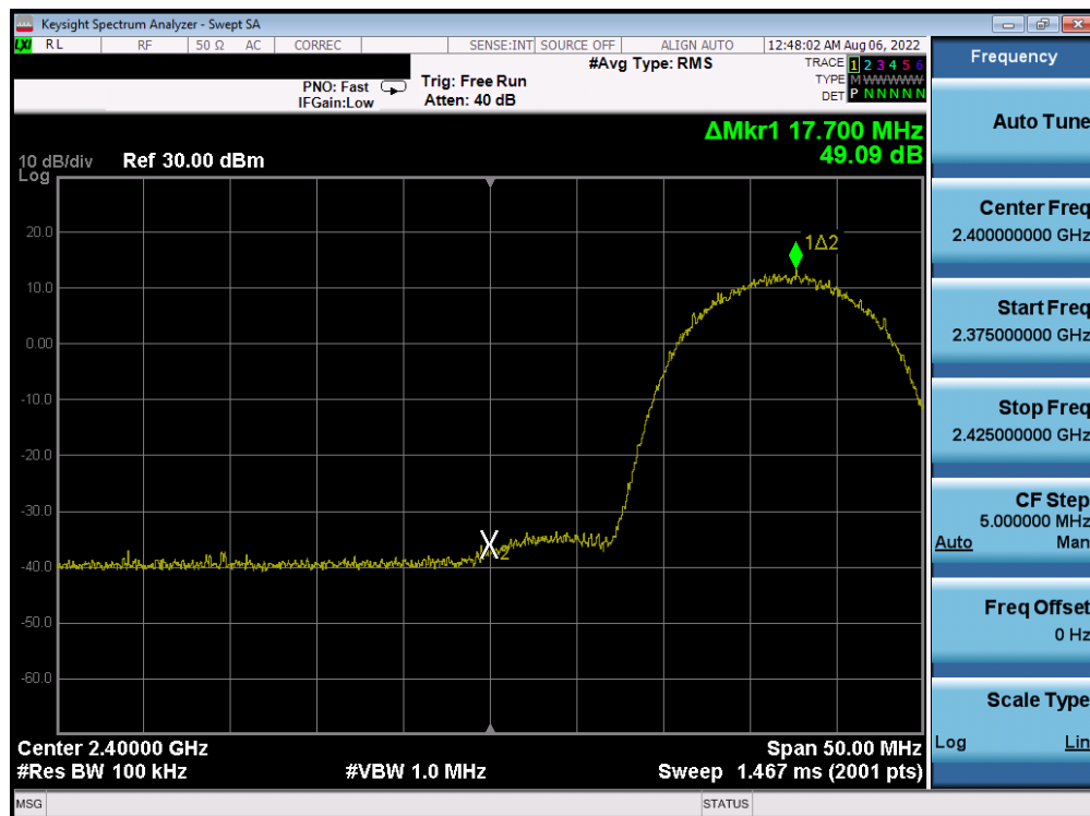
Plot 7-255. Band Edge Plot Antenna 4a (802.11b– Ch. 2) – 11Mbps
