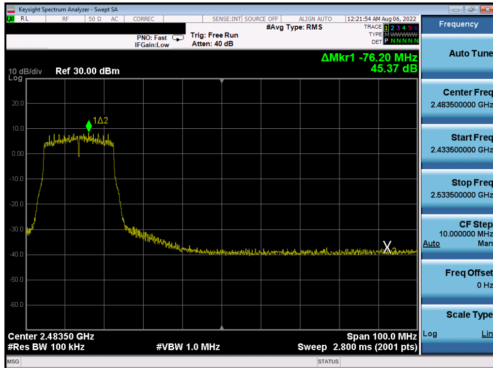
Plot 7-235. Band Edge Plot Antenna 4a (802.11n (2.4GHz) - Ch. 8) - MCS3
