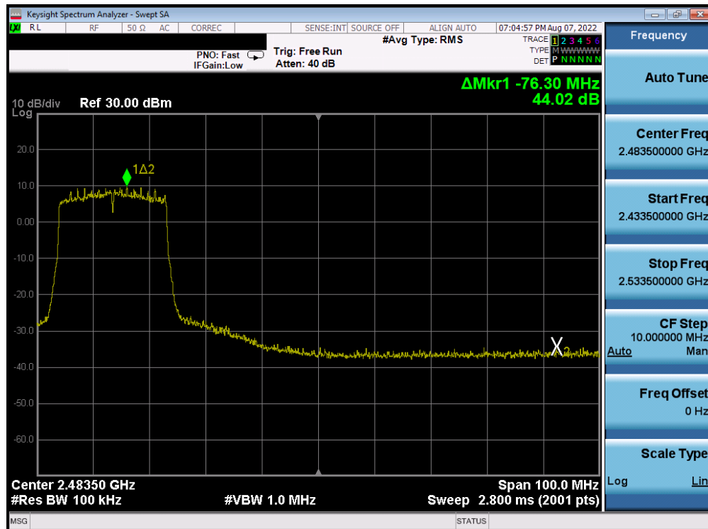
Plot 7-208. Band Edge Plot Antenna 4a (802.11ax (2.4GHz) – Ch. 8) – MCS2
