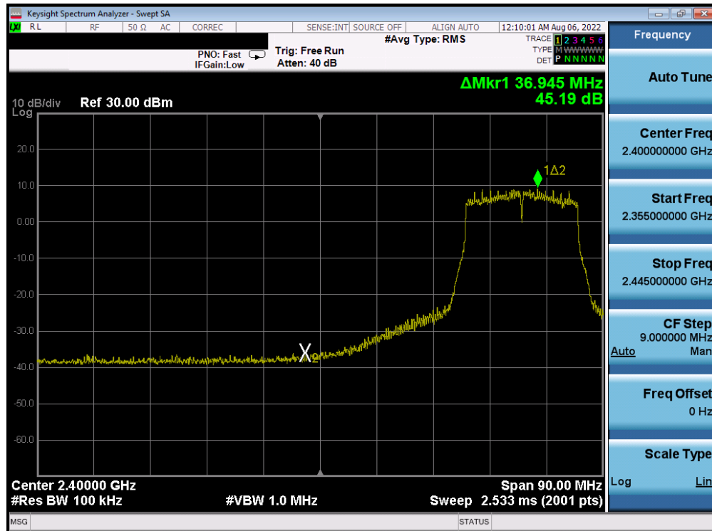
Plot 7-231. Band Edge Plot Antenna 4a (802.11n (2.4GHz) – Ch. 5) – MCS3
