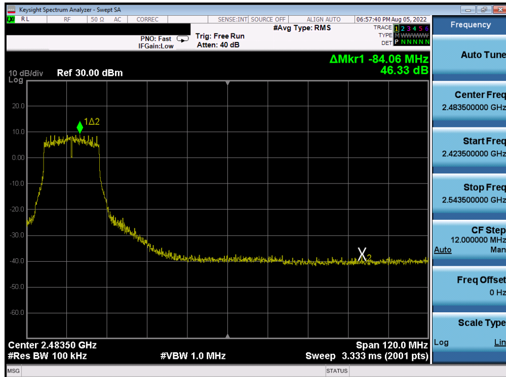
Plot 7-266. Band Edge Plot Antenna 4a (802.11g- Ch. 6 (high)) – 36Mbps
