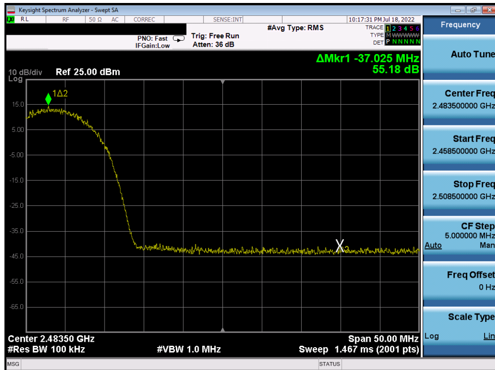
Plot 7-257. Band Edge Plot Antenna 4a (802.11b – Ch. 11) – 11Mbps
