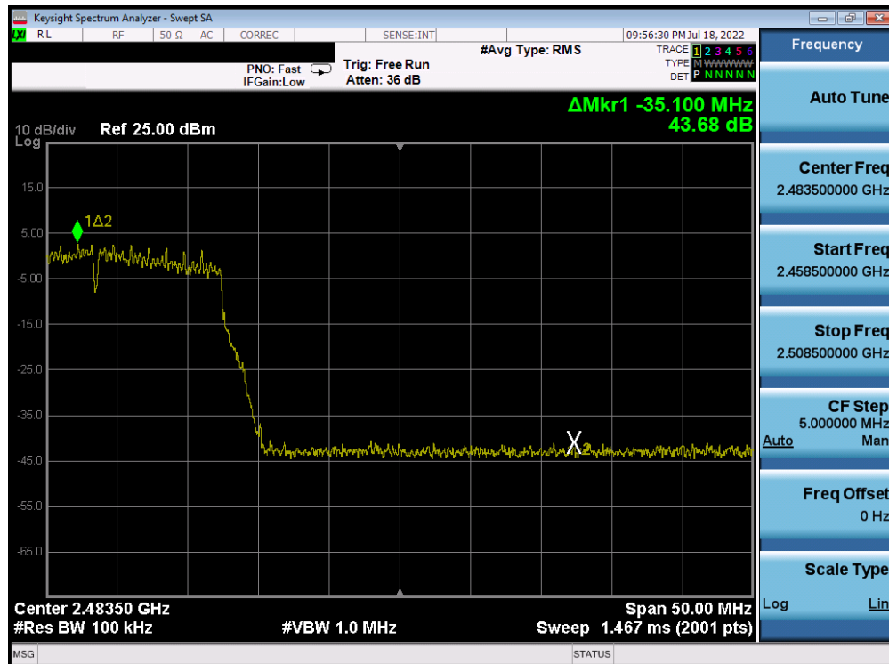
Plot 7-238. Band Edge Plot Antenna 4a (802.11n (2.4GHz) - Ch. 11) - MCS3
