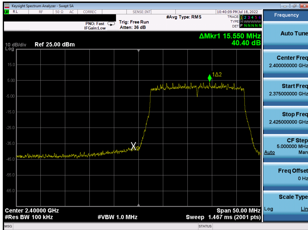
Plot 7-288. Band Edge Plot Antenna 4a (802.11ax (SU - 2.4GHz) - Ch. 1) - MCS5
