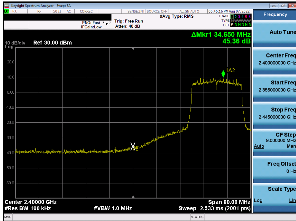
Plot 7-205. Band Edge Plot Antenna 4a (802.11ax (2.4GHz) – Ch. 5) – MCS2
