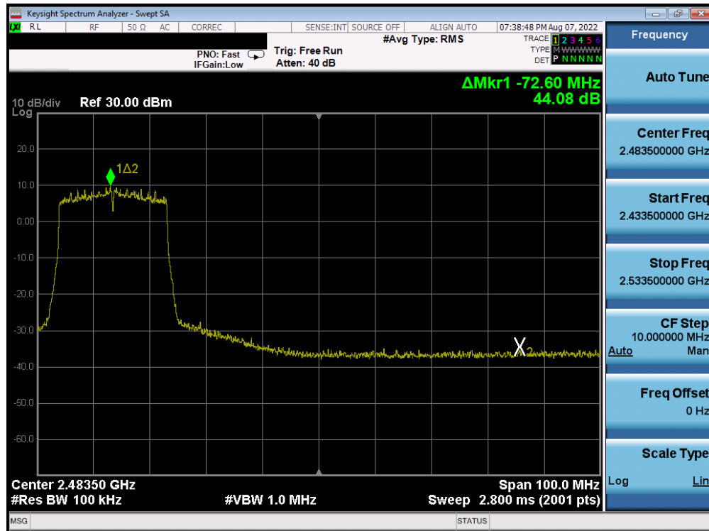
Plot 7-249. Band Edge Plot Antenna 4a (802.11ax (2.4GHz) – Ch. 8) – MCS3
