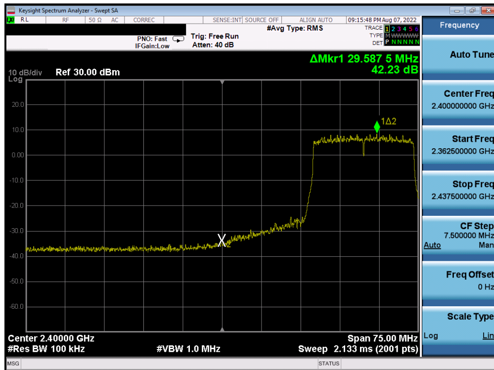
Plot 7-291. Band Edge Plot Antenna 4a (802.11ax (2.4GHz) – Ch. 4) – MCS5
