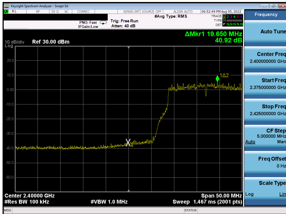
Plot 7-261. Band Edge Plot Antenna 4a (802.11g- Ch. 2) – 36Mbps
