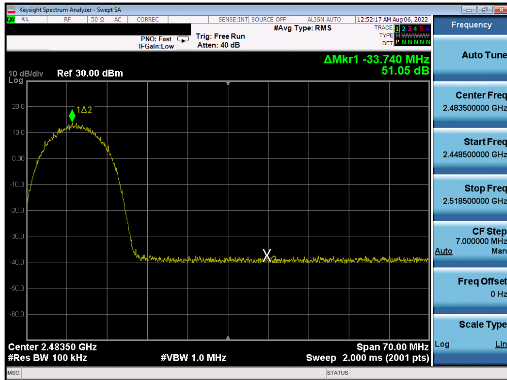
Plot 7-256. Band Edge Plot Antenna 4a (802.11b – Ch. 10) – 11Mbps
