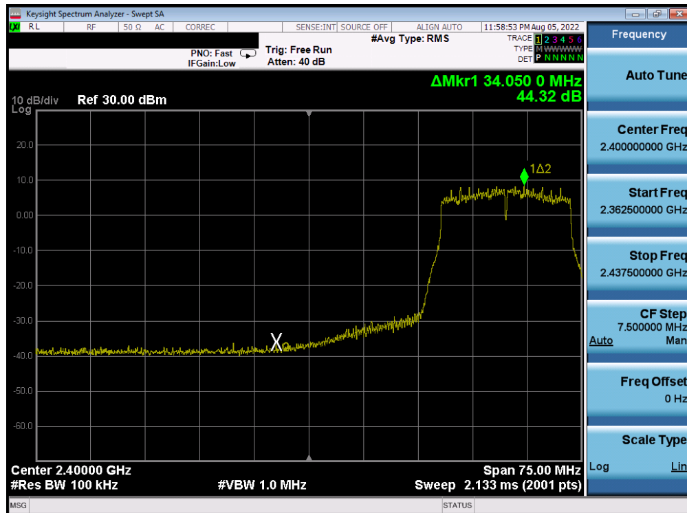
Plot 7-230. Band Edge Plot Antenna 4a (802.11n (2.4GHz) - Ch. 4) - MCS3
