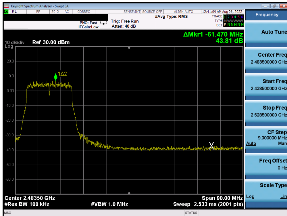
Plot 7-283. Band Edge Plot Antenna 4a (802.11n (2.4GHz) – Ch. 9) – MCS5
