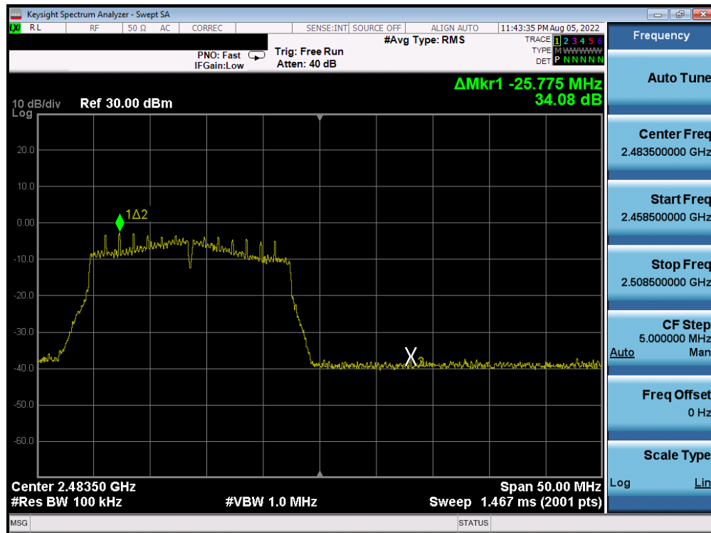
Plot 7-200. Band Edge Plot Antenna 4a (802.11n (2.4GHz) - Ch. 13) - MCS2
