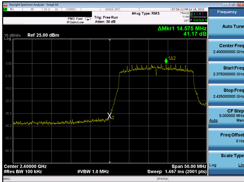
Plot 7-201. Band Edge Plot Antenna 4a (802.11ax (SU - 2.4GHz) – Ch. 1) – MCS2
