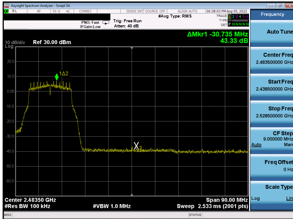
Plot 7-222. Band Edge Plot Antenna 4a (802.11g – Ch. 9) – 18Mbps
