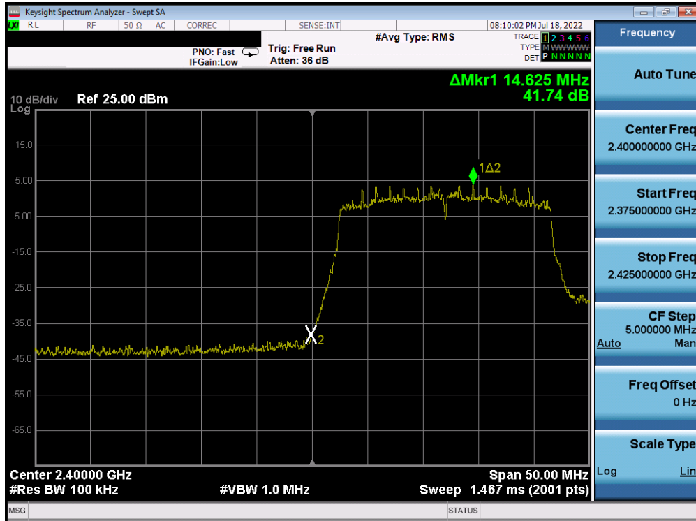
Plot 7-213. Band Edge Plot Antenna 4a (802.11g- Ch. 1) – 18Mbps
