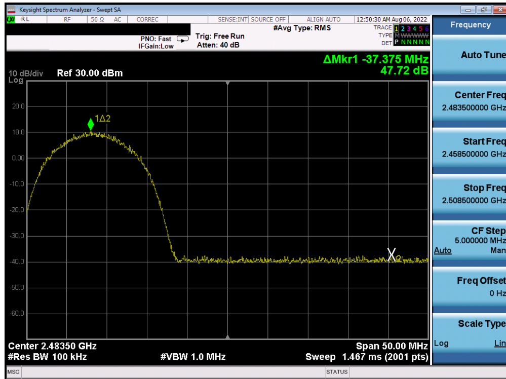
Plot 7-258. Band Edge Plot Antenna 4a (802.11b – Ch. 12) – 11Mbps
