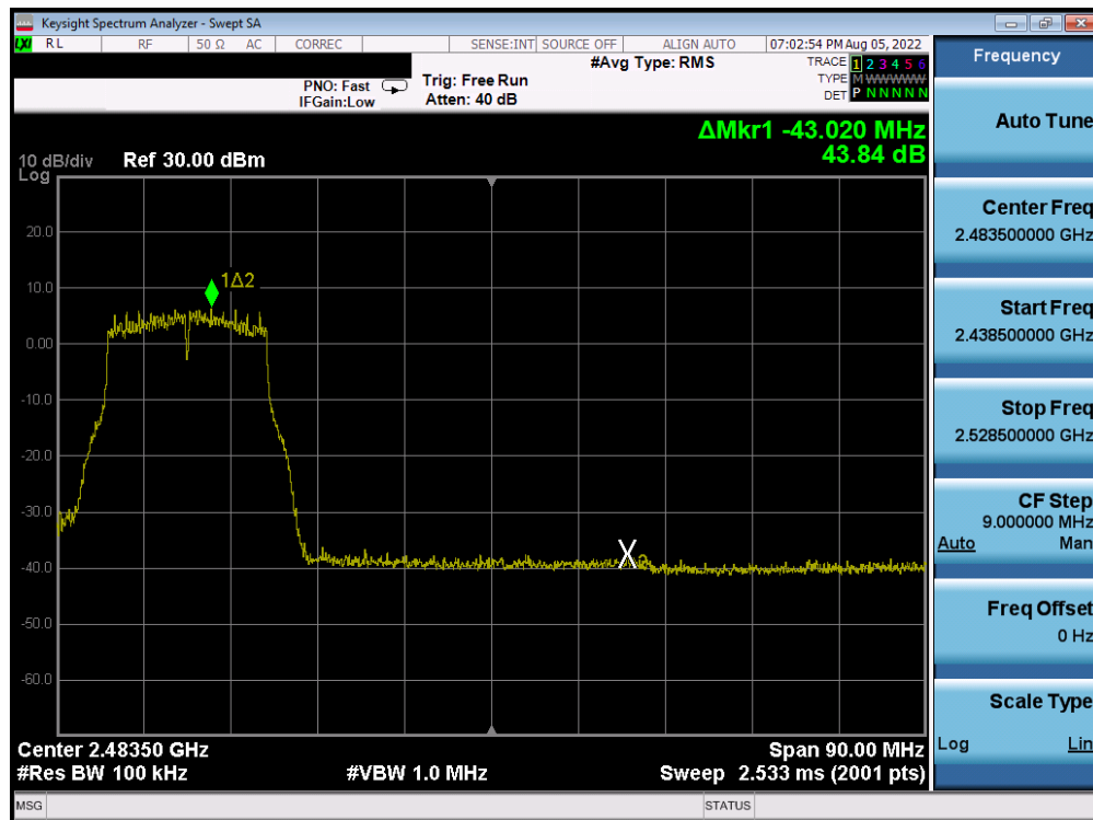
Plot 7-269. Band Edge Plot Antenna 4a (802.11g - Ch. 9) – 36Mbps
