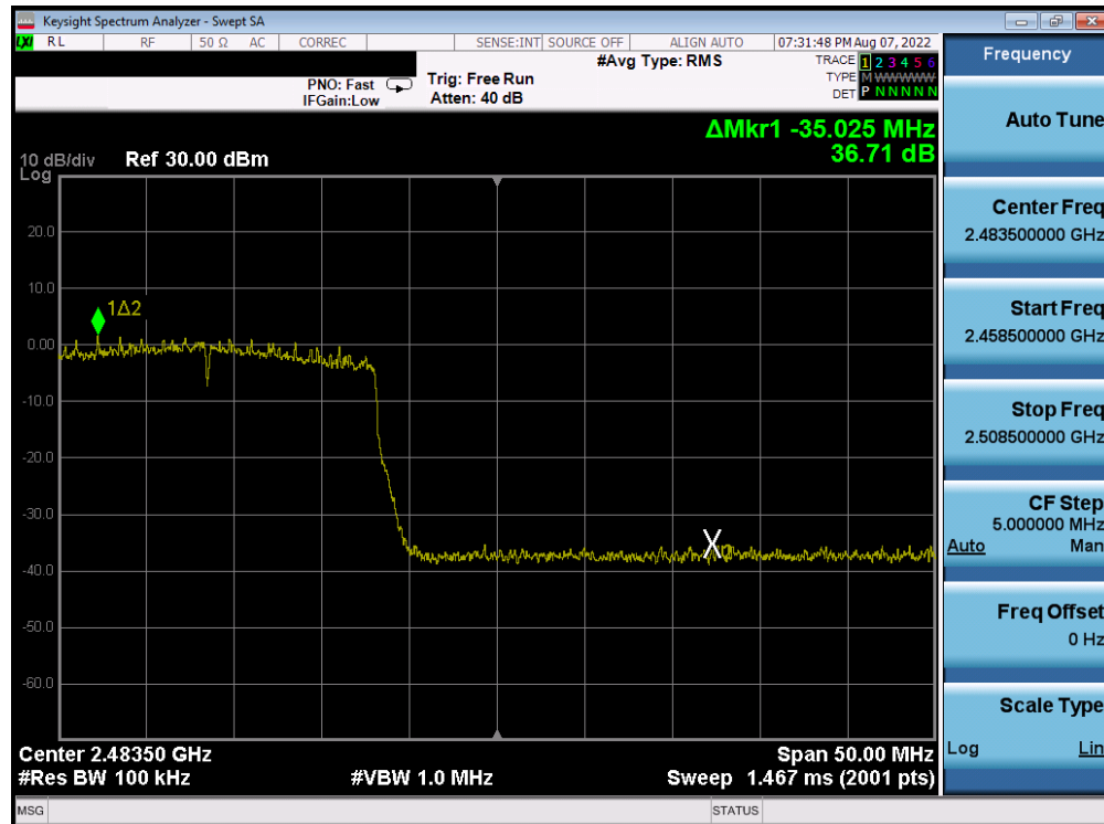
Plot 7-253. Band Edge Plot Antenna 4a (802.11ax (SU - 2.4GHz) - Ch. 12) - MCS3
