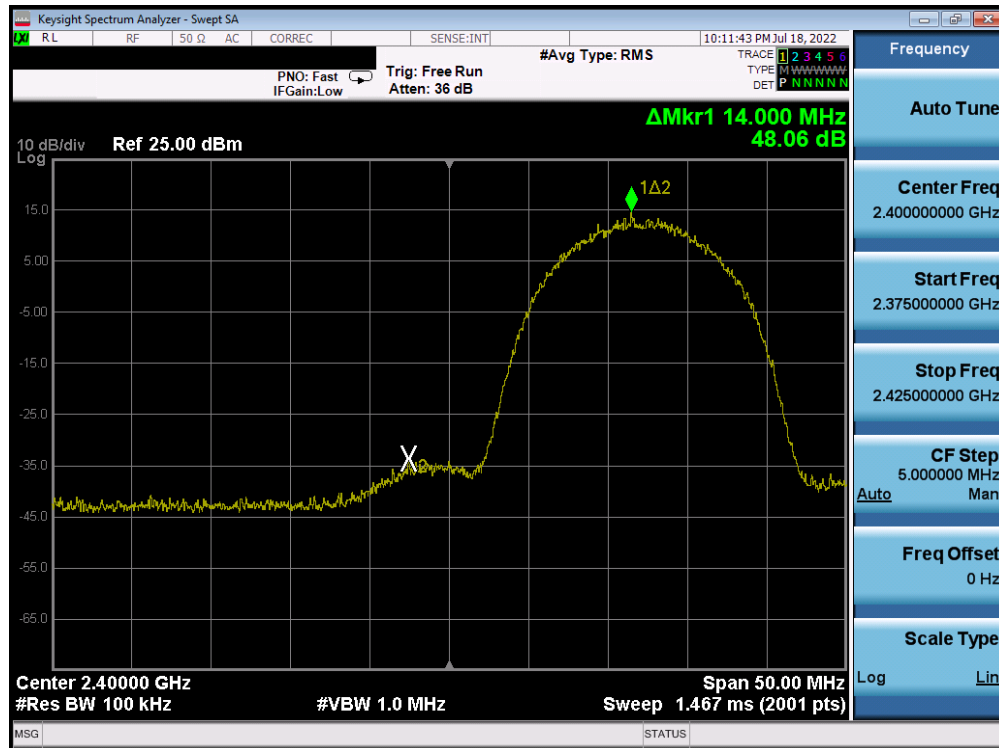
Plot 7-254. Band Edge Plot Antenna 4a (802.11b – Ch. 1) – 11Mbps
