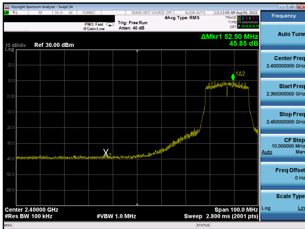
Plot 7-232. Band Edge Plot Antenna 4a (802.11n (2.4GHz) – Ch. 6 (low)) – MCS3
