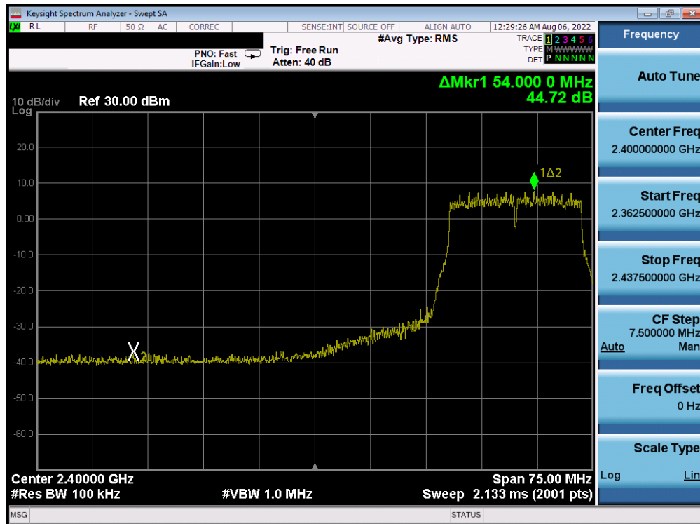
Plot 7-277. Band Edge Plot Antenna 4a (802.11n (2.4GHz) - Ch. 4) - MCS5
