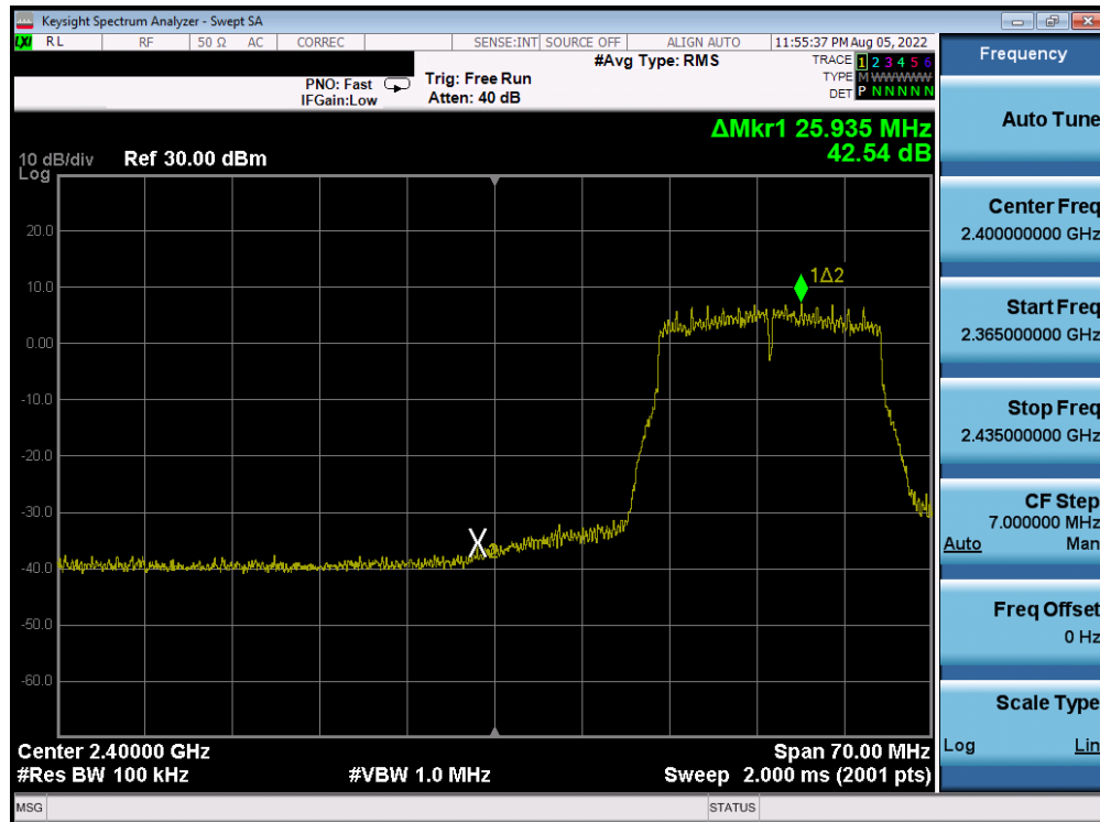
Plot 7-229. Band Edge Plot Antenna 4a (802.11n (2.4GHz) - Ch. 3) - MCS3
