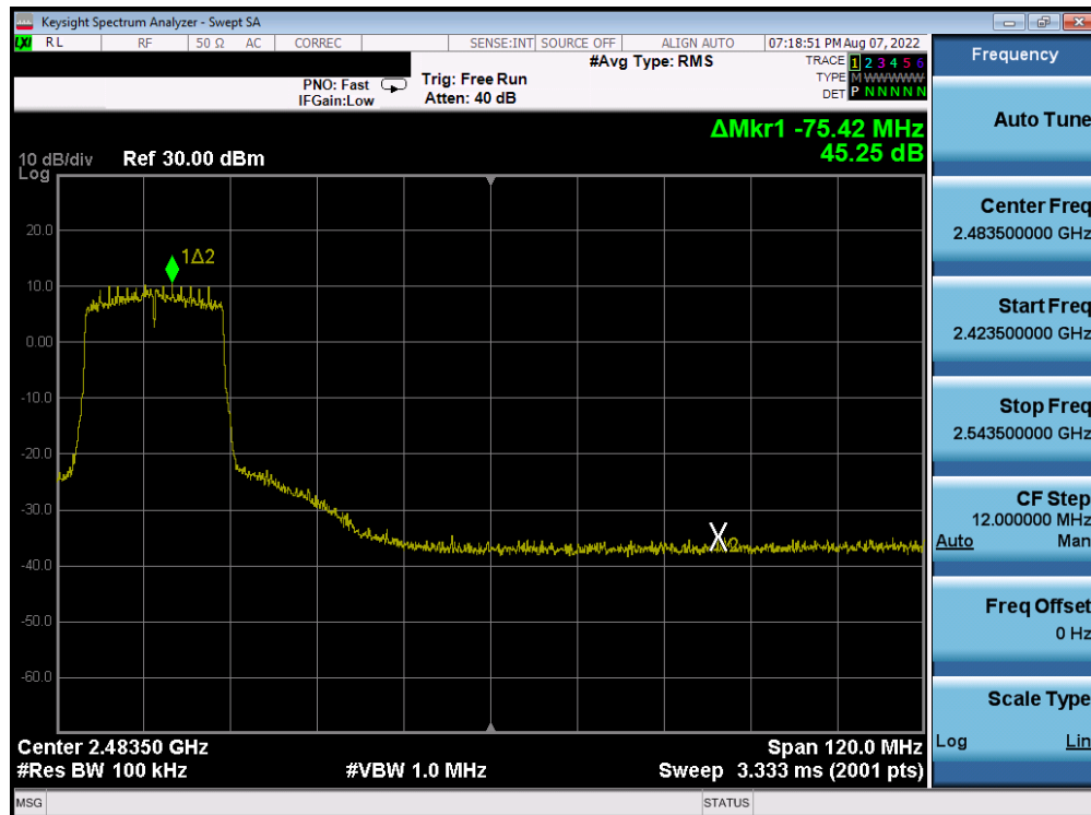
Plot 7-206. Band Edge Plot Antenna 4a (802.11ax (2.4GHz) – Ch. 6 (high)) – MCS2
