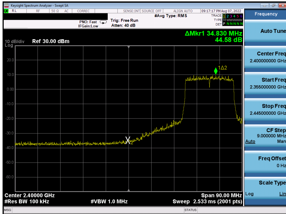
Plot 7-292. Band Edge Plot Antenna 4a (802.11ax (2.4GHz) – Ch. 5) – MCS5
