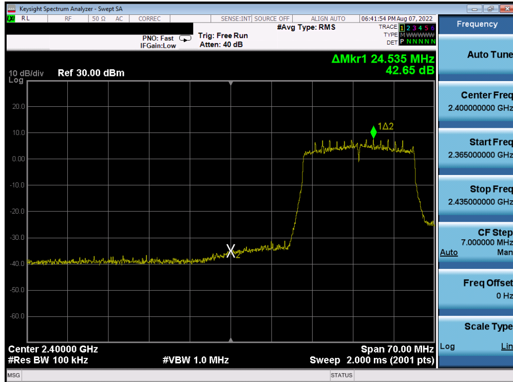
Plot 7-203. Band Edge Plot Antenna 4a (802.11ax (SU - 2.4GHz) – Ch. 3) – MCS2
