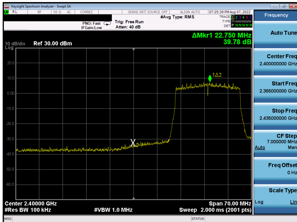
Plot 7-243. Band Edge Plot Antenna 4a (802.11ax (SU - 2.4GHz) – Ch. 3) – MCS3
