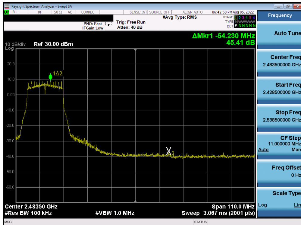
Plot 7-220. Band Edge Plot Antenna 4a (802.11g- Ch. 7) – 18Mbps
