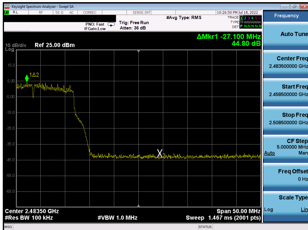
Plot 7-271. Band Edge Plot Antenna 4a (802.11g – Ch. 11) – 36Mbps
