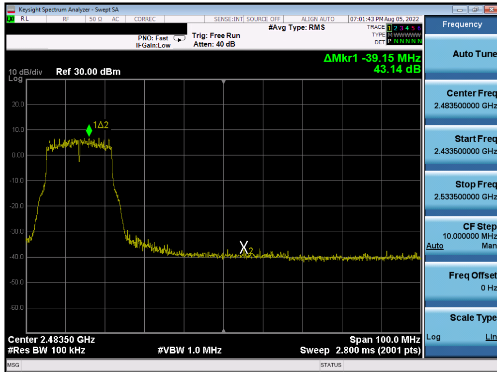
Plot 7-268. Band Edge Plot Antenna 4a (802.11g- Ch. 8) – 36Mbps
