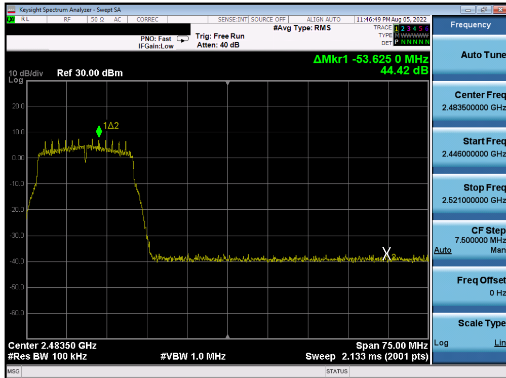
Plot 7-197. Band Edge Plot Antenna 4a (802.11n (2.4GHz) - Ch. 10) - MCS2
