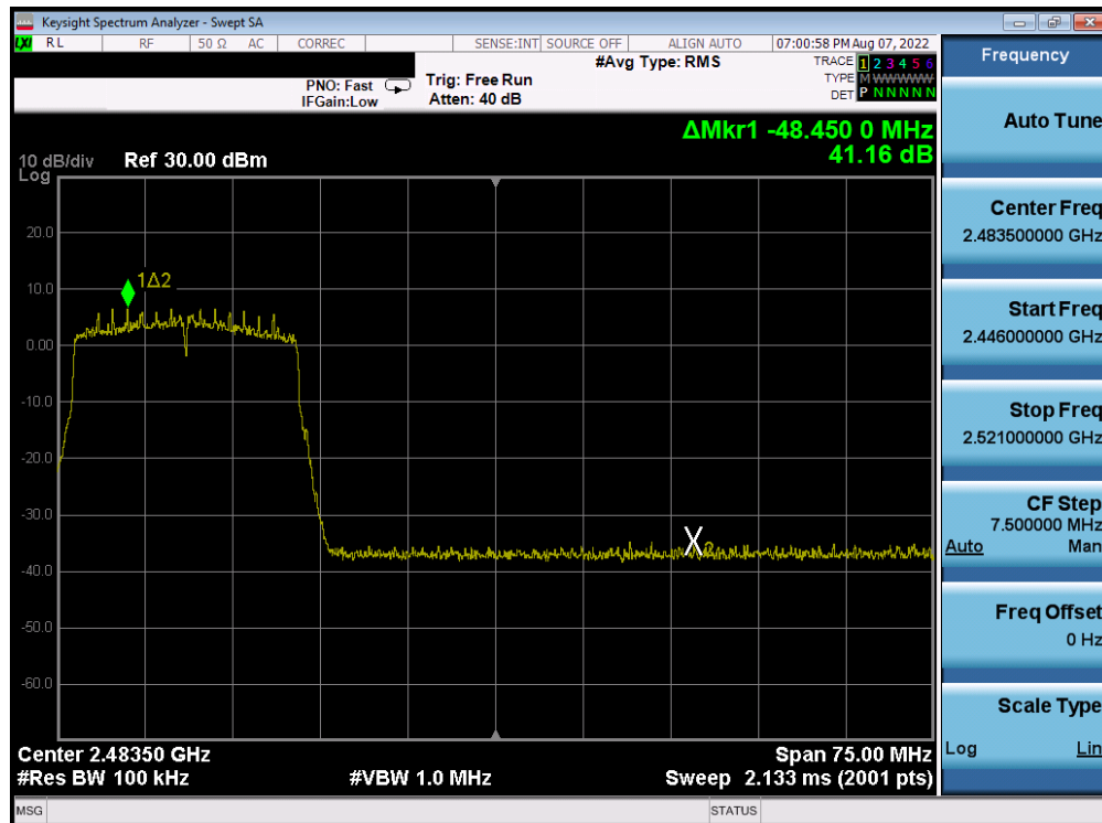
Plot 7-210. Band Edge Plot Antenna 4a (802.11ax (SU - 2.4GHz) - Ch. 10) - MCS2
