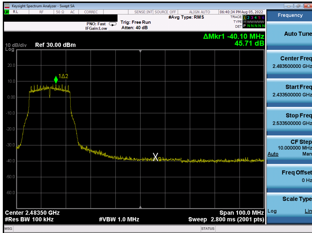
Plot 7-221. Band Edge Plot Antenna 4a (802.11g- Ch. 8) – 18Mbps
