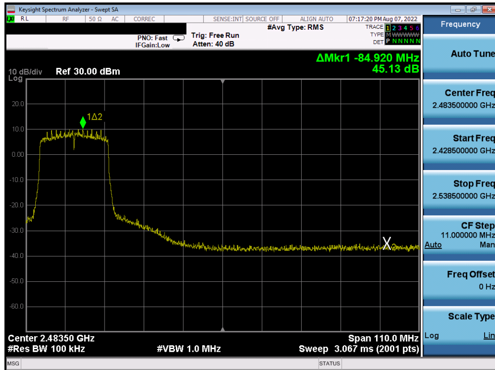
Plot 7-207. Band Edge Plot Antenna 4a (802.11ax (2.4GHz) – Ch. 7) – MCS2
