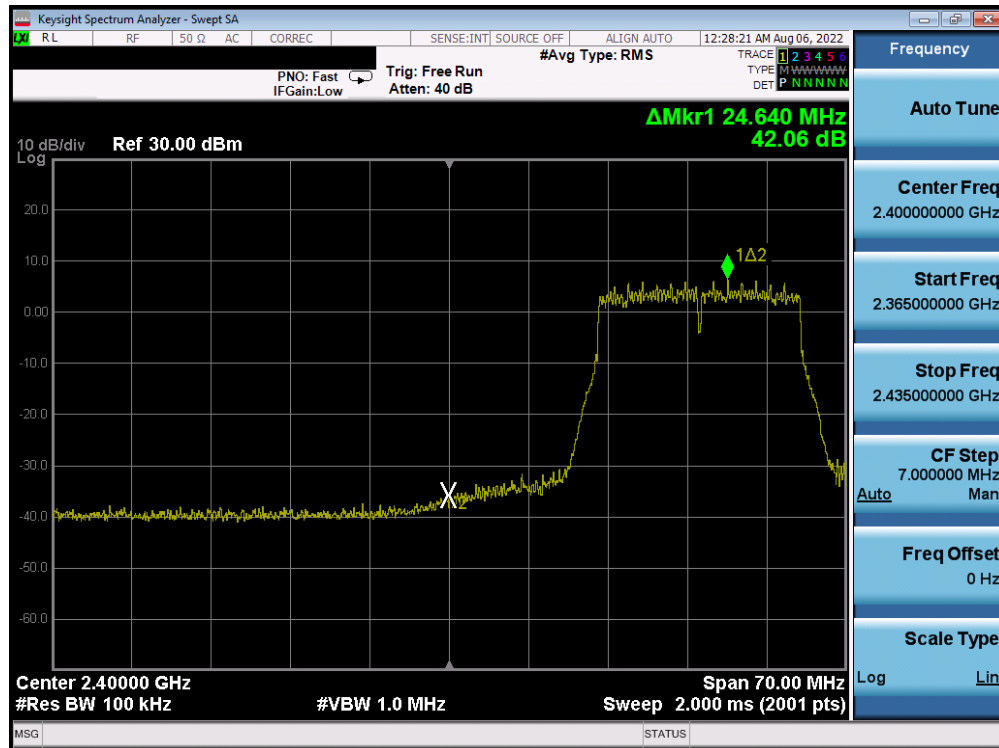
Plot 7-276. Band Edge Plot Antenna 4a (802.11n (2.4GHz) - Ch. 3) - MCS5
