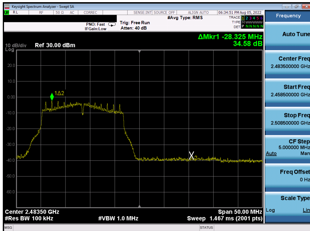
Plot 7-226. Band Edge Plot Antenna 4a (802.11g – Ch. 13) – 18Mbps
