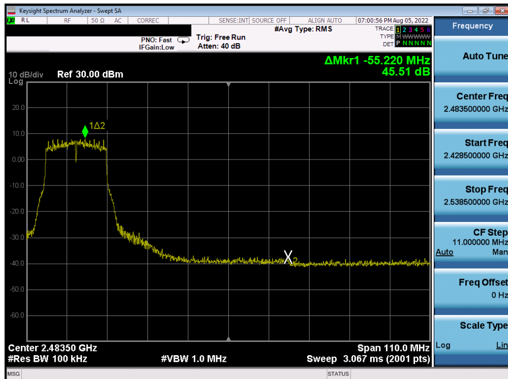
Plot 7-267. Band Edge Plot Antenna 4a (802.11g- Ch. 7) – 36Mbps
