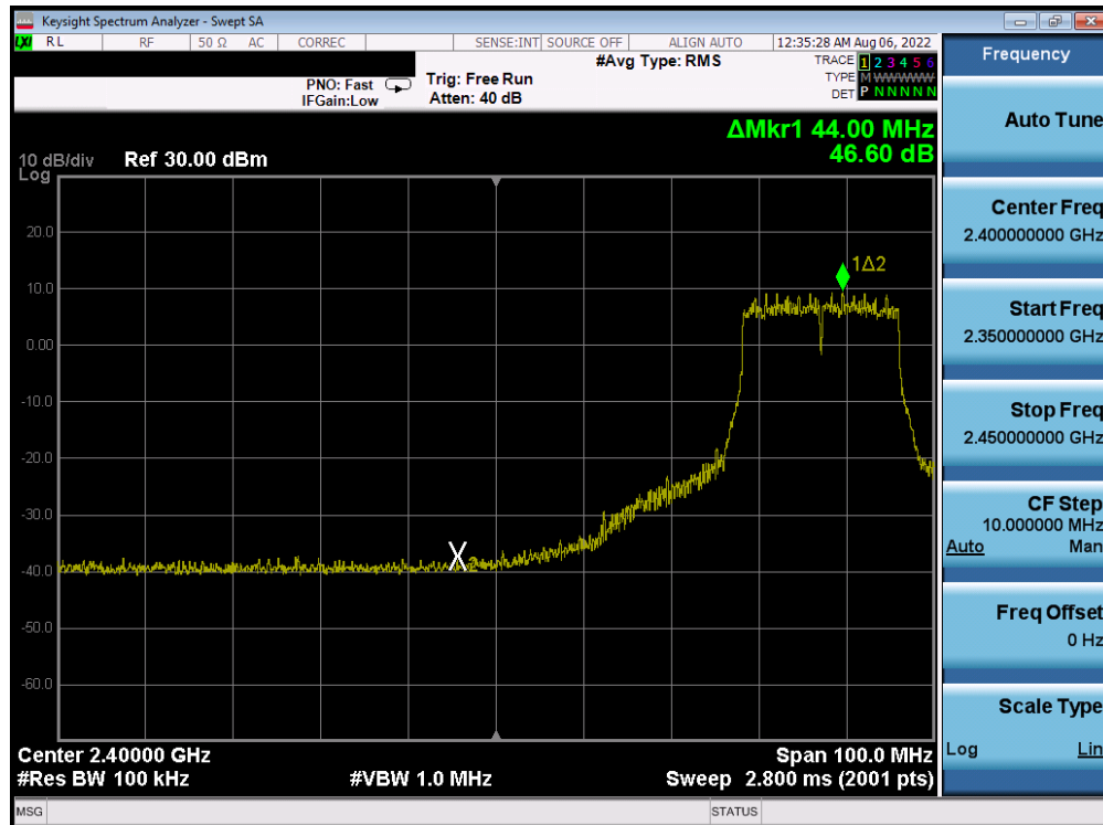
Plot 7-279. Band Edge Plot Antenna 4a (802.11n (2.4GHz) – Ch. 6 (low)) – MCS5
