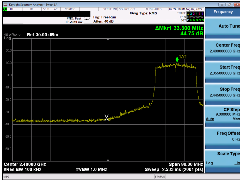
Plot 7-245. Band Edge Plot Antenna 4a (802.11ax (2.4GHz) – Ch. 5) – MCS3
