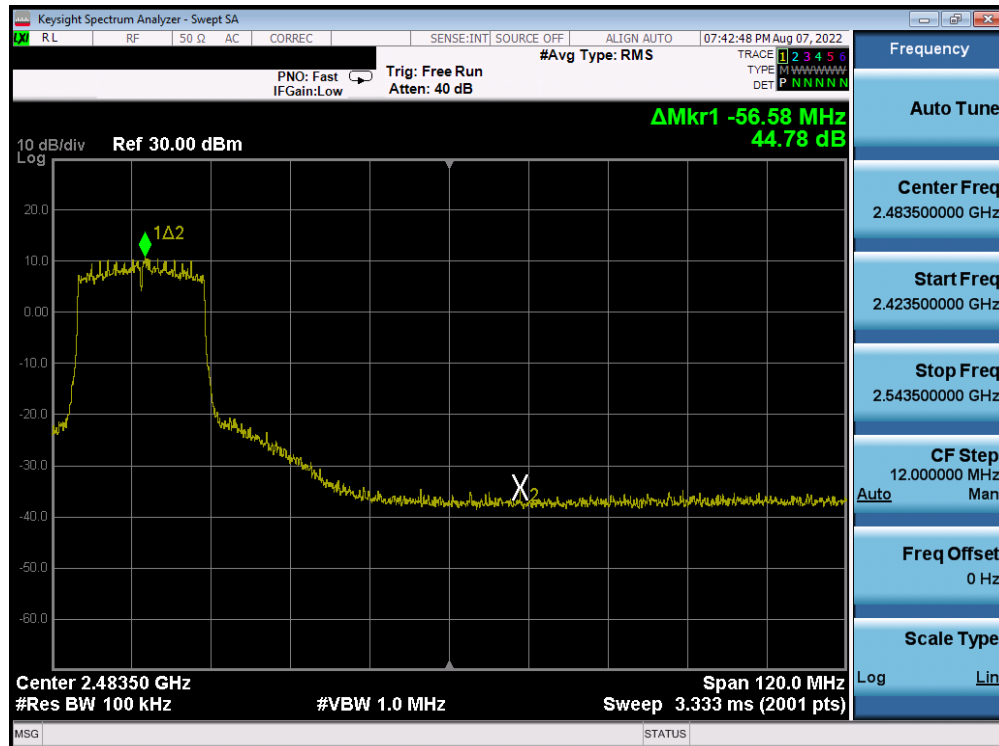
Plot 7-247. Band Edge Plot Antenna 4a (802.11ax (2.4GHz) – Ch. 6 (High)) – MCS3
