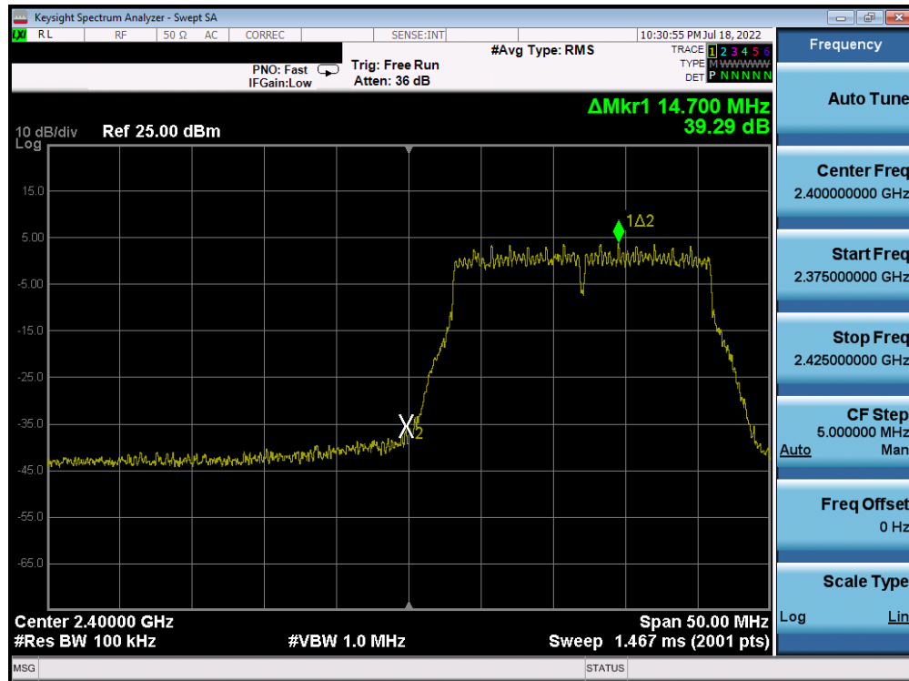
Plot 7-274. Band Edge Plot Antenna 4a (802.11n (2.4GHz) - Ch. 1) - MCS5
