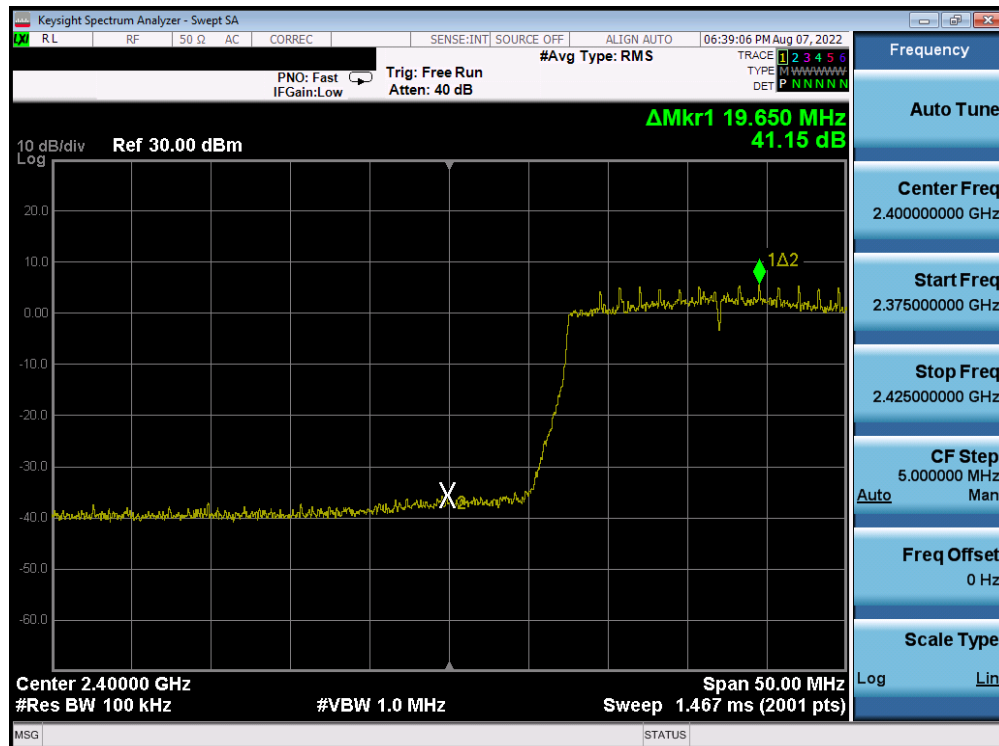
Plot 7-202. Band Edge Plot Antenna 4a (802.11ax (SU - 2.4GHz) – Ch. 2) – MCS2
