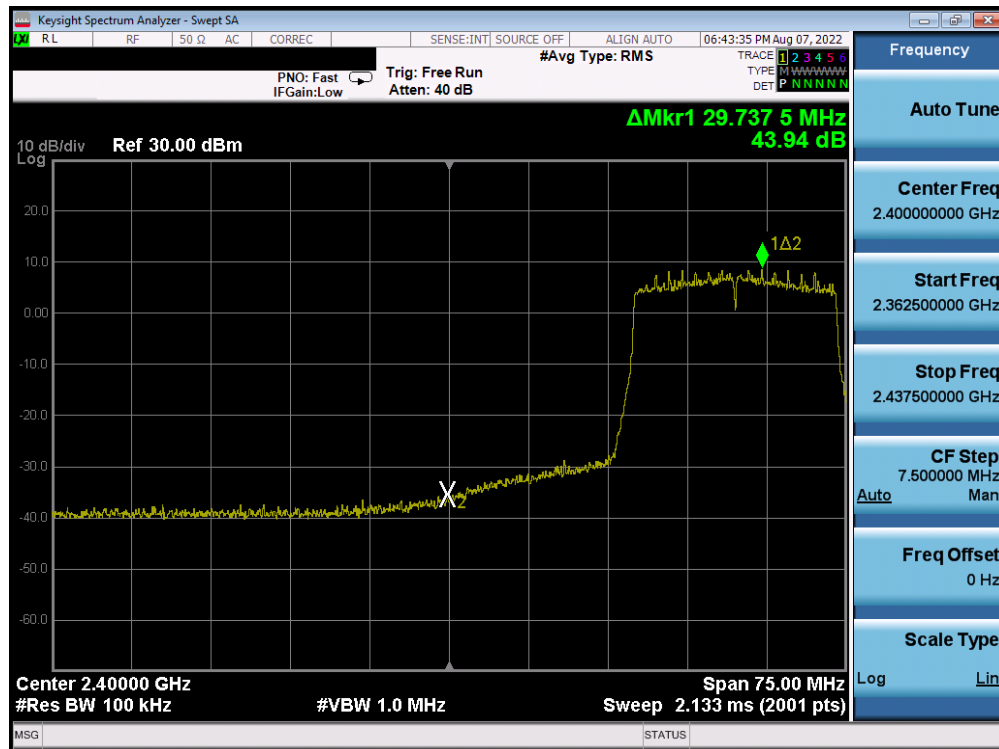
Plot 7-204. Band Edge Plot Antenna 4a (802.11ax (2.4GHz) – Ch. 4) – MCS2
