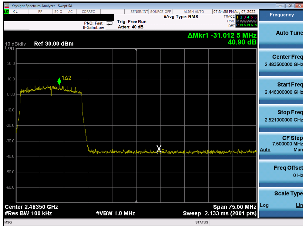
Plot 7-251. Band Edge Plot Antenna 4a (802.11ax (SU - 2.4GHz) – Ch. 10) – MCS3
