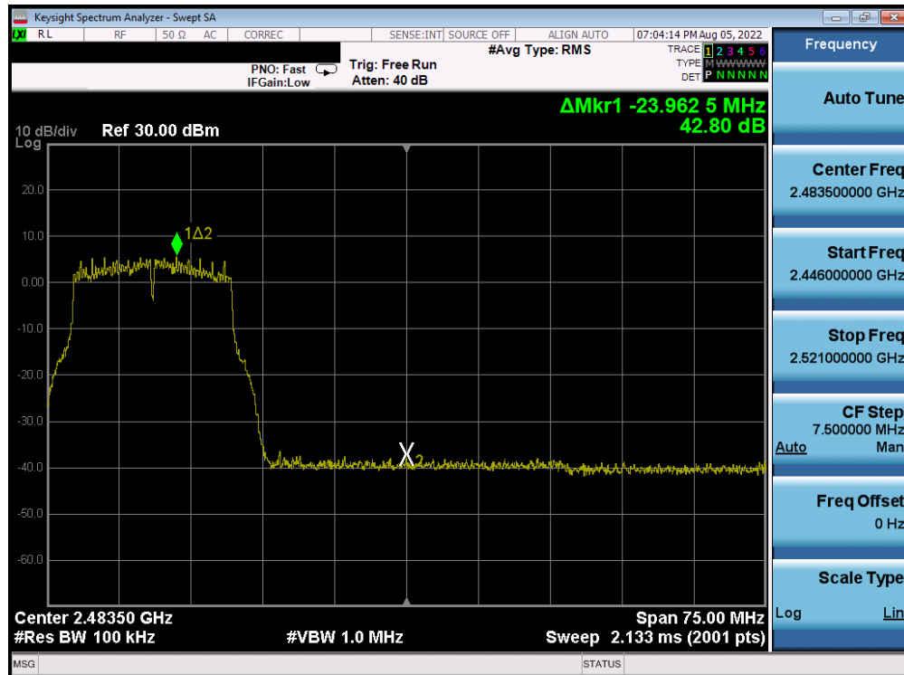
Plot 7-270. Band Edge Plot Antenna 4a (802.11g – Ch. 10) – 36Mbps
