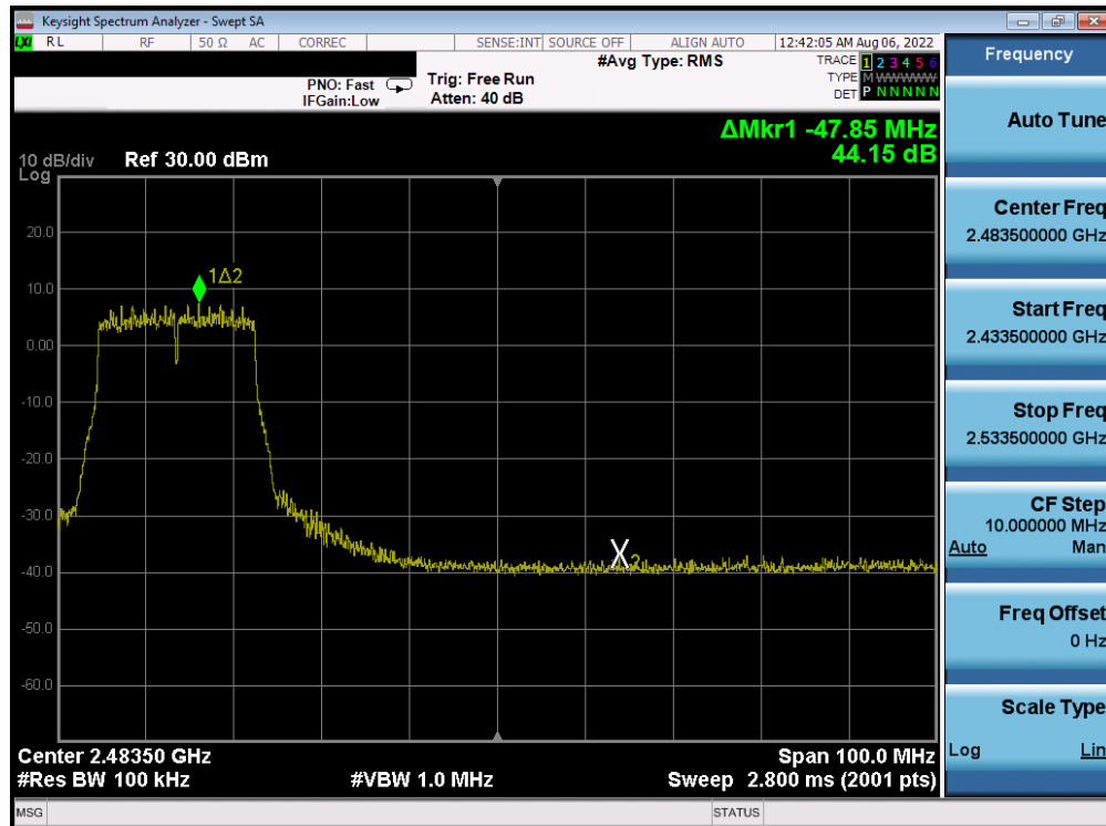
Plot 7-282. Band Edge Plot Antenna 4a (802.11n (2.4GHz) – Ch. 8) – MCS5
