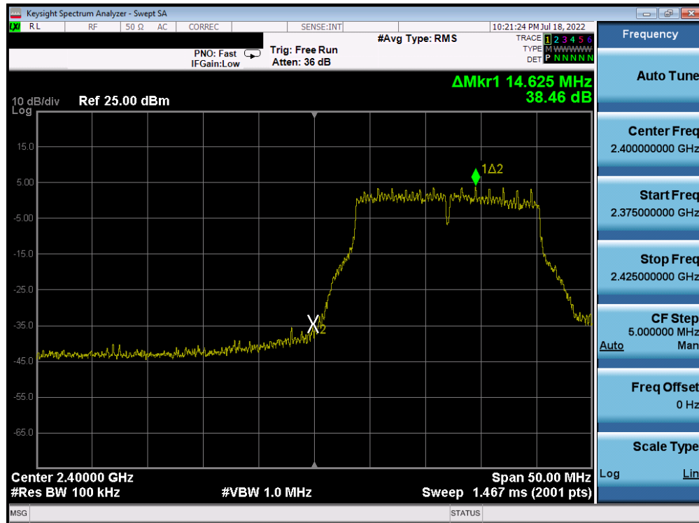
Plot 7-260. Band Edge Plot Antenna 4a (802.11g- Ch. 1) – 36Mbps
