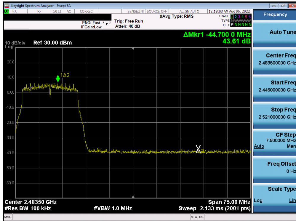
Plot 7-237. Band Edge Plot Antenna 4a (802.11n (2.4GHz) - Ch. 10) - MCS3
