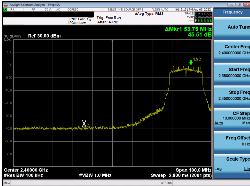
Plot 7-218. Band Edge Plot Antenna 4a (802.11g- Ch. 6 (low)) – 18Mbps
