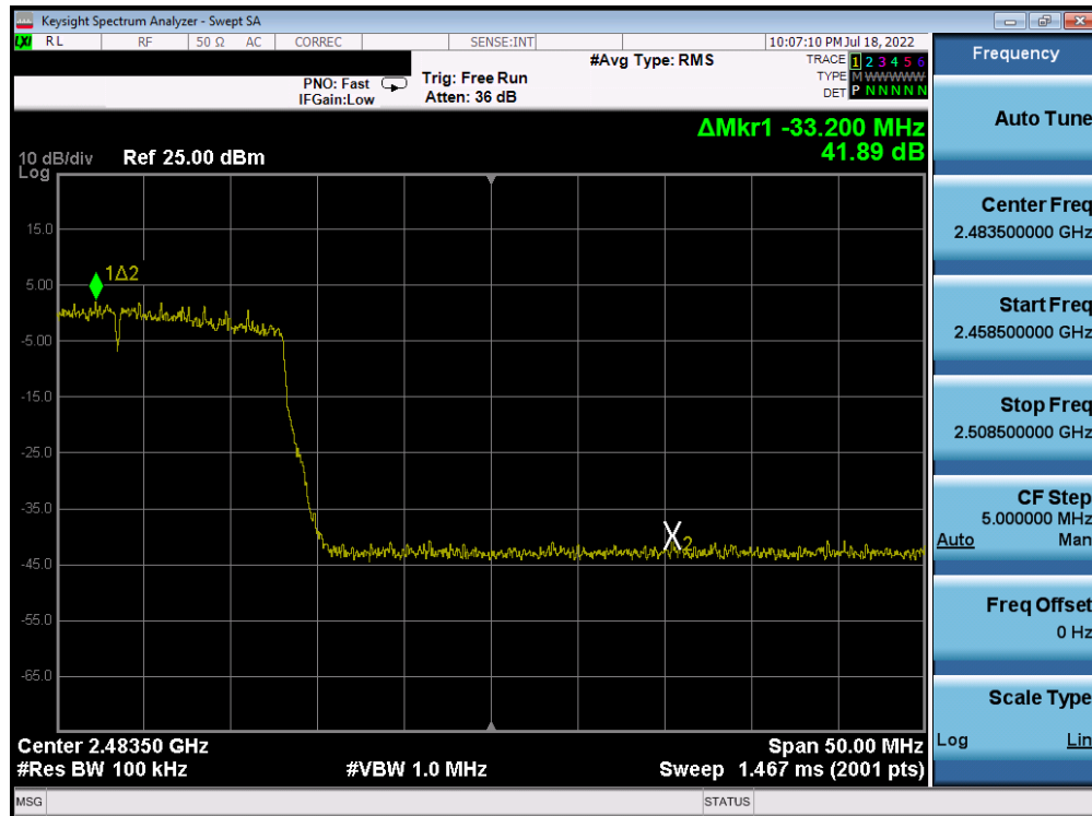
Plot 7-252. Band Edge Plot Antenna 4a (802.11ax (SU - 2.4GHz) – Ch. 11) – MCS3
