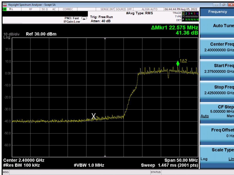
Plot 7-214. Band Edge Plot Antenna 4a (802.11g- Ch. 2) – 18Mbps
