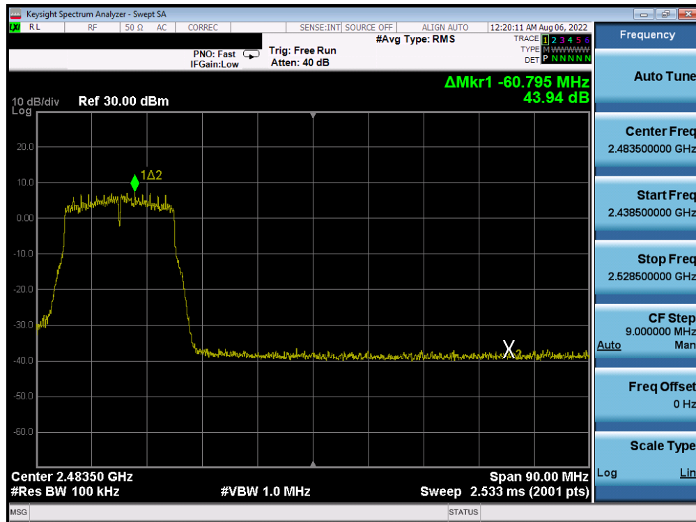
Plot 7-236. Band Edge Plot Antenna 4a (802.11n (2.4GHz) - Ch. 9) - MCS3
