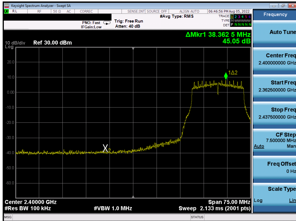
Plot 7-216. Band Edge Plot Antenna 4a (802.11g- Ch. 4) – 18Mbps
