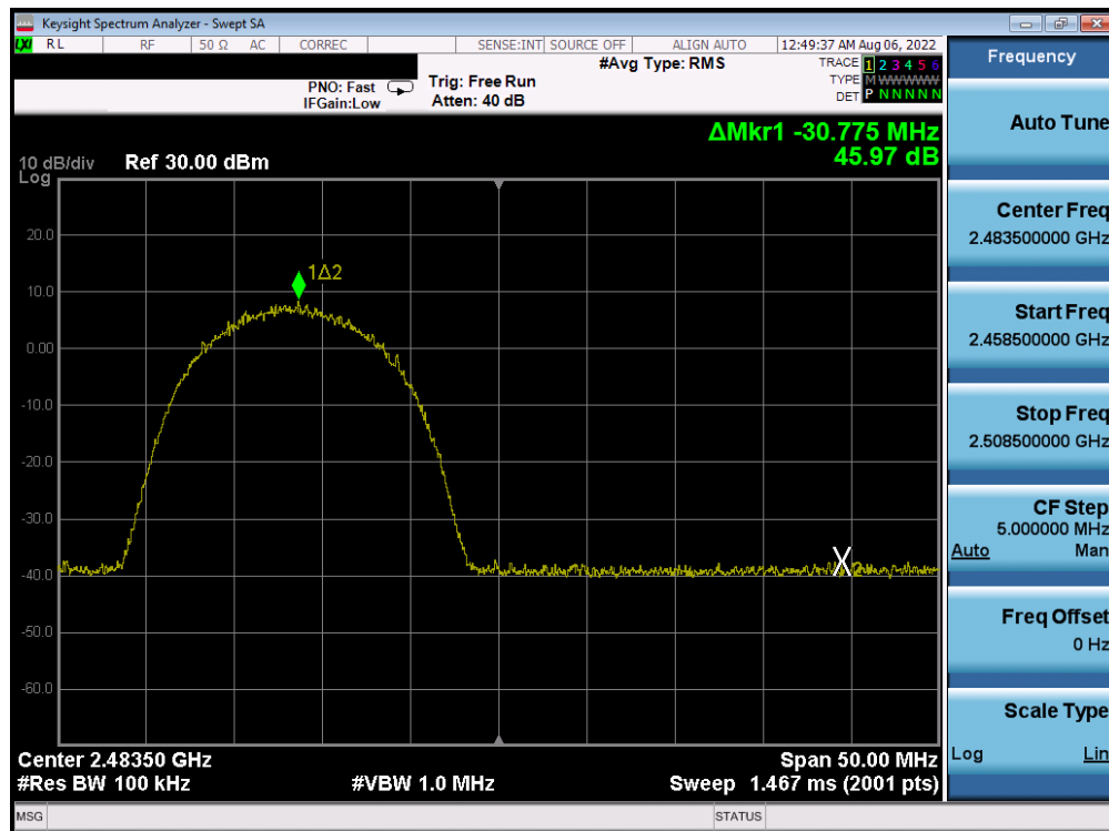
Plot 7-259. Band Edge Plot Antenna 4a (802.11b – Ch. 13) – 11Mbps
