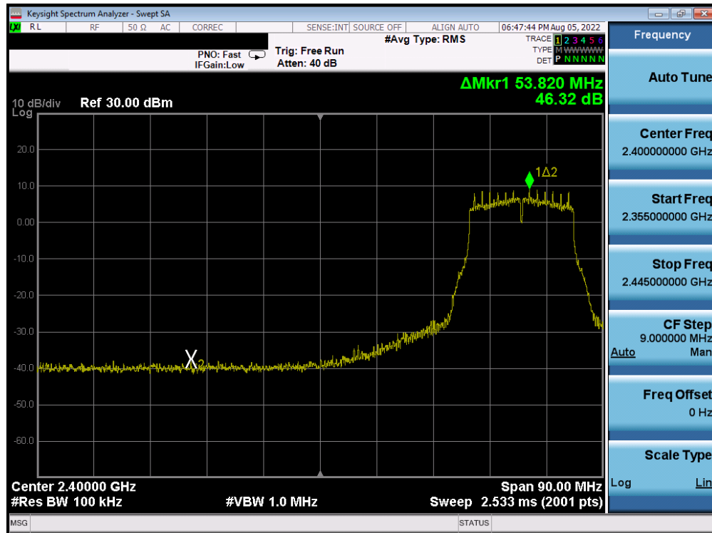
Plot 7-217. Band Edge Plot Antenna 4a (802.11g- Ch. 5) – 18Mbps
