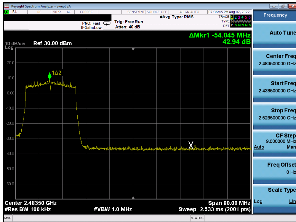
Plot 7-250. Band Edge Plot Antenna 4a (802.11ax (SU - 2.4GHz) – Ch. 9) – MCS3
