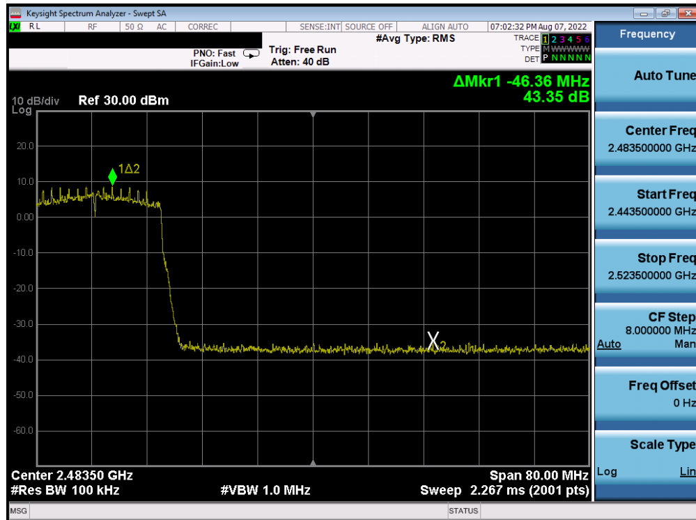
Plot 7-209. Band Edge Plot Antenna 4a (802.11ax (SU - 2.4GHz) - Ch. 9) - MCS2
