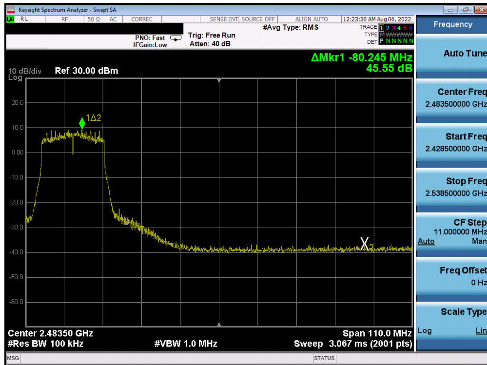
Plot 7-234. Band Edge Plot Antenna 4a (802.11n (2.4GHz) – Ch. 7) – MCS3
