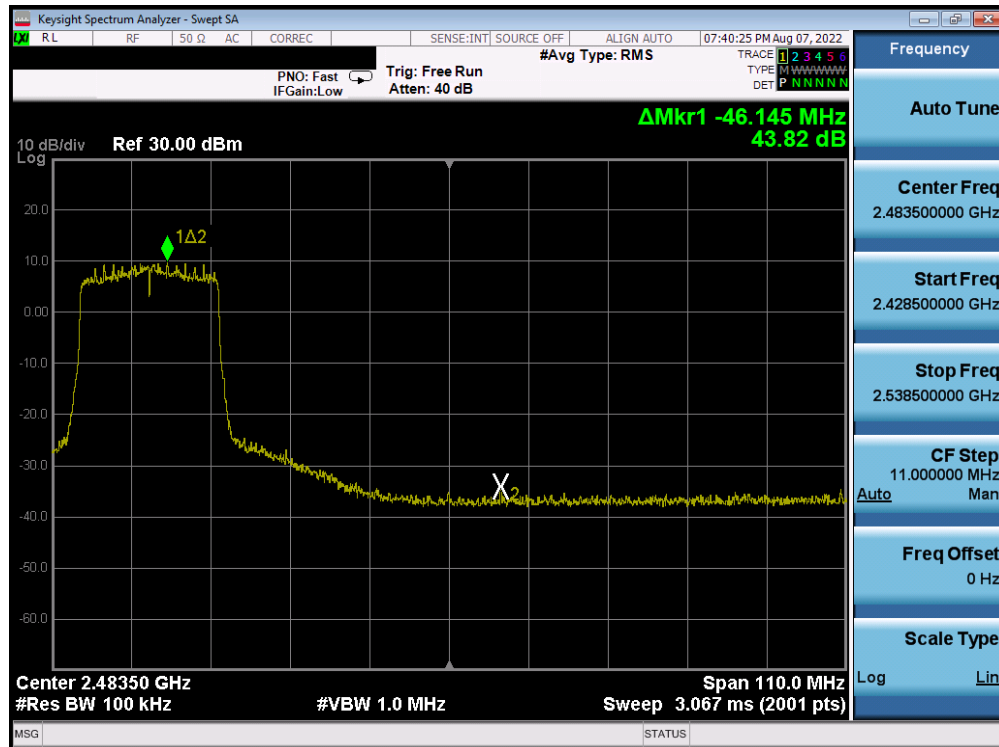
Plot 7-248. Band Edge Plot Antenna 4a (802.11ax (2.4GHz) – Ch. 7) – MCS3
