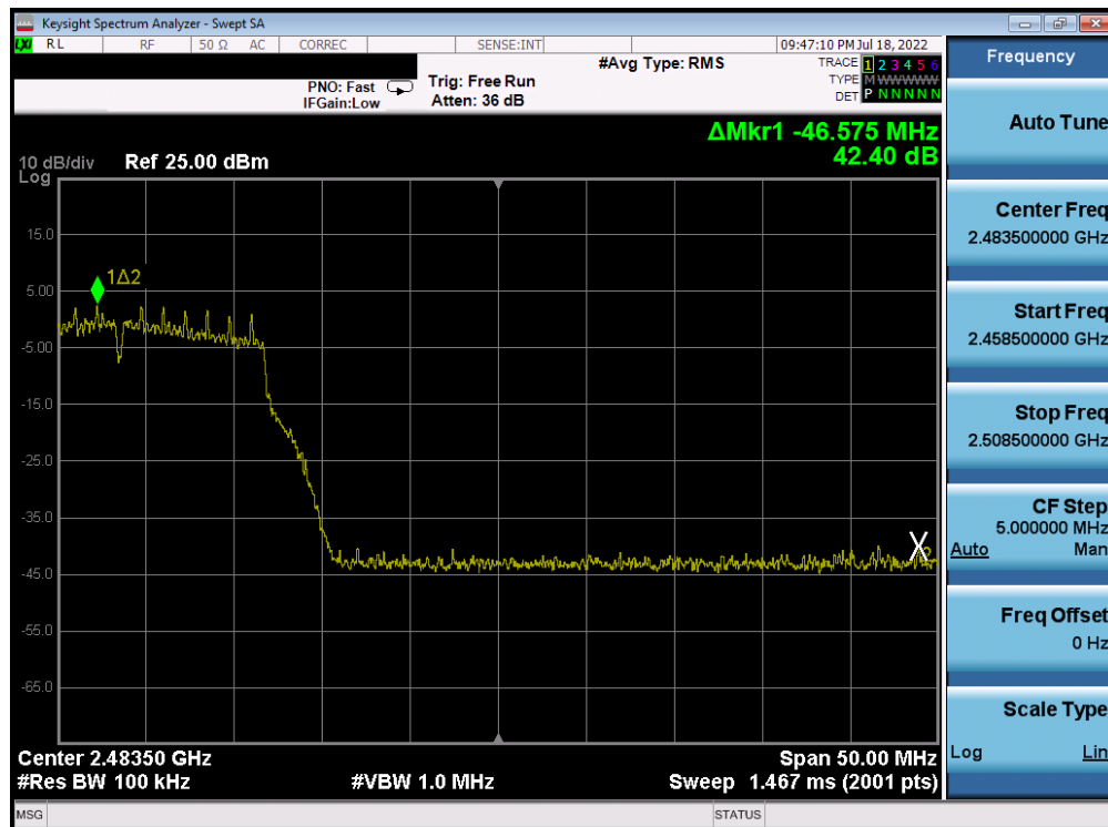
Plot 7-224. Band Edge Plot Antenna 4a (802.11g – Ch. 11) – 18Mbps
