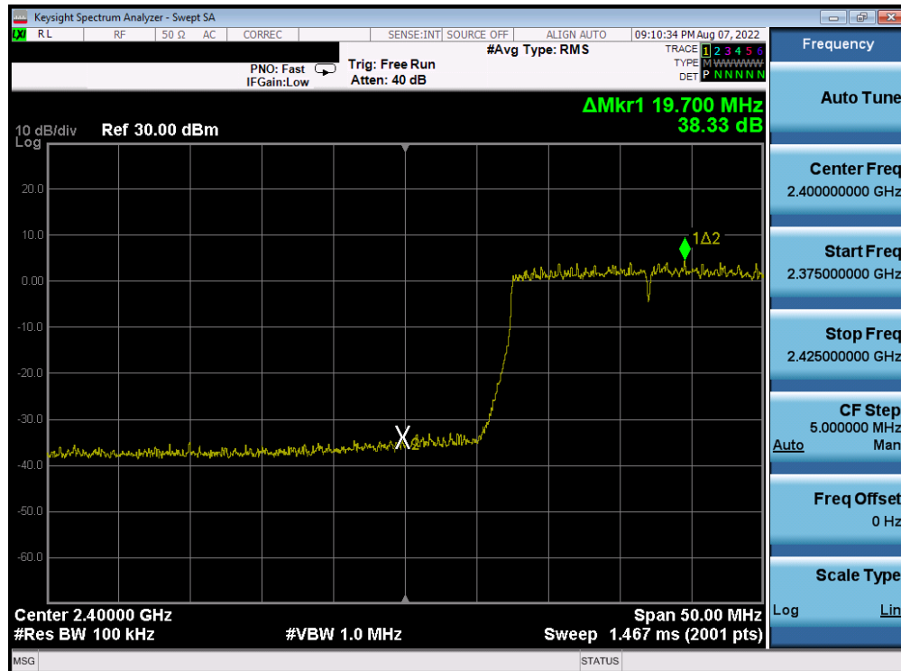
Plot 7-289. Band Edge Plot Antenna 4a (802.11ax (SU - 2.4GHz) - Ch. 2) - MCS5
