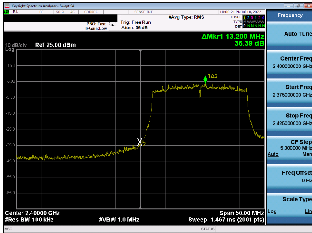
Plot 7-241. Band Edge Plot Antenna 4a (802.11ax (SU - 2.4GHz) – Ch. 1) – MCS3
