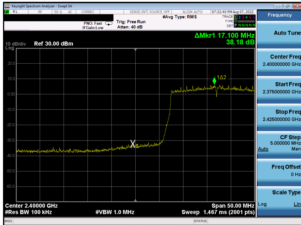
Plot 7-242. Band Edge Plot Antenna 4a (802.11ax (SU - 2.4GHz) – Ch. 2) – MCS3
