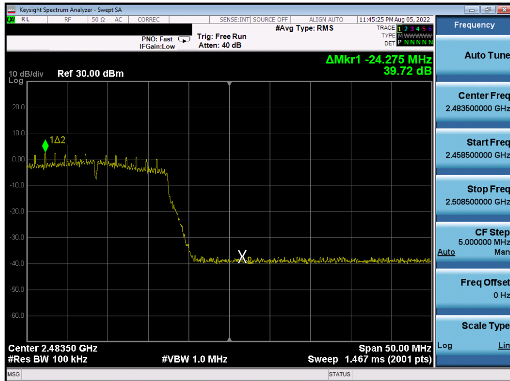
Plot 7-199. Band Edge Plot Antenna 4a (802.11n (2.4GHz) - Ch. 12) - MCS2
