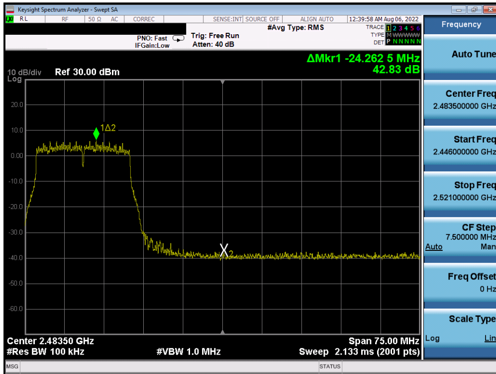
Plot 7-284. Band Edge Plot Antenna 4a (802.11n (2.4GHz) - Ch. 10) - MCS5
