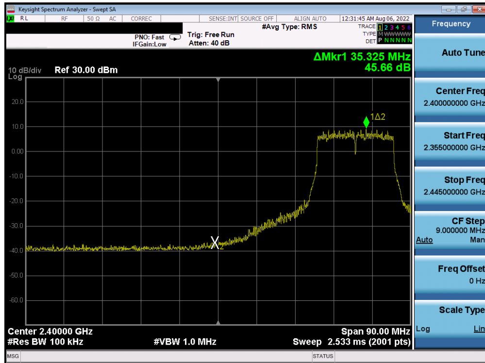
Plot 7-278. Band Edge Plot Antenna 4a (802.11n (2.4GHz) – Ch. 5) – MCS5
