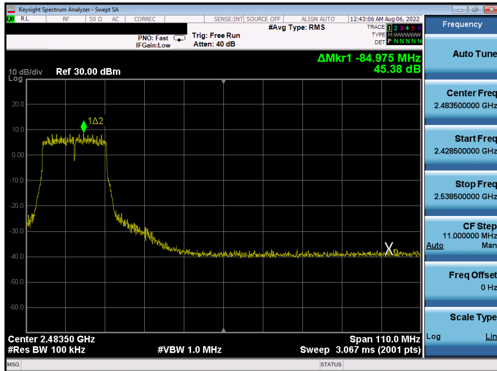
Plot 7-281. Band Edge Plot Antenna 4a (802.11n (2.4GHz) – Ch. 7) – MCS5
