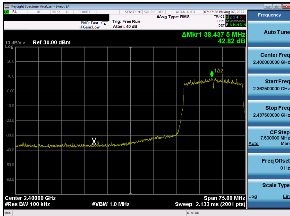
Plot 7-244. Band Edge Plot Antenna 4a (802.11ax (2.4GHz) – Ch. 4) – MCS3
