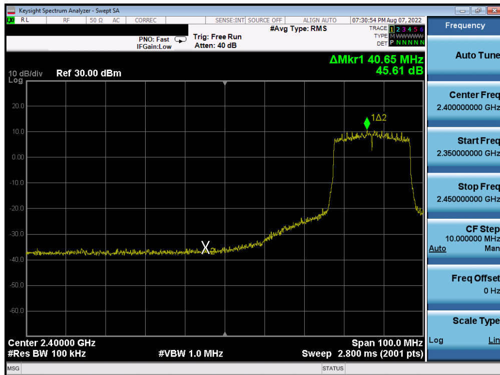
Plot 7-246. Band Edge Plot Antenna 4a (802.11ax (2.4GHz) – Ch. 6 (low)) – MCS3
