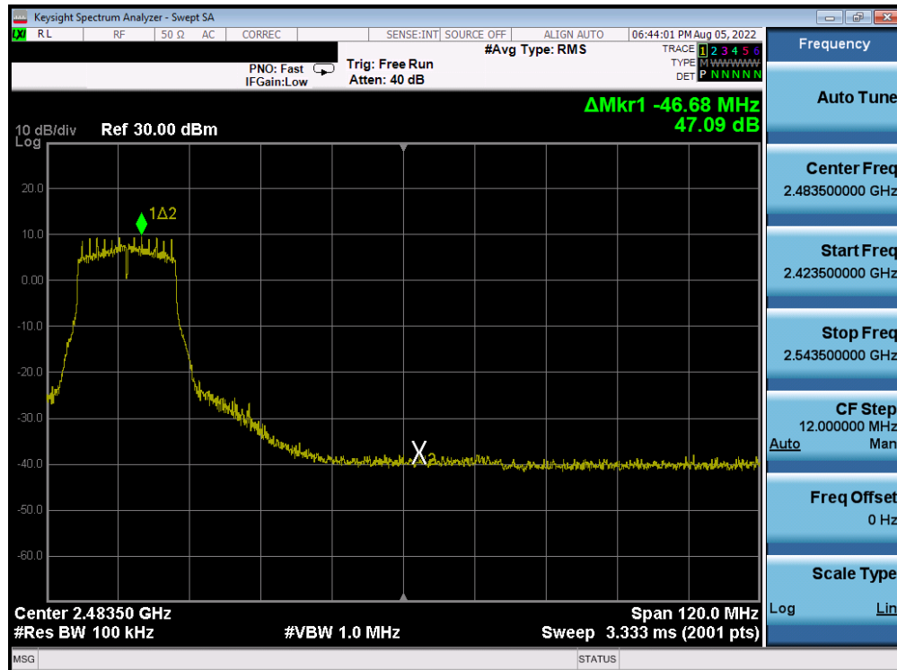
Plot 7-219. Band Edge Plot Antenna 4a (802.11g- Ch. 6 (high)) – 18Mbps
