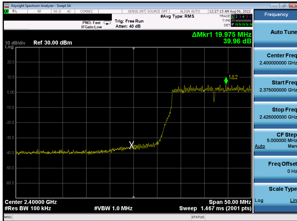
Plot 7-275. Band Edge Plot Antenna 4a (802.11n (2.4GHz) - Ch. 2) - MCS5
