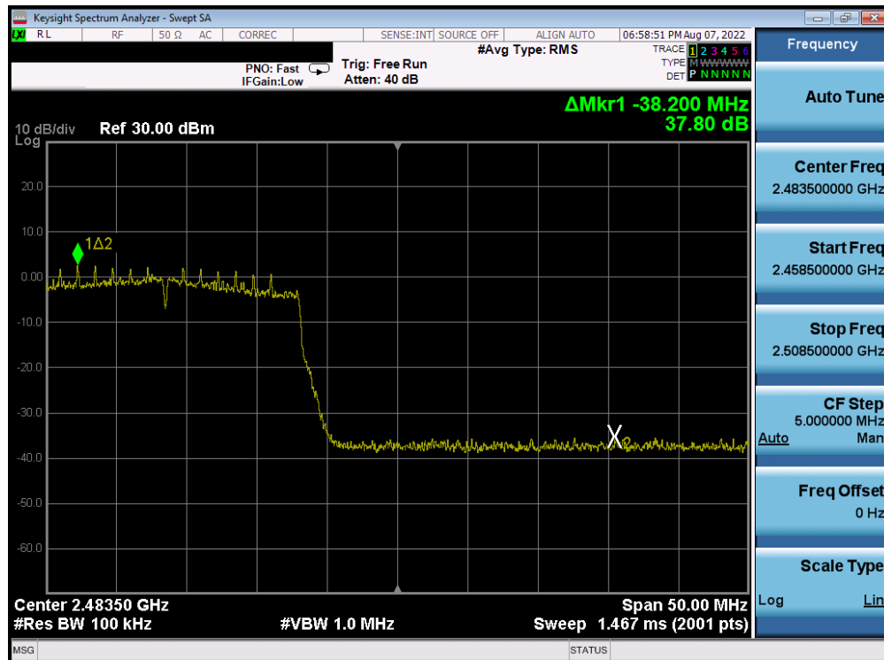
Plot 7-212. Band Edge Plot Antenna 4a (802.11ax (SU - 2.4GHz) – Ch. 12) – MCS2
