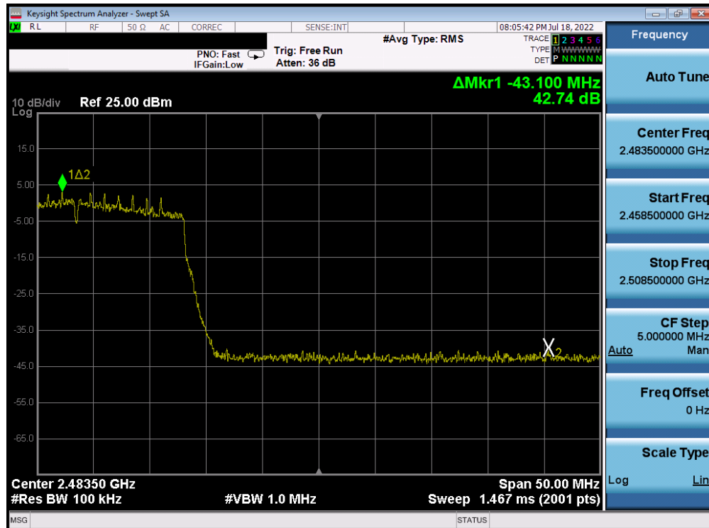
Plot 7-211. Band Edge Plot Antenna 4a (802.11ax (SU - 2.4GHz) – Ch. 11) – MCS2
