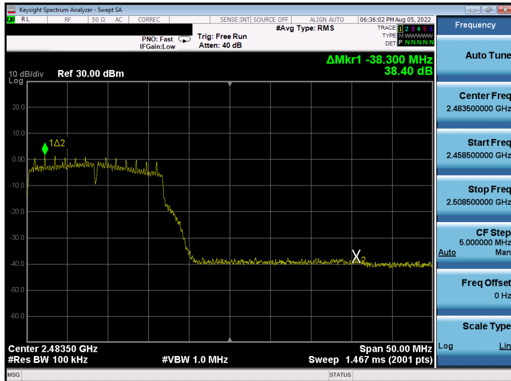
Plot 7-225. Band Edge Plot Antenna 4a (802.11g – Ch. 12) – 18Mbps
