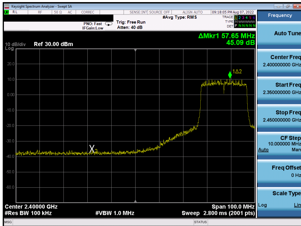
Plot 7-293. Band Edge Plot Antenna 4a (802.11ax (2.4GHz) – Ch. 6 (low)) – MCS5
