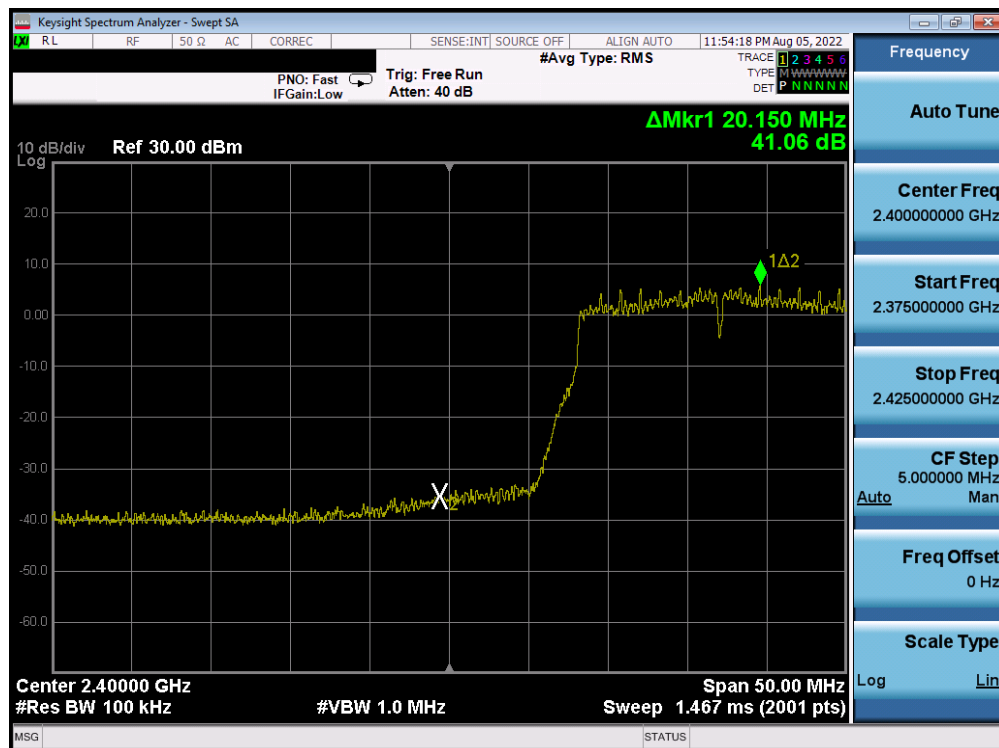
Plot 7-228. Band Edge Plot Antenna 4a (802.11n (2.4GHz) – Ch. 2) – MCS3
