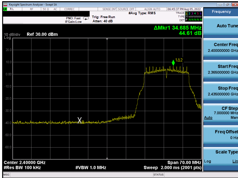
Plot 7-215. Band Edge Plot Antenna 4a (802.11g- Ch. 3) – 18Mbps
