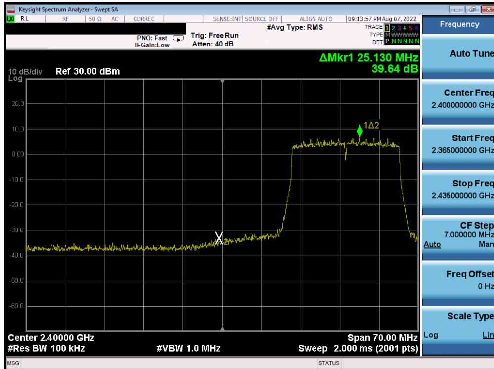
Plot 7-290. Band Edge Plot Antenna 4a (802.11ax (SU - 2.4GHz) – Ch. 3) – MCS5
