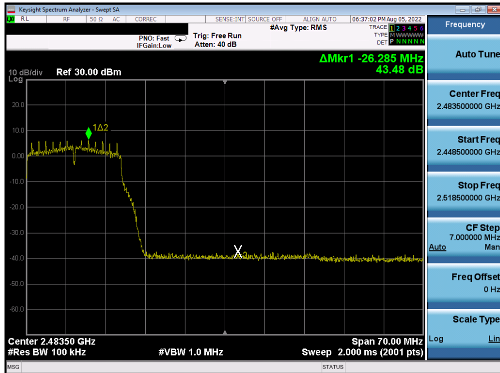
Plot 7-223. Band Edge Plot Antenna 4a (802.11g – Ch. 10) – 18Mbps
