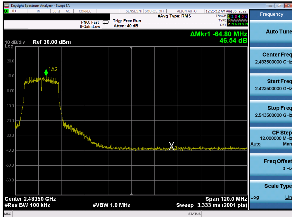
Plot 7-233. Band Edge Plot Antenna 4a (802.11n (2.4GHz) – Ch. 6 (high)) – MCS3
