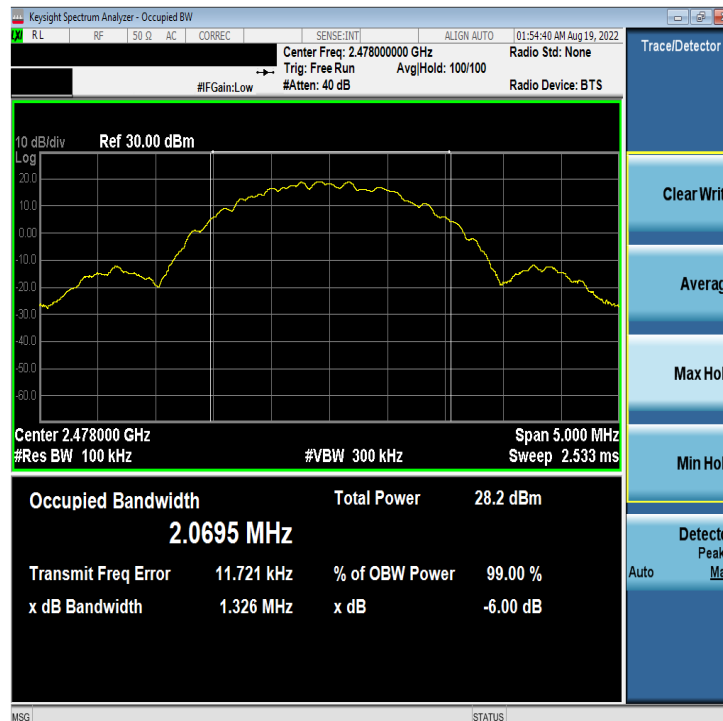
Plot 7-6. 6dB BW & 99% OBW Plot Antenna 4a (Bluetooth (LE), 2Mbps, ePA – Ch. 38)
