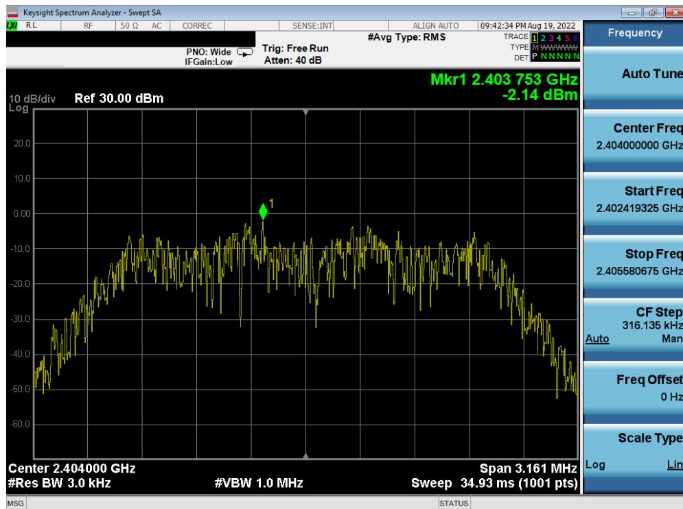
Plot 7-44. Power Spectral Density Plot Antenna 2a (Bluetooth (HDR4), 4Mbps, iPA – Ch. 1)
