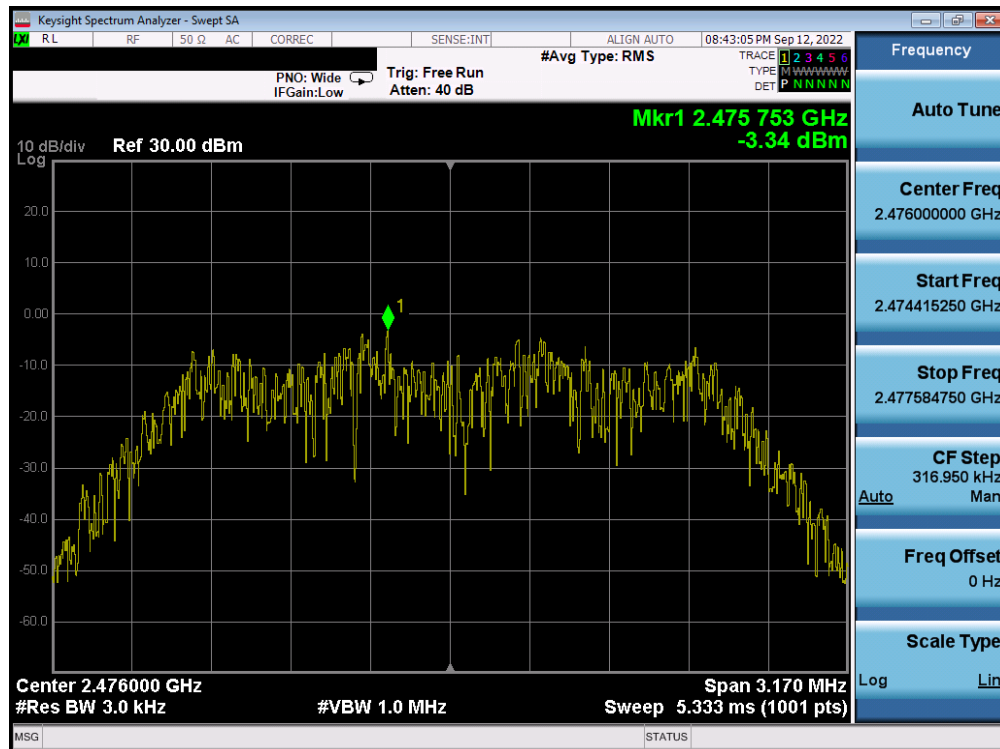
Plot 7-48. Power Spectral Density Plot Antenna 2a (Bluetooth (HDR4), 4Mbps, iPA – Ch. 73)
