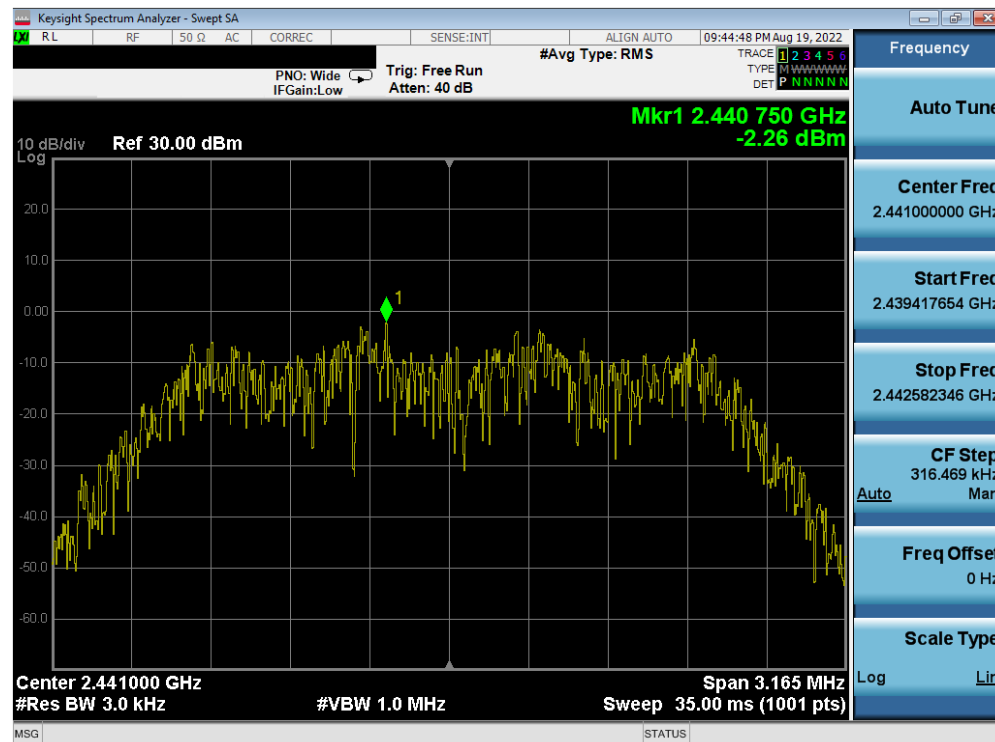
Plot 7-46. Power Spectral Density Plot Antenna 2a (Bluetooth (HDR4), 4Mbps, iPA – Ch. 38)
