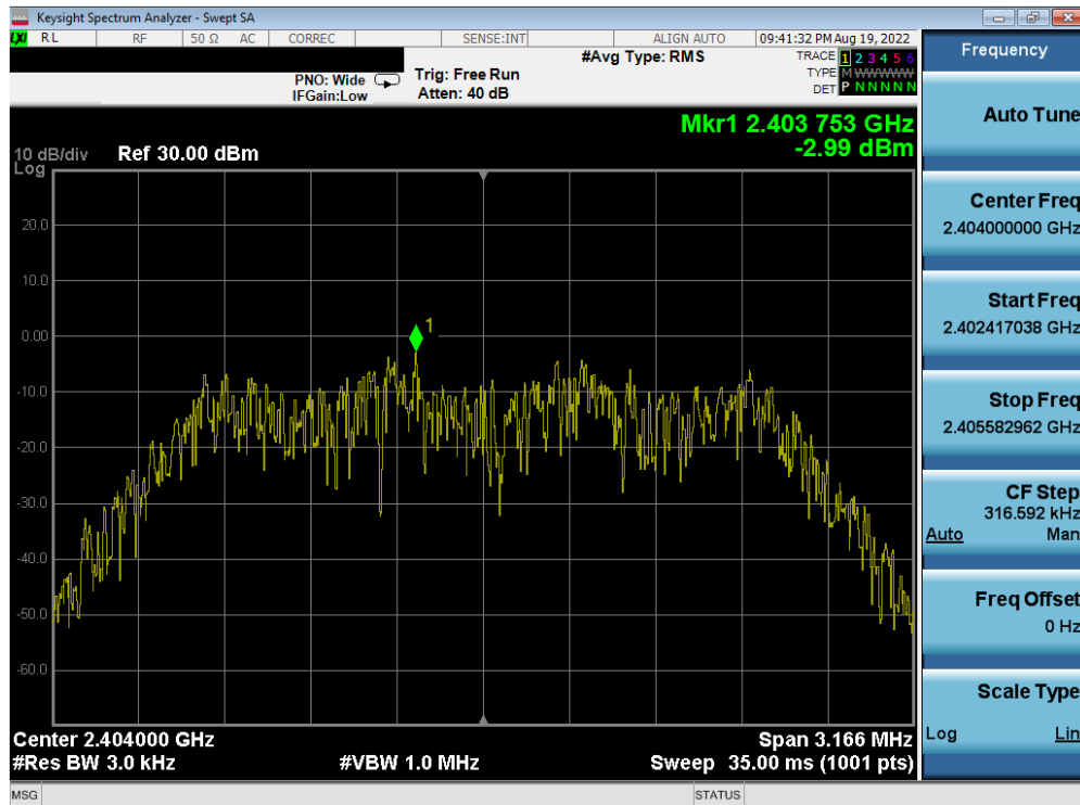
Plot 7-43. Power Spectral Density Plot Antenna 4a (Bluetooth (HDR4), 4Mbps, iPA – Ch. 1)
