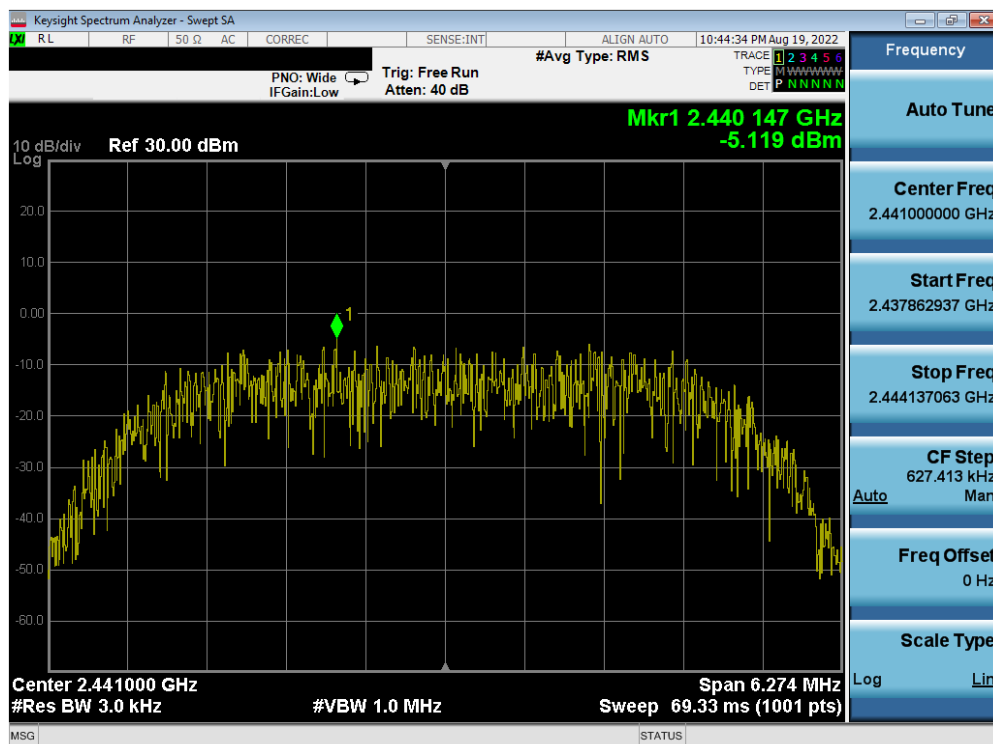
Plot 7-58. Power Spectral Density Plot Antenna 2a (Bluetooth (HDR8), 8Mbps, iPA – Ch. 38)
