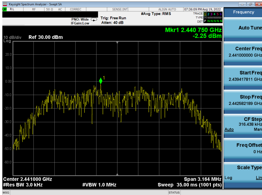
Plot 7-39. Power Spectral Density Plot Antenna 4a (Bluetooth (HDR4), 4Mbps, ePA – Ch. 38)
