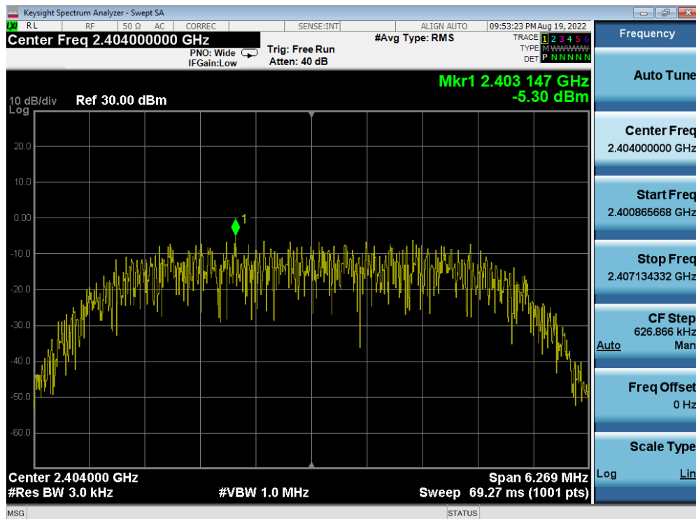
Plot 7-50. Power Spectral Density Plot Antenna 2a (Bluetooth (HDR8), 8Mbps, ePA – Ch. 1)
