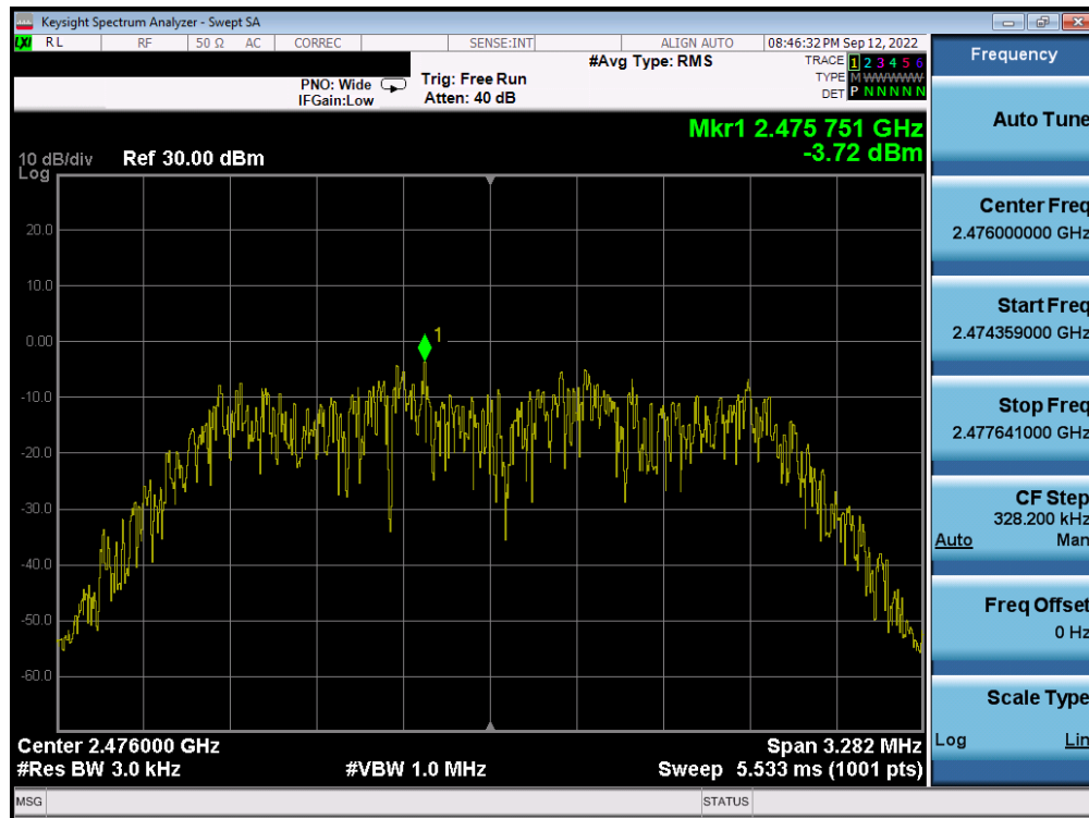
Plot 7-41. Power Spectral Density Plot Antenna 4a (Bluetooth (HDR4), 4Mbps, ePA – Ch. 73)
