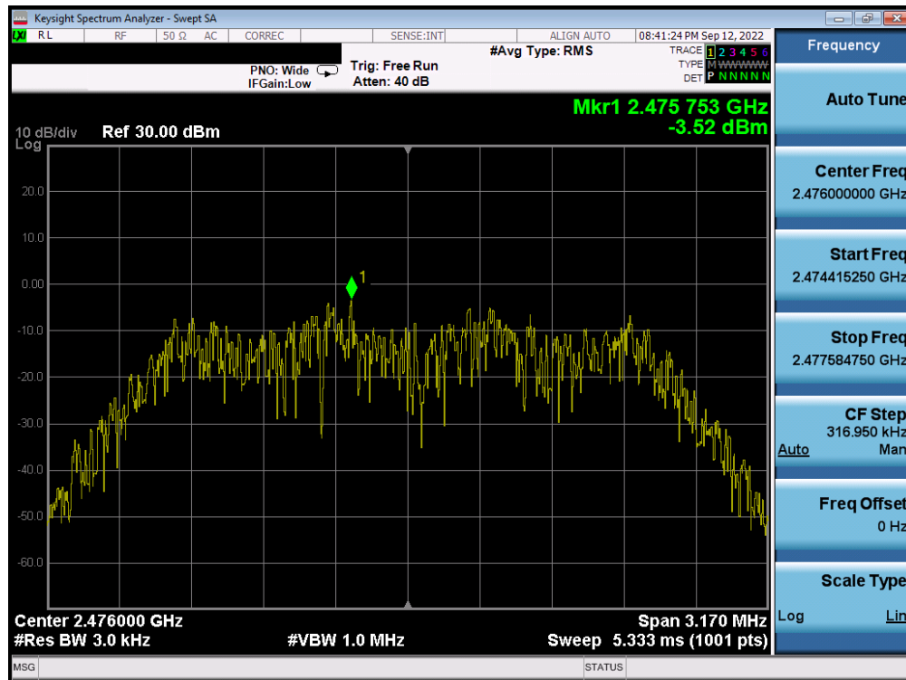
Plot 7-42. Power Spectral Density Plot Antenna 2a (Bluetooth (HDR4), 4Mbps, ePA – Ch. 73)
