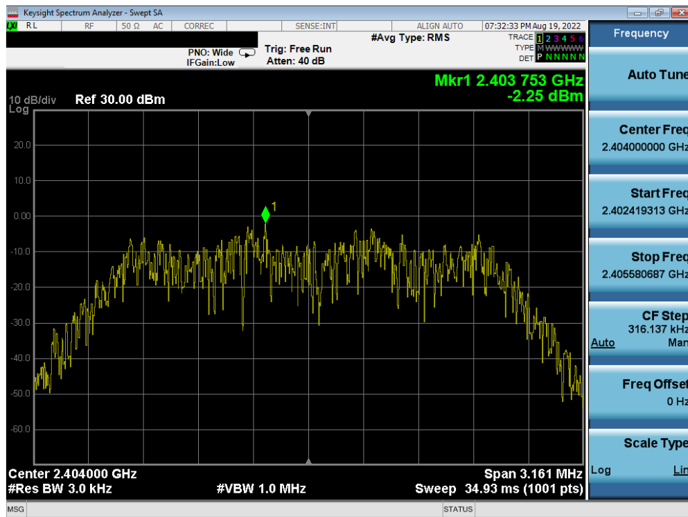
Plot 7-38. Power Spectral Density Plot Antenna 2a (Bluetooth (HDR4), 4Mbps, ePA – Ch. 1)
