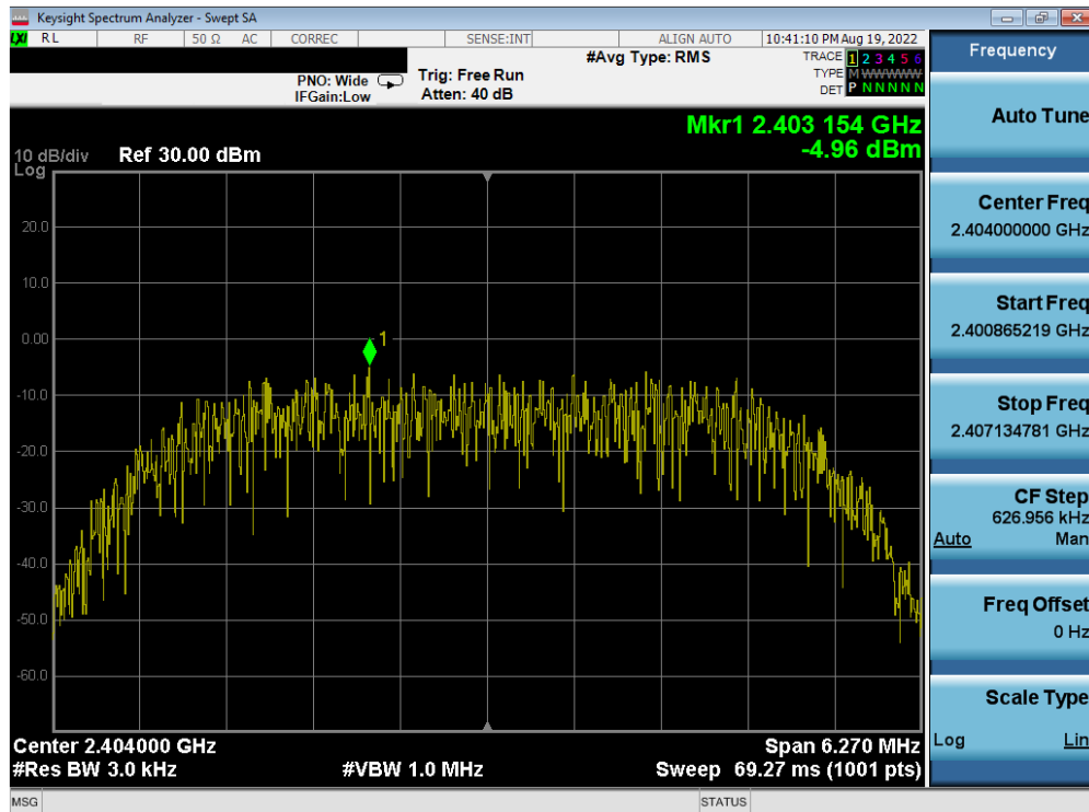
Plot 7-55. Power Spectral Density Plot Antenna 4a (Bluetooth (HDR8), 8Mbps, iPA – Ch. 1)
