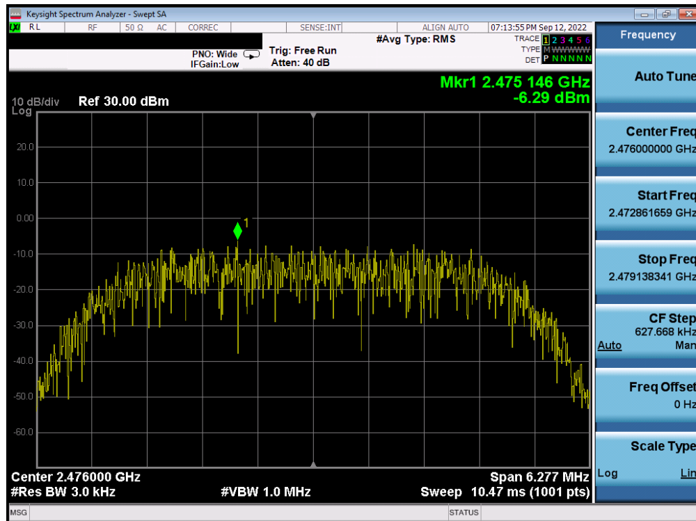
Plot 7-60. Power Spectral Density Plot Antenna 2a (Bluetooth (HDR8), 8Mbps, iPA – Ch. 73)
