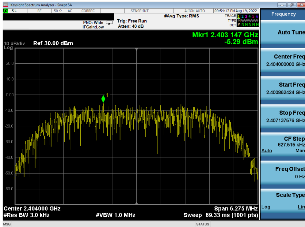
Plot 7-49. Power Spectral Density Plot Antenna 4a (Bluetooth (HDR8), 8Mbps, ePA – Ch. 1)
