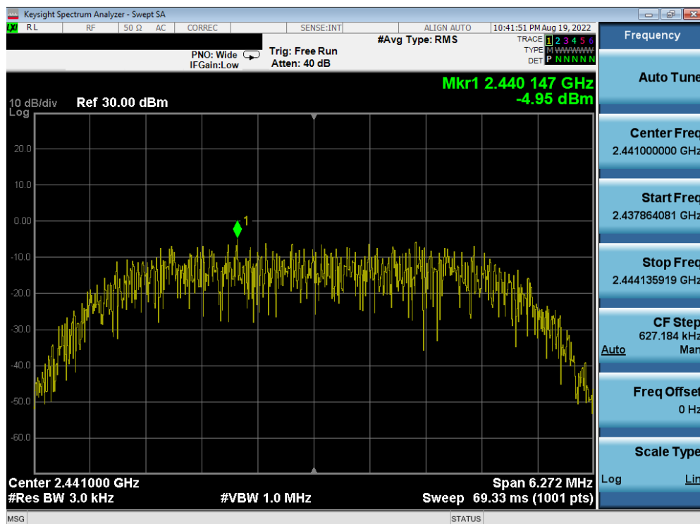
Plot 7-57. Power Spectral Density Plot Antenna 4a (Bluetooth (HDR8), 8Mbps, iPA – Ch. 38)
