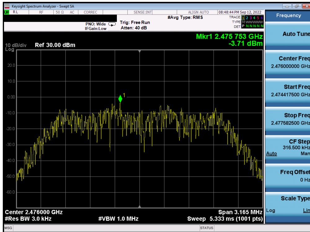
Plot 7-47. Power Spectral Density Plot Antenna 4a (Bluetooth (HDR4), 4Mbps, iPA – Ch. 73)
