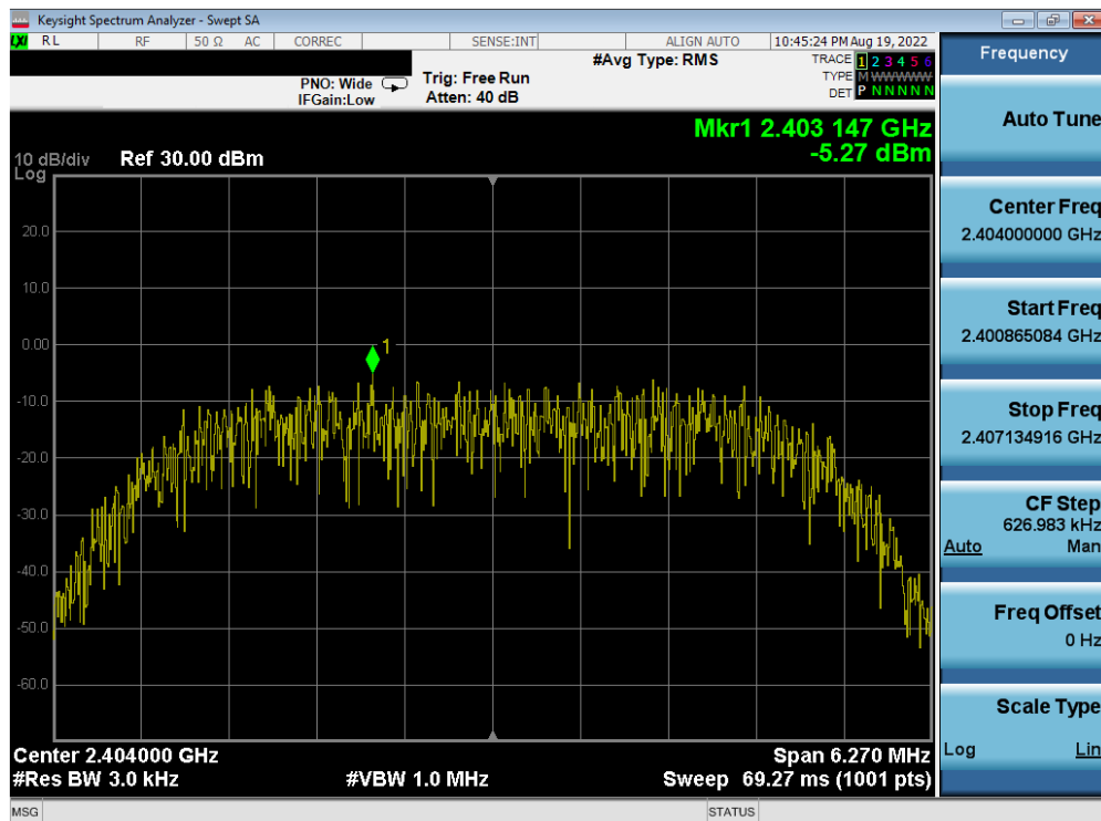
Plot 7-56. Power Spectral Density Plot Antenna 2a (Bluetooth (HDR8), 8Mbps, iPA – Ch. 1)
