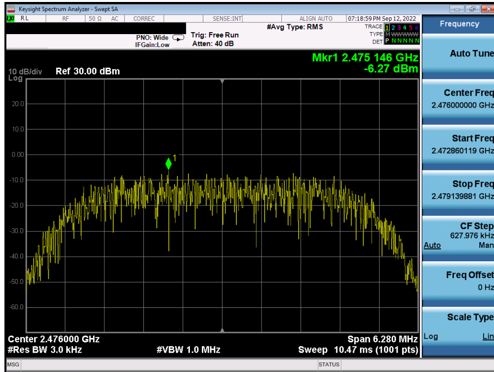
Plot 7-53. Power Spectral Density Plot Antenna 4a (Bluetooth (HDR8), 8Mbps, ePA – Ch. 73)
