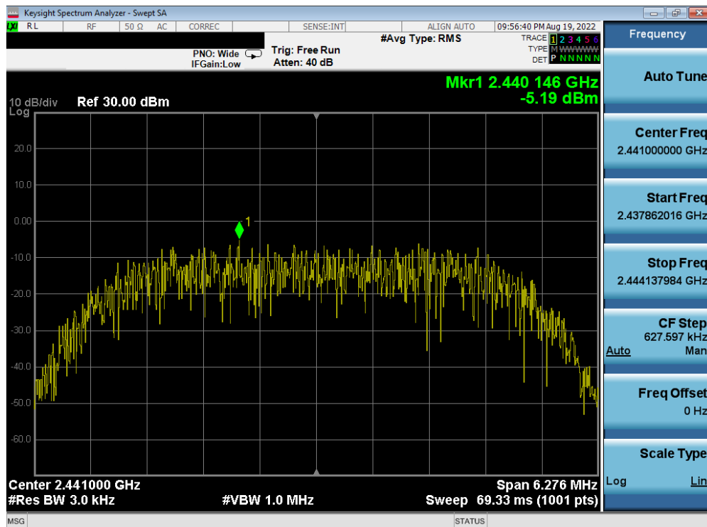
Plot 7-52. Power Spectral Density Plot Antenna 2a (Bluetooth (HDR8), 8Mbps, ePA – Ch. 38)
