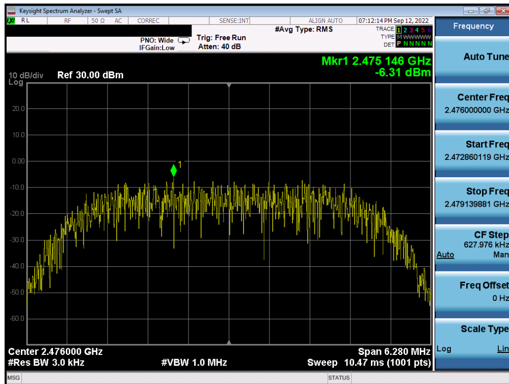
Plot 7-54. Power Spectral Density Plot Antenna 2a (Bluetooth (HDR8), 8Mbps, ePA – Ch. 73)
