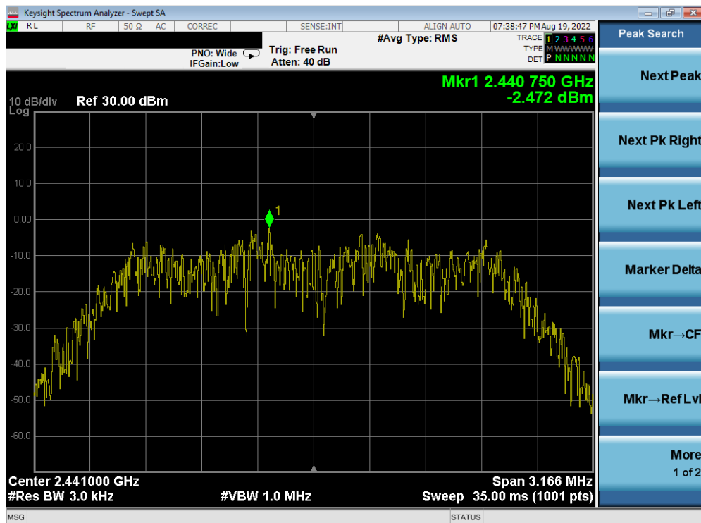
Plot 7-40. Power Spectral Density Plot Antenna 2a (Bluetooth (HDR4), 4Mbps, ePA – Ch. 38)
