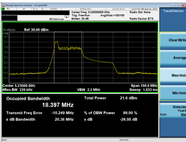
Plot 7-5. 26dB BW & 99% OBW Antenna WF5b (40MHz BW 11ax Index 0 – RU26 – Ch.46)
