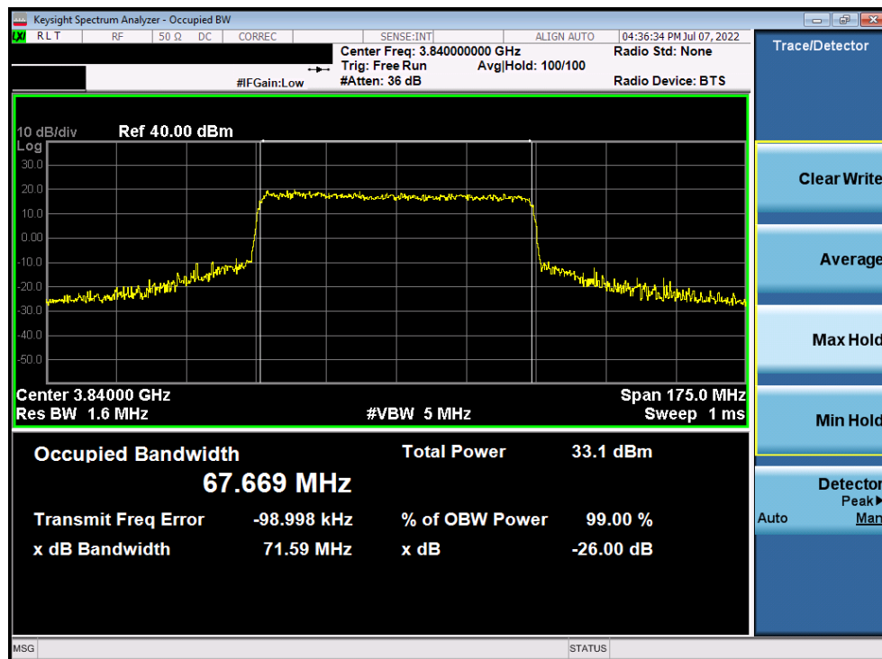
Plot 7-93. Occupied Bandwidth Plot (NR Band n77 C-Band - 70MHz CP-OFDM 16-QAM - Full RB)
