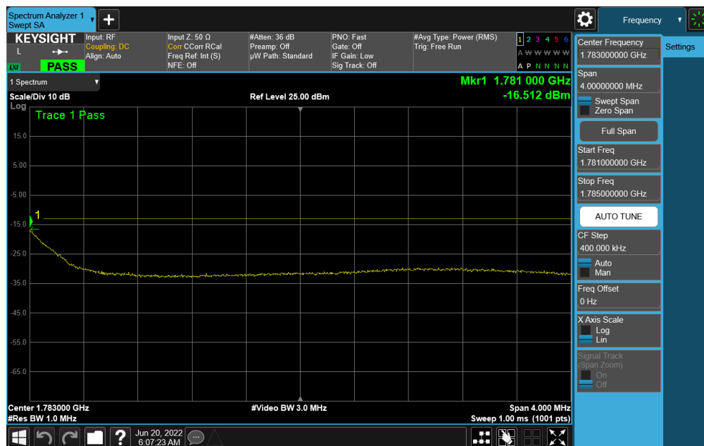
Plot 7-304. Upper Extended Band Edge Plot (NR Band n66 – 10.0MHz DFT-s-OFDM \pi/2 BPSK - Full RB)
