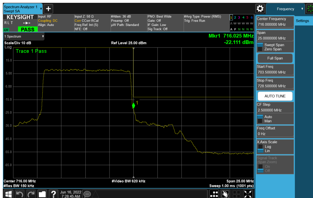
Plot 7-344. Upper Band Edge Plot (NR Band n12 – 10.0MHz DFT-s-OFDM \pi/2 BPSK - Full RB)
