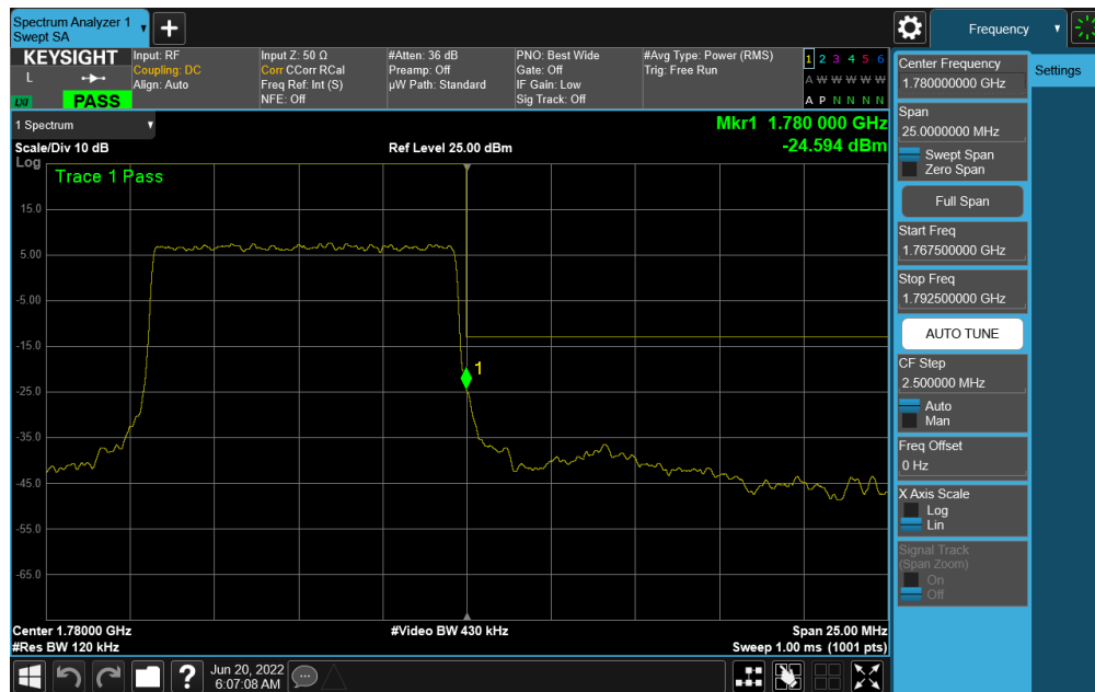
Plot 7-303. Upper Band Edge Plot (NR Band n66 – 10.0MHz DFT-s-OFDM \pi/2 BPSK - Full RB)
