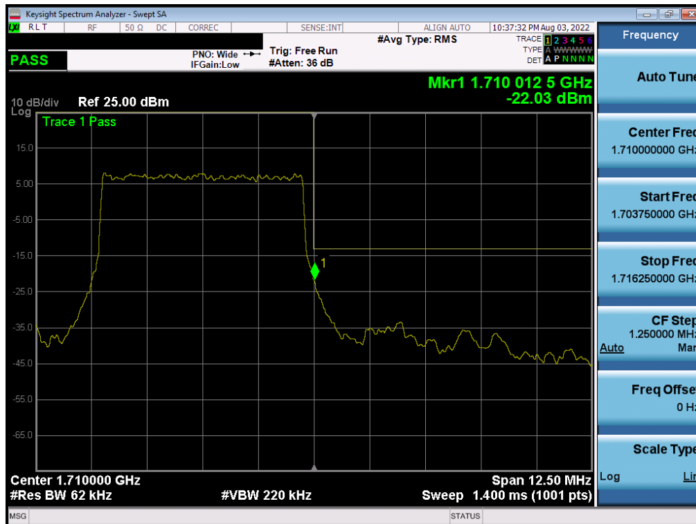
Plot 7-323. Upper Band Edge Plot (NR Band n70 – 5.0MHz DFT-s-OFDM \pi/2 BPSK - Full RB)
