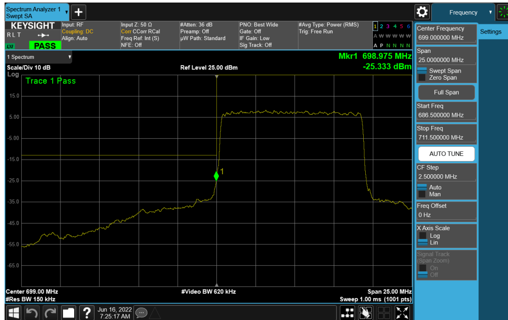
Plot 7-343. Lower Band Edge Plot (NR Band n12 – 10.0MHz DFT-s-OFDM \pi/2 BPSK - Full RB)
