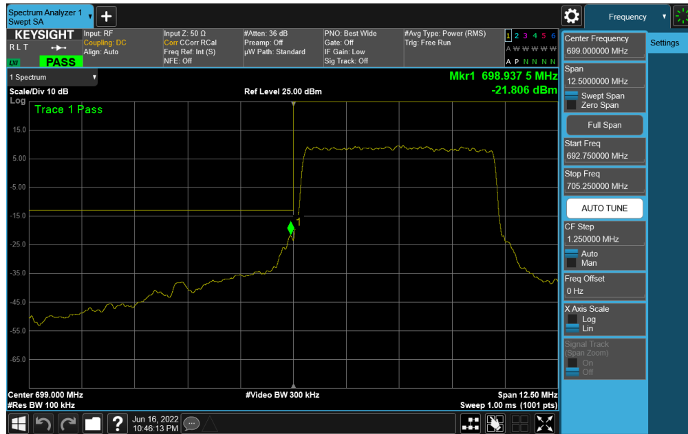
Plot 7-341. Lower Band Edge Plot (NR Band n12 – 5.0MHz DFT-s-OFDM \pi/2 BPSK - Full RB)
