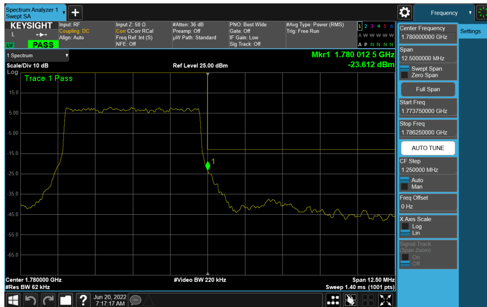
Plot 7-299. Upper Band Edge Plot (NR Band n66 – 5.0MHz DFT-s-OFDM \pi/2 BPSK - Full RB)
