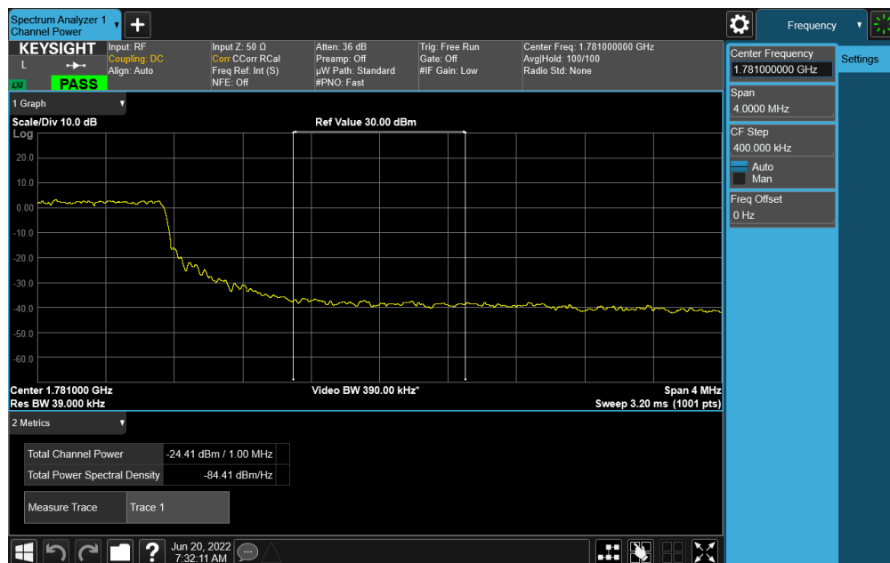
Plot 7-300. Upper Extended Band Edge Plot (NR Band n66 – 5.0MHz CP-OFDM \pi/2 BPSK - Full RB)
