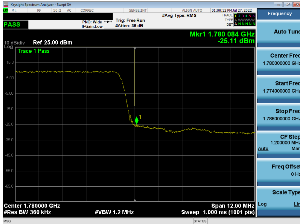
Plot 7-239. Upper Band Edge Plot (LTE Band 66 - 15MHz QPSK – Full RB)
