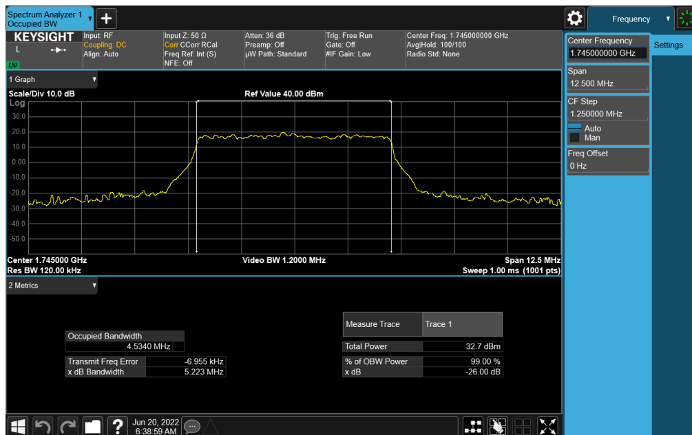
Plot 7-66. Occupied Bandwidth Plot (NR Band n66 - 5.0MHz DFT-s-OFDM QPSK - Full RB)
