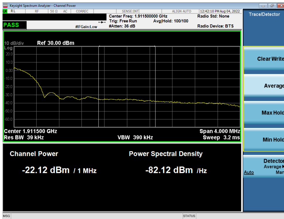
Plot 7-183. Extended Upper Band Edge Plot (WCDMA PCS – Ch. 9538)
