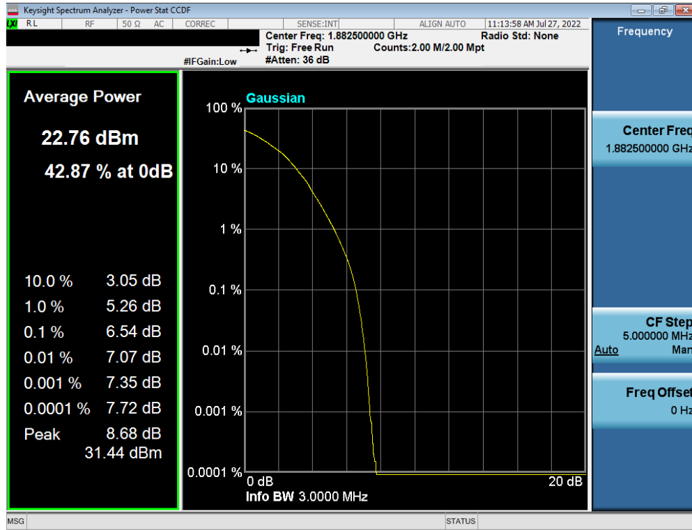
Plot 7-190. PAR Plot (LTE Band 25 - 3MHz 64-QAM - Full RB Configuration)
