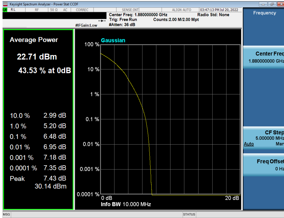
Plot 7-222. PAR Plot (LTE Band 2 - 10MHz 64-QAM - Full RB Configuration)
