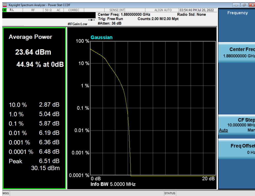
Plot 7-217. PAR Plot (LTE Band 2 - 5MHz 16-QAM - Full RB Configuration)
