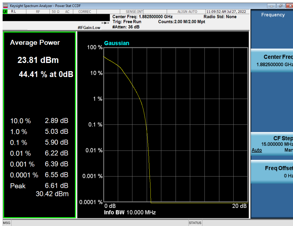
Plot 7-197. PAR Plot (LTE Band 25 - 10MHz 16-QAM - Full RB Configuration)
