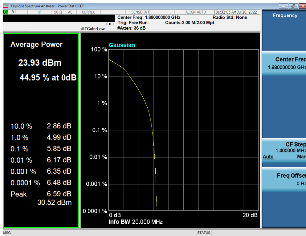
Plot 7-229. PAR Plot (LTE Band 2 - 20MHz 16-QAM - Full RB Configuration)
