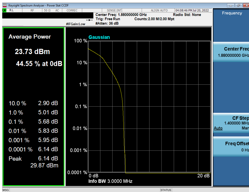
Plot 7-213. PAR Plot (LTE Band 2 - 3MHz 16-QAM - Full RB Configuration)
