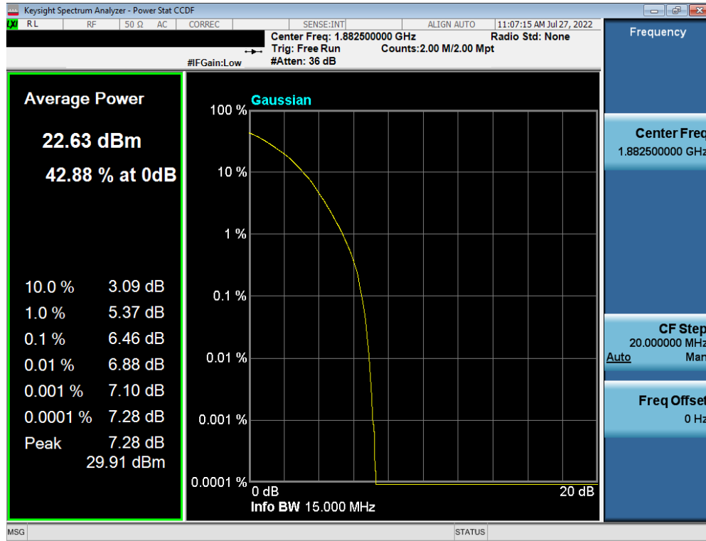
Plot 7-202. PAR Plot (LTE Band 25 - 15MHz 64-QAM - Full RB Configuration)
