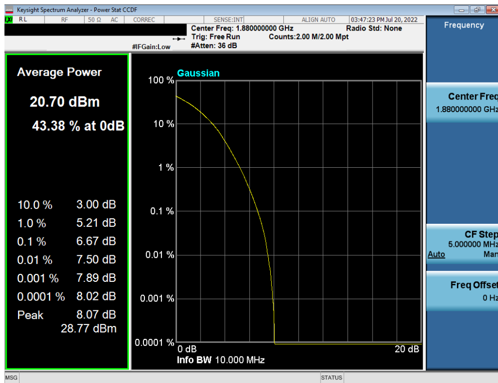
Plot 7-223. PAR Plot (LTE Band 2 - 10MHz 256-QAM - Full RB Configuration)
