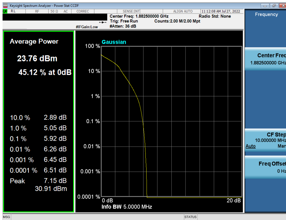
Plot 7-193. PAR Plot (LTE Band 25 - 5MHz 16-QAM - Full RB Configuration)
