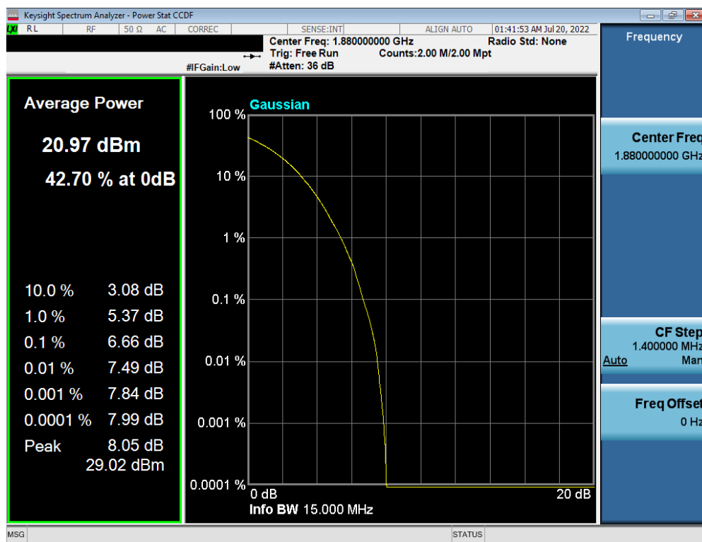
Plot 7-227. PAR Plot (LTE Band 2 - 15MHz 256-QAM - Full RB Configuration)
