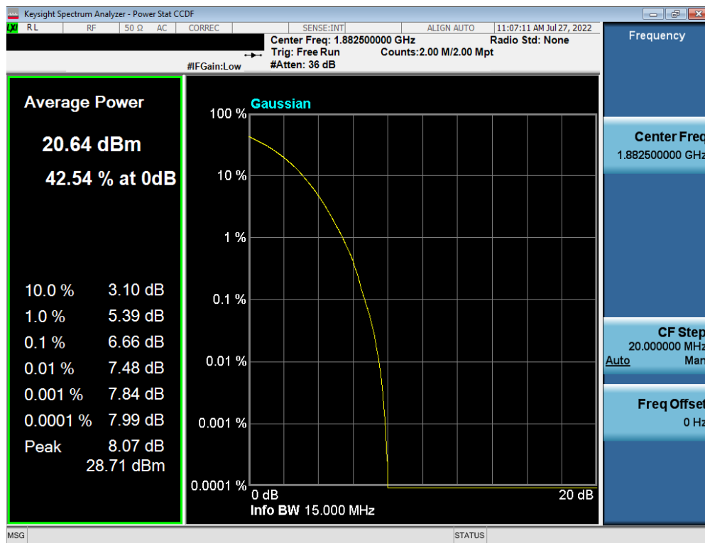
Plot 7-203. PAR Plot (LTE Band 25 - 15MHz 256-QAM - Full RB Configuration)
