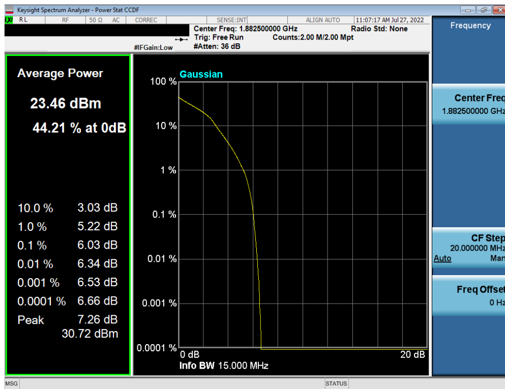
Plot 7-201. PAR Plot (LTE Band 25 - 15MHz 16-QAM - Full RB Configuration)
