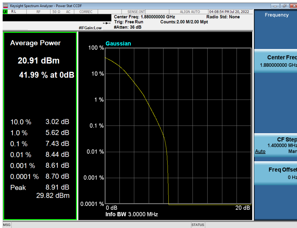
Plot 7-215. PAR Plot (LTE Band 2 - 3MHz 256-QAM - Full RB Configuration)
