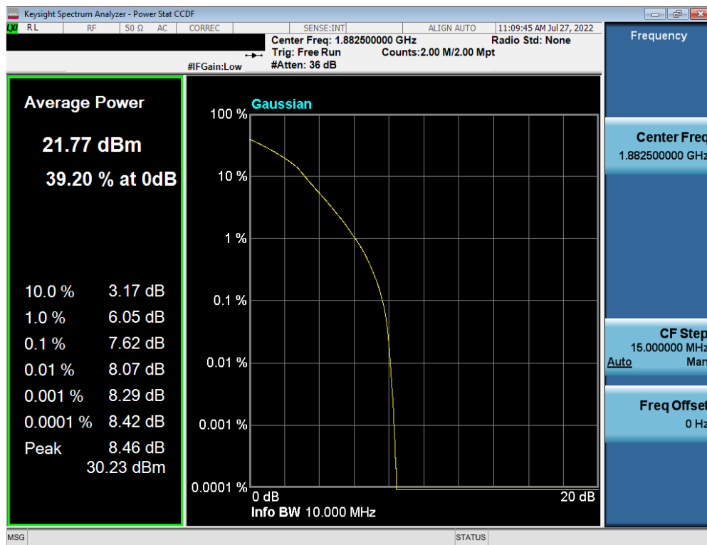
Plot 7-199. PAR Plot (LTE Band 25 - 10MHz 256-QAM - Full RB Configuration)
