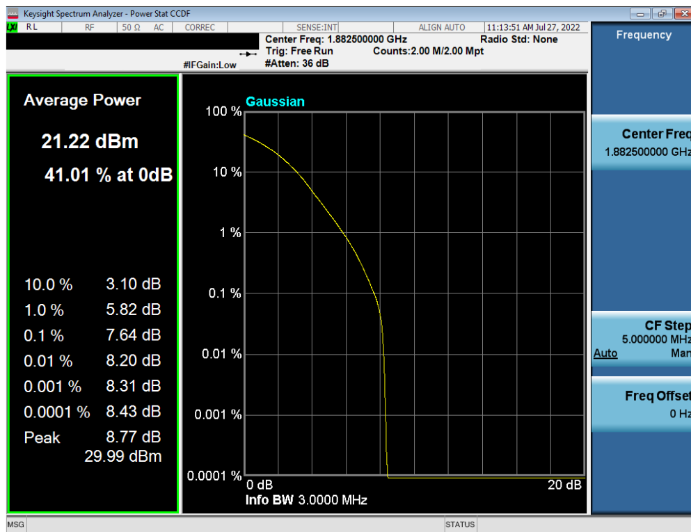
Plot 7-191. PAR Plot (LTE Band 25 - 3MHz 256-QAM - Full RB Configuration)
