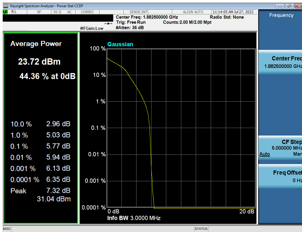
Plot 7-189. PAR Plot (LTE Band 25 - 3MHz 16-QAM - Full RB Configuration)
