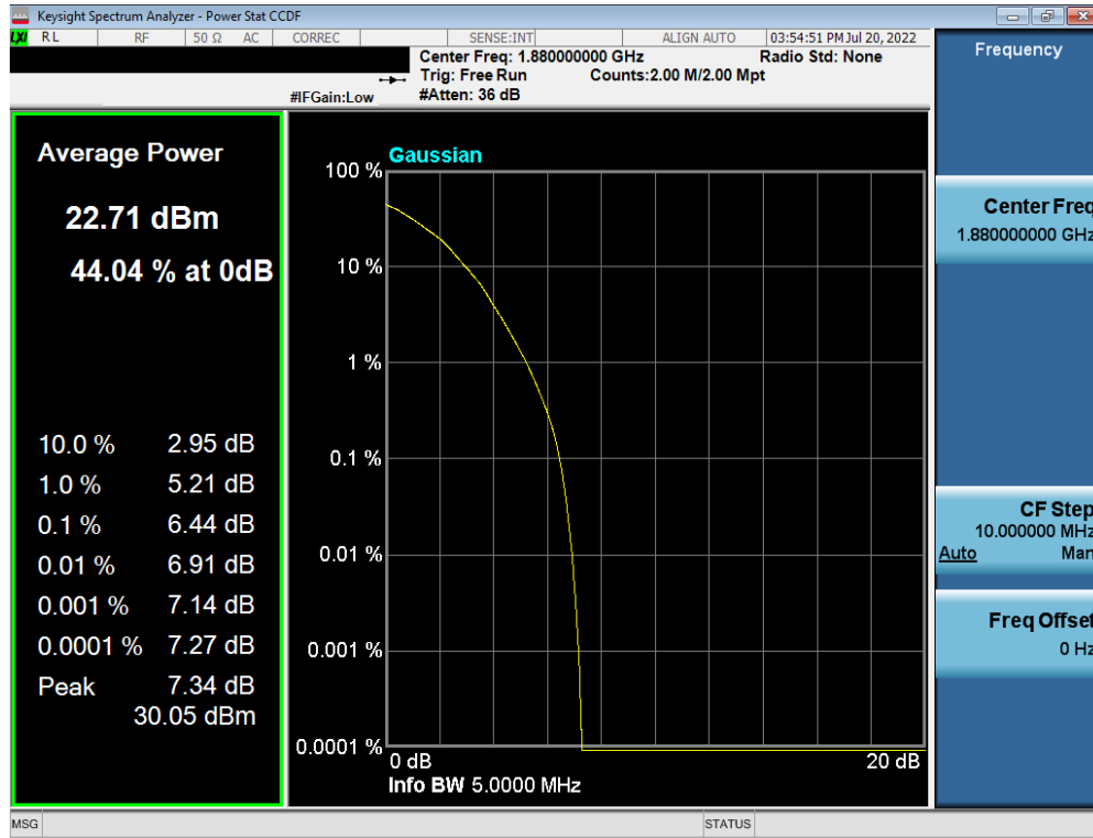
Plot 7-218. PAR Plot (LTE Band 2 - 5MHz 64-QAM - Full RB Configuration)
