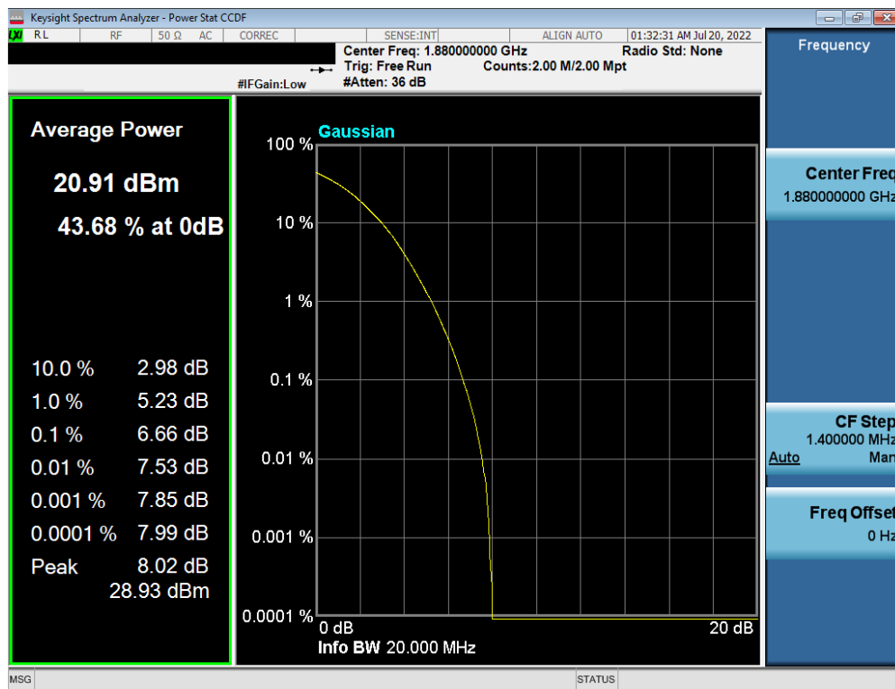
Plot 7-231. PAR Plot (LTE Band 2 - 20MHz 256-QAM - Full RB Configuration)
