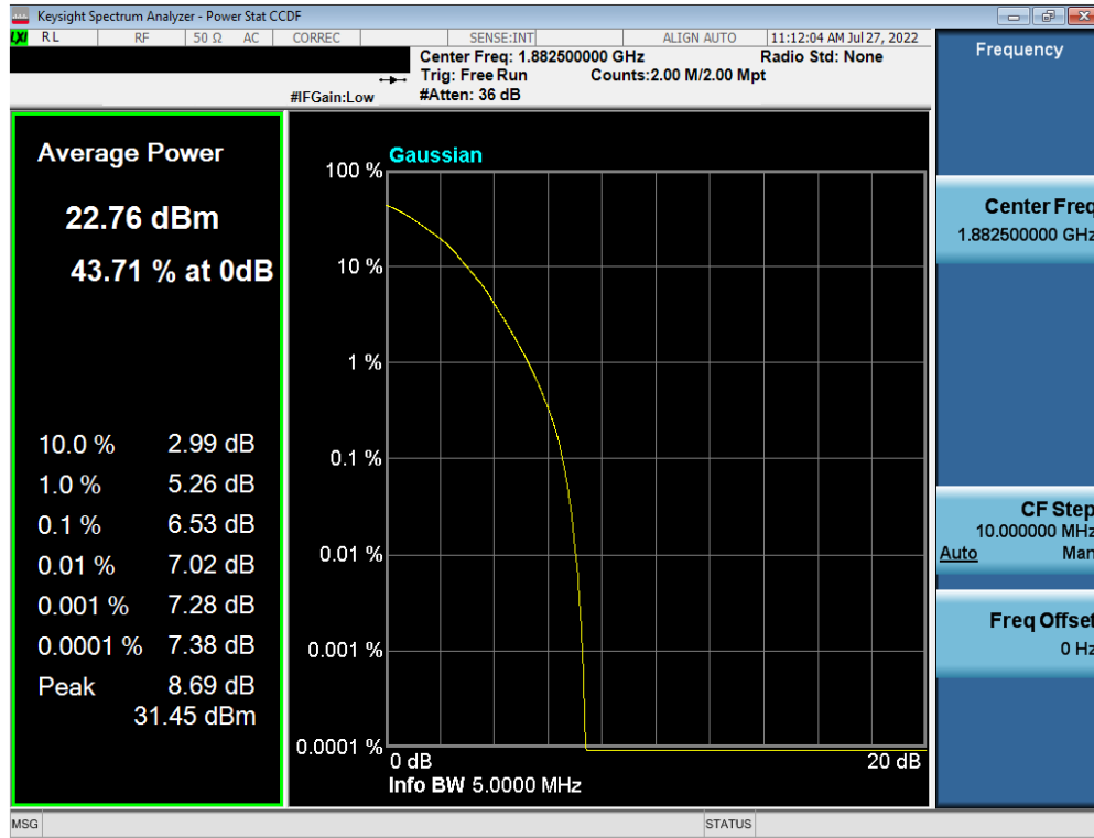
Plot 7-194. PAR Plot (LTE Band 25 - 5MHz 64-QAM - Full RB Configuration)
