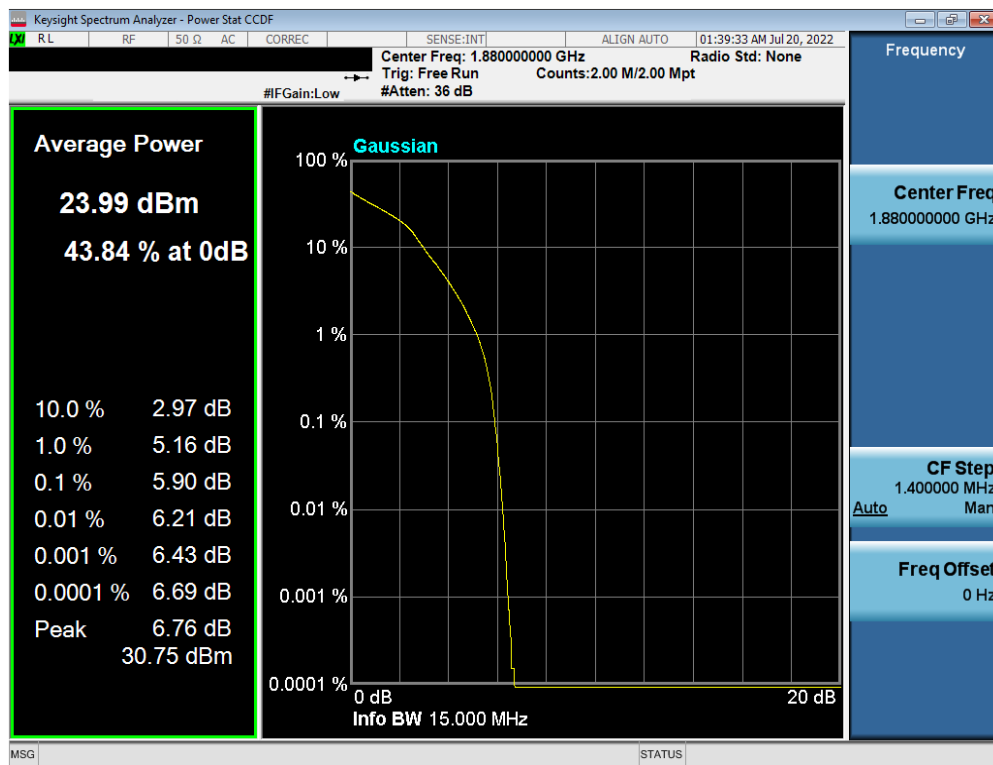
Plot 7-225. PAR Plot (LTE Band 2 - 15MHz 16-QAM - Full RB Configuration)
