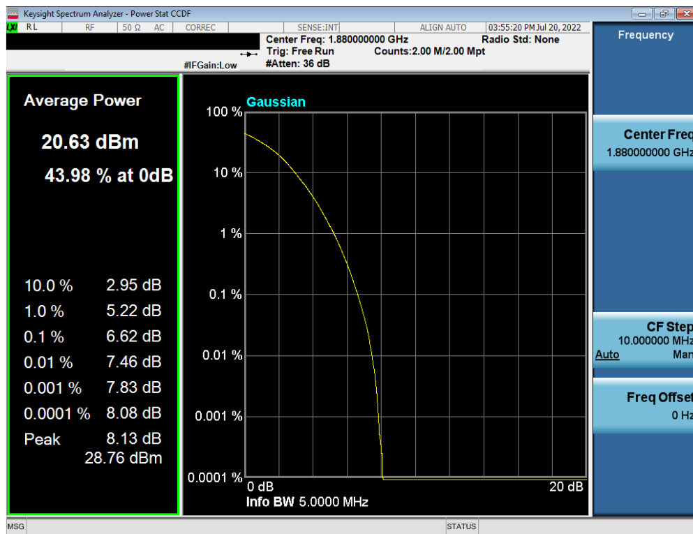
Plot 7-219. PAR Plot (LTE Band 2 - 5MHz 256-QAM - Full RB Configuration)
