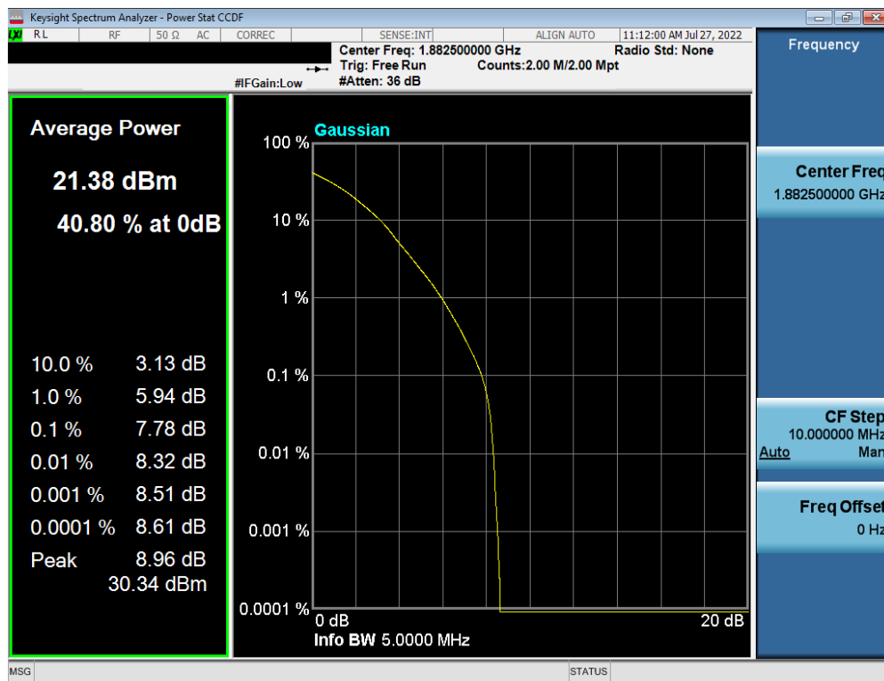
Plot 7-195. PAR Plot (LTE Band 25 - 5MHz 256-QAM - Full RB Configuration)
