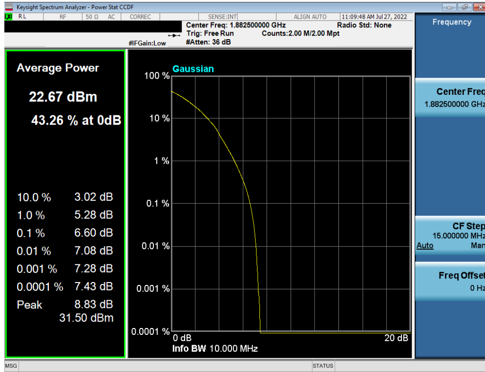
Plot 7-198. PAR Plot (LTE Band 25 - 10MHz 64-QAM - Full RB Configuration)
