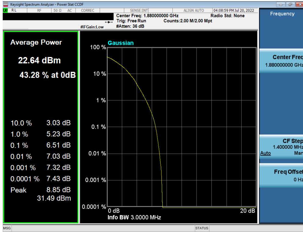
Plot 7-214. PAR Plot (LTE Band 2 - 3MHz 64-QAM - Full RB Configuration)
