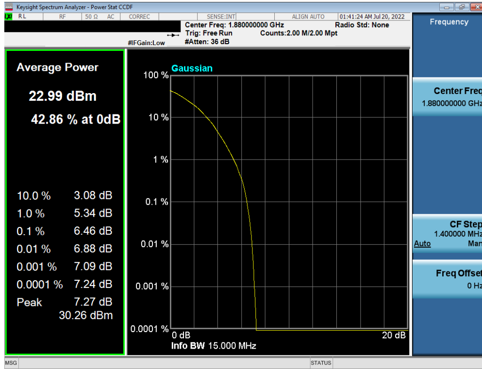
Plot 7-226. PAR Plot (LTE Band 2 - 15MHz 64-QAM - Full RB Configuration)
