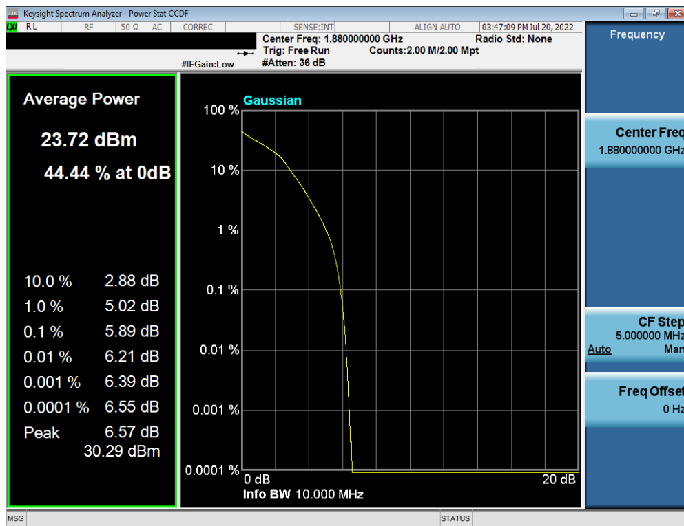
Plot 7-221. PAR Plot (LTE Band 2 - 10MHz 16-QAM - Full RB Configuration)
