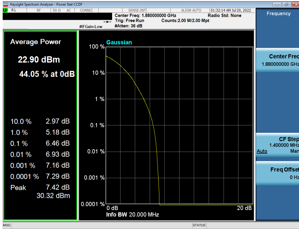
Plot 7-230. PAR Plot (LTE Band 2 - 20MHz 64-QAM - Full RB Configuration)
