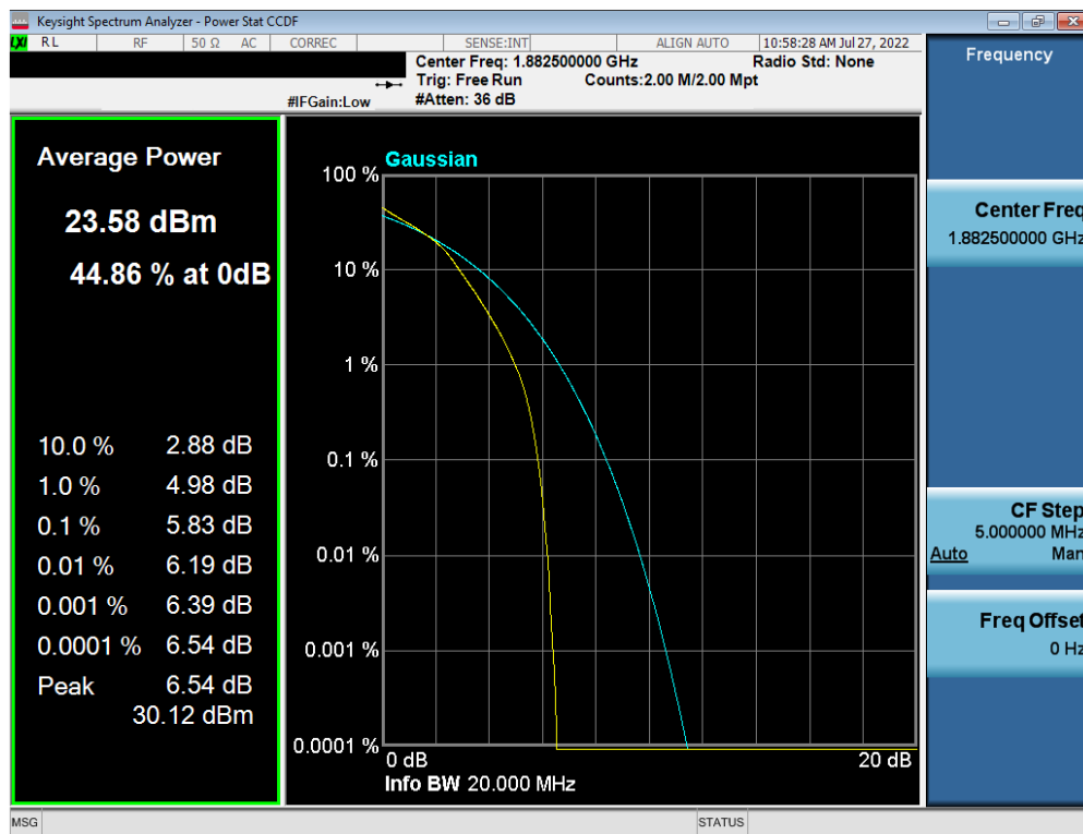
Plot 7-205. PAR Plot (LTE Band 25 - 20MHz 16-QAM - Full RB Configuration)
