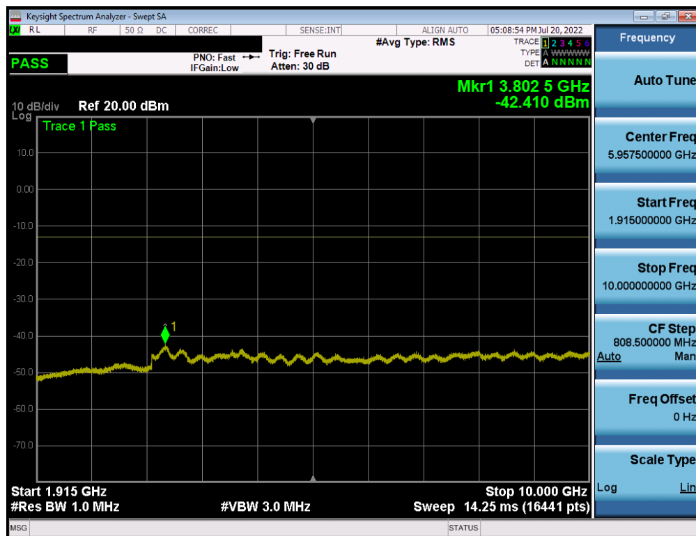
Plot 7-77. Conducted Spurious Plot (NR Band n25/n2 - 40.0MHz DFT-s-OFDM QPSK - RB Size 1, RB Offset 0 - High Channel)
