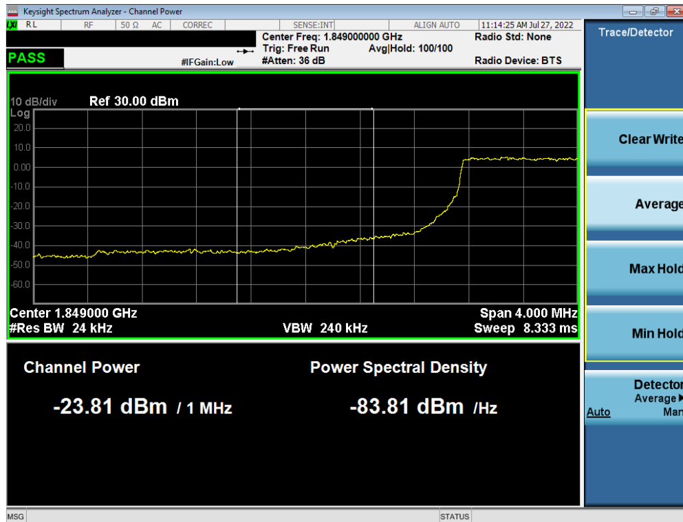
Plot 7-93. Extended Lower Band Edge Plot (LTE Band 25 – 3MHz QPSK – Full RB Configuration)
