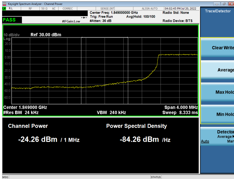
Plot 7-117. Extended Lower Band Edge Plot (LTE Band 2 – 3MHz QPSK – Full RB Configuration)
