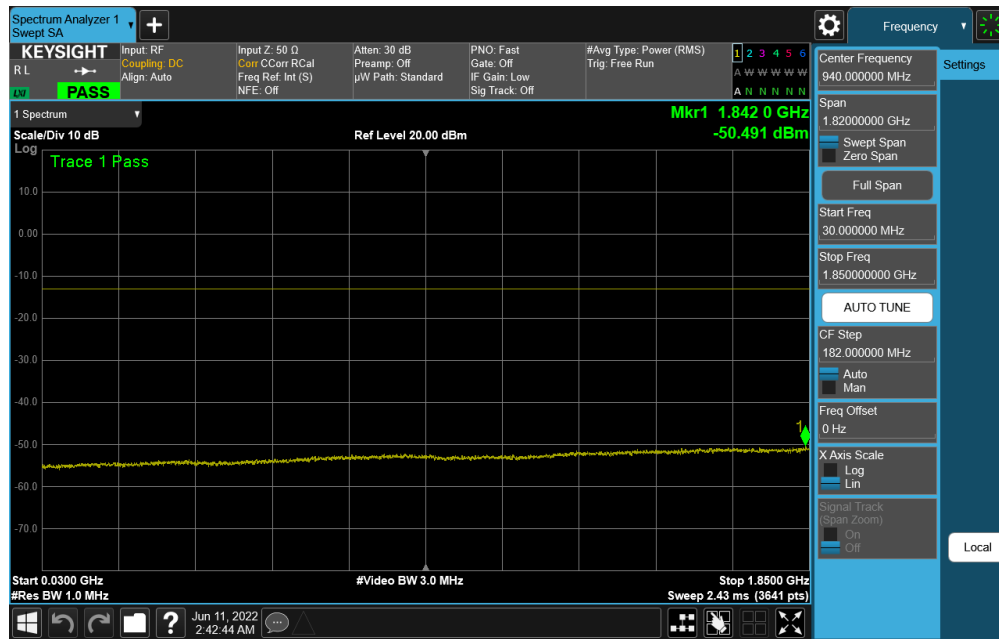
Plot 7-76. Conducted Spurious Plot (NR Band n25/n2 - 40.0MHz DFT-s-OFDM QPSK - RB Size 1, RB Offset 0 - High Channel)
