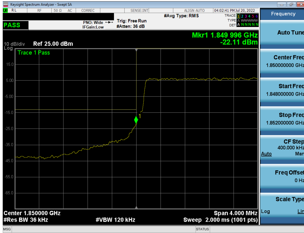
Plot 7-116. Lower Band Edge Plot (LTE Band 2 – 3MHz QPSK – Full RB Configuration)
