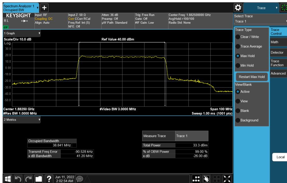
Plot 7-56. Occupied Bandwidth Plot (NR Band n25 - 40.0MHz DFT-s-OFDM QPSK - Full RB)
