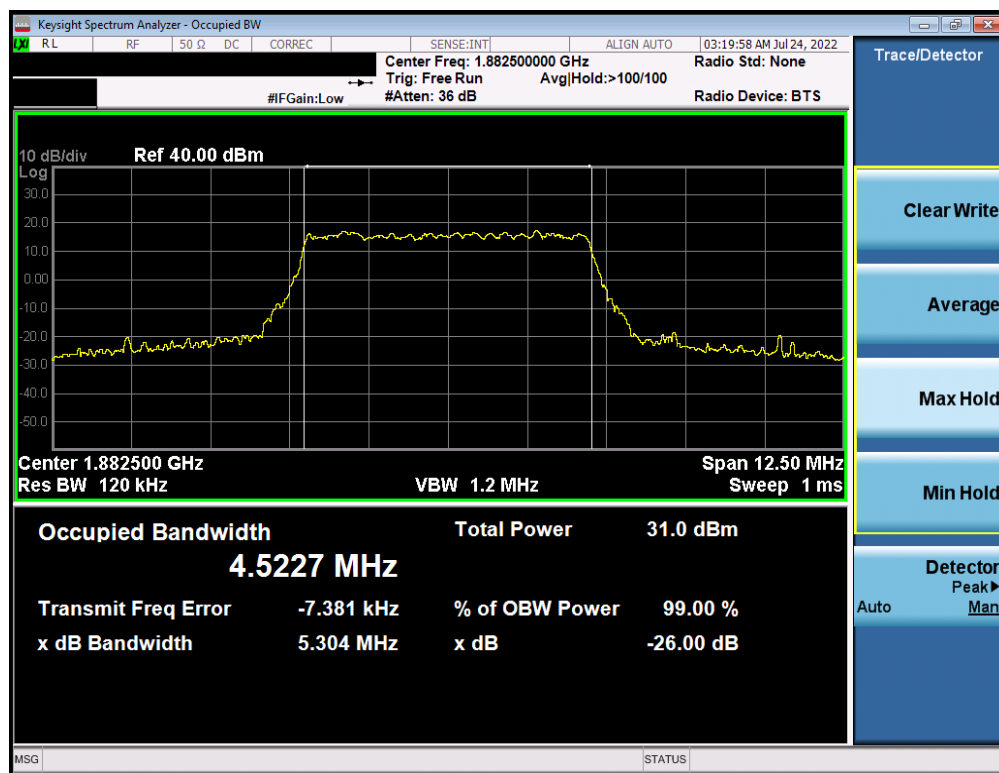
Plot 7-28. Occupied Bandwidth Plot (NR Band n25/n2 - 5.0MHz CP-OFDM 64QAM - Full RB)
