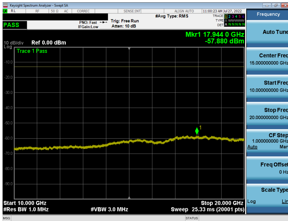
Plot 7-69. Conducted Spurious Plot (LTE Band 25/2 - 20MHz QPSK - RB Size 1, RB Offset 0 - High Channel)
