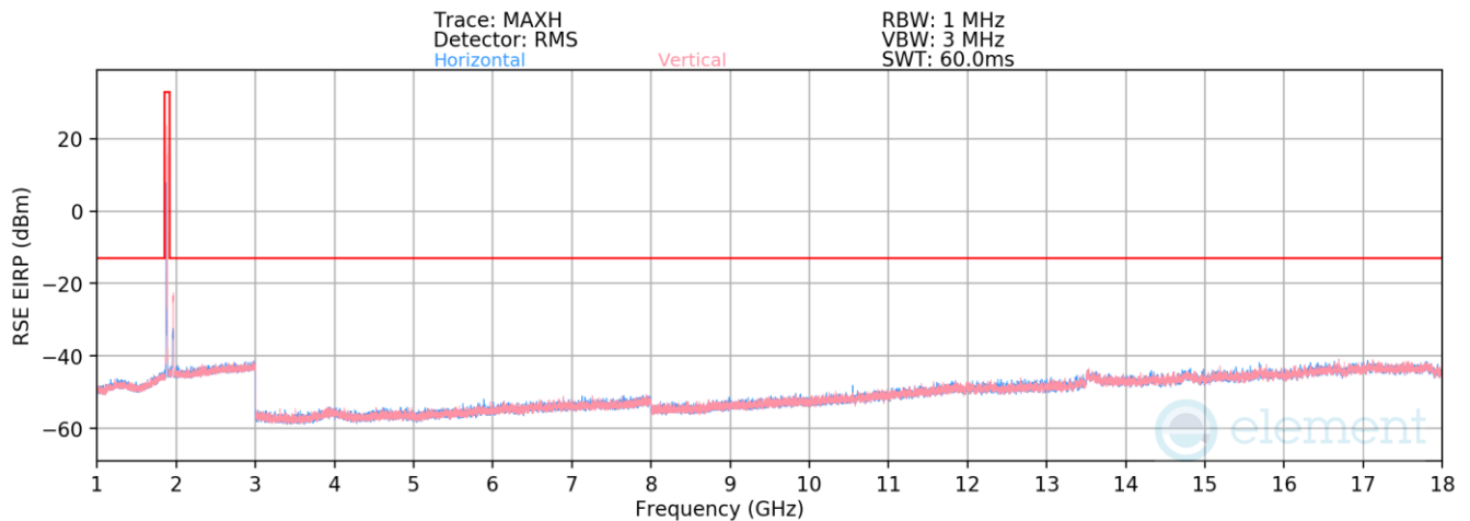
Plot 7-2. Antenna 4b Radiated Spurious Emission above 1GHz (LTE Band 2)
