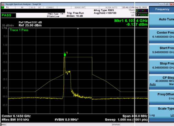
Plot 7-392. In-Band Emission Plot Antenna WF5t (80MHz 802.11ax RU26 (UNII Band 5) – Ch. 39)
