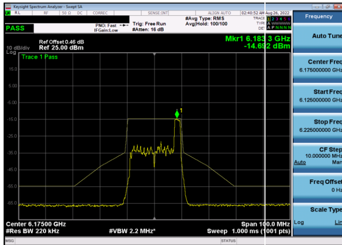
Plot 7-386. In-Band Emission Plot Antenna WF5t (20MHz 802.11ax RU26 (UNII Band 5) – Ch. 45)
