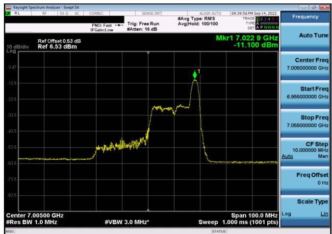
Plot 7-364. Power Spectral Density Plot SDM Antenna WF5t (40MHz 802.11ax RU26 (UNII Band 8) – Ch. 211)
