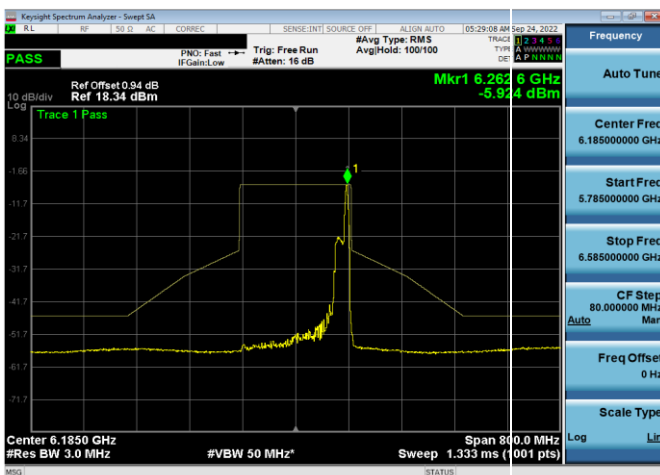
Plot 7-398. In-Band Emission Plot Antenna WF5t (160MHz 802.11ax RU26 (UNII Band 5) – Ch. 47)
