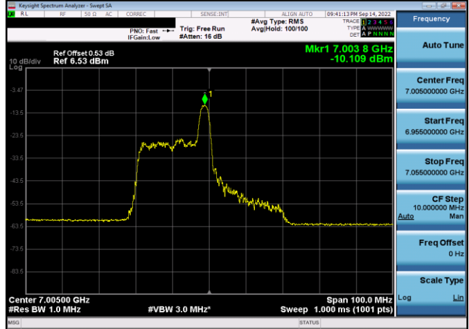
Plot 7-362. Power Spectral Density Plot SDM Antenna WF5t (40MHz 802.11ax RU26 (UNII Band 8) – Ch. 211)
