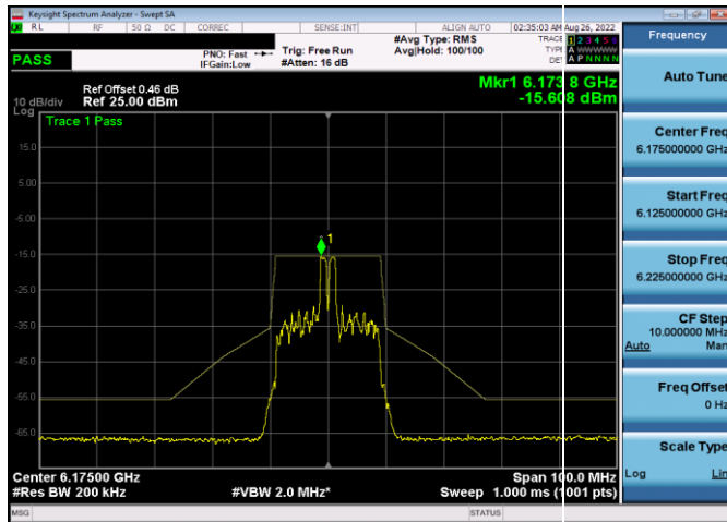
Plot 7-385. In-Band Emission Plot Antenna WF5t (20MHz 802.11ax RU26 (UNII Band 5) – Ch. 45)
