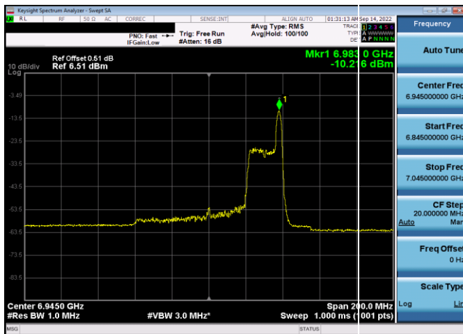
Plot 7-373. Power Spectral Density Plot SDM Antenna WF5b (80MHz 802.11ax RU26 (UNII Band 8) – Ch. 199)
