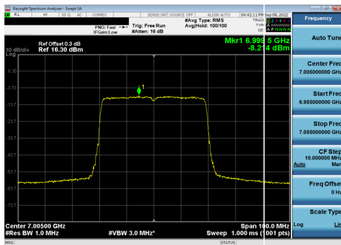
Plot 7-367. Power Spectral Density Plot SDM Antenna WF5b (40MHz 802.11ax RU484 (UNII Band 8) – Ch. 211)
