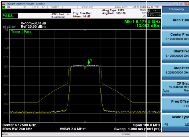
Plot 7-338. In-Band Emission Plot Antenna WF5t (20MHz 802.11ax (UNII Band 5) – Ch. 45, MCS2)
