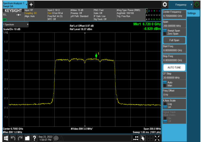
Plot 7-326. Power Spectral Density Plot SDM Antenna WF5b (80MHz 802.11ax (UNII Band 7) – Ch. 151, MCS11)
