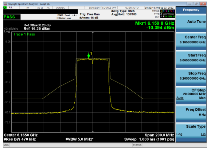
Plot 7-339. In-Band Emission Plot Antenna WF5t (40MHz 802.11ax (UNII Band 5) – Ch. 43, MCS2)
