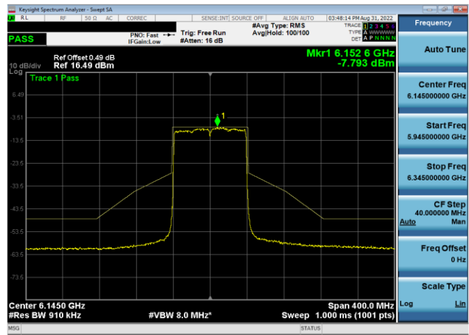
Plot 7-340. In-Band Emission Plot Antenna WF5t (80MHz 802.11ax (UNII Band 5) – Ch. 39, MCS2)
