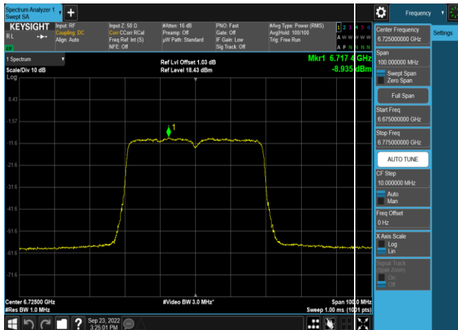
Plot 7-324. Power Spectral Density Plot SDM Antenna WF5b (40MHz 802.11ax (UNII Band 7) – Ch. 155, MCS11)
