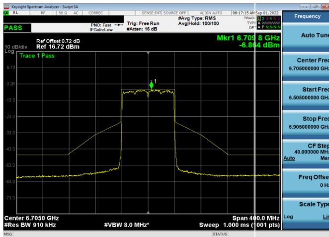
Plot 7-370. In-Band Emission Plot Antenna WF5t (80MHz 802.11ax (UNII Band 7) - Ch. 151, MCS4)
