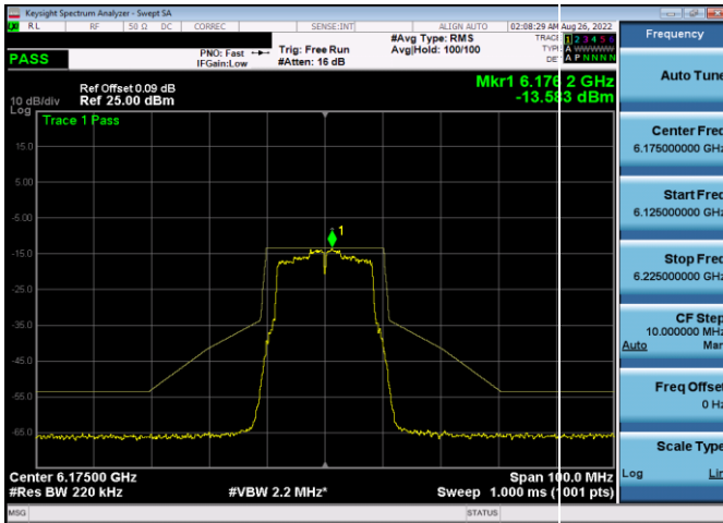
Plot 7-337. In-Band Emission Plot Antenna WF5t (20MHz 802.11a (UNII Band 5) – Ch. 45, MCS2)
