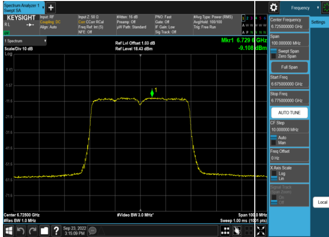
Plot 7-323. Power Spectral Density Plot SDM Antenna WF5t (40MHz 802.11ax (UNII Band 7) – Ch. 155, MCS11)
