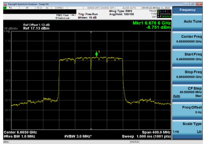
Plot 7-327. Power Spectral Density Plot SDM Antenna WF5t (160MHz 802.11ax (UNII Band 7) – Ch. 143, MCS11)
