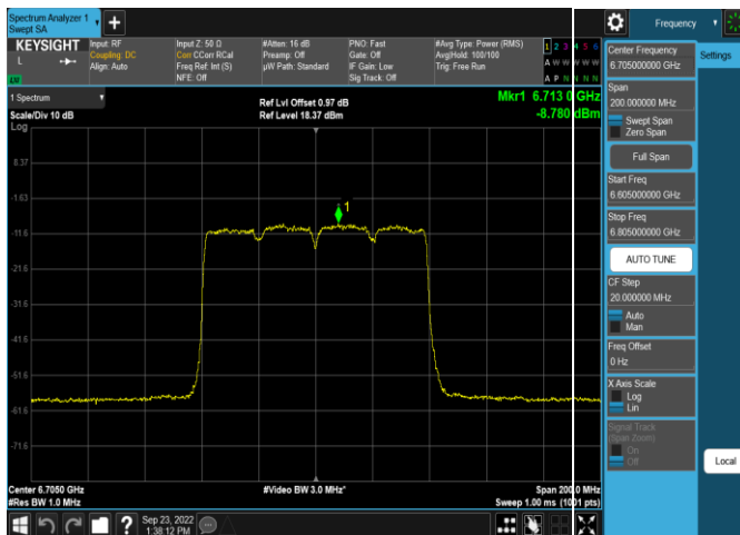
Plot 7-325. Power Spectral Density Plot SDM Antenna WF5t (80MHz 802.11ax (UNII Band 7) – Ch. 151, MCS11)
