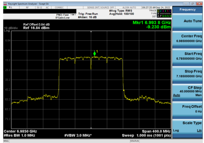
Plot 7-336. Power Spectral Density Plot SDM Antenna WF5b (160MHz 802.11ax (UNII Band 8) – Ch. 207, MCS11)
