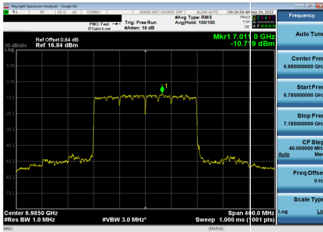
Plot 7-335. Power Spectral Density Plot SDM Antenna WF5t (160MHz 802.11ax (UNII Band 8) – Ch. 207, MCS11)
