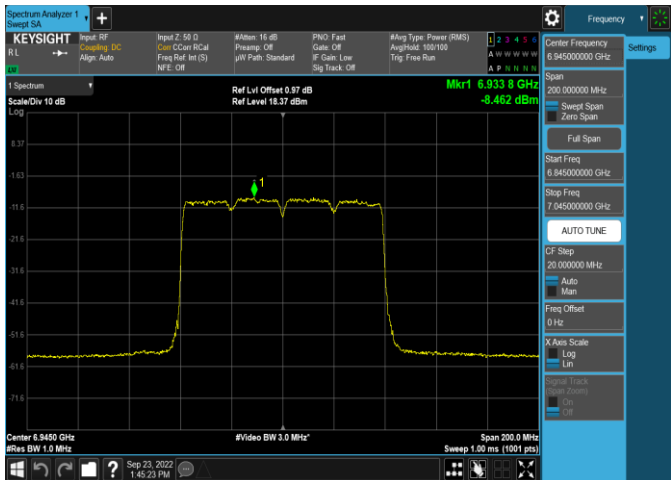
Plot 7-333. Power Spectral Density Plot SDM Antenna WF5t (80MHz 802.11ax (UNII Band 8) – Ch. 199, MCS11)
