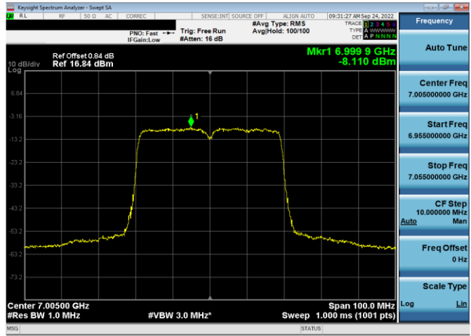
Plot 7-332. Power Spectral Density Plot SDM Antenna WF5b (40MHz 802.11ax (UNII Band 8) – Ch. 211, MCS11)
