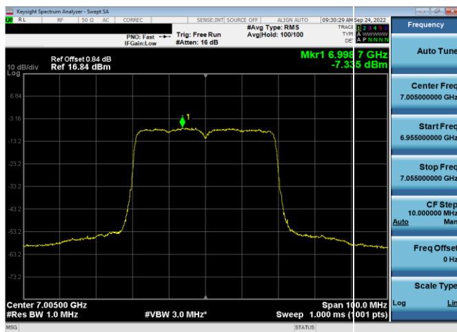
Plot 7-331. Power Spectral Density Plot SDM Antenna WF5t (40MHz 802.11ax (UNII Band 8) – Ch. 211, MCS11)
