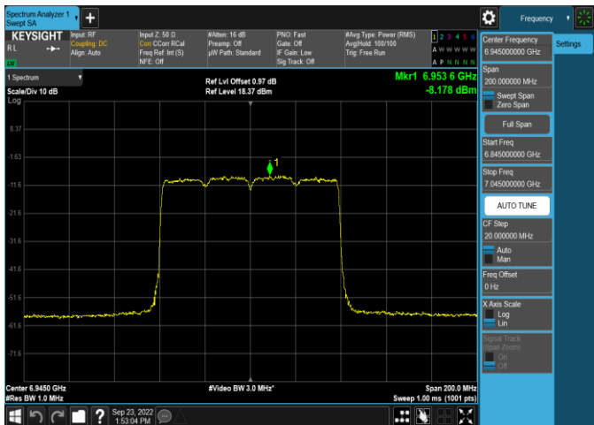
Plot 7-334. Power Spectral Density Plot SDM Antenna WF5b (80MHz 802.11ax (UNII Band 8) – Ch. 199, MCS11)
