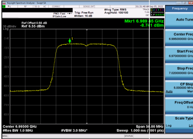
Plot 7-329. Power Spectral Density Plot SDM Antenna WF5t (20MHz 802.11ax (UNII Band 8) – Ch. 209, MCS11)
