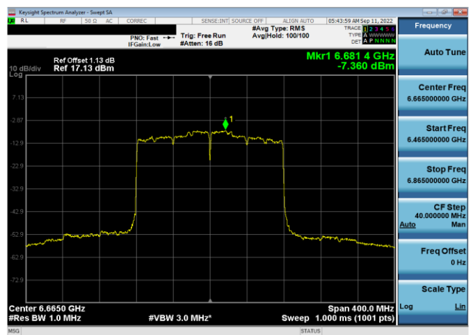
Plot 7-328. Power Spectral Density Plot SDM Antenna WF5b (160MHz 802.11ax (UNII Band 7) – Ch. 143, MCS11)
