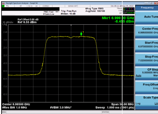
Plot 7-330. Power Spectral Density Plot SDM Antenna WF5b (20MHz 802.11ax (UNII Band 8) – Ch. 209, MCS11)
