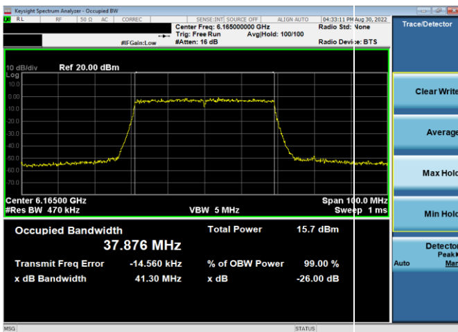
Plot 7-103. 26dB & 99% Bandwidth Plot Antenna WF5t (40MHz 802.11ax (UNII Band 5) – Ch. 43, MCS11)
