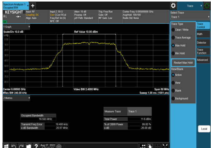
Plot 7-11. 26dB & 99% Bandwidth Plot Antenna WF5t (20MHz 802.11a (UNII Band 7) – Ch. 149, 12Mbps)
