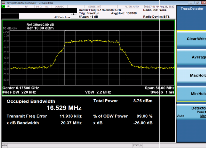
Plot 7-1. 26dB & 99% Bandwidth Plot Antenna WF5t (20MHz 802.11a (UNII Band 5) – Ch. 45, 12Mbps)
