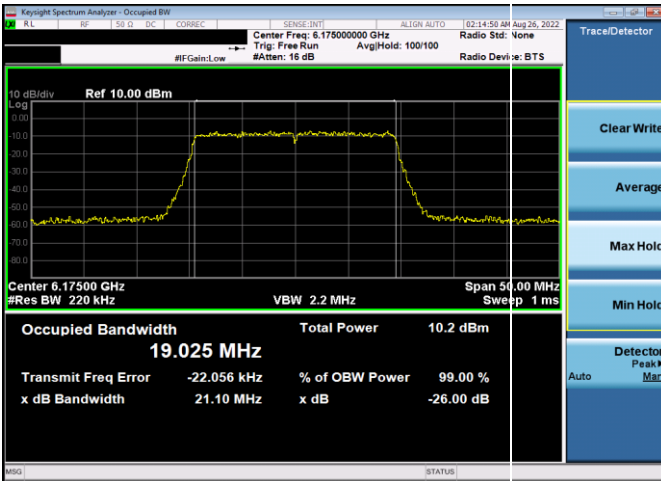
Plot 7-22. 26dB & 99% Bandwidth Plot Antenna WF5t (20MHz 802.11ax (UNII Band 5) – Ch. 45, MCS4)
