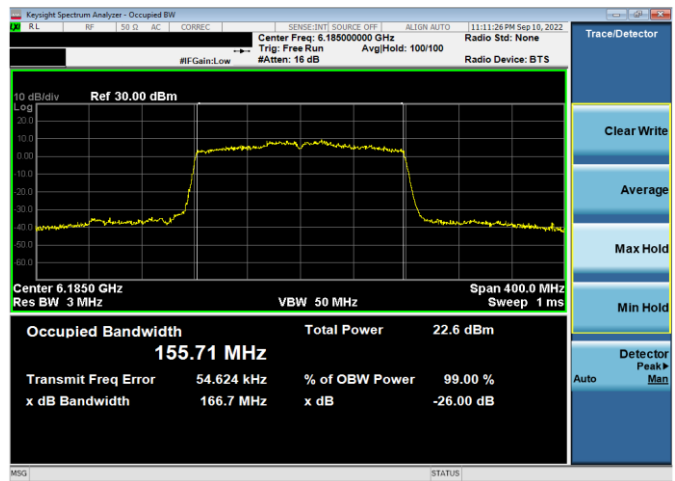
Plot 7-45. 26dB & 99% Bandwidth Plot Antenna WF5t (160MHz 802.11ax (UNII Band 5) – Ch. 47, MCS11)
