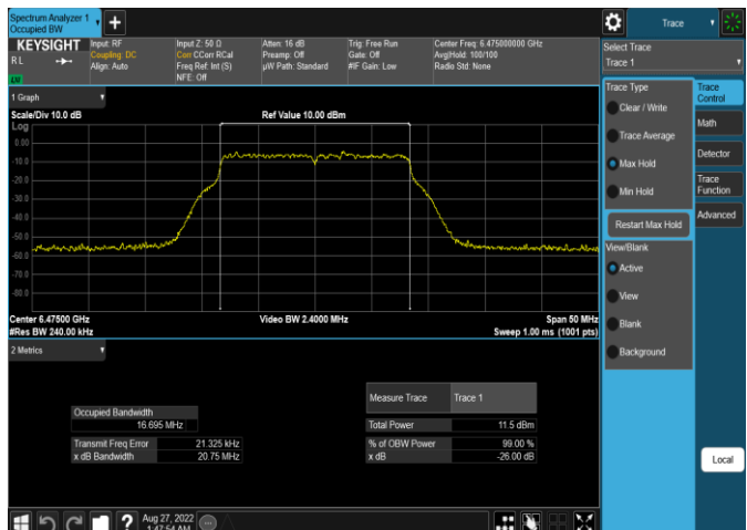
Plot 7-46. 26dB & 99% Bandwidth Plot Antenna WF5t (20MHz 802.11a (UNII Band 6) – Ch. 105, 54Mbps)
