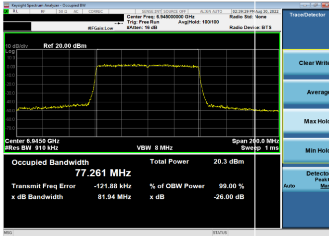
Plot 7-39. 26dB & 99% Bandwidth Plot Antenna WF5t (80MHz 802.11ax (UNII Band 8) – Ch. 199, MCS4)
