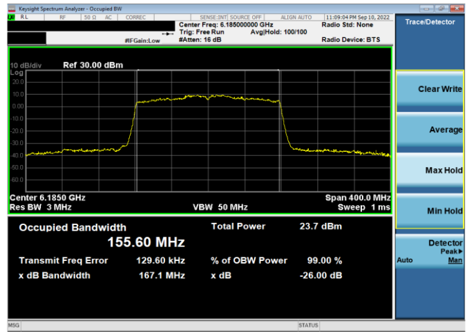
Plot 7-5. 26dB & 99% Bandwidth Plot Antenna WF5t (160MHz 802.11ax (UNII Band 5) – Ch. 47, MCS2)
