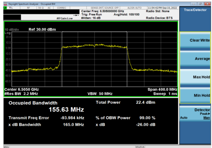
Plot 7-30. 26dB & 99% Bandwidth Plot Antenna WF5t (160MHz 802.11ax (UNII Band 6) – Ch. 111, MCS4)
