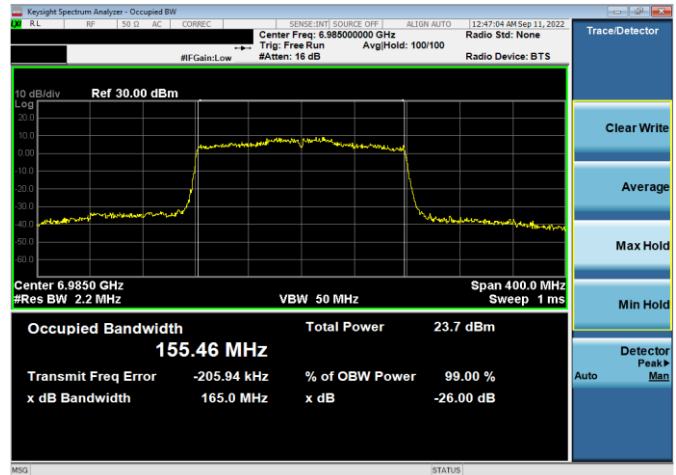
Plot 7-60. 26dB & 99% Bandwidth Plot Antenna WF5t (160MHz) 802.11ax (UNII Band 8) – Ch. 207, MCS11)
