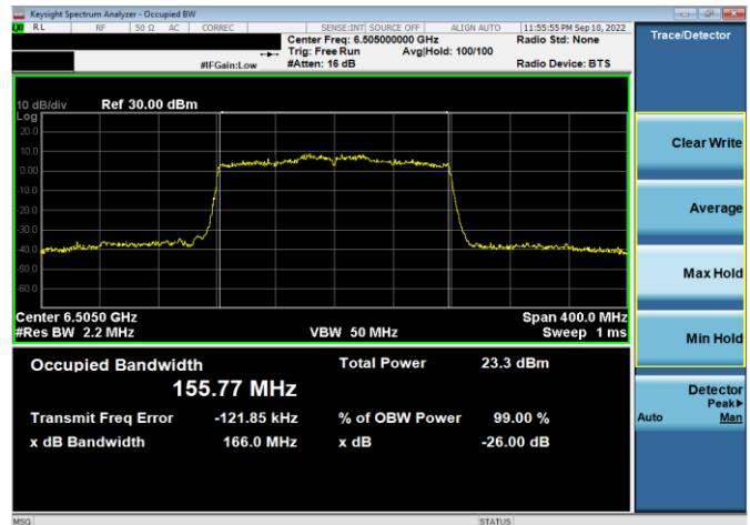
Plot 7-50. 26dB & 99% Bandwidth Plot Antenna WF5t (160MHz 802.11ax (UNII Band 6) – Ch. 111, MCS11)
