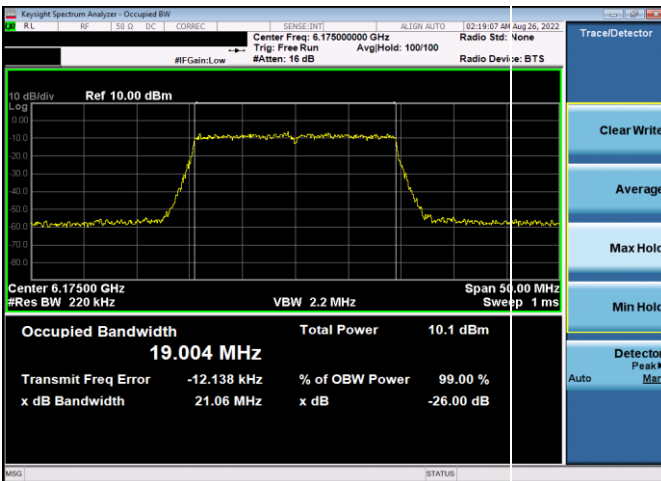
Plot 7-42. 26dB & 99% Bandwidth Plot Antenna WF5t (20MHz 802.11ax (UNII Band 5) – Ch. 45, MCS11)
