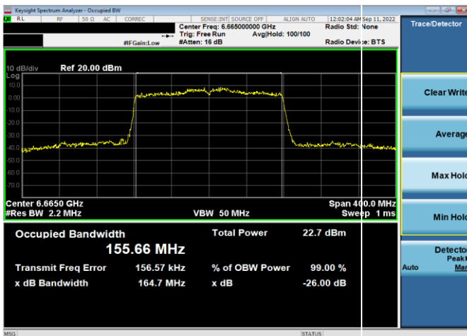
Plot 7-15. 26dB & 99% Bandwidth Plot Antenna WF5t (160MHz 802.11ax (UNII Band 7) - Ch. 143, MCS2)
