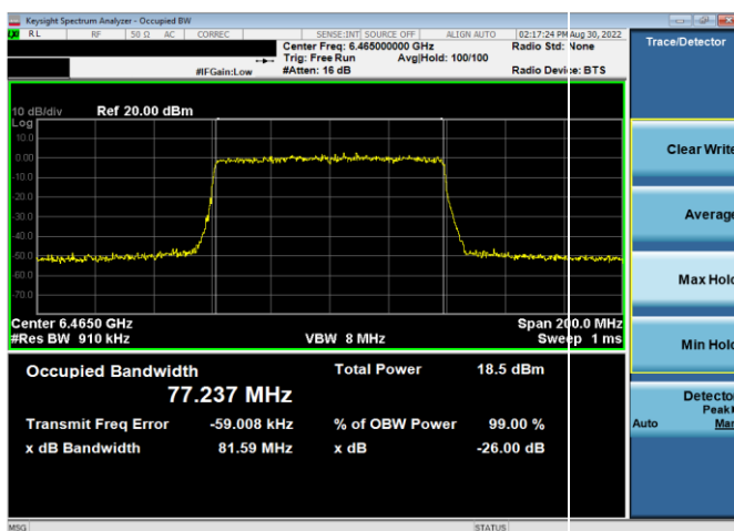
Plot 7-29. 26dB & 99% Bandwidth Plot Antenna WF5t (80MHz 802.11ax (UNII Band 6) – Ch. 103, MCS4)
