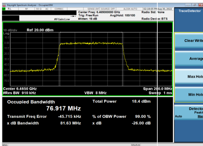
Plot 7-49. 26dB & 99% Bandwidth Plot Antenna WF5t (80MHz 802.11ax (UNII Band 6) – Ch. 103, MCS11)
