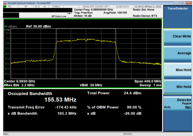
Plot 7-40. 26dB & 99% Bandwidth Plot Antenna WF5t (160MHz 802.11ax (UNII Band 8) – Ch. 207, MCS4)
