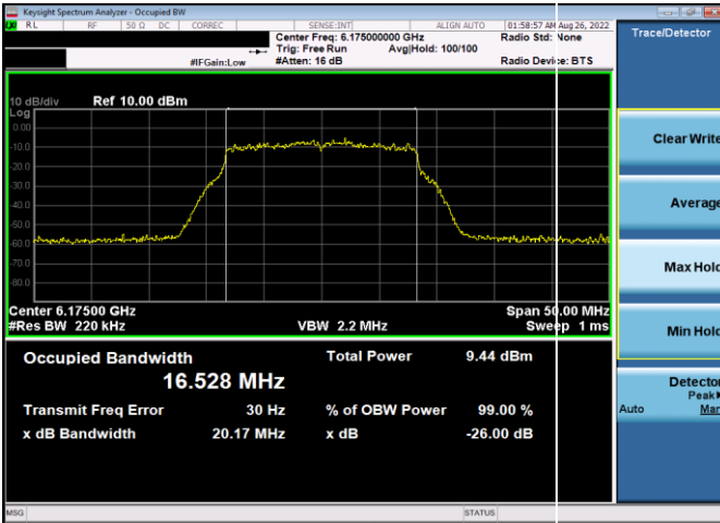
Plot 7-21. 26dB & 99% Bandwidth Plot Antenna WF5t (20MHz 802.11a (UNII Band 5) – Ch. 45, 24Mbps)
