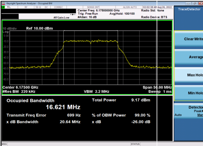
Plot 7-41. 26dB & 99% Bandwidth Plot Antenna WF5t (20MHz 802.11a (UNII Band 5) – Ch. 45, 54Mbps)
