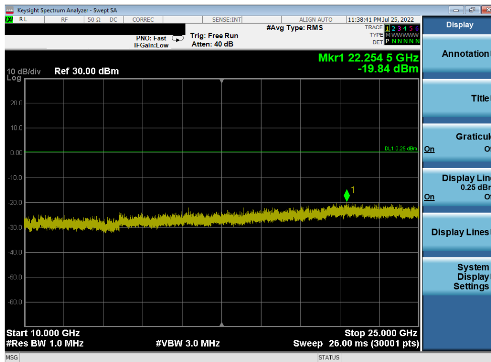
Plot 7-56. Conducted Spurious Plot Antenna WF7 (Bluetooth, GFSK, ePA – 2480 MHz)
