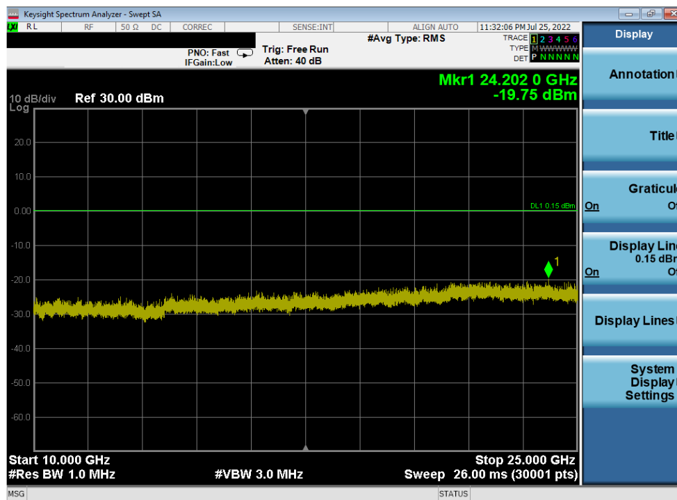
Plot 7-54. Conducted Spurious Plot Antenna WF7 (Bluetooth, GFSK, ePA 2441 MHz)
