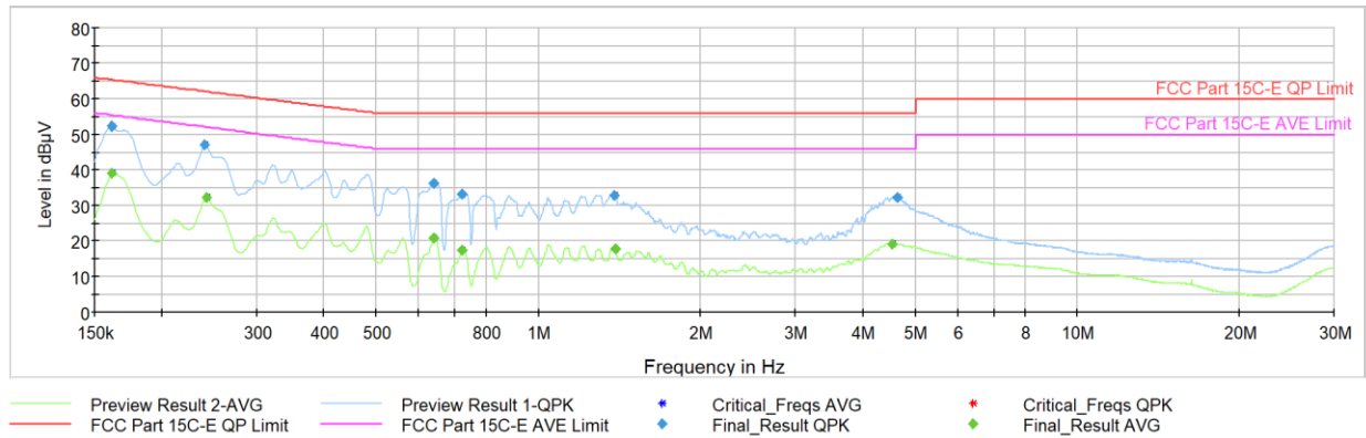
Plot 7-82. AC Line-Conducted Test Plot TxBF, 2.4GHz (N, GFSK ePA – 2402 MHz, with AC/DC Adapter)
