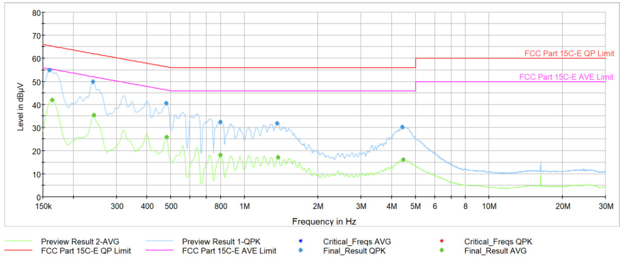
Plot 7-81. AC Line-Conducted Test Plot TxBF, 2.4GHz (L1, GFSK ePA – 2402 MHz, with AC/DC Adapter)
