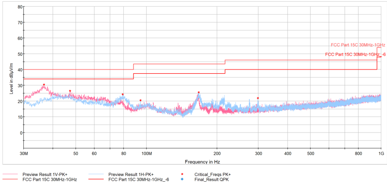
Plot 7-80. Radiated Spurious Emissions Below 1GHz TxBF, 2.4GHz (GFSK ePA – 2402 MHz, with AC/DC Adapter)
