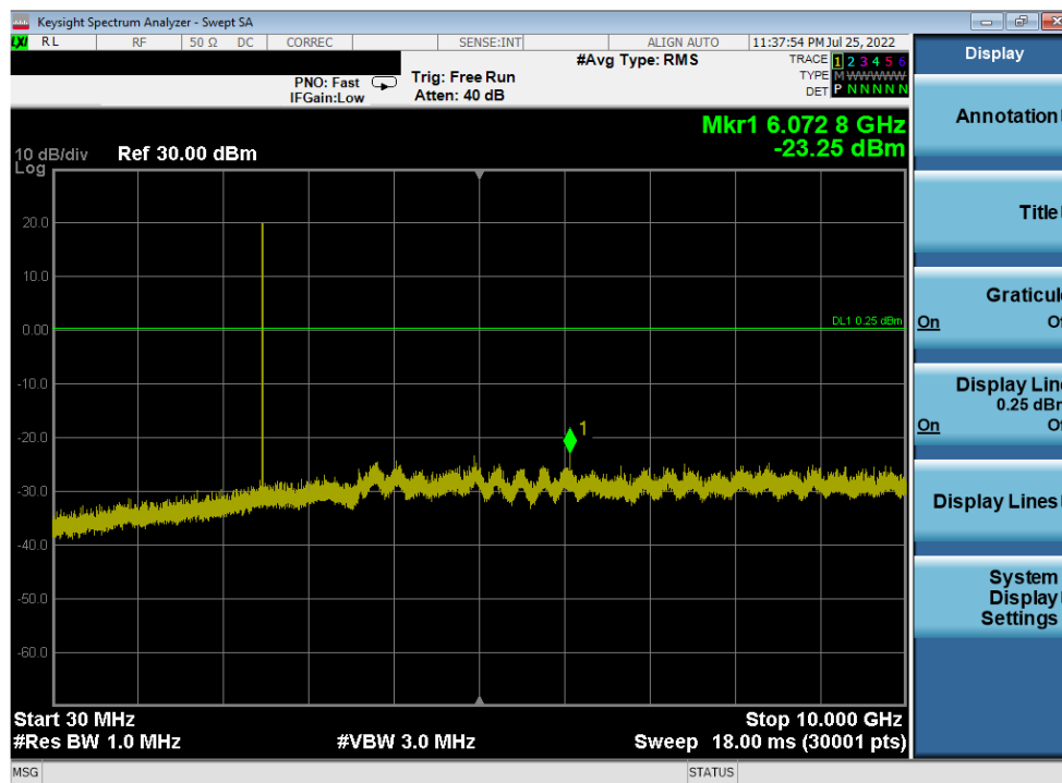
Plot 7-55. Conducted Spurious Plot Antenna WF7 (Bluetooth, GFSK, ePA – 2480 MHz)
